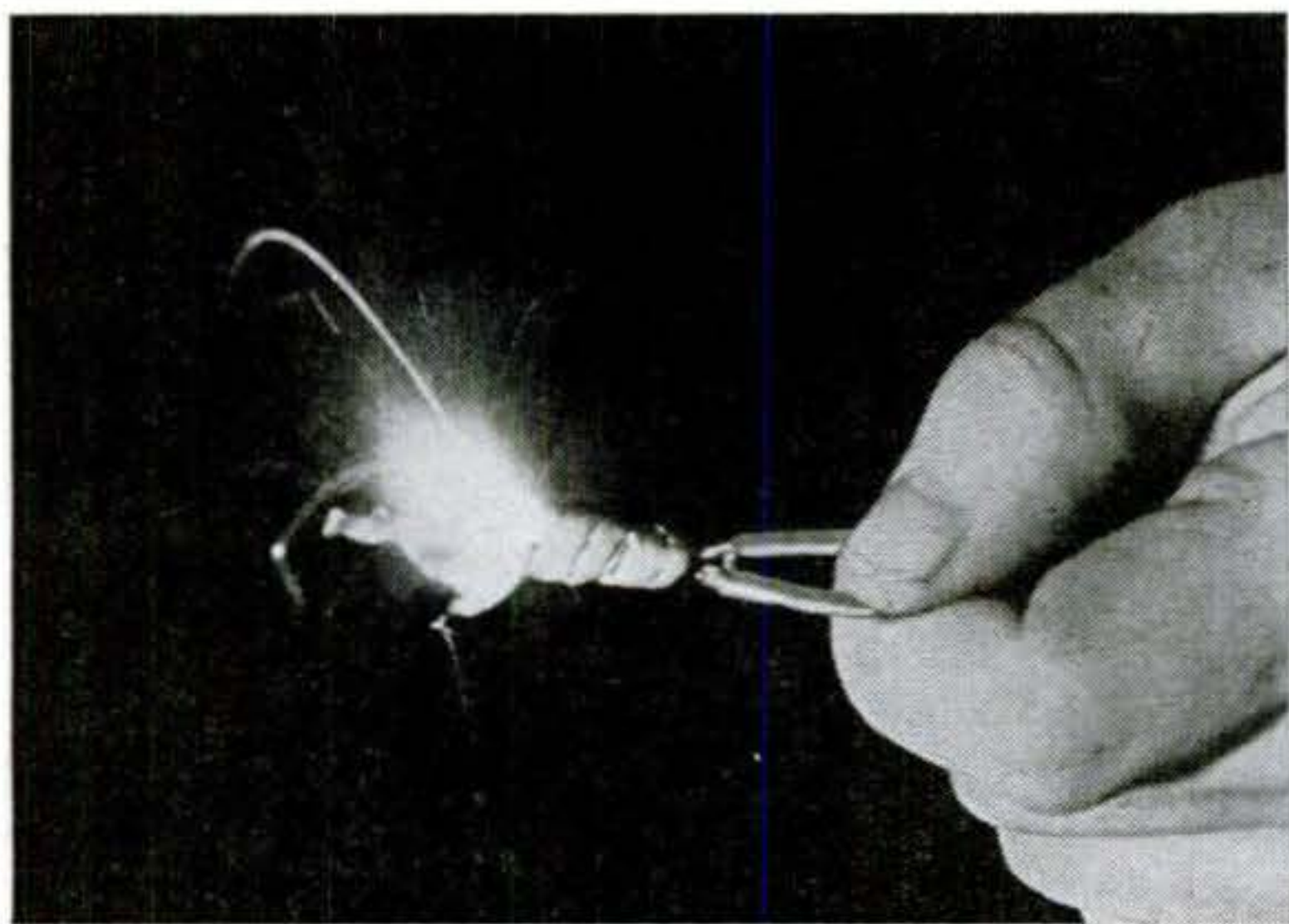
Flame and sparks follow the twist along the splice. Take precautions to protect clothing and woodwork from damage.
