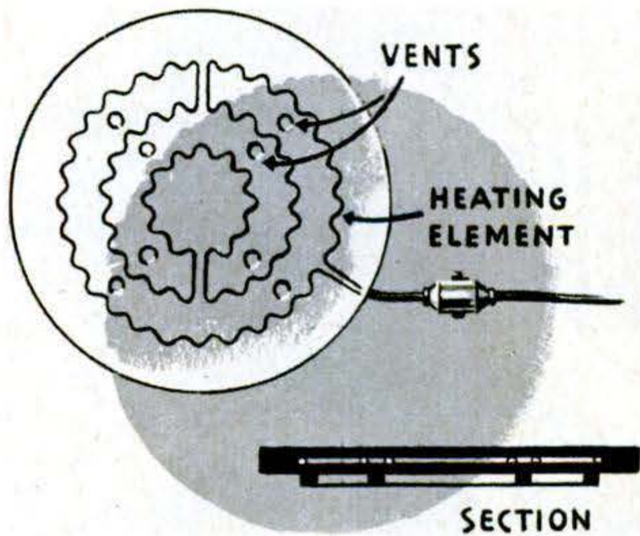
Hot Plate Made of Glass. By embedding circularly arranged wire coils in Pyrex glass, inventor John Bilan has devised a novel electric hot plate. The holes in the plate provide draft.
