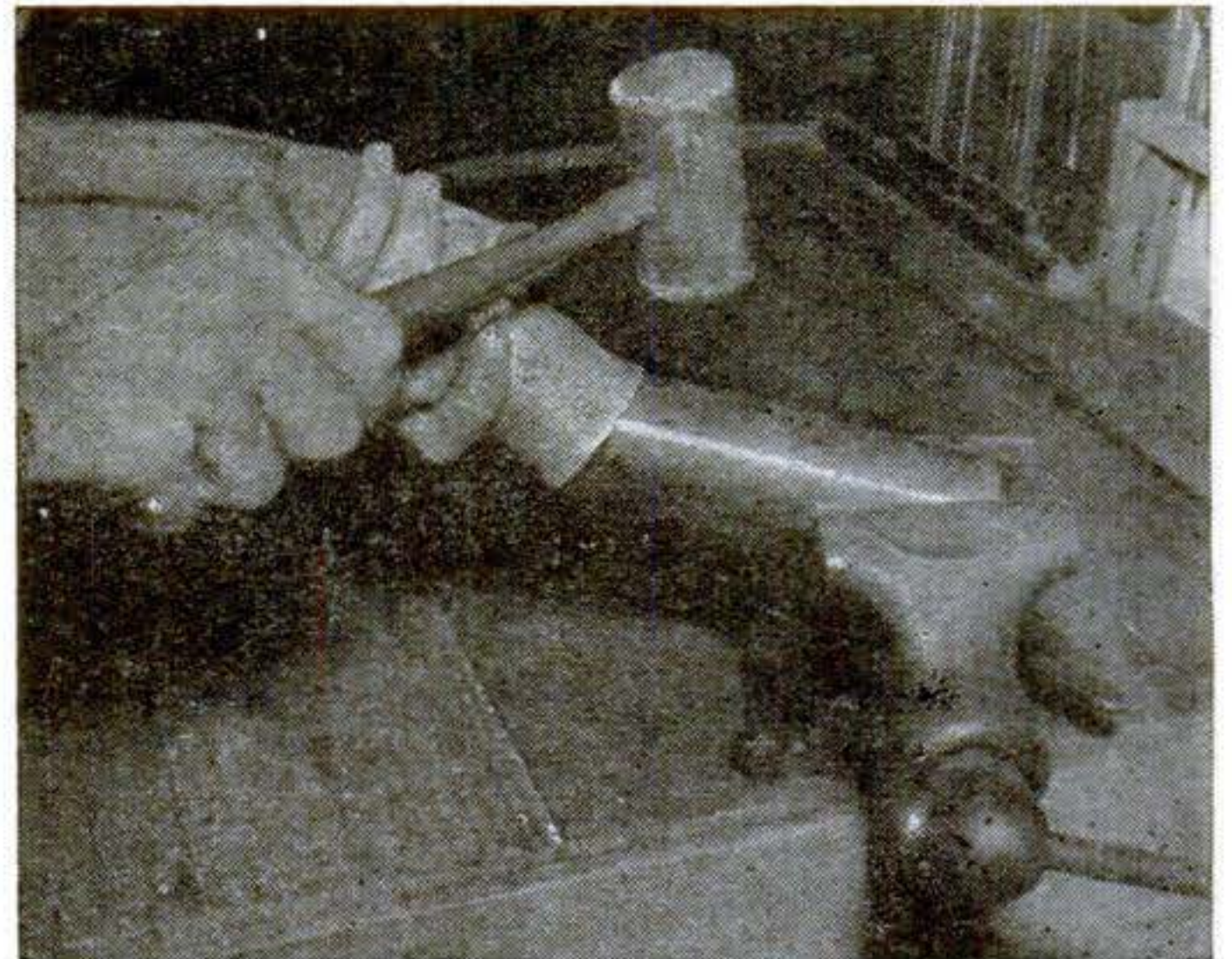
Flanging is done with the edge of a mallet while the tubing is revolved on a round bar. The hammer head and handle shown were turned on a lathe.
