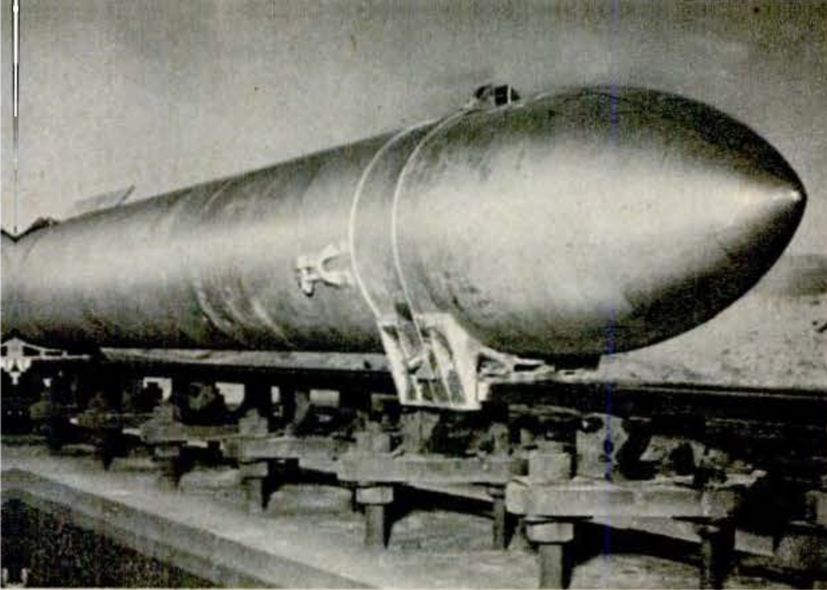
3. Manganese steel grips hold the one-ton projectile to the track. After leaving its 1,500-foot rail, the rocket flies another 500 feet true to the target.
