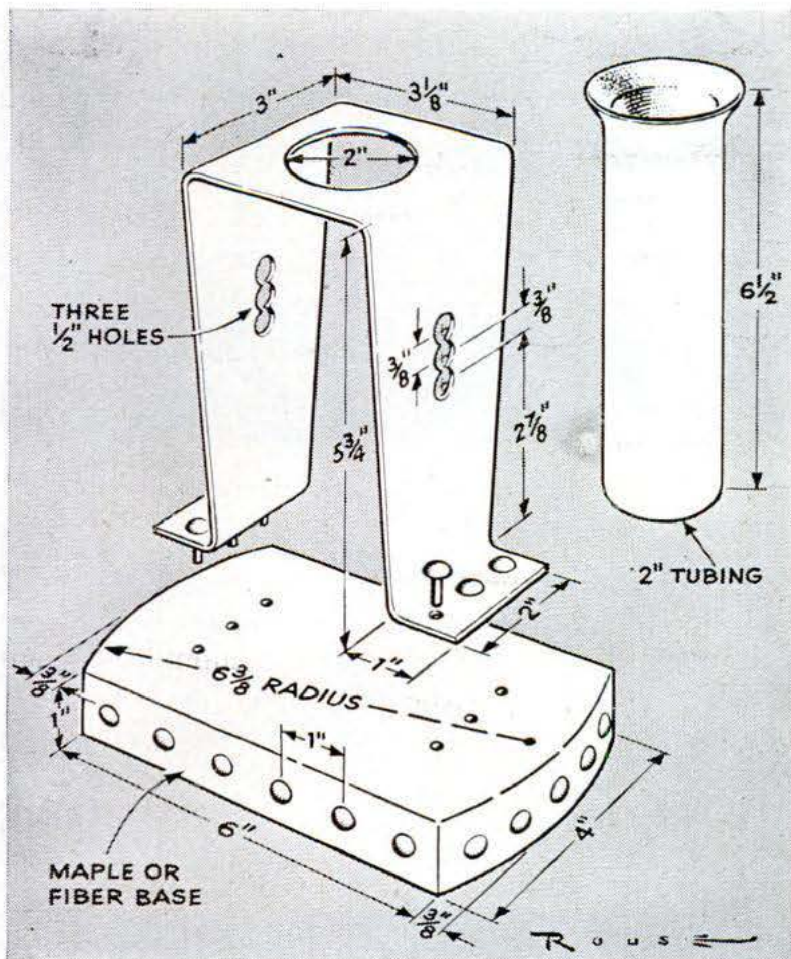
All parts of the table vase are shown in the drawing. The vase is a loose fit in the stand to permit removal for filling. Felt is glued to the bottom of the base.
