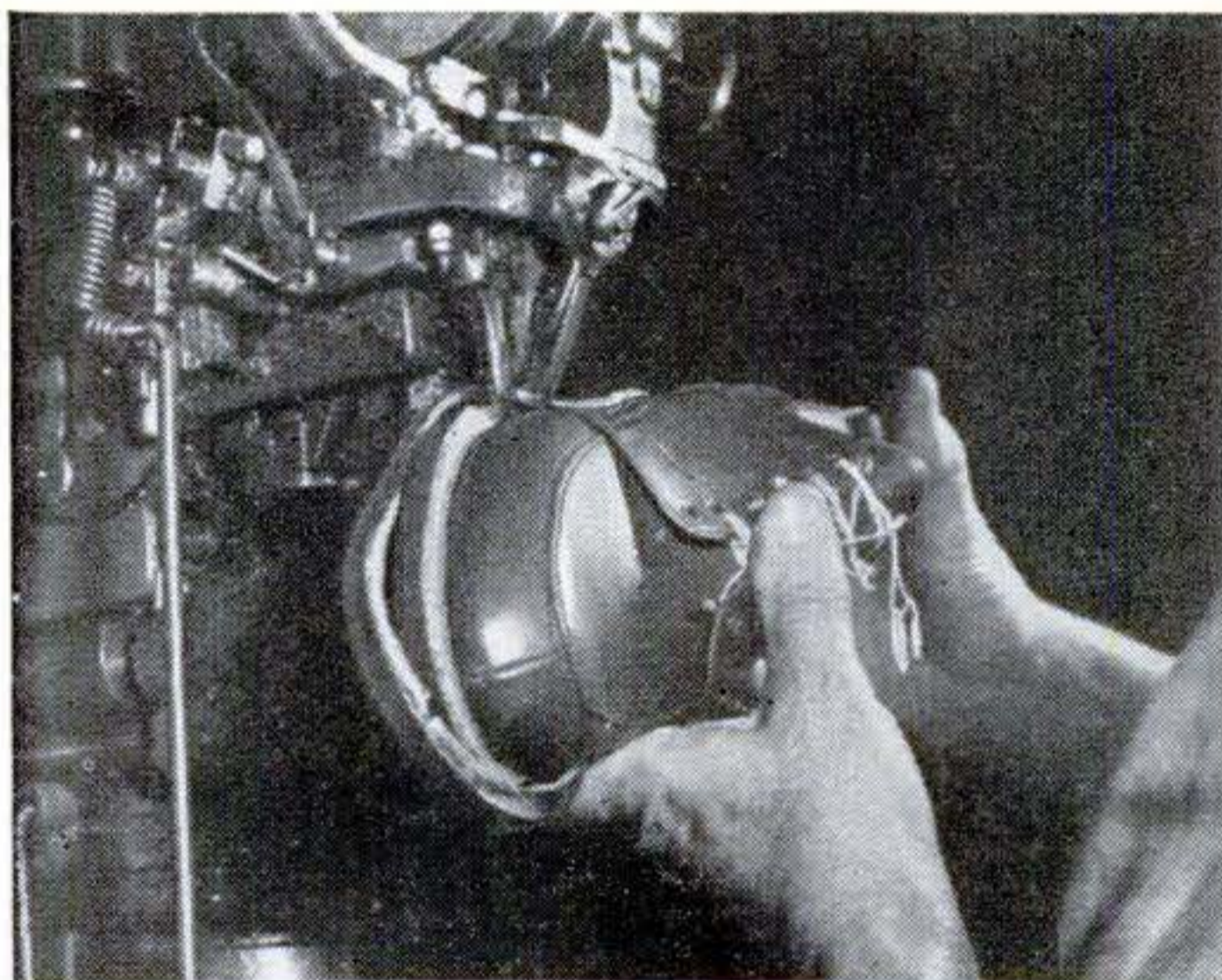
9. Of the 49 main operations, one of the most important is the rounding of the sole. This is done on another automatic machine that trims the excess from its edges and determines its final shape.
