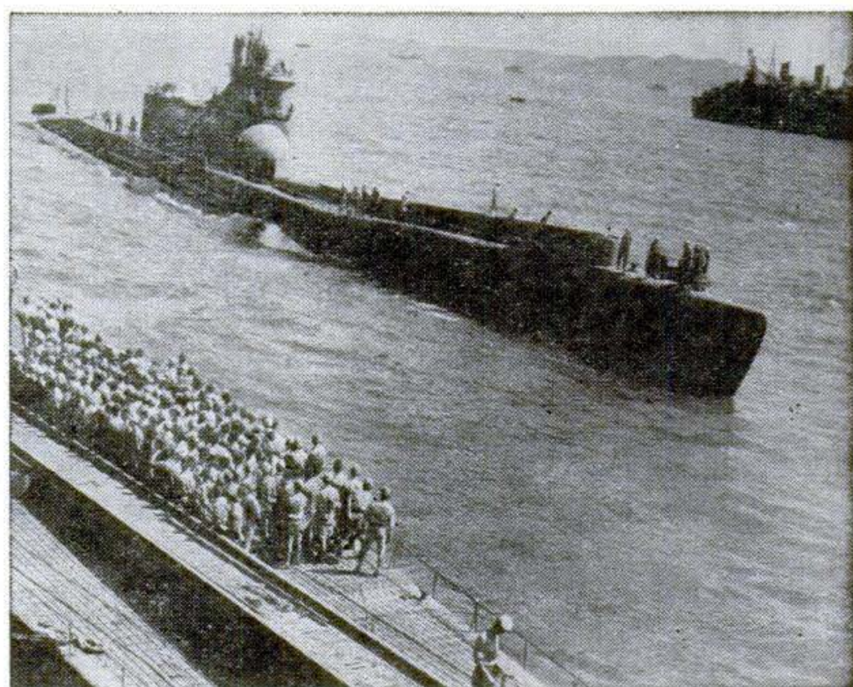
This angle shot of the I-14 gives a clear view of the railed ramp for launching planes carried in the space behind the bulbous hangar doors.
