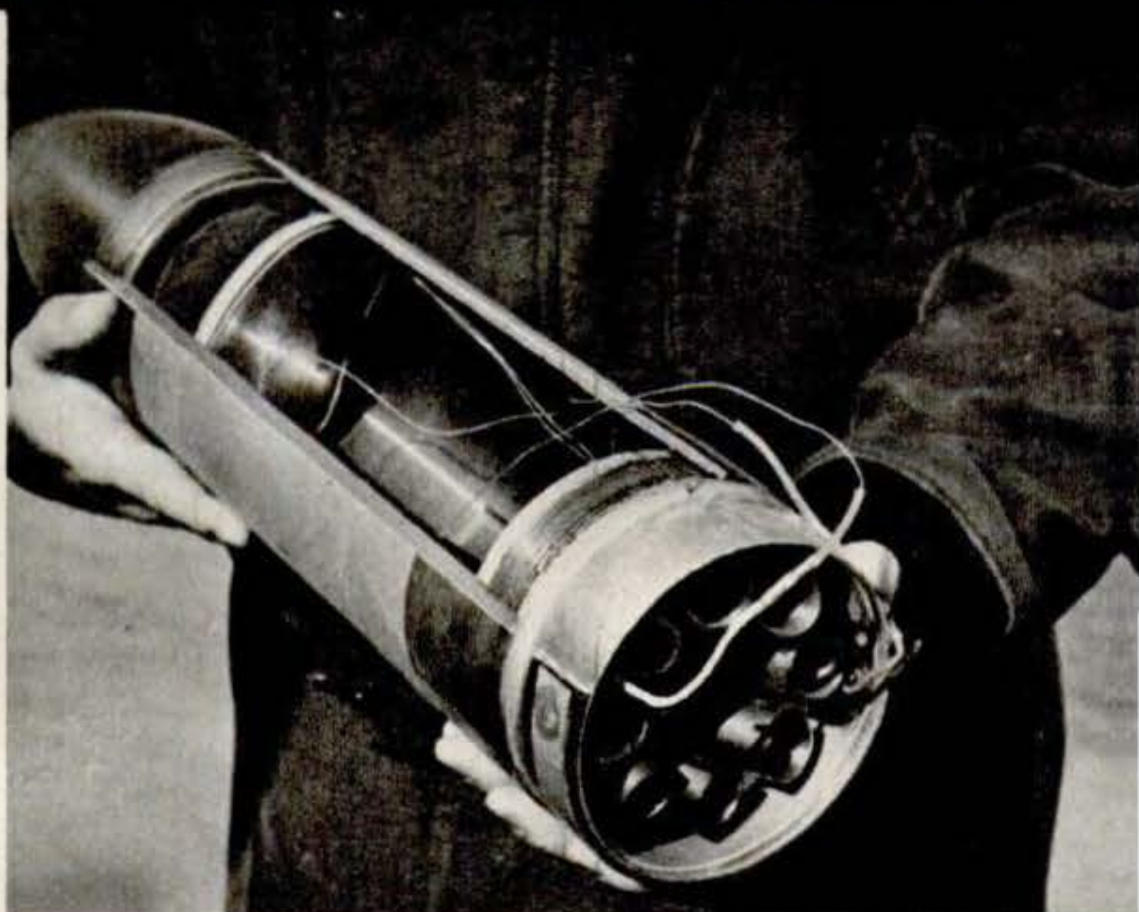
Cutaway of spinner rocket shows angled ports that make it whirl. Rockets are fired from two motor-driven drums, which can be reloaded during flight.
