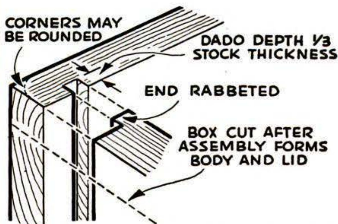
RABBET-AND-DADO CONSTRUCTION
