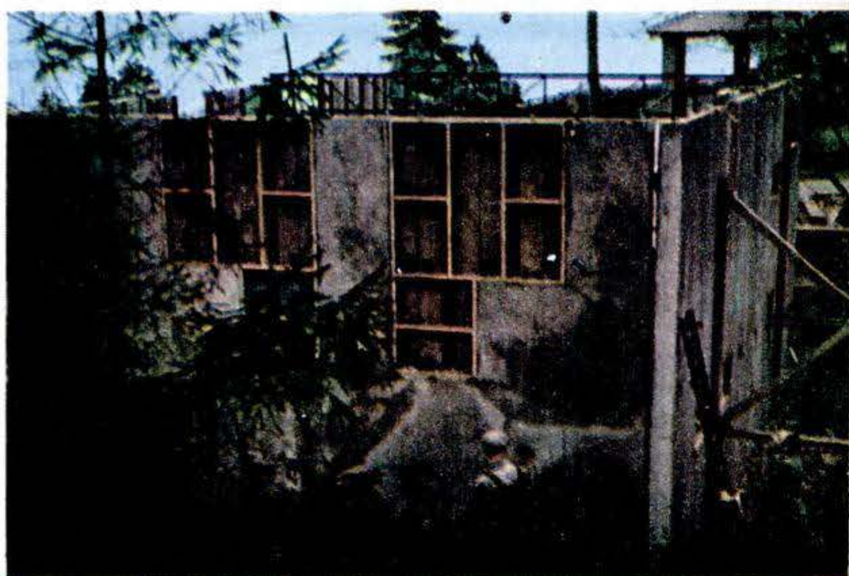
Two walls in place. Corner seam will be made watertight with impregnated fabric, packed with oakum and covered with caulking. Meanwhile, temporary trusses hold walls and support metal forms for casting roof and floor.
