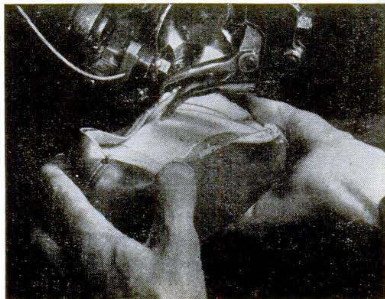
6. The side-lasting machine pulls the upper part of the shoe down tight over the wooden form, known as a last, around which the shoe is molded. The shoe is then stapled to the last with small metal tacks.
