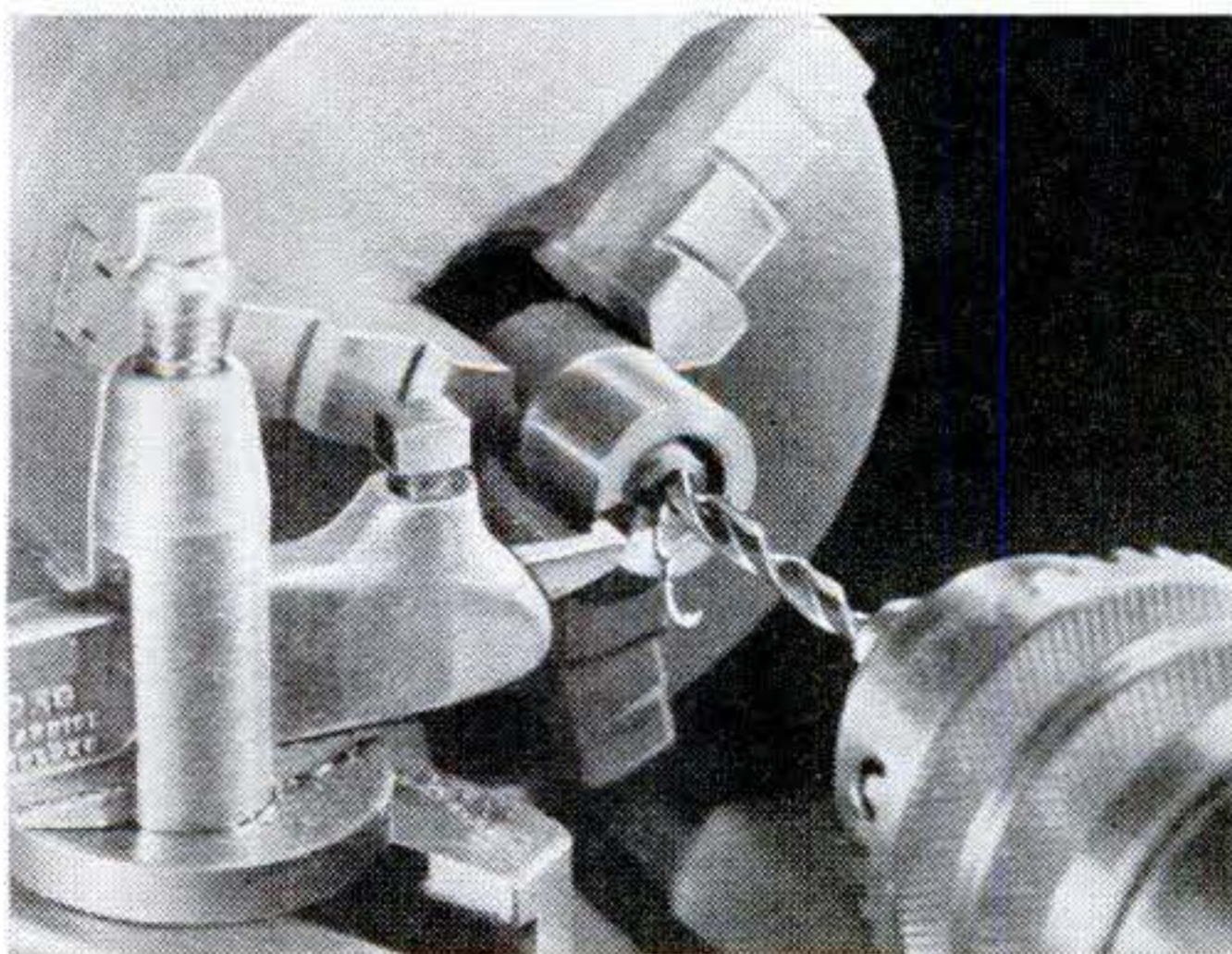
Stock for the crosshead is turned to a sliding fit in the main-column bore; then one end is recessed and turned to shape. The piece is also drilled and tapped for the piston rod while chucked.
