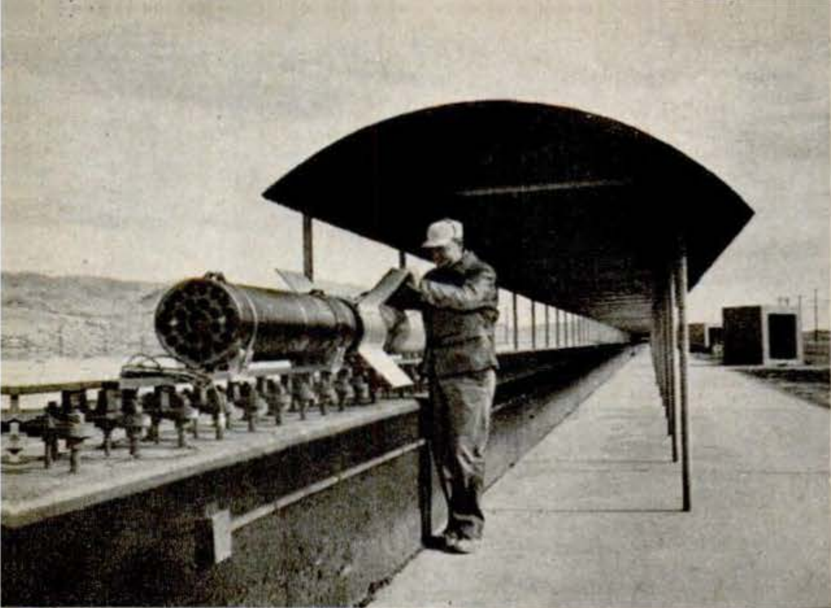
1. Tiny Tim is groomed for a railroad take-off. Its booster, or auxiliary motor, is nearest the camera. Metal roof protects track from heat of desert sun.
