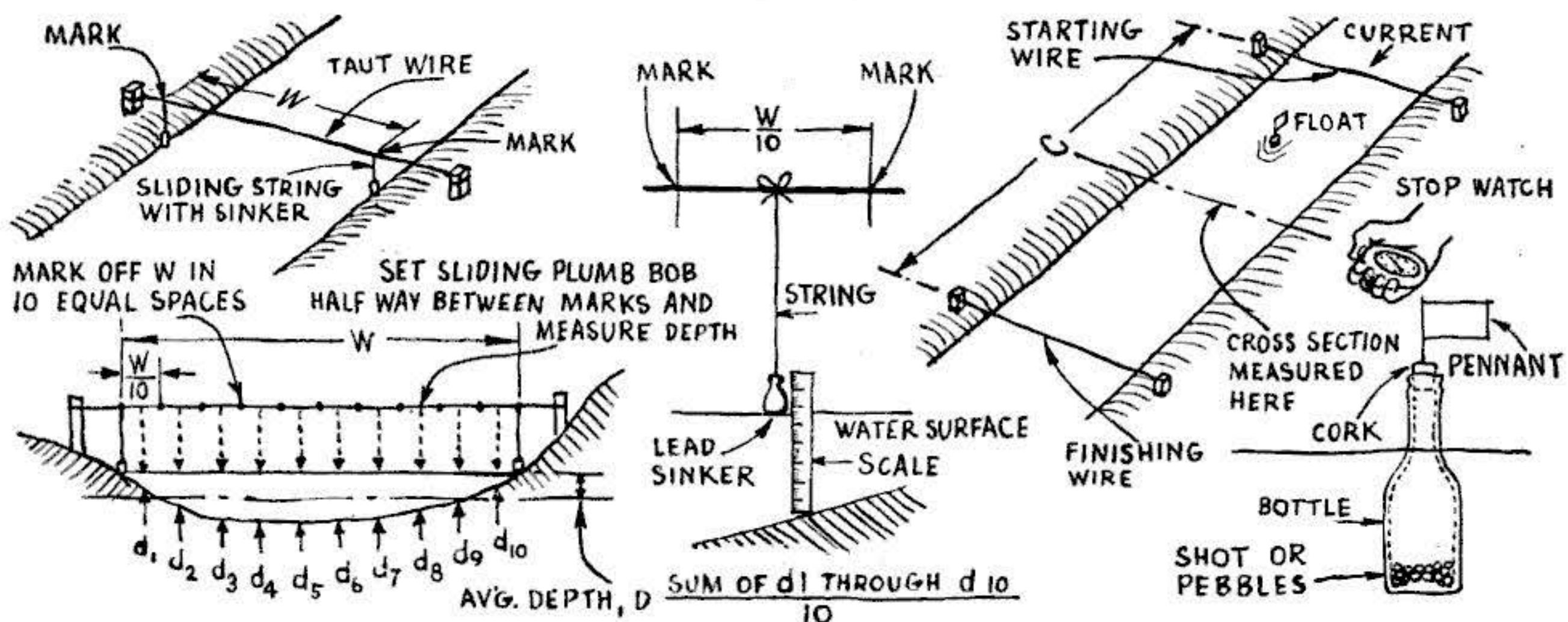
FIG. 3. FLOAT METHOD OF MEASURING FLOW
