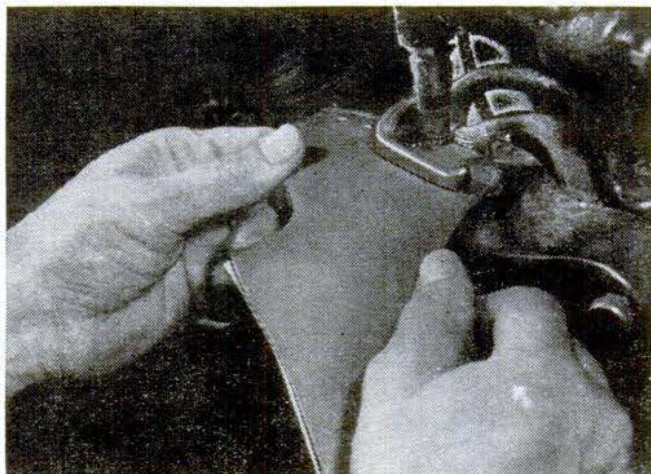
4. The eyeleting machine, handling up to 4,000 shoes a day, stamps out two rows of metal-rimmed perforations for the laces. On some shoes, the eyelets are attached on the inside and cannot be seen.
