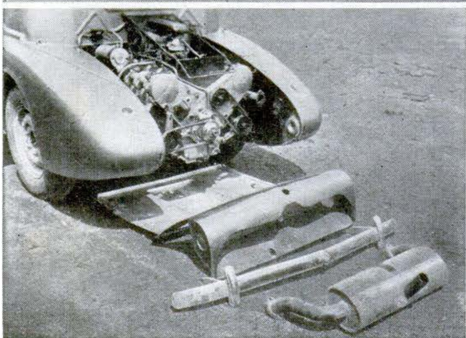
Built of light materials, the Tatra engine adds little more weight than is usually found at the rear of a car. Shown in black above, the entire power unit readily rolls free for servicing after the engine cover, bumper, and muffler are detached and the rear of the car is jacked up. As illustrated directly above, the Tatra rests on a Y-shaped steel backbone.
