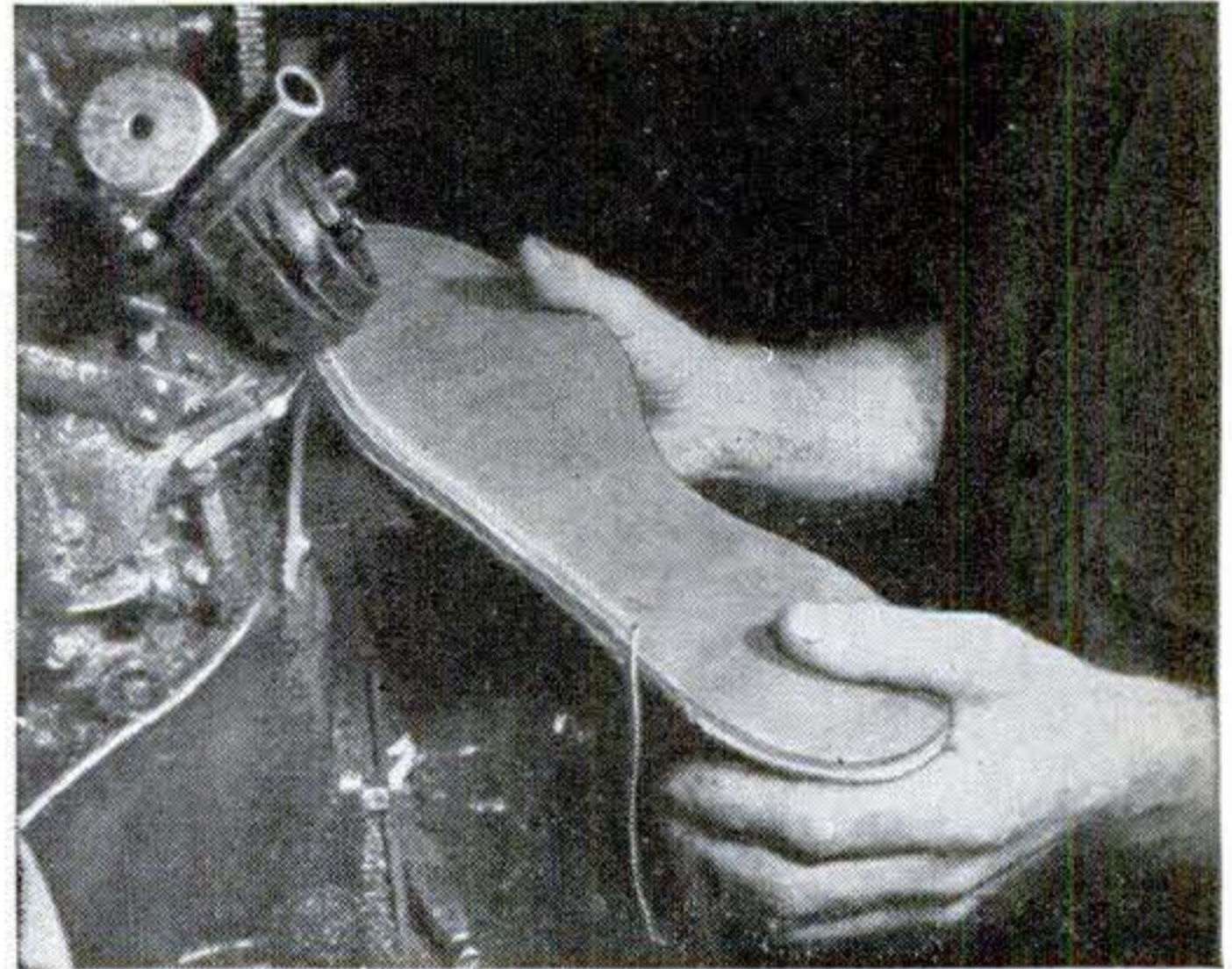
10. The sole, cut from the tough kidney portion of South American steer hides, is first cemented and then sewed onto the bottom of the shoe with a fine linen thread that can withstand a pull of 58 pounds.
