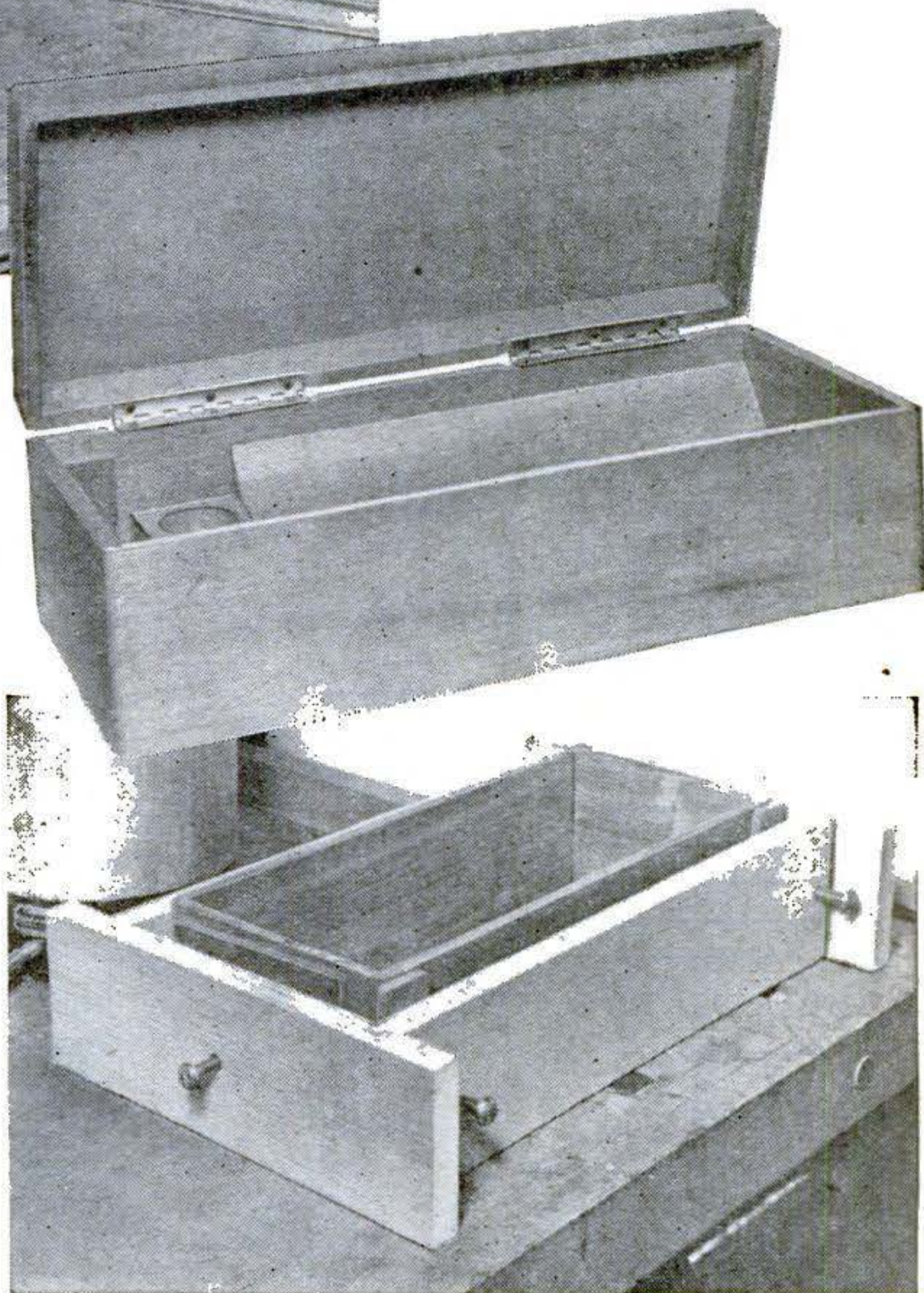
An efficient clamp for gluing dado-and-rabbit joints applies pressure at the corners and ends. Wedges or screws are used.
