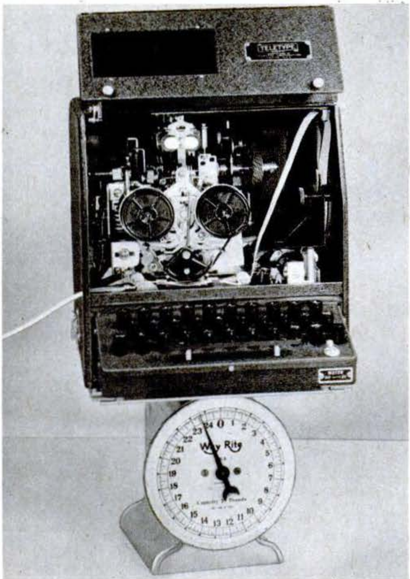
Teletype Goes Aloft. To provide printed communications for aircraft in flight, Bell Telephone technicians developed the teletype printer at left. The printer itself weighs less than 24 pounds, and a complete airborne installation adds only about 35 pounds to a plane's load.
