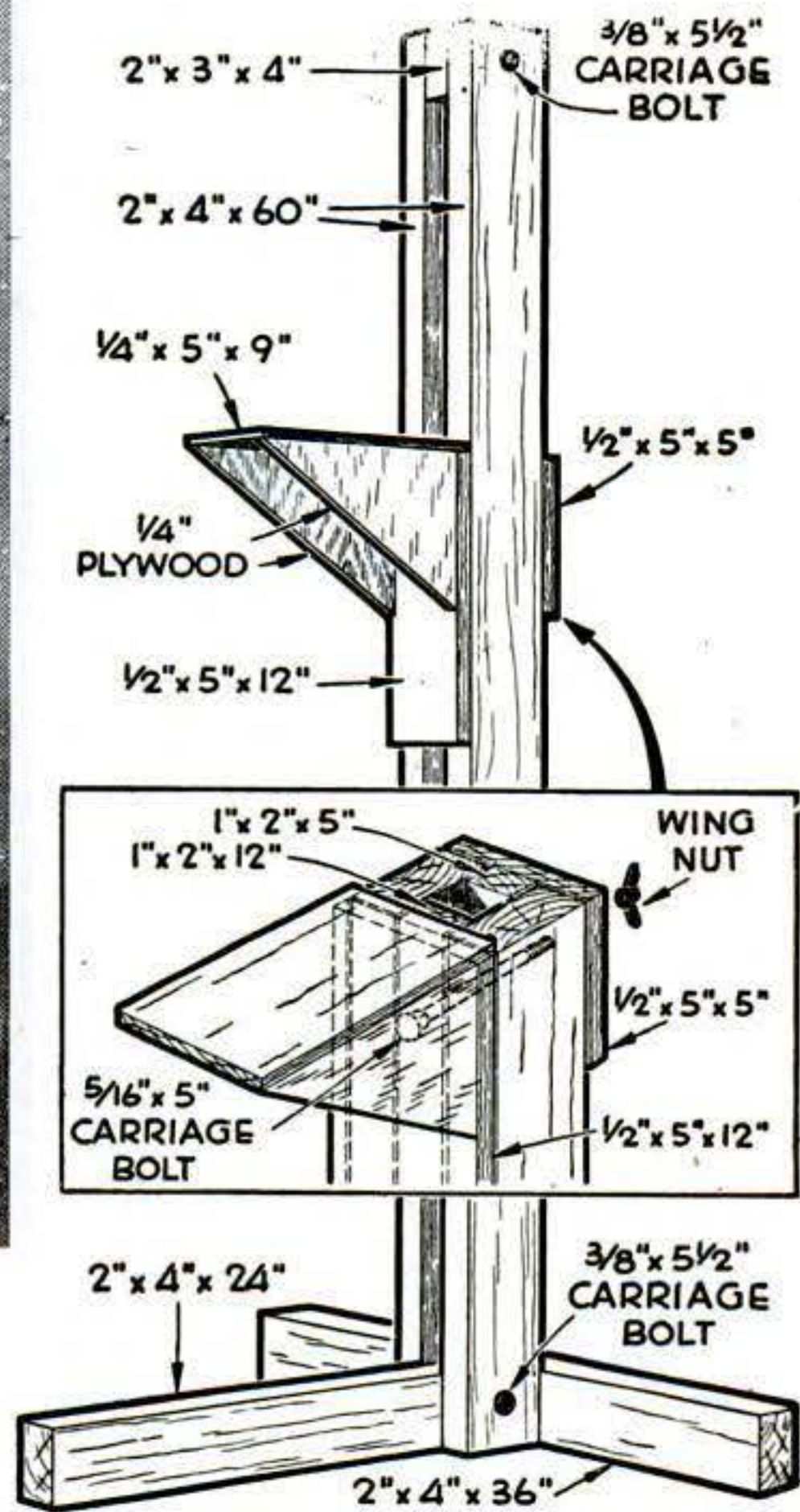
Despite its cumbersome appearance, this studio stand is readily maneuverable. One wing nut loosens the camera shelf for quick adjustment to any level. The base slides on dome gliders.
