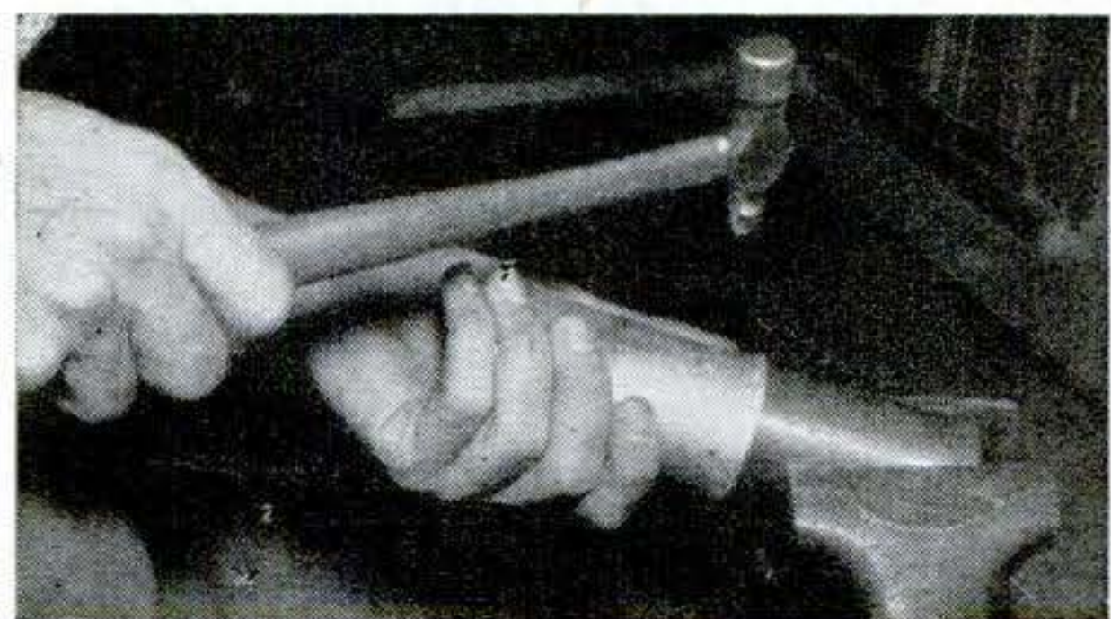
Instead of spot-polishing, a hammered effect can be obtained by peening the entire surface of the tubing with a ball-peen hammer.
