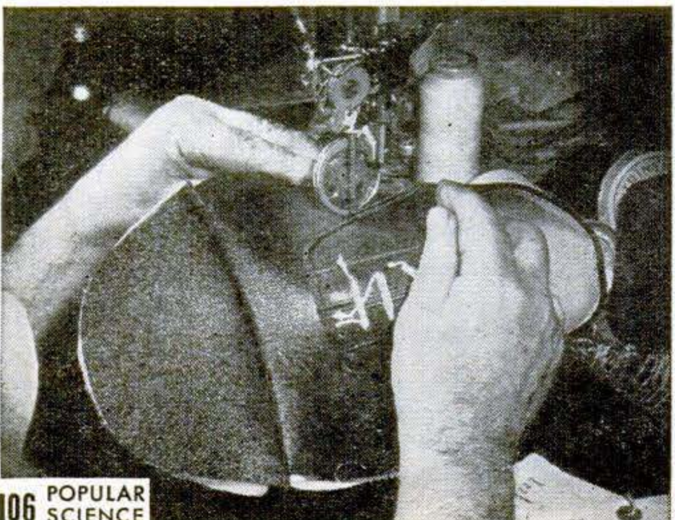
5. Silk threads are used for permanent stitching of the upper parts of the shoe, which are first cemented together to insure perfect alignment. Only the center portion of the hide is used for these parts.
