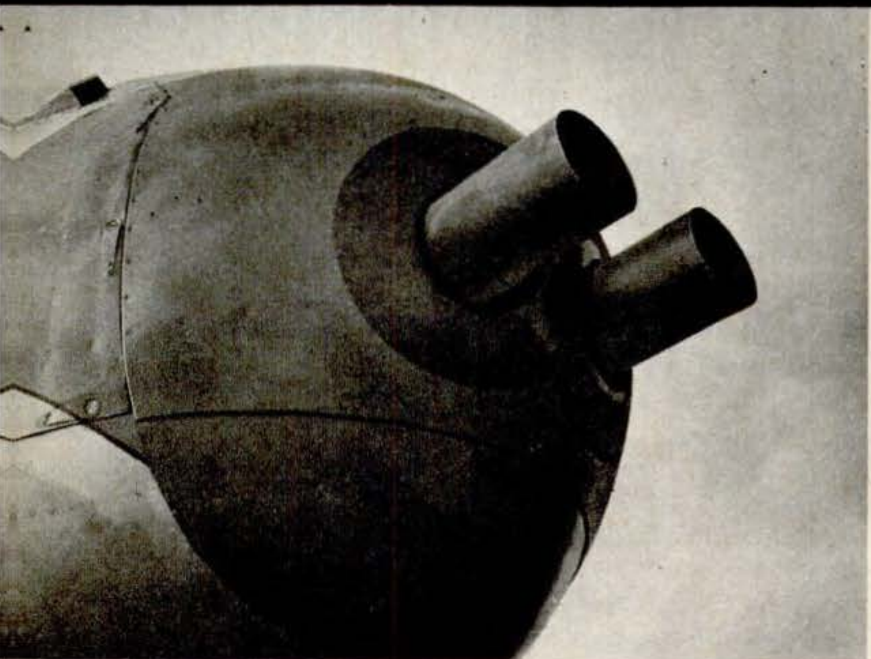
With a new automatic revolving launcher, these twin tubes in a plane's nose fire a whole salvo of five-inch spinner rockets in a matter of seconds.
