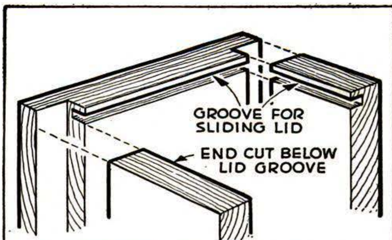
RABBETED CONSTRUCTION
