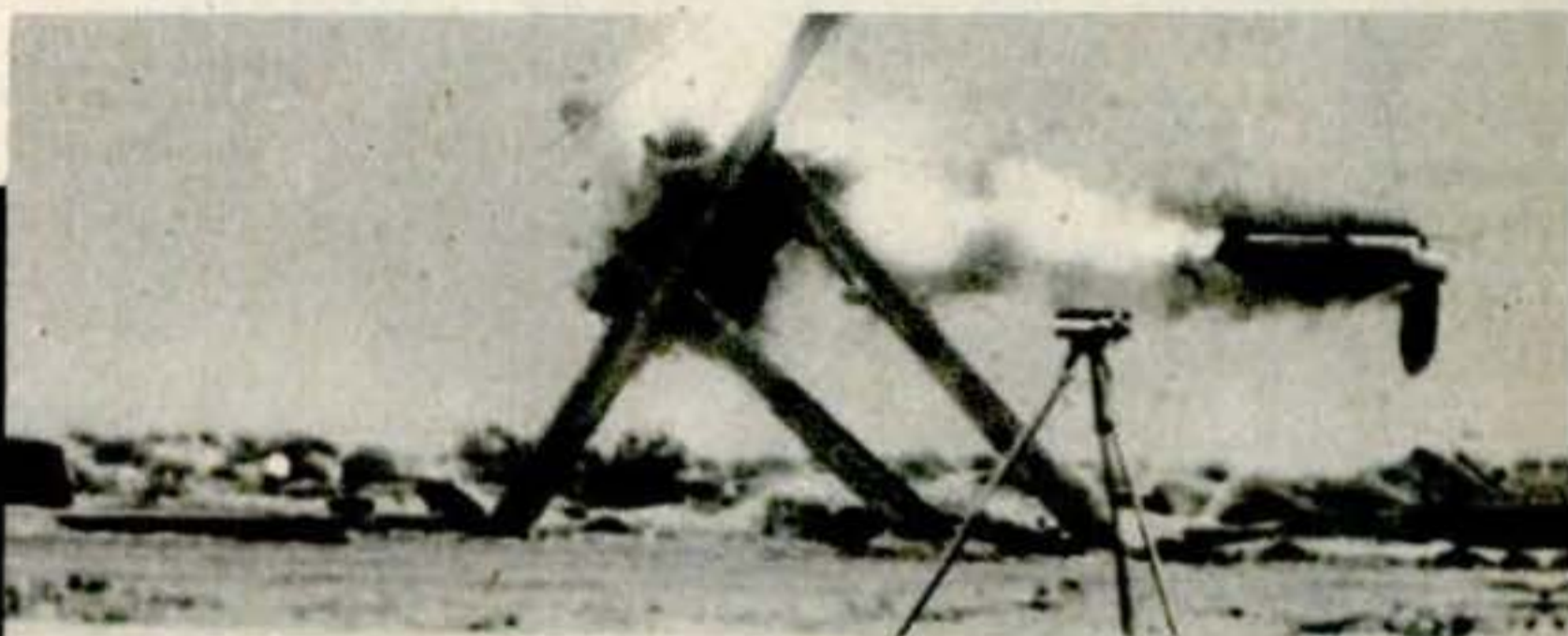
3. Manganese steel grips hold the one-ton projectile to the track. After leaving its 1,500-foot rail, the rocket flies another 500 feet true to the target.
