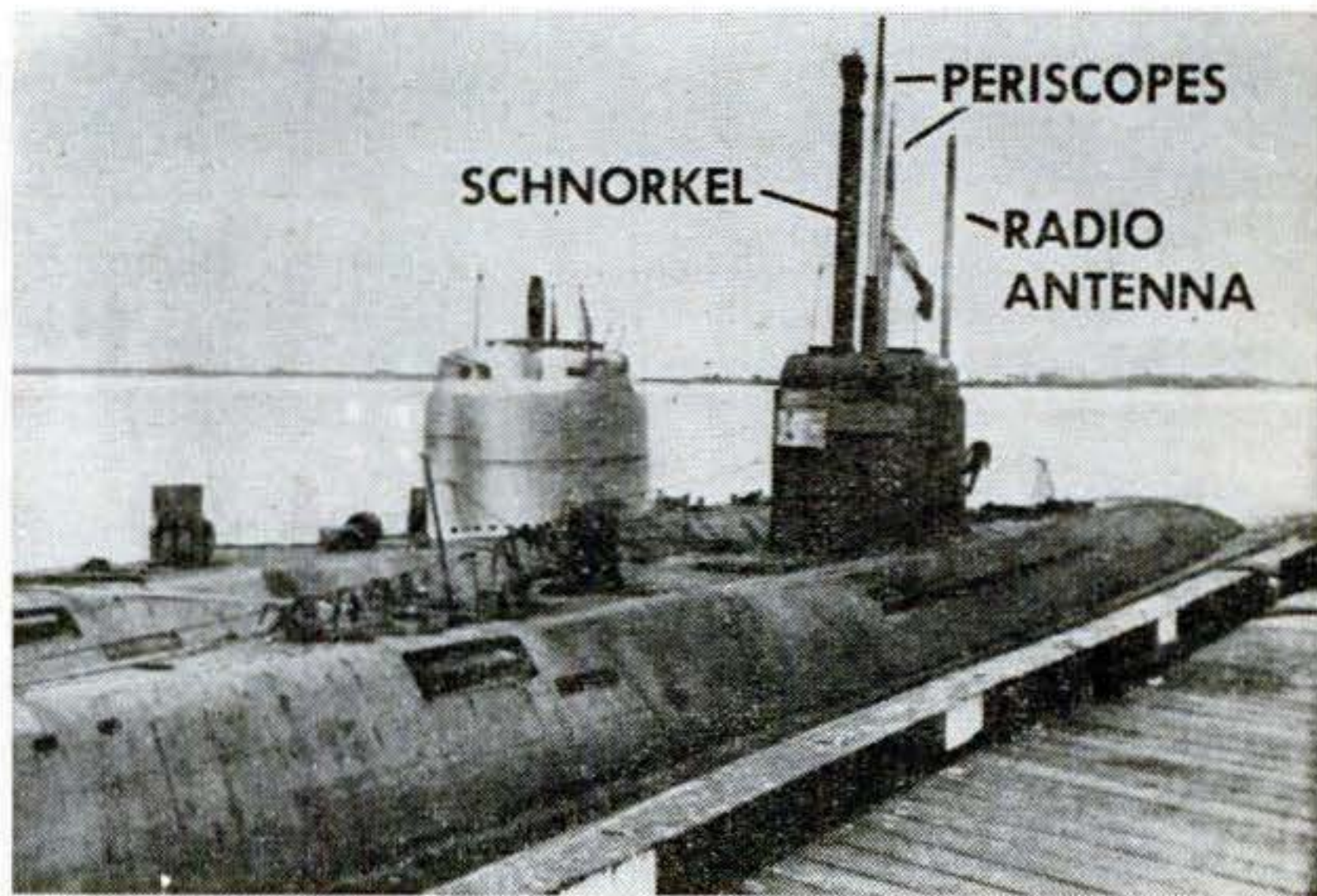
Two captured Type 21s. Schnorkel—breather tube—and elaborate periscopes and radio antennas are extended on sub at right, retracted on craft at left.
