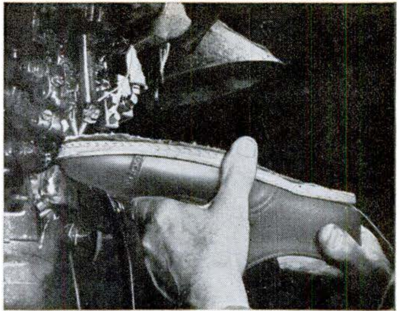
8. To form a foundation for the bottom of the shoe, a welt, or leather strip, is sewed around the rim of the shoe with a wax-coated thread. A steel shank is then inserted to form a firm support for the arch.
