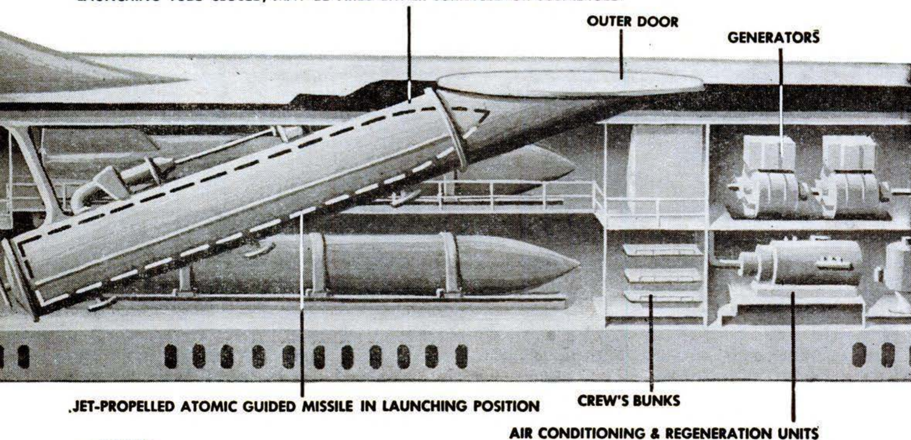
LAUNCHING TUBE CLOSED; MAY BE FIRED EITHER SURFACED OR SUBMERGED
