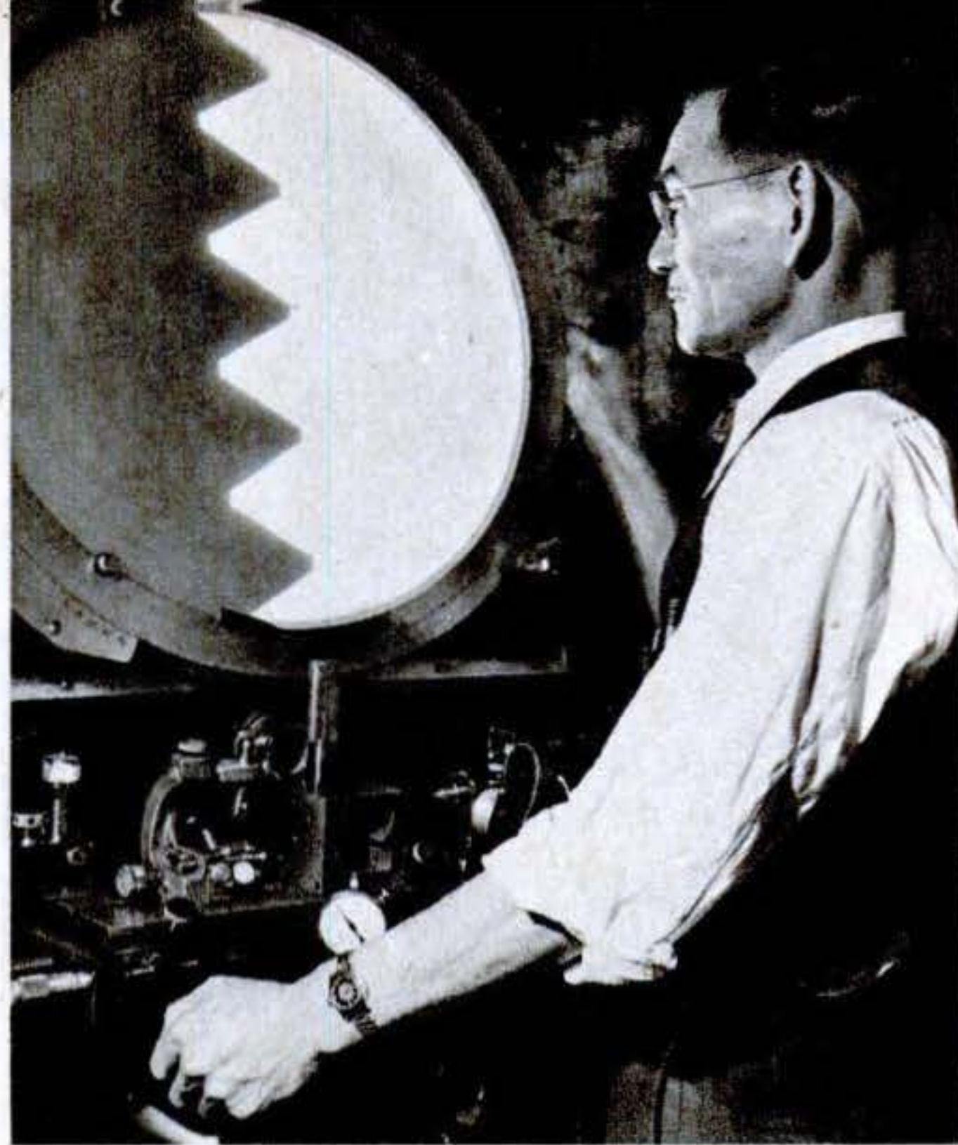
It Magnifies Mistakes. The giant teeth shown by this Ford "comparator," used to test precision gauges, are really magnified shadows of screw threads in the gauge visible below the screen.
