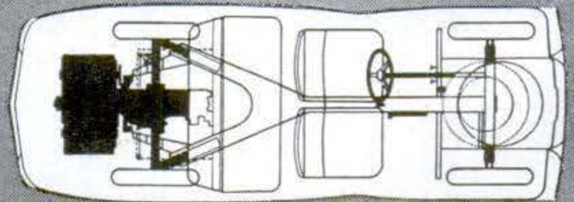
Built of light materials, the Tatra engine adds little more weight than is usually found at the rear of a car. Shown in black above, the entire power unit readily rolls free for servicing after the engine cover, bumper, and muffler are detached and the rear of the car is jacked up. As illustrated directly above, the Tatra rests on a Y-shaped steel backbone.
