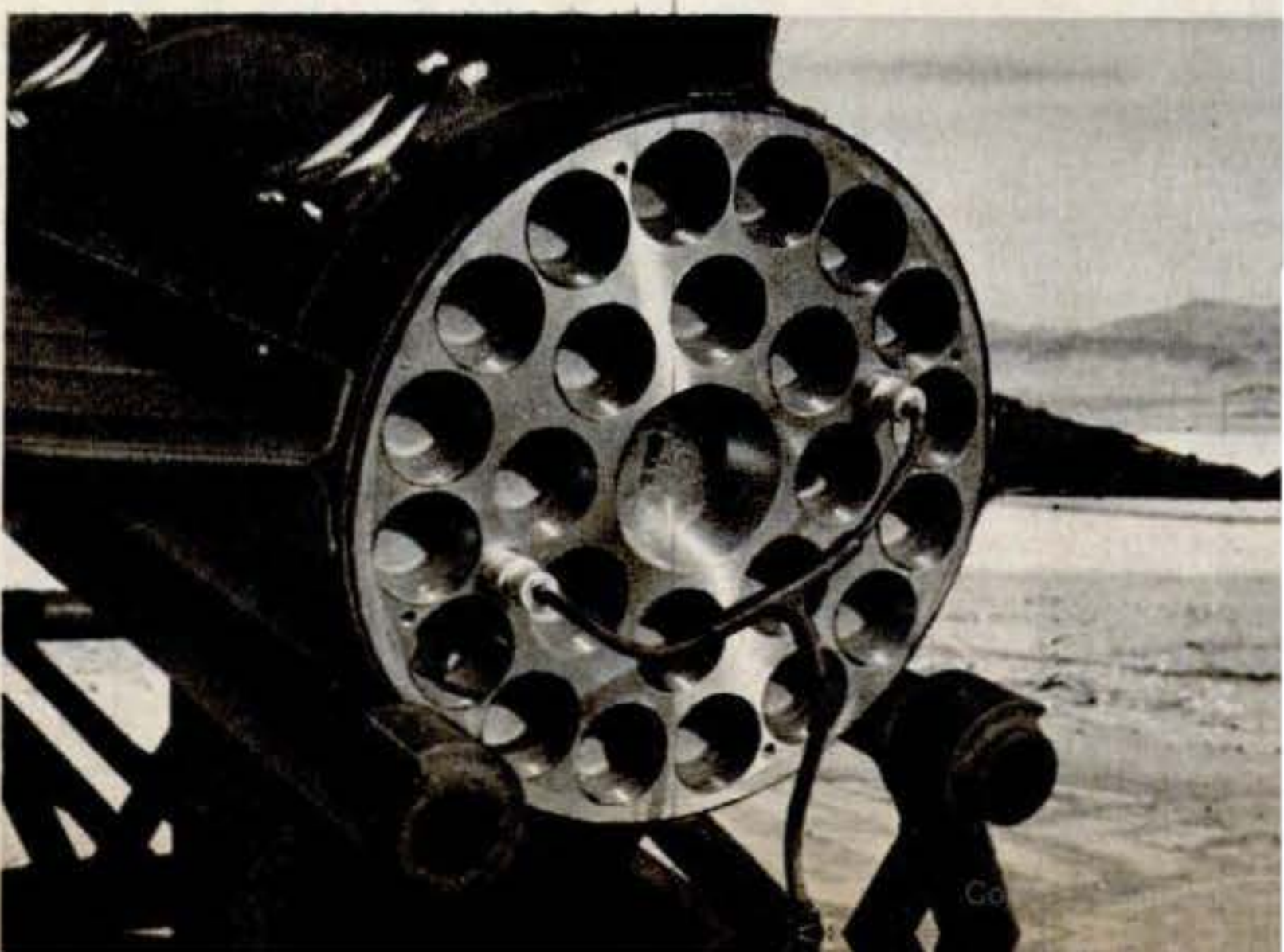
Closeup of Big Dick's nozzle plate shows multiple ports through which burning gas escapes. Electrical contacts are in position, ready for firing.
