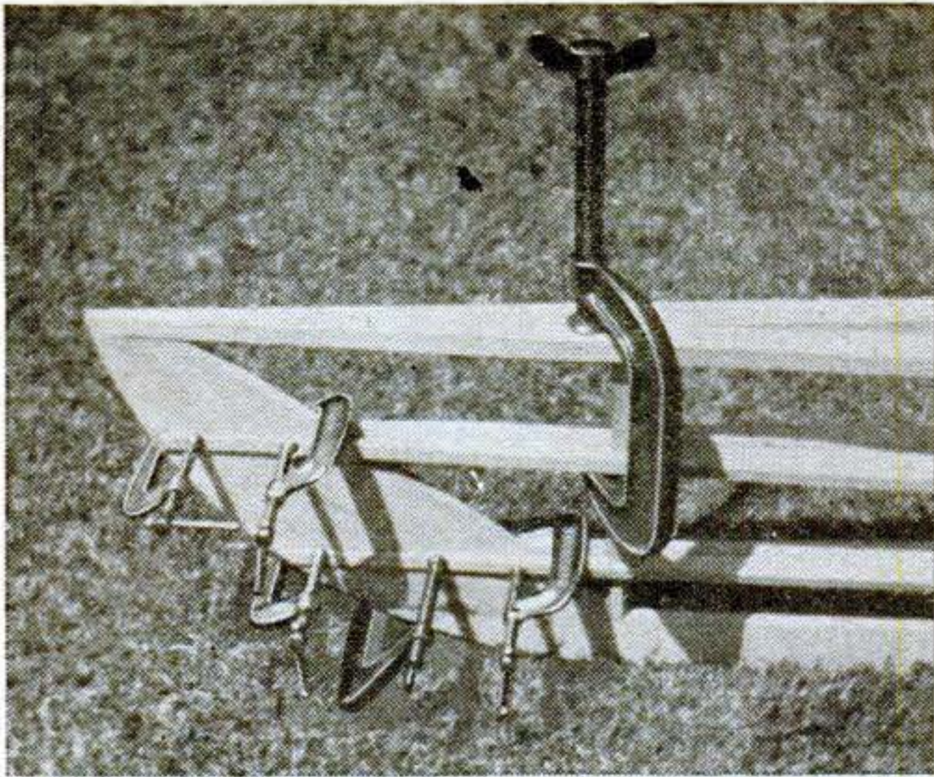
Kerfing may help in bending hull stringers fore and aft. Clamps hold them while the glue sets.
