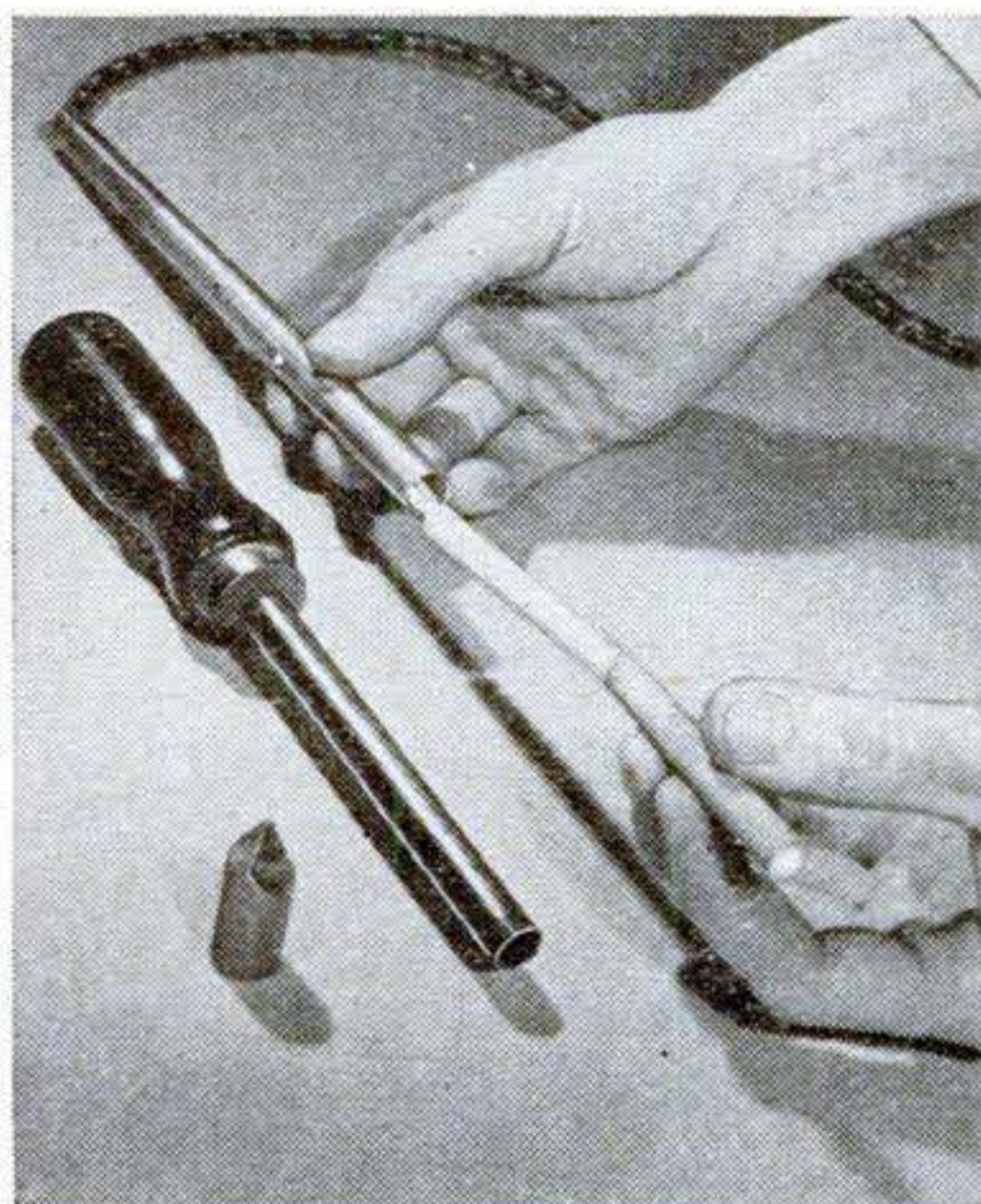
After enlarging the inside diameter of a 12" length of \frac{1}{4} " brass pipe for 4" at one end, insert the resistance element from a 60-watt soldering iron.
