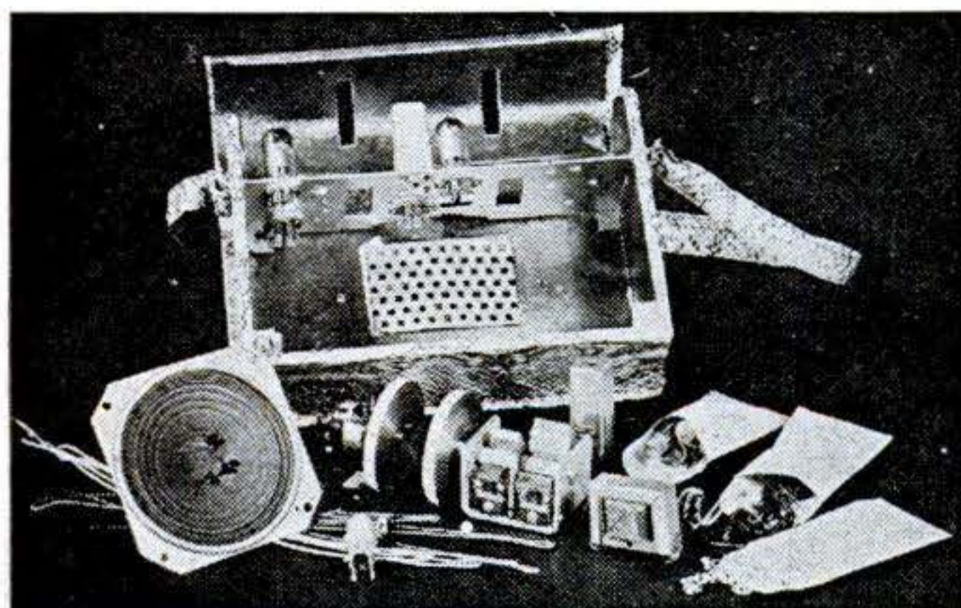
HANDBAG RADIO. Shoulder-strap pocket-books can please the ear as well as the eye. The complete four-tube superhet handbag shown at right above is made by the ARC
