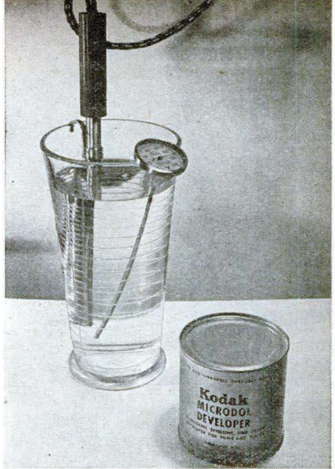
Built around the heating element from a soldering iron, this immersion heater quickly raises a photo solution to the temperature needed for good work.
