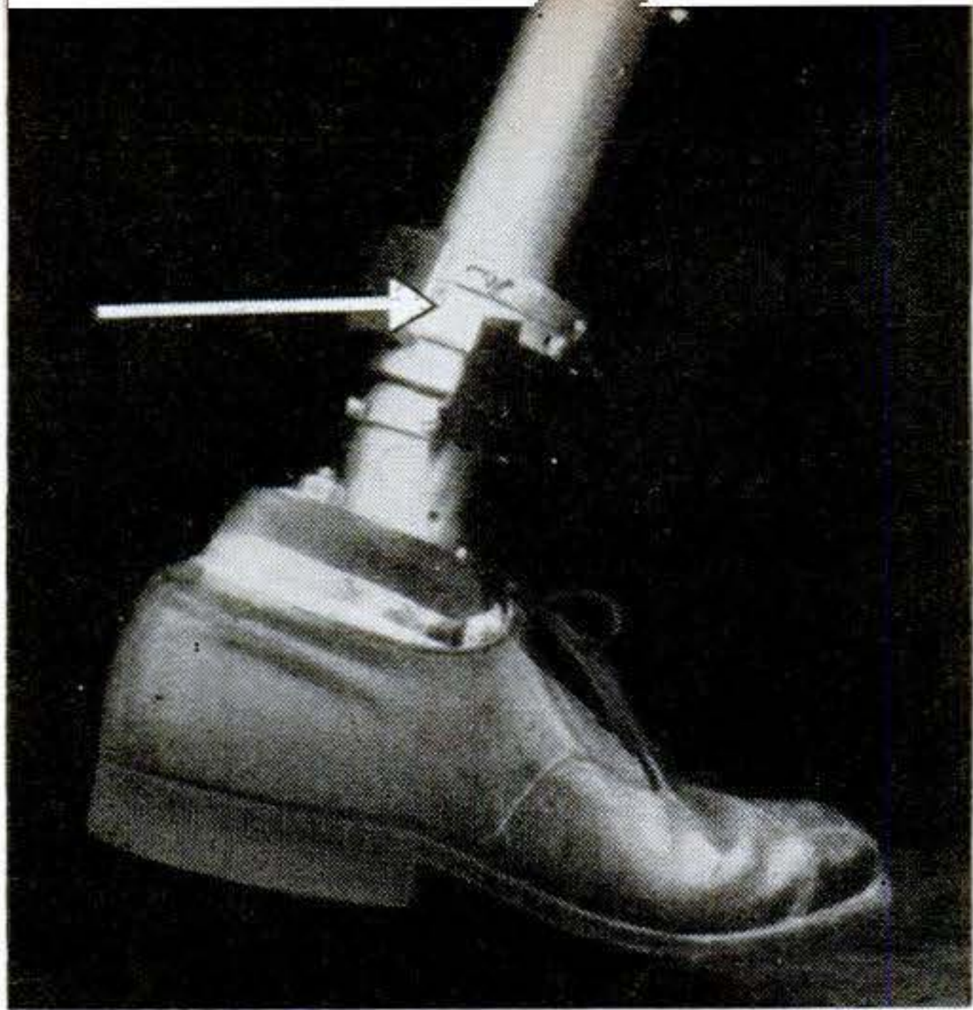
straight ahead. Arrows in above pictures show variation in opening between bumper and stop from time heel touches ground and toe completes step. Guards prevent foot from turning too far.
