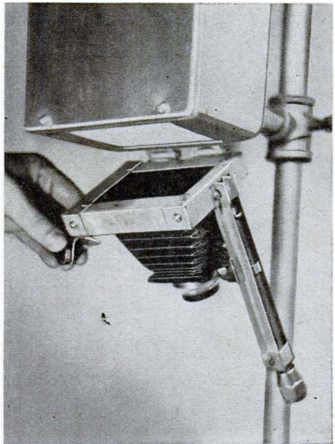
HINGED BELLOWS ASSEMBLY. Negatives are put in place by swinging the frame down, the assembly normally being held up by two spring hinges.
