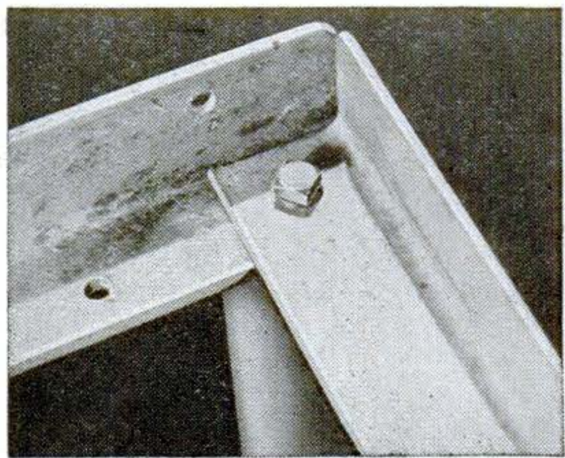
Angles form a frame for the bench top. A filler strip is needed over angle A, the thickness of the iron in E.
