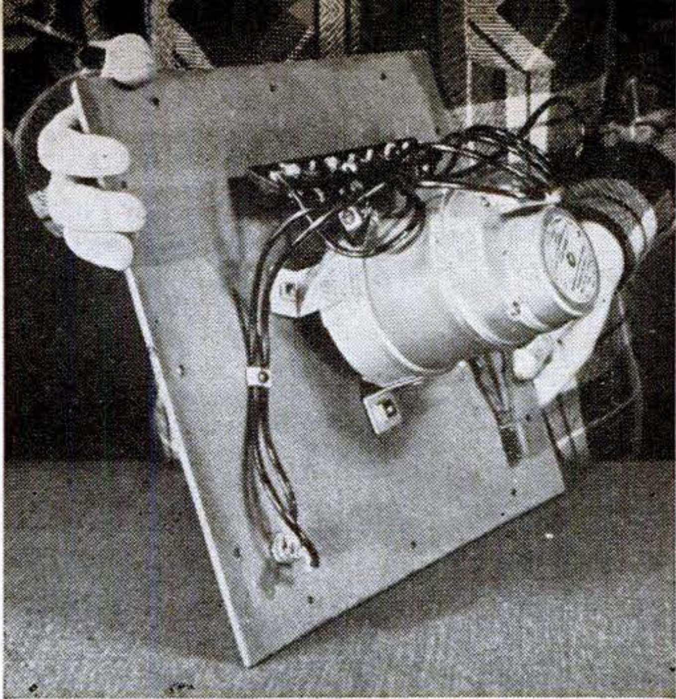
Mount each selsyn on the back of its dial panel by means of metal clips bolted to its collar. Run the shaft through to take the letter pointer.
