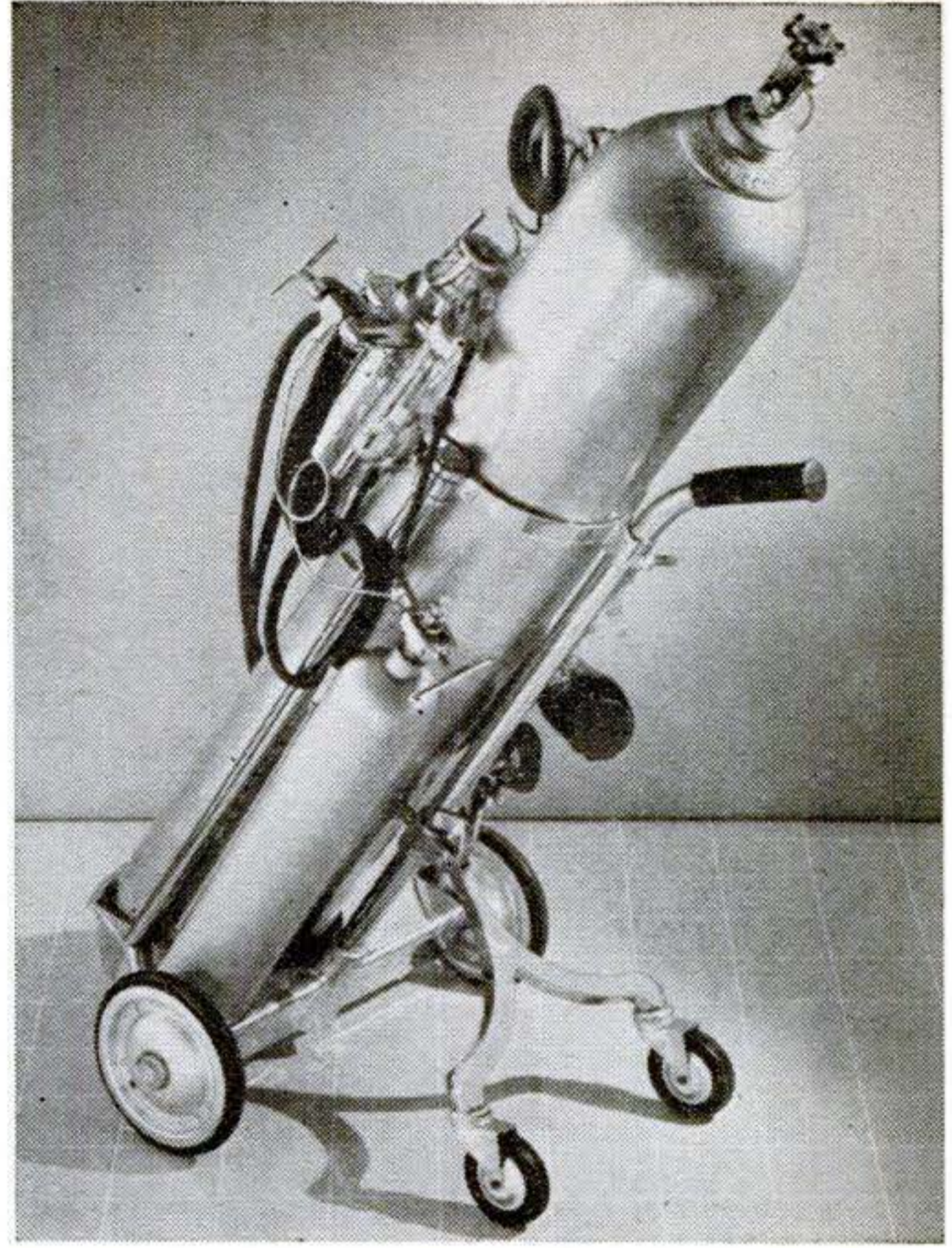
Folding fork wheelbase of this portable hospital model enables a nurse to handle easily a 130-pound oxygen cylinder by herself. Complete E & J unit is attached to side of the cylinder.
