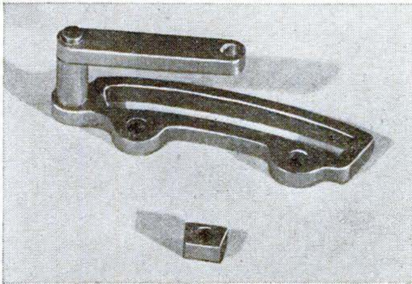
A short pivot stud connects the drag link to the reverse link. Also above is the link block, shaped to match the slot, which fits the valve-rod fork.
