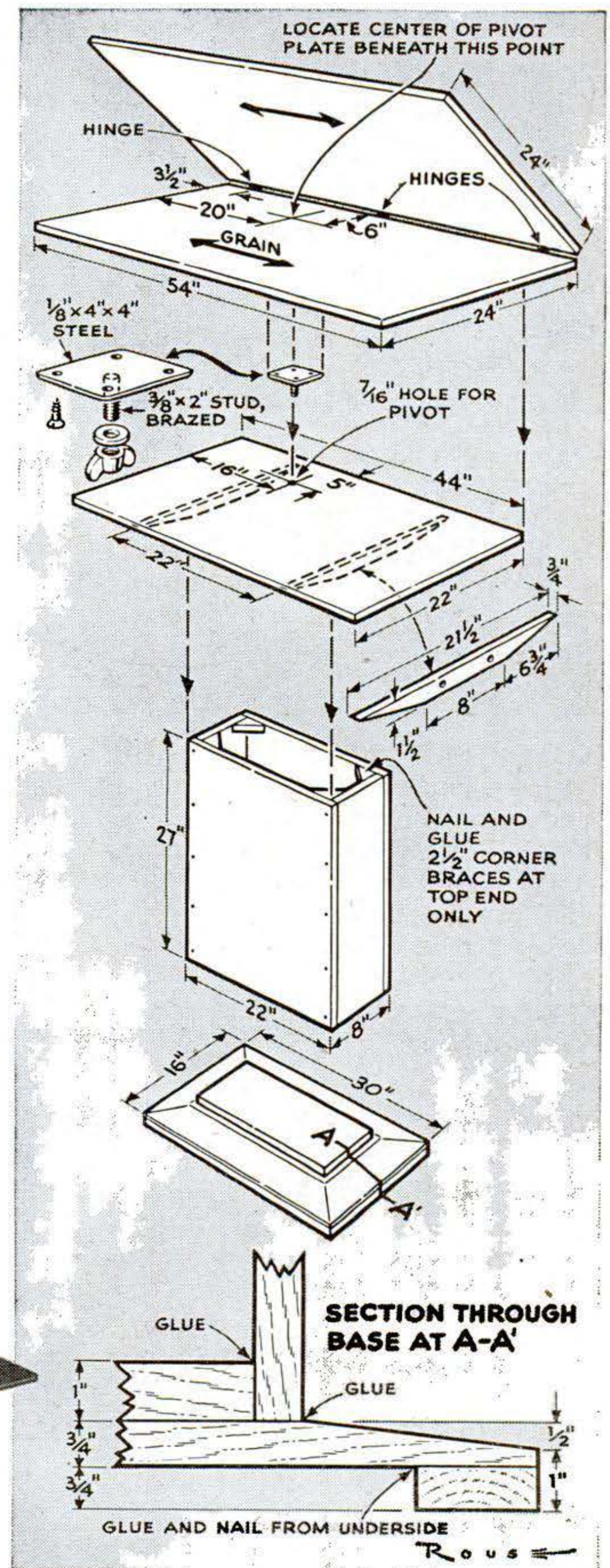
Construction is in four pieces, with the lower three—base, column, and column top—glued and screwed together as a rigid unit. The folding leaves forming the table top are held in place loosely with a pivot bolt and wing nut.
