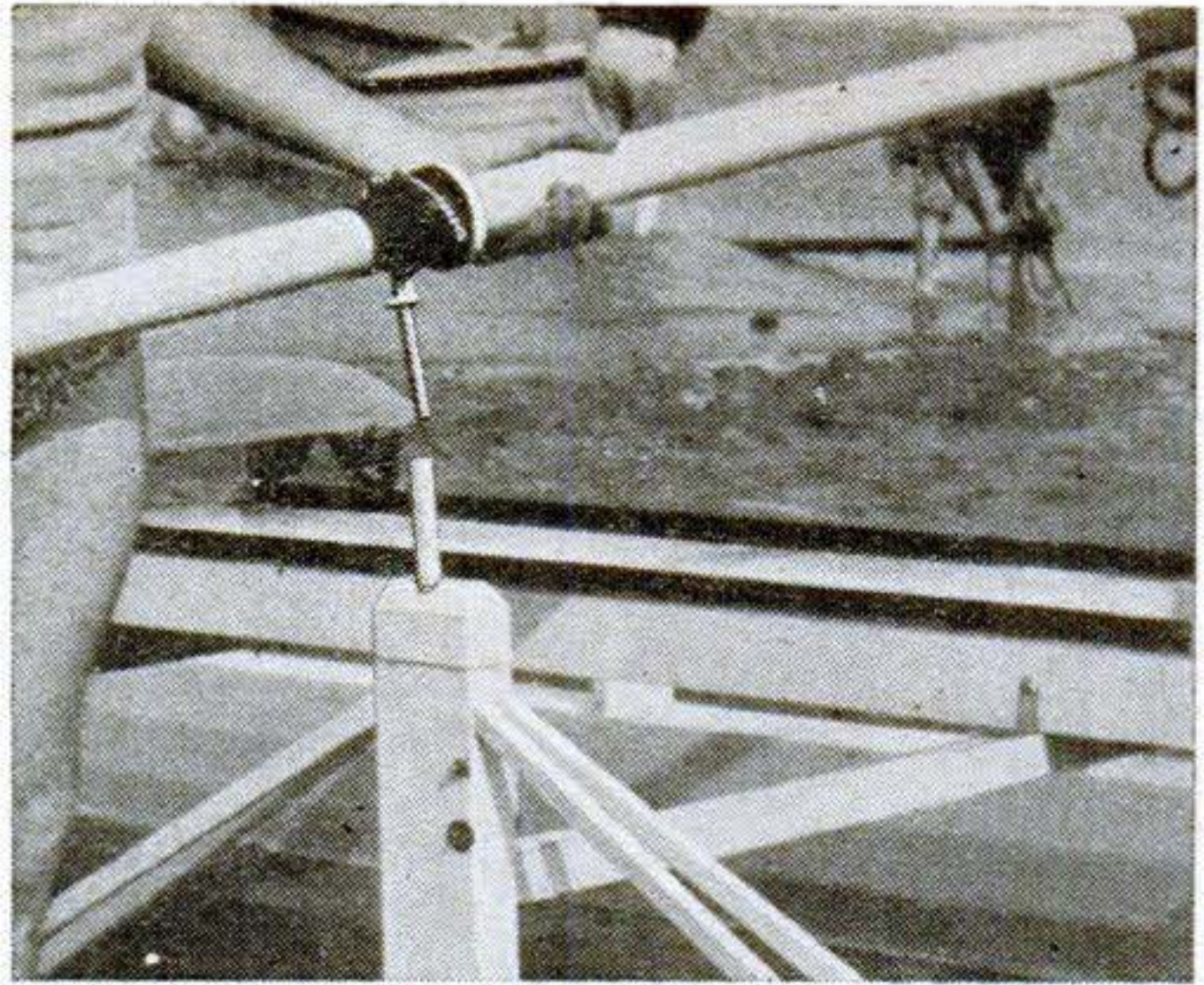
Oarlocks are made from steel rod and are seated in \frac{1}{2} " I.D. steel tubing wedged in the oarlock posts.
