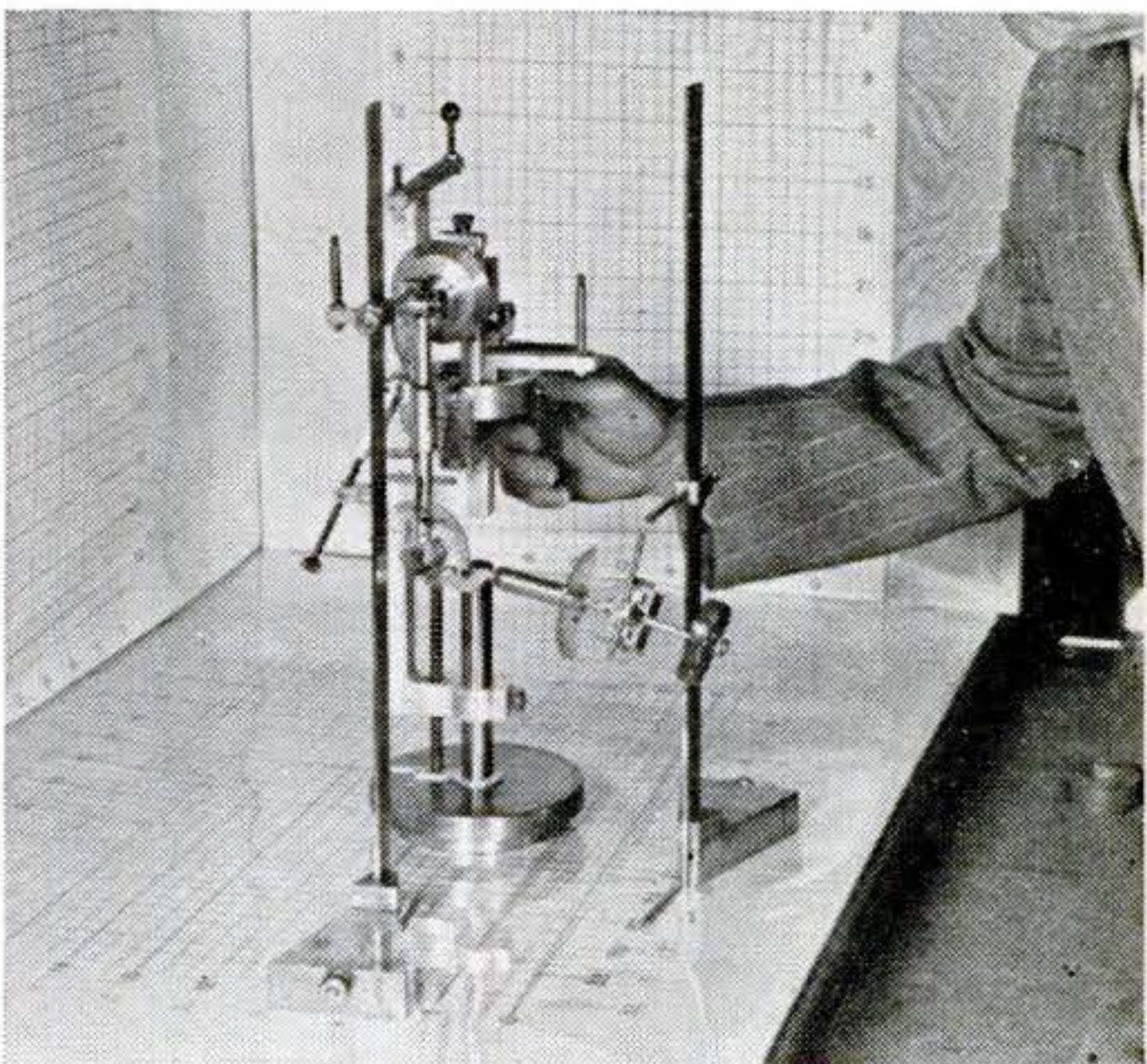
Using kinematic analyzer , researcher transfers information obtained from pictures to grids. The result is a picture of typical hand patterns.
