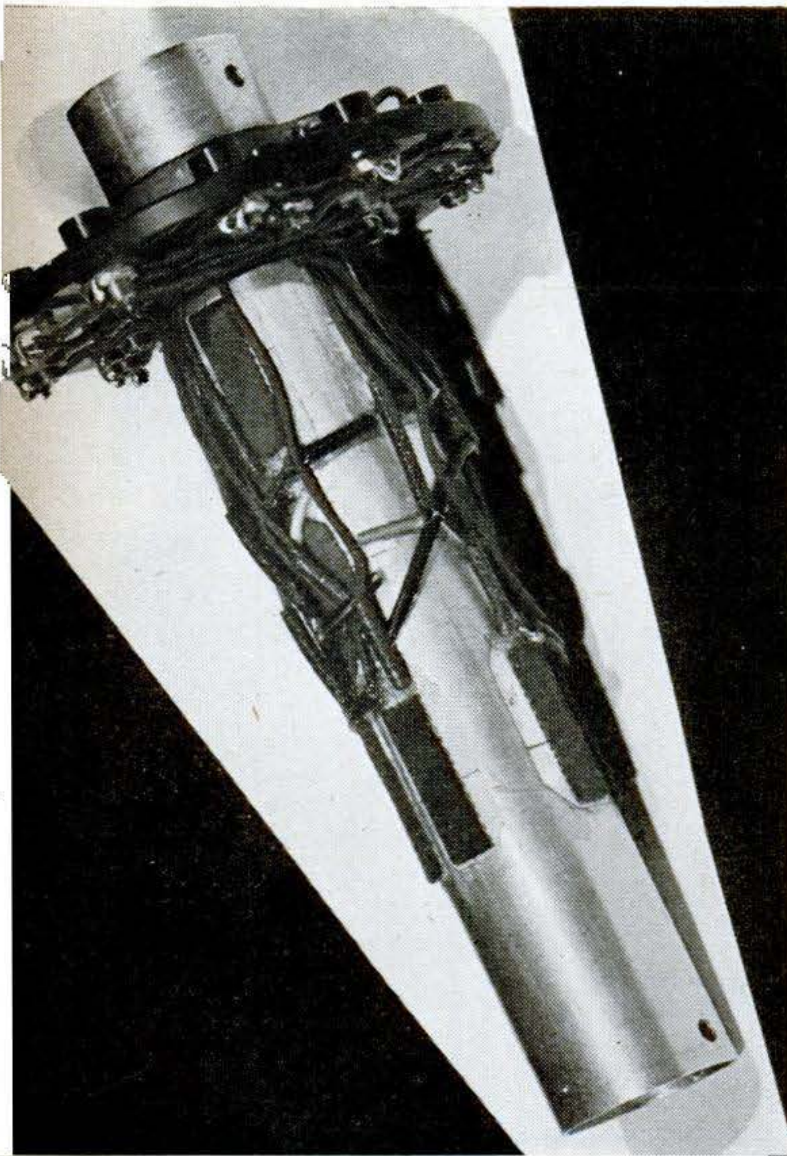
Aluminum "pylon" that measures forces acting on an amputee's leg. When pylon is substituted in shank of artificial limb, electrical gauges measure the torque, axial and vertical loads.
