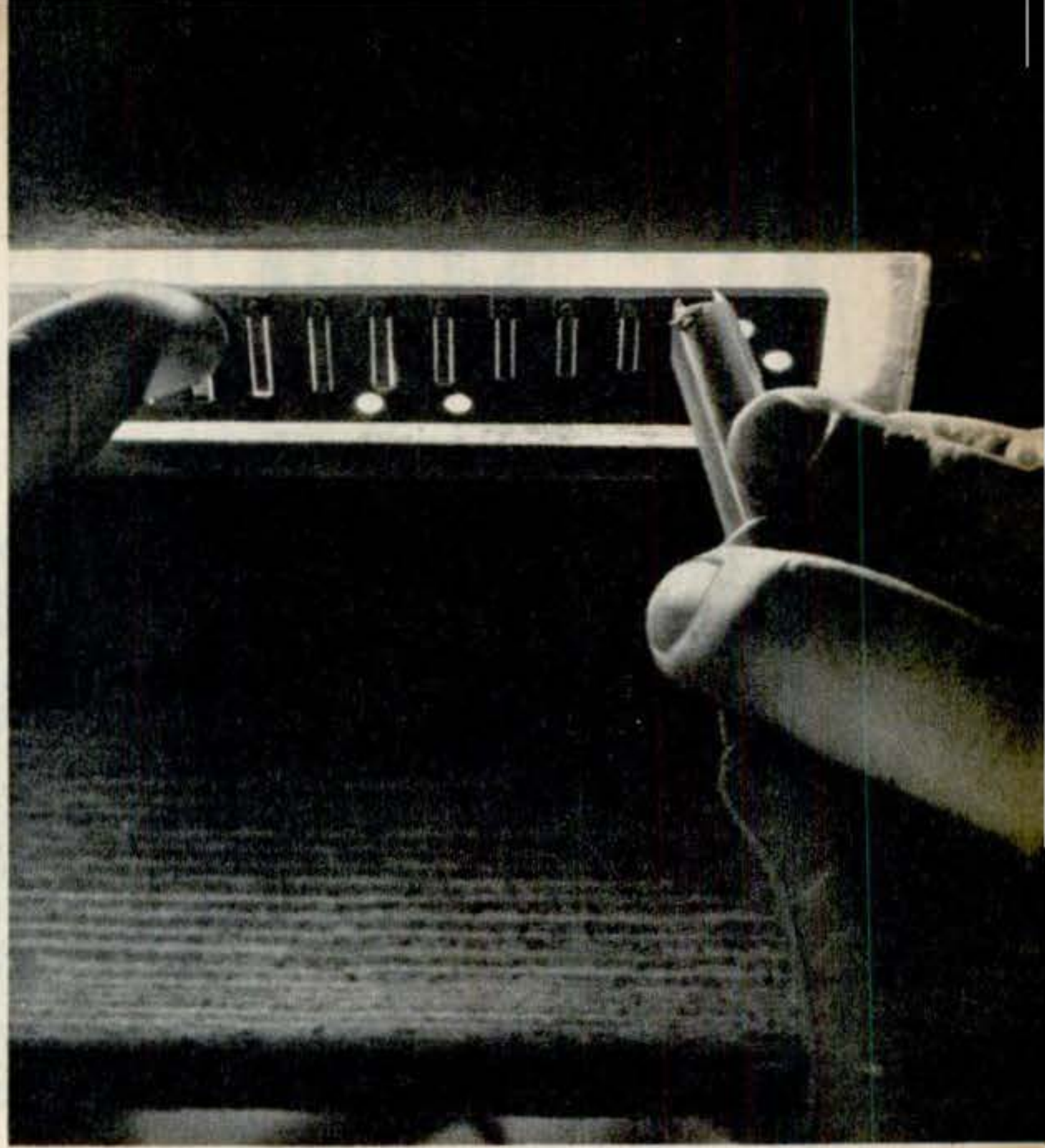
3. A beam of light, shining through the reeds, is used to check their alignment after riveting. Tolerances must be held to a fraction the thickness of human hair.
