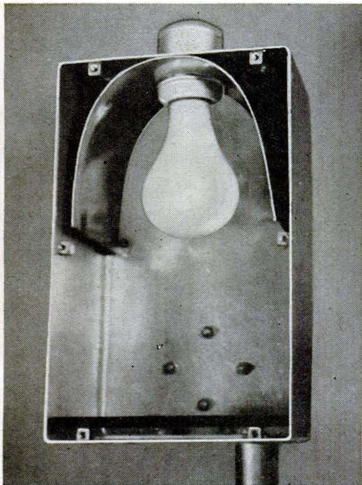
REFLECTOR IS ALSO BAFFLE. Heat escapes past the ends of the reflector to holes in the top. Heat-absorbing glass protects the negatives.
