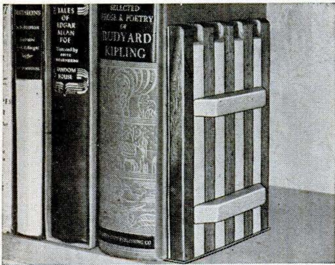
Sheet metal fastened with countersunk screws and covered with felt acts as a base for this book end.
