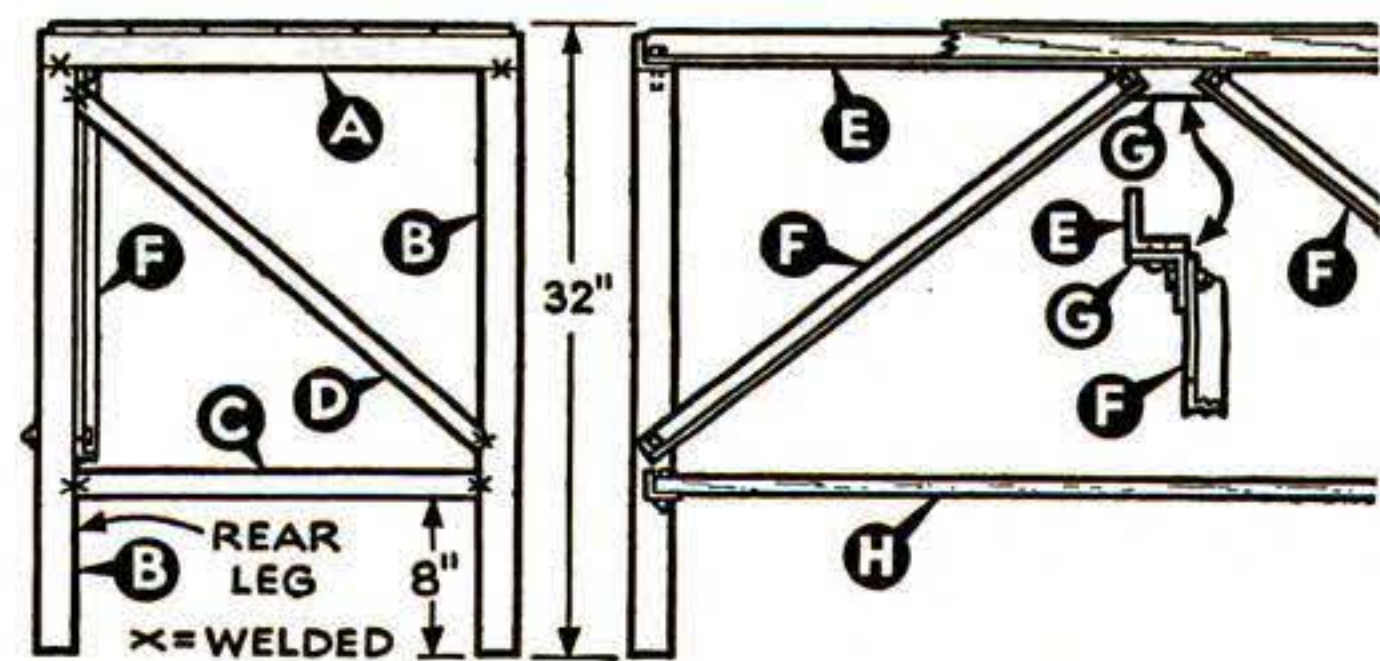
All parts lettered here are pieces of scrap metal with the exception of H, which is a board shelf.
