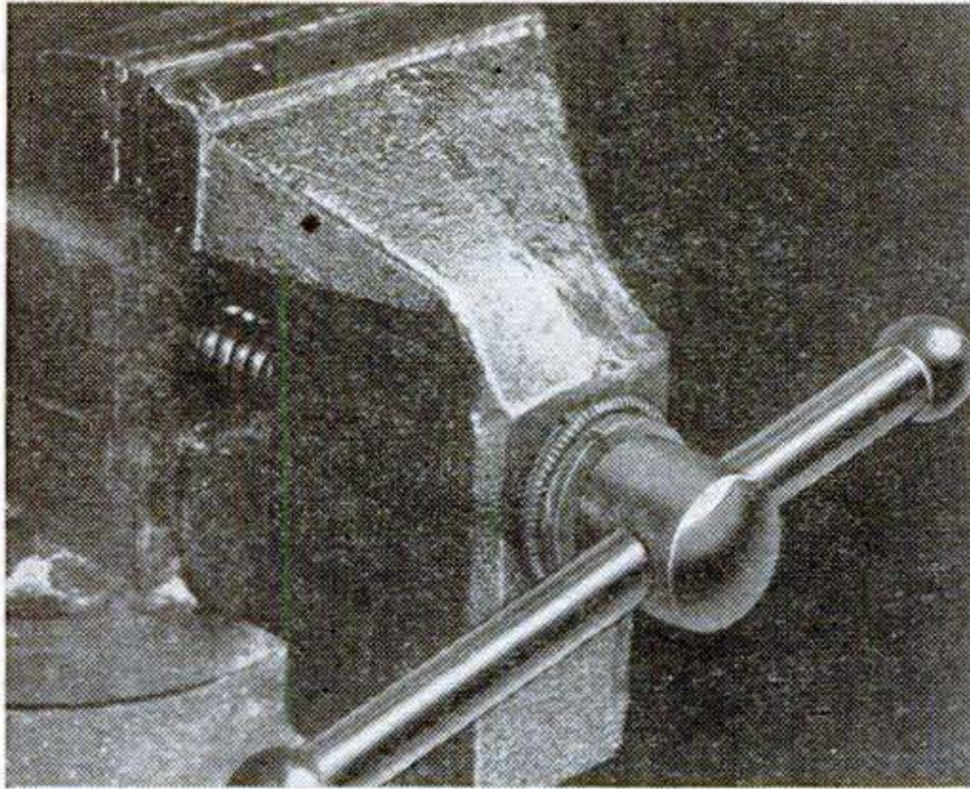
A thrust bearing gives a far stronger grip to this vise. The coil spring retains a leather dust guard.
