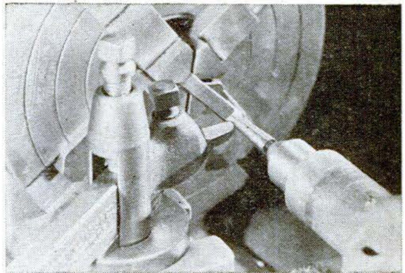
Chucked in the four-jaw, a piece of 1/4" square steel is turned down to form the handle of the reverse lever. Holes must be located as in the drawing.
