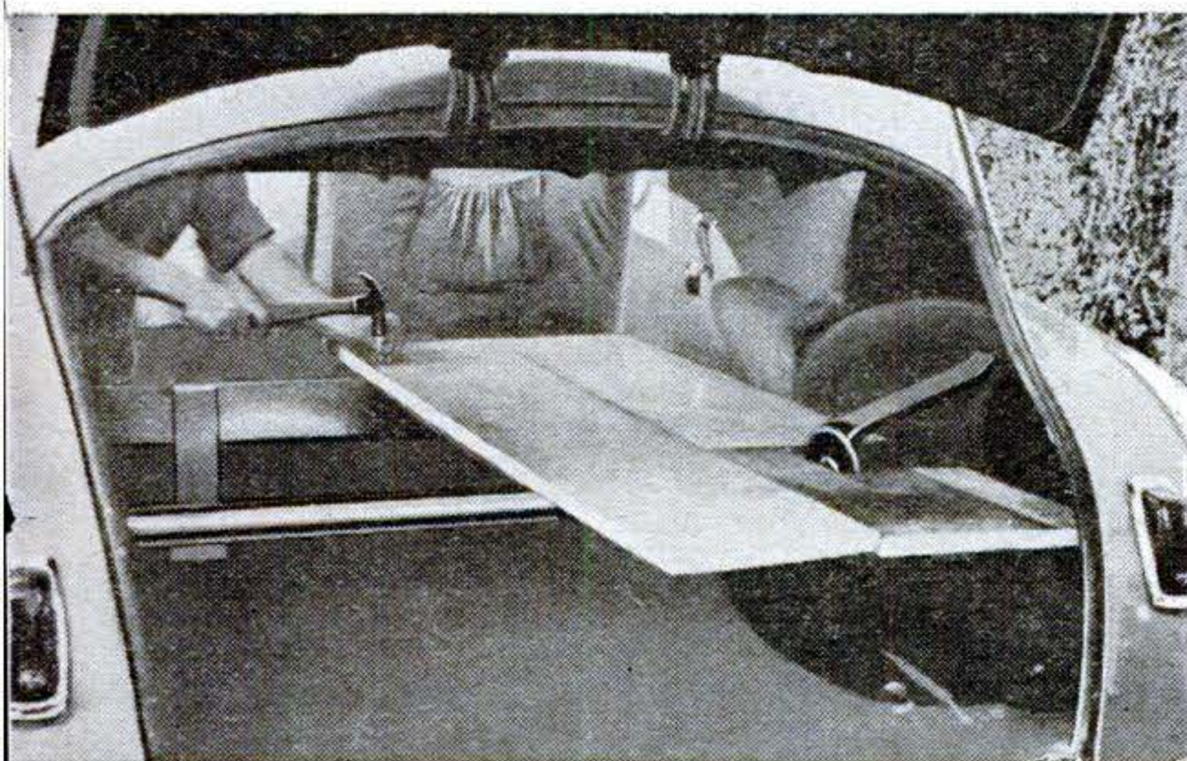
Finally planks are nailed to the front support as a platform for the mattress. When the vacation is over, the bed is taken out and the seat put back.
