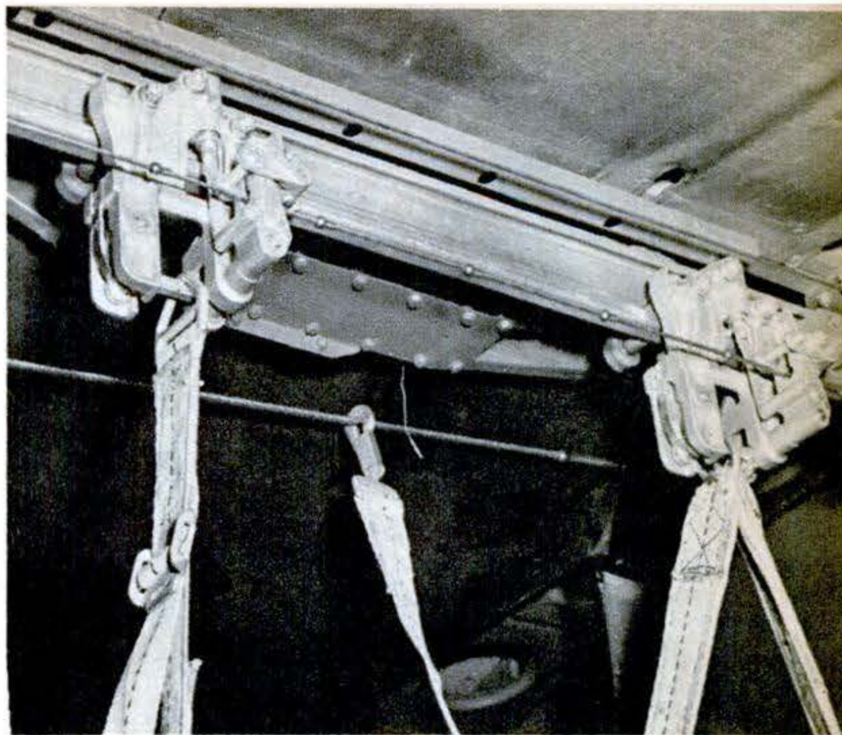
The paracans are hung on trolleys pulled along the aluminum monorail by an electrically driven cable. Wire in background is the static line that trips the parachute of each pack as it leaves the plane.
