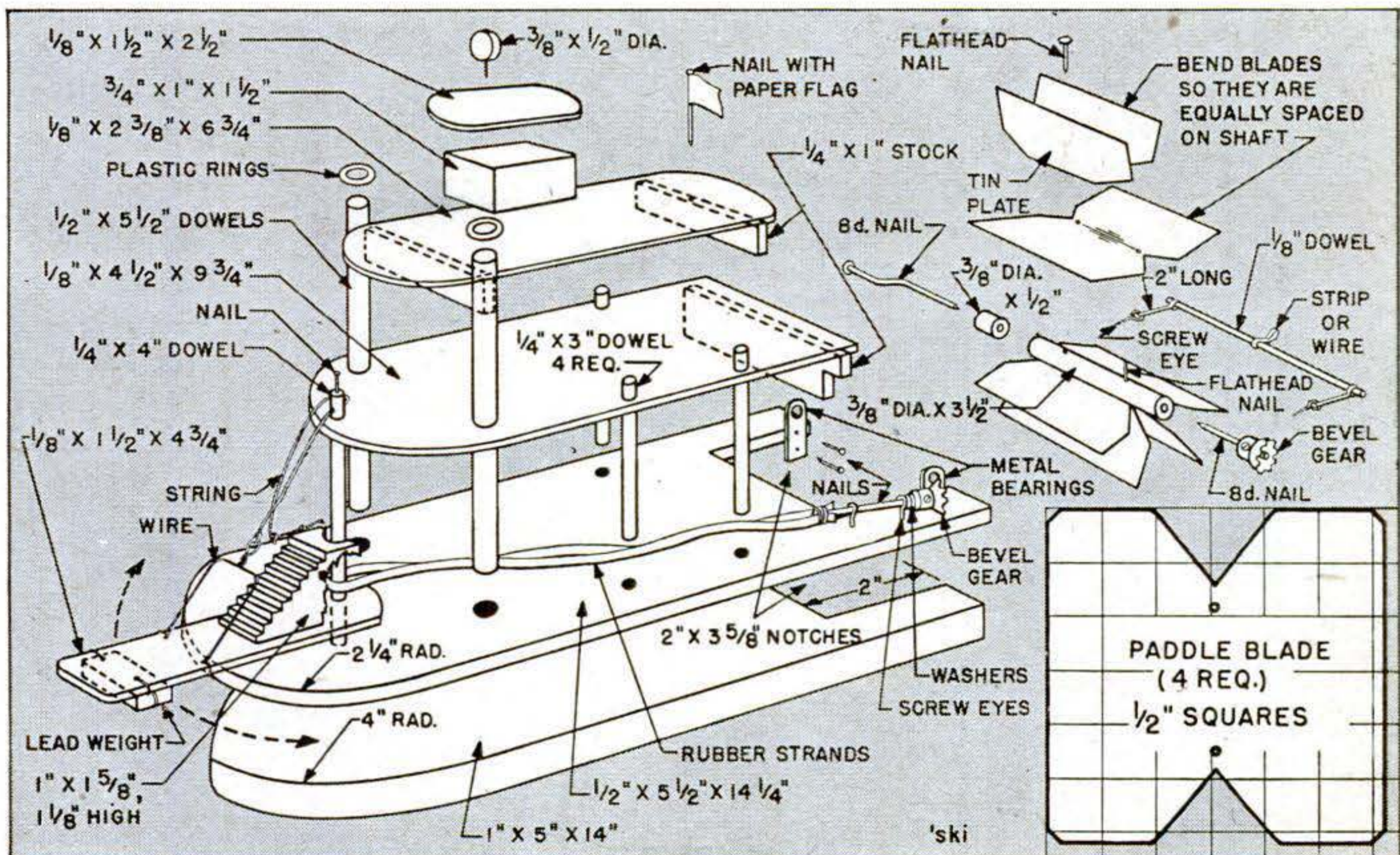
Here are the construction details. Parts are assembled with waterproof plastic glue and nails. None of the dimensions is critical, so don't hesitate to change them to suit pieces available in your scrap bin.
