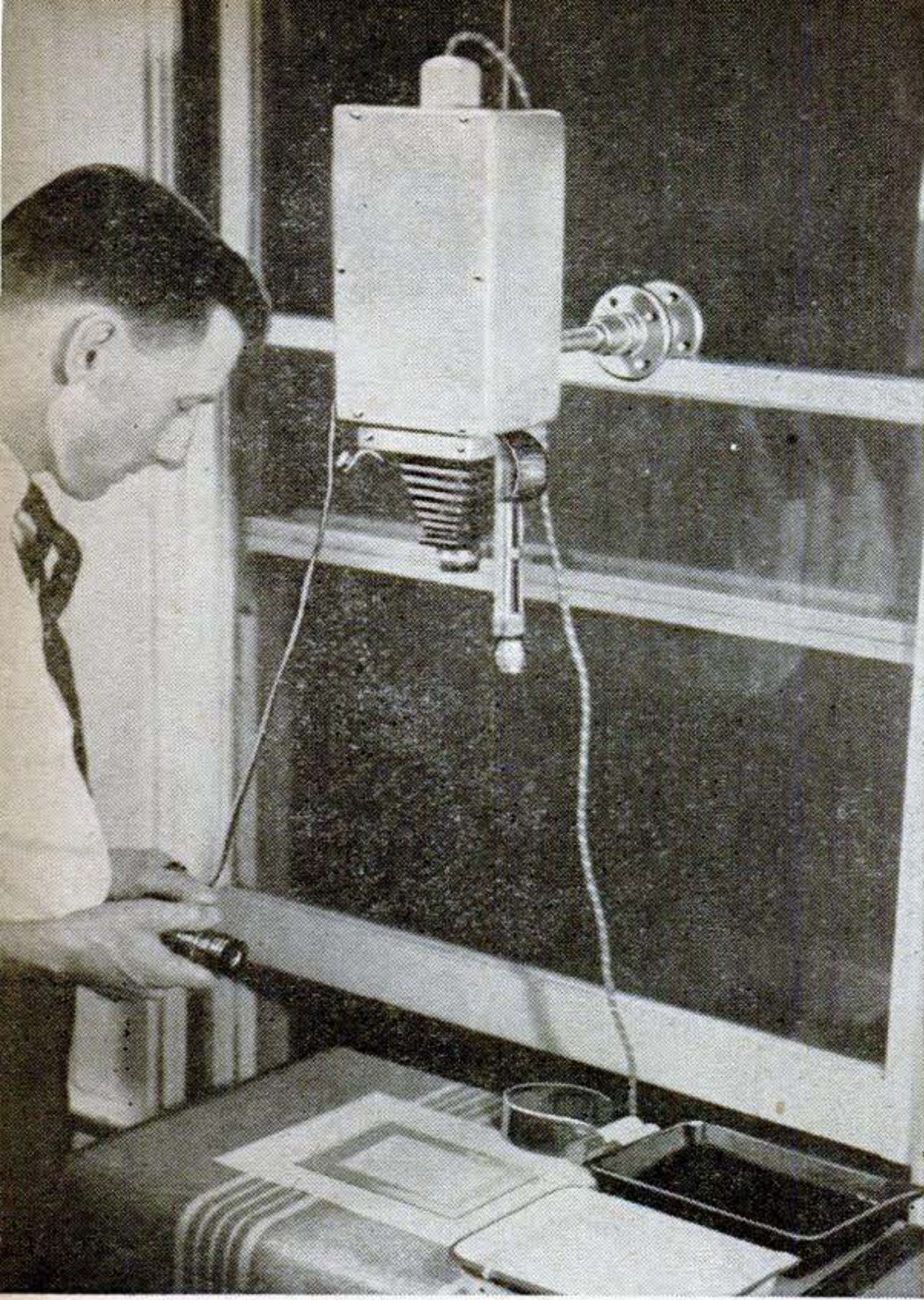
CLAMP THE ENLARGER ANYWHERE. Attached to a window sash, it is adjusted quickly for height.
