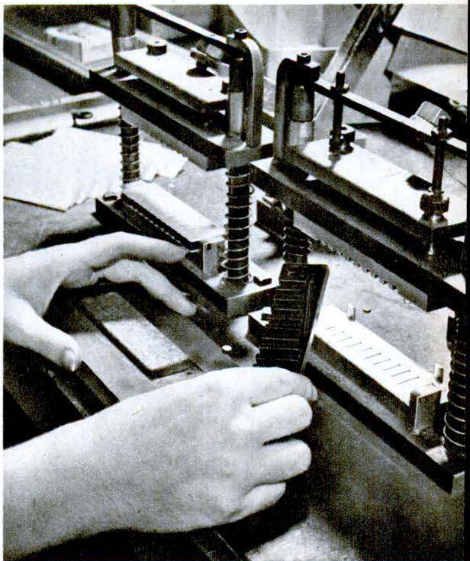
5. Reed plates are fastened to either side of the center section, comblike and usually formed of plastic. Metal or plastic covers are then attached to complete assembly.
