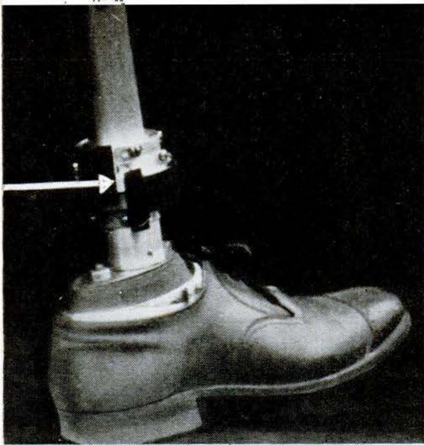
New artificial leg is the first that permits rotation of foot as in natural walking. Steel torsion rod within shin piece permits the foot to toe out and in as much as two inches from
