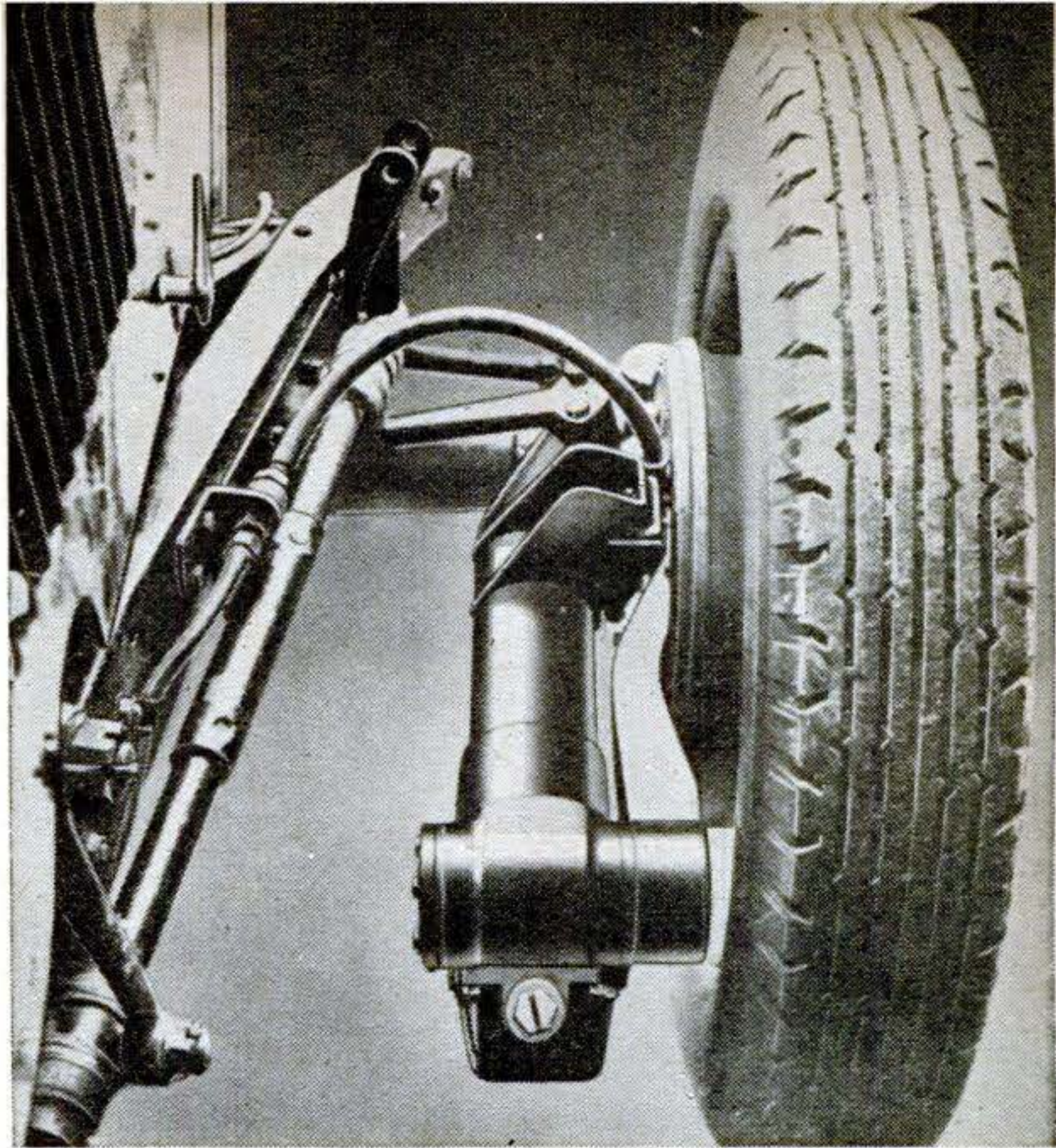
Installed on cars, a new liquid spring is said to improve riding comfort and roadability. A resilient gland ring sandwiched between two steel plates expands under pressure and keeps the oil from leaking out.
