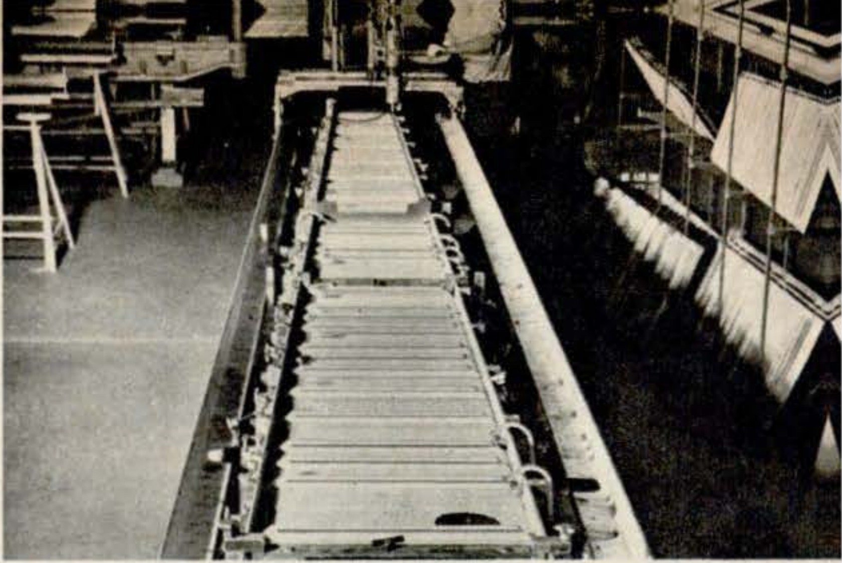
On long fixtures like the one above, the wing center section spar is assembled. The two side girders form a track for the drill shown in the background.
