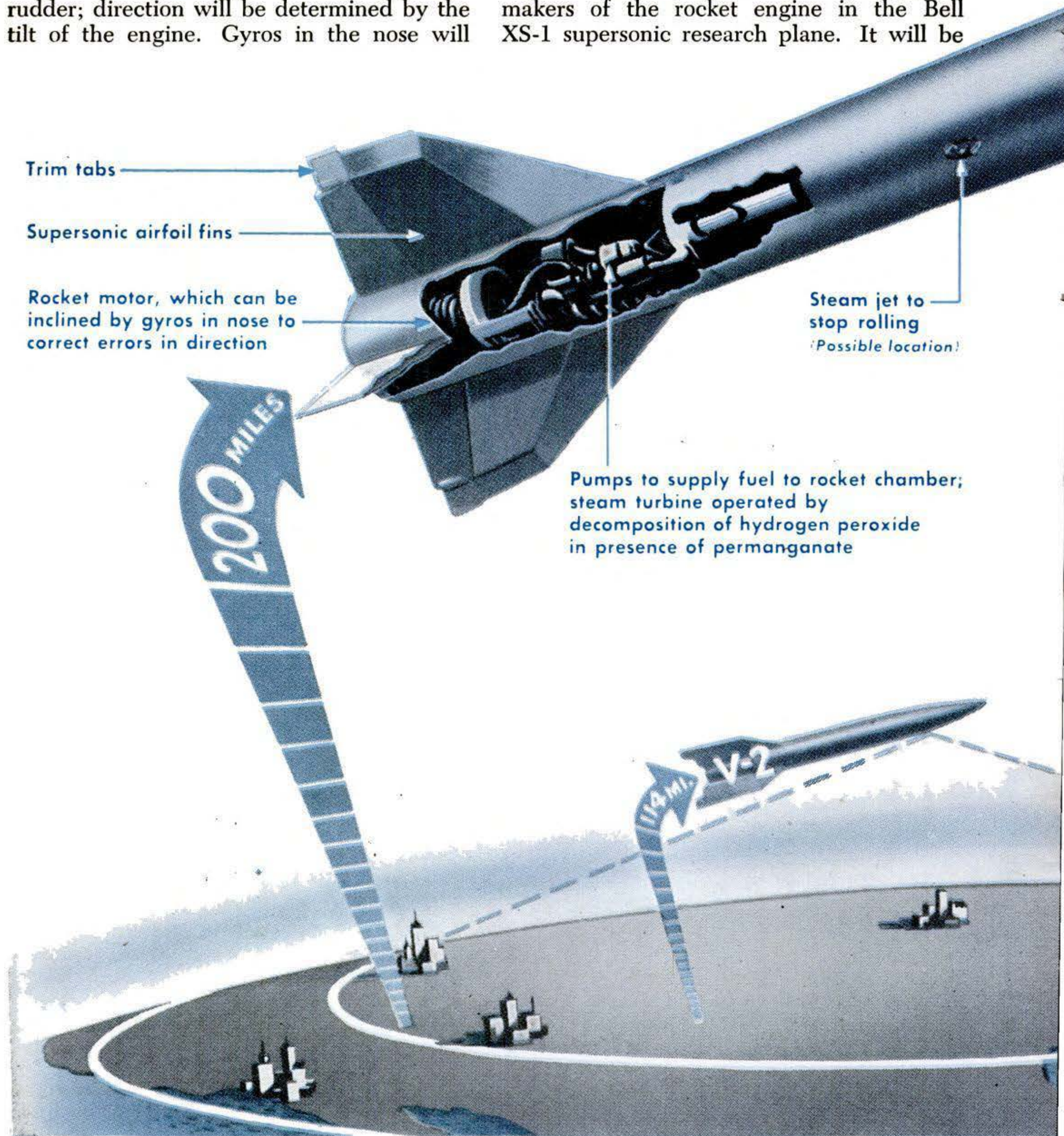
Drawings illustrate Neptune's construction and field of vision compared to V-2 (white circles).
