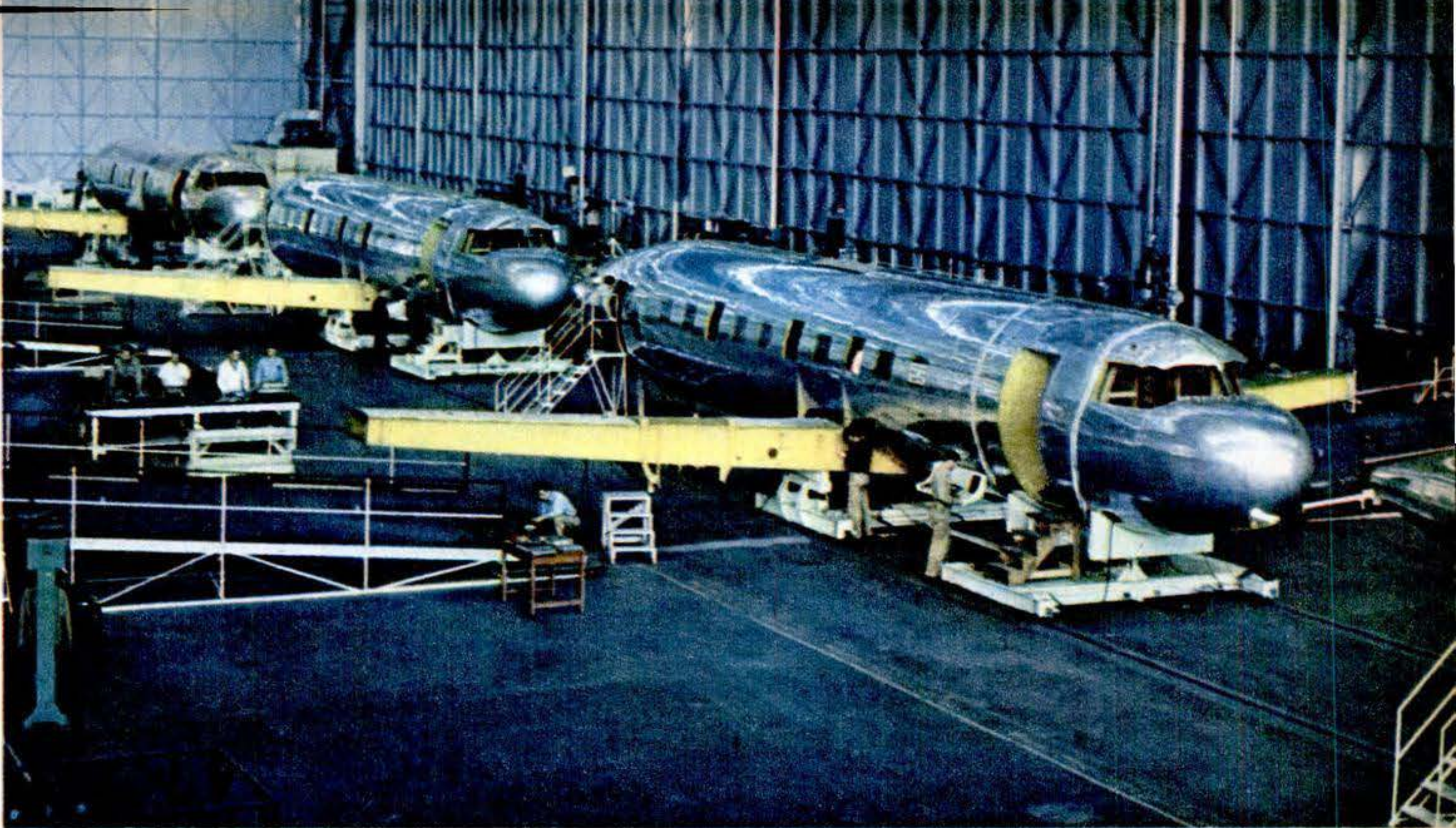
The 40-passenger Consolidated Vultee liners, in various stages of construction, roll along the assembly line.
