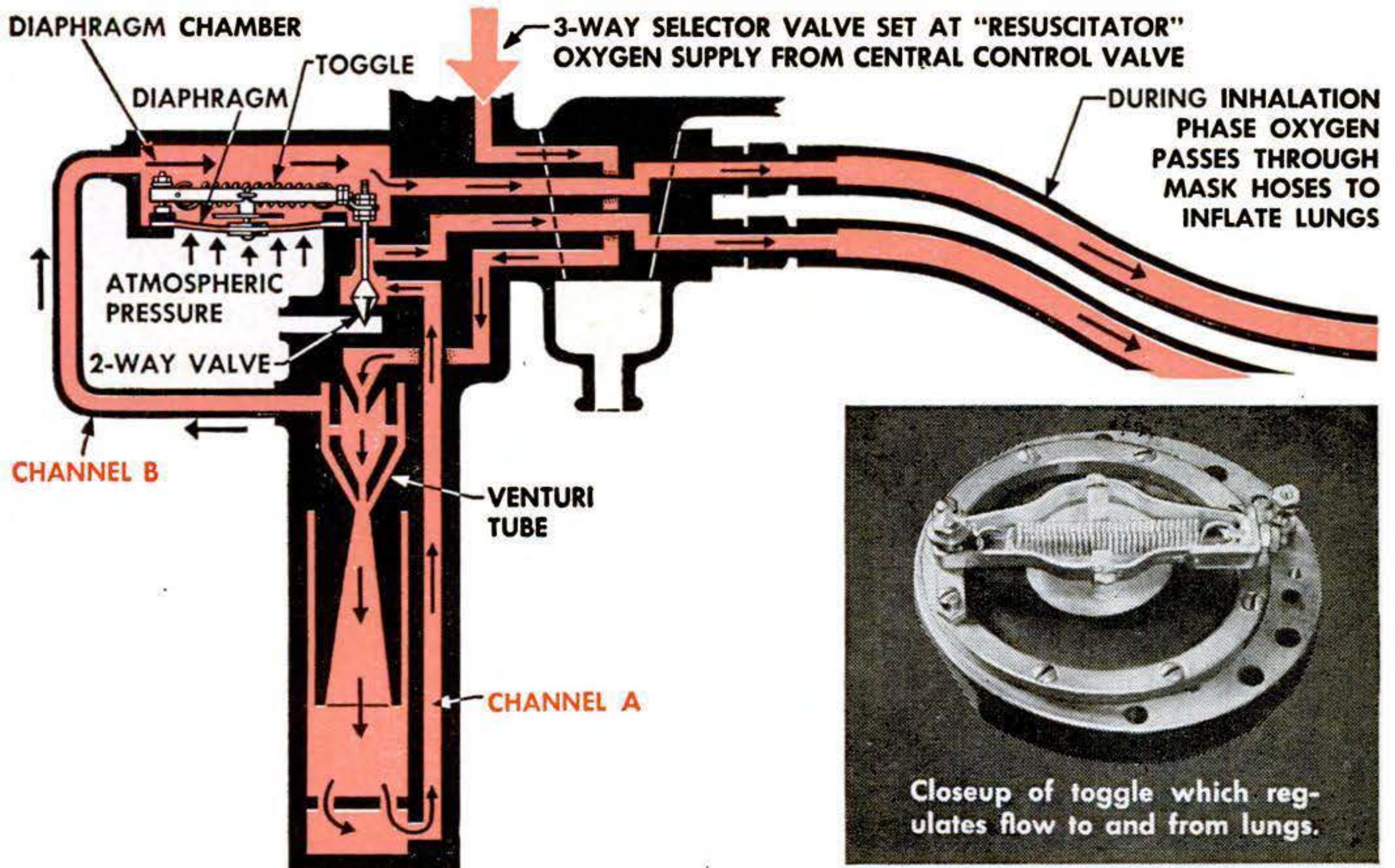
Cutaway of operating head showing first stage of resuscitation. In going past Venturi tube, half of gas follows channel A, half channel B. Later passes through diaphragm chamber. Oxygen
