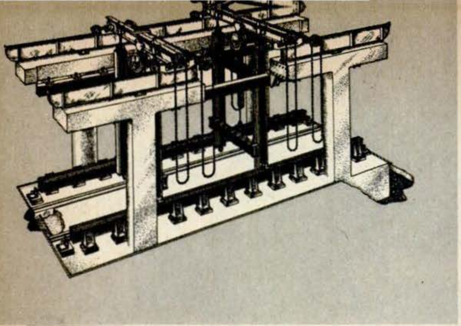
Accurate to 2/1,000 inch, this tooling dock provides precision checking and duplication of fixtures on which parts for the planes are formed.
