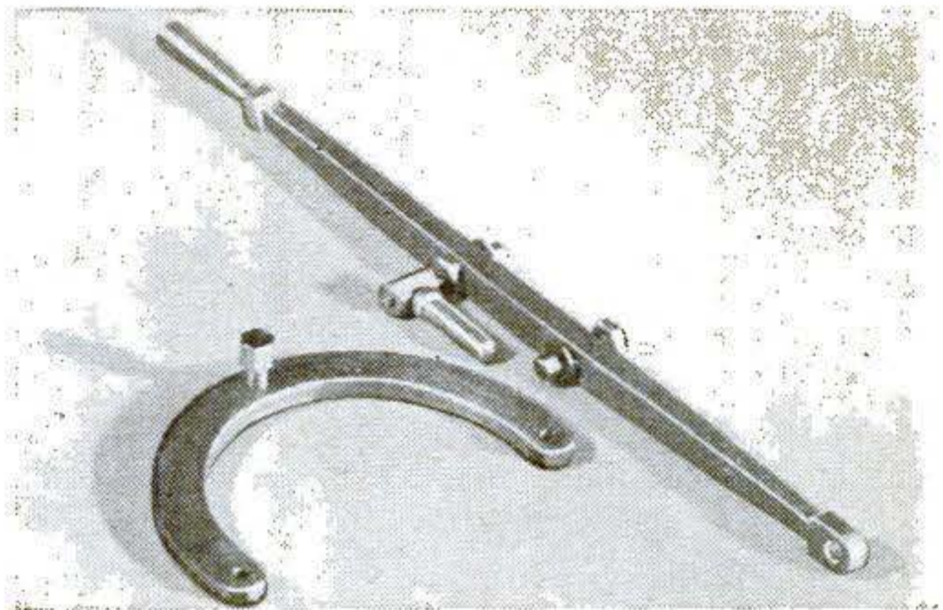
At its lower end, the lever pivots on a stud that screws into the ring, which will itself be bolted to the base. The clamp nut is fitted with a handle.
