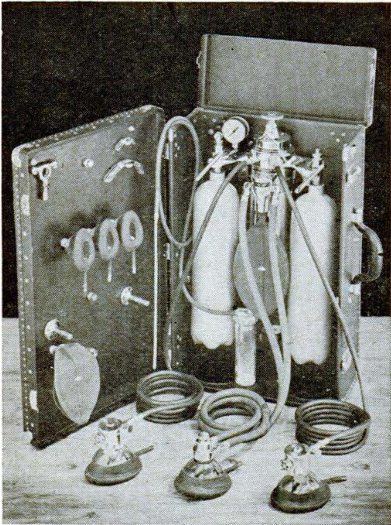
Complete in its carrying case, the E & J Resuscitator consists of two oxygen tanks, operating head (top center), main breathing mask (center foreground), and two auxiliary micromasks. Panel at left holds infant masks and a test bladder.
