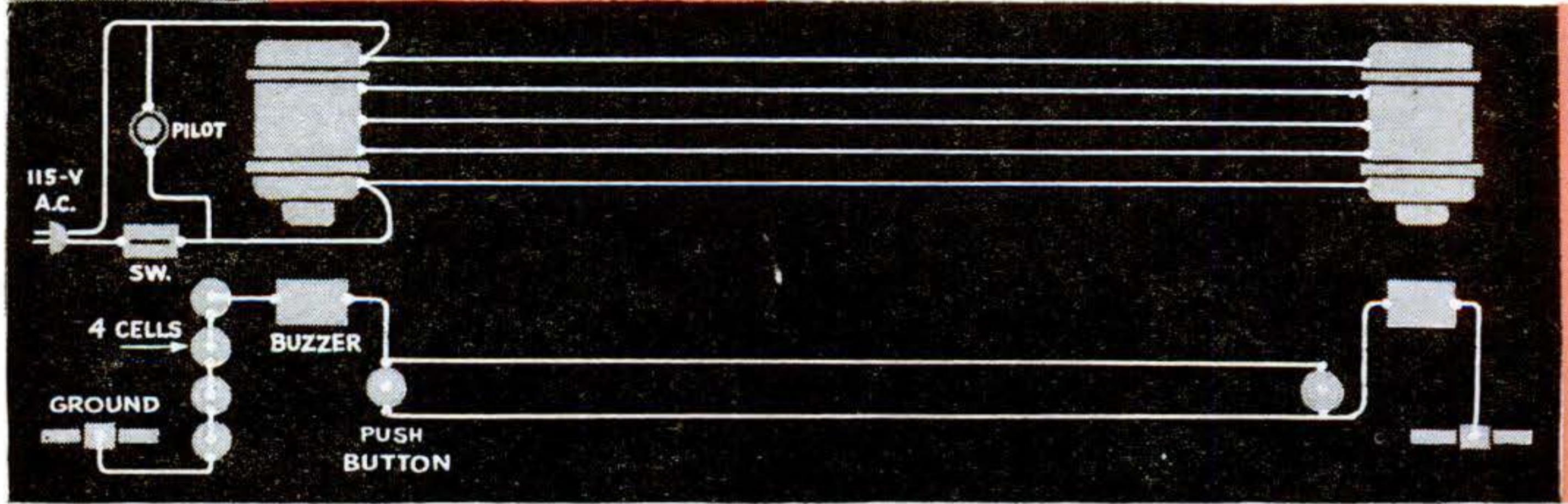
Five wires of a type suitable for carrying house current connect the selsyns. Join the leads to the proper numbered terminals. A separate buzzer circuit for a calling signal is wired with dry cells and a ground return.
