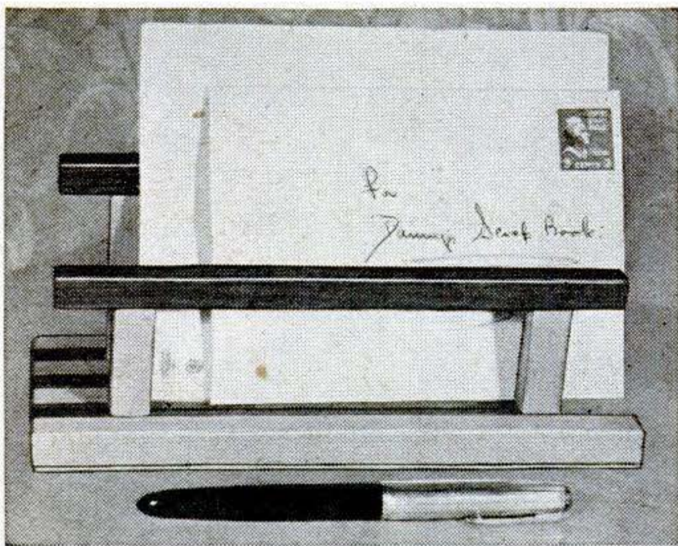
Screws through the underside hold the letter-rack posts. Make the rear rail higher than the front.
