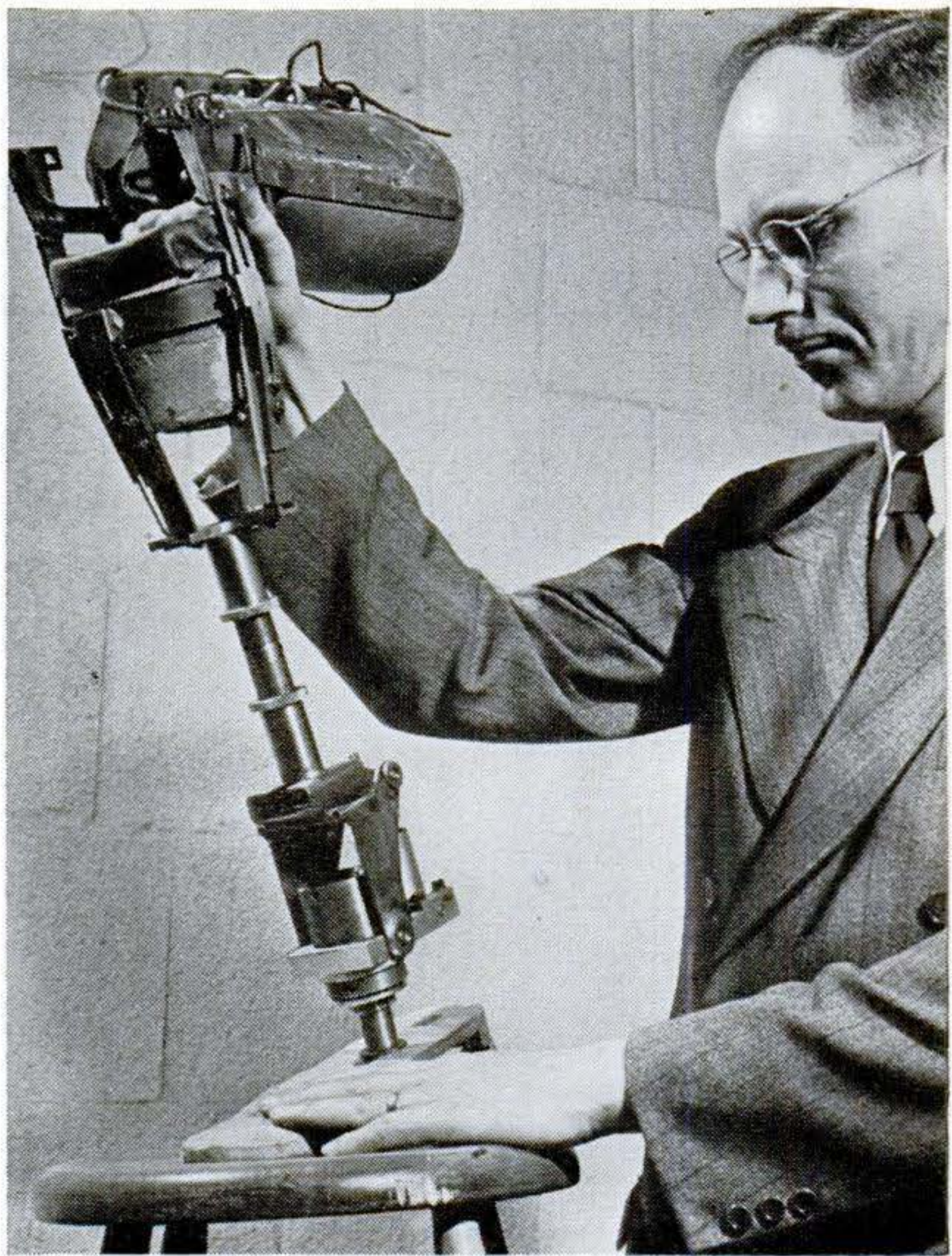
"We must mimic the action of the normal leg," maintains Professor Eberhart. He is shown here checking an adjustable artificial limb that is used to determine the needs of individuals.
