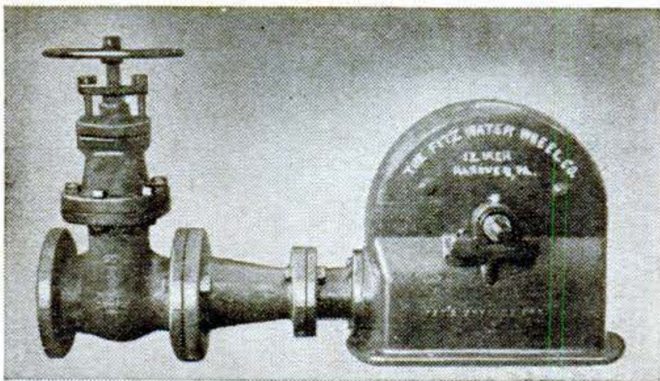
Dramatic contrast in wheel sizes. Top, a 25-ton job designed for installation in a 30,000-hp. unit. It turns at 171 r.p.m. and has a 1,008' head. Below, a 12" wheel with reducer and gate-valve throttle.
