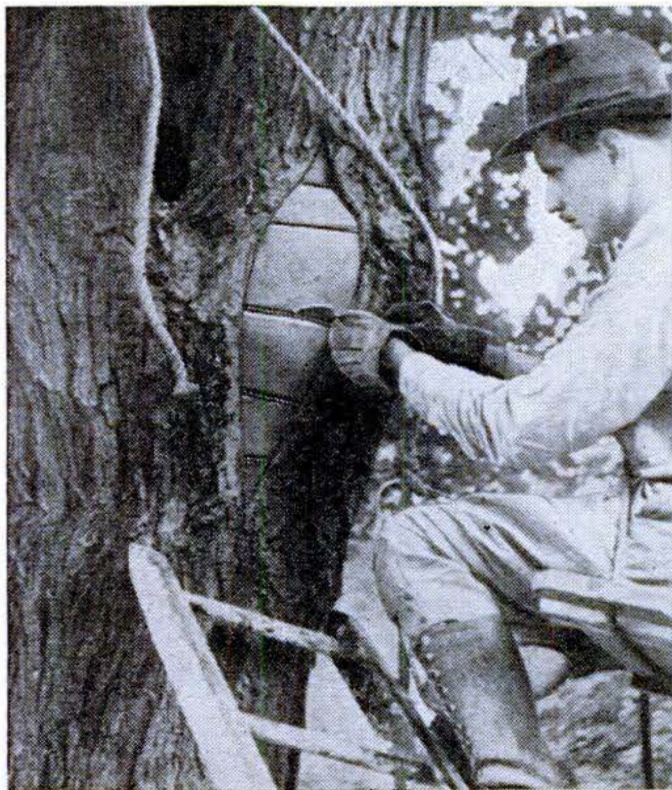
Concrete is put in a little at a time and spaced with roofing-paper sheets. The filling is slicked level with the wood, and the edges are beveled.
