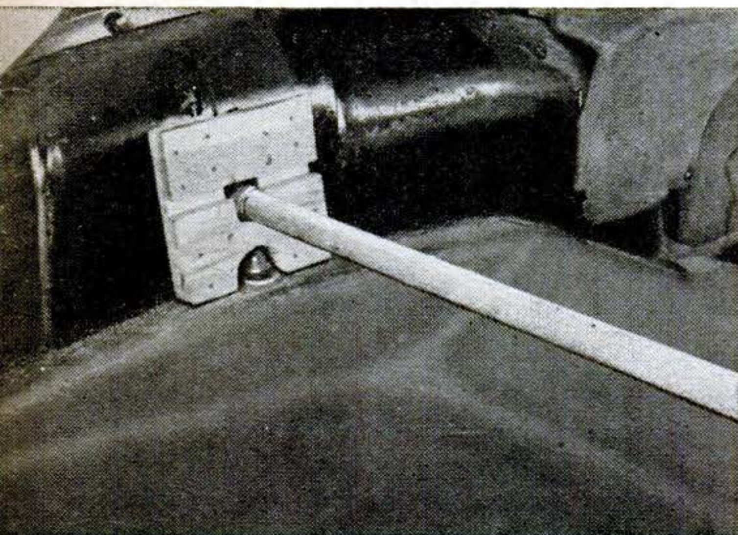
The other end of the pipe is held between blocks. If the spare-tire brace isn't on the side, put in blocks at both ends and use a wood crosspiece.
