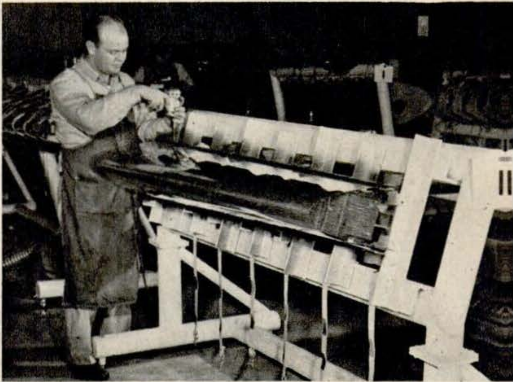
Wing edges are assembled on frames formed of heavy pipe and mounted at a 15^\circ angle. Tooling holes locate ribs and insure interchangeability.
