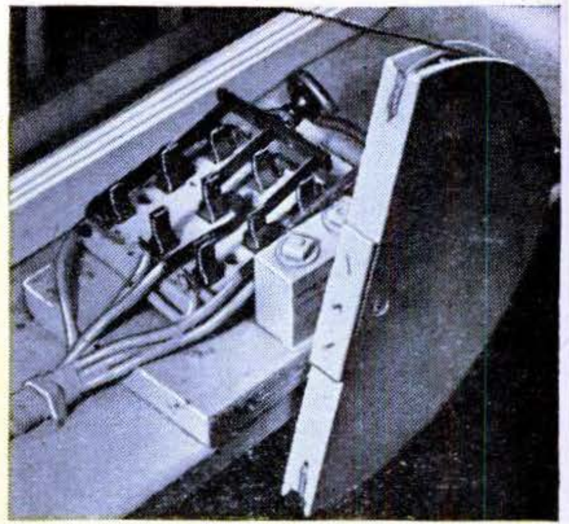
Two poles of the three-pole double-throw switch control motor direction, while the third serves as an on-off switch.
