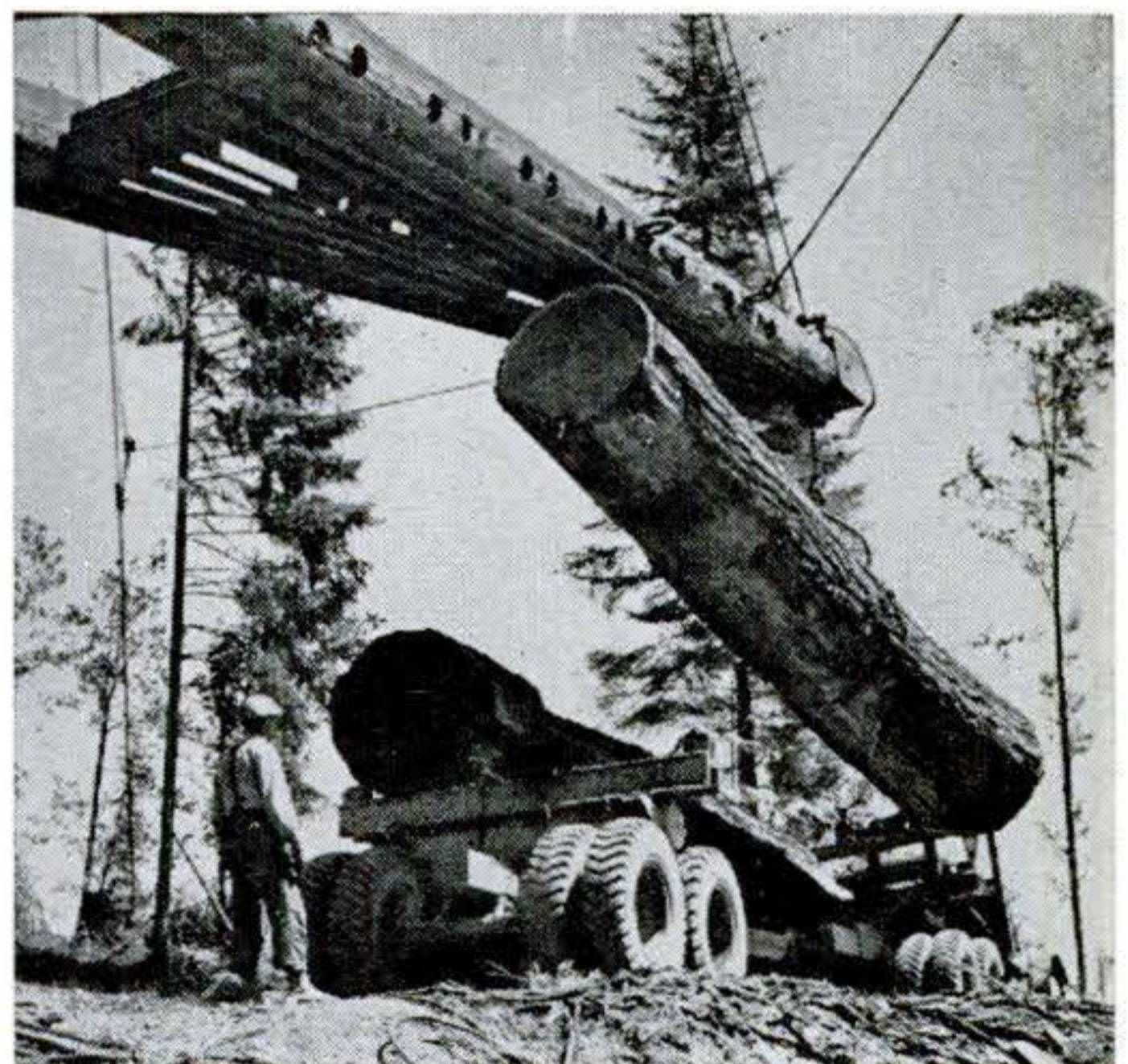
In the yard, the loader groups the logs and loads them on the trucks. A Diesel tractor, powers the yarder tree used as a derrick.
