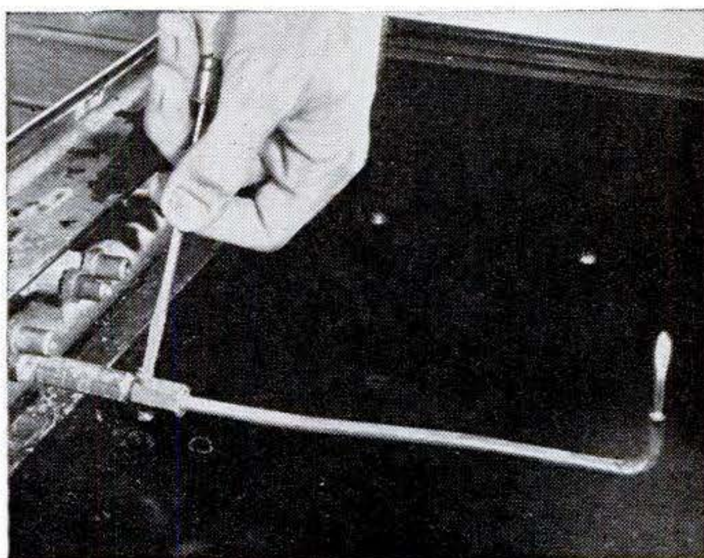
Most pilots have a yellow flame and no adjustment for air. Turn a valve or screw as shown or under the jet end for a small, steady flame. A clogged opening can be cleaned with a wire or needle.
