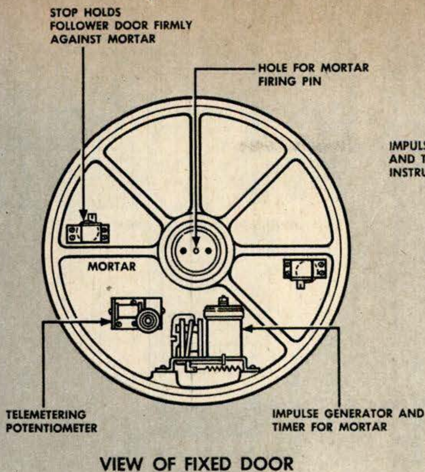
Fixed cover plate and the container's center bulkhead illustrate details of construction.
