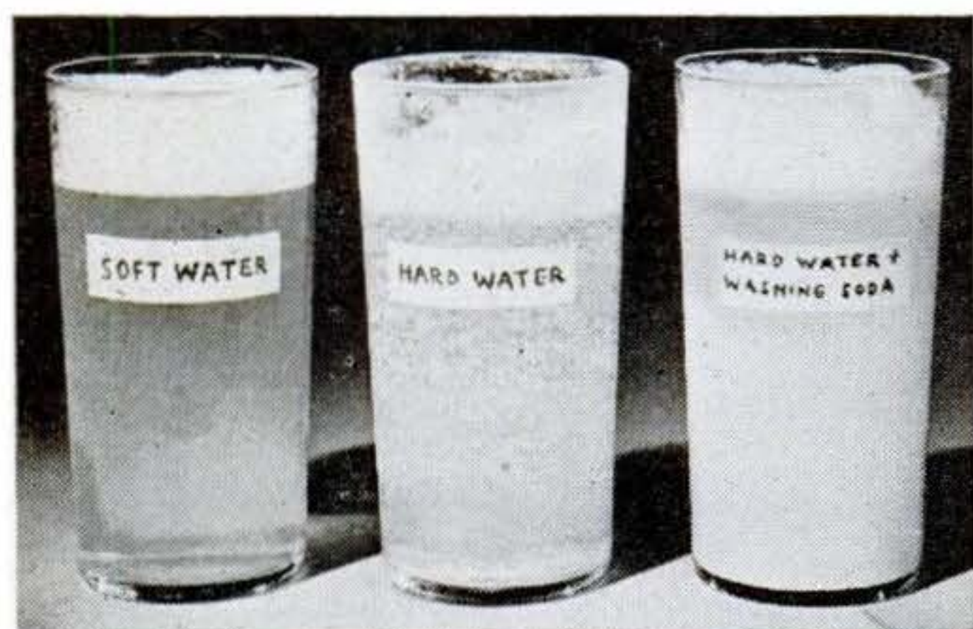
Until recent years, ordinary washing soda was the agent most frequently used for home softening of water. Soap added to water softened in this way produces suds about as freely as in soft water.
