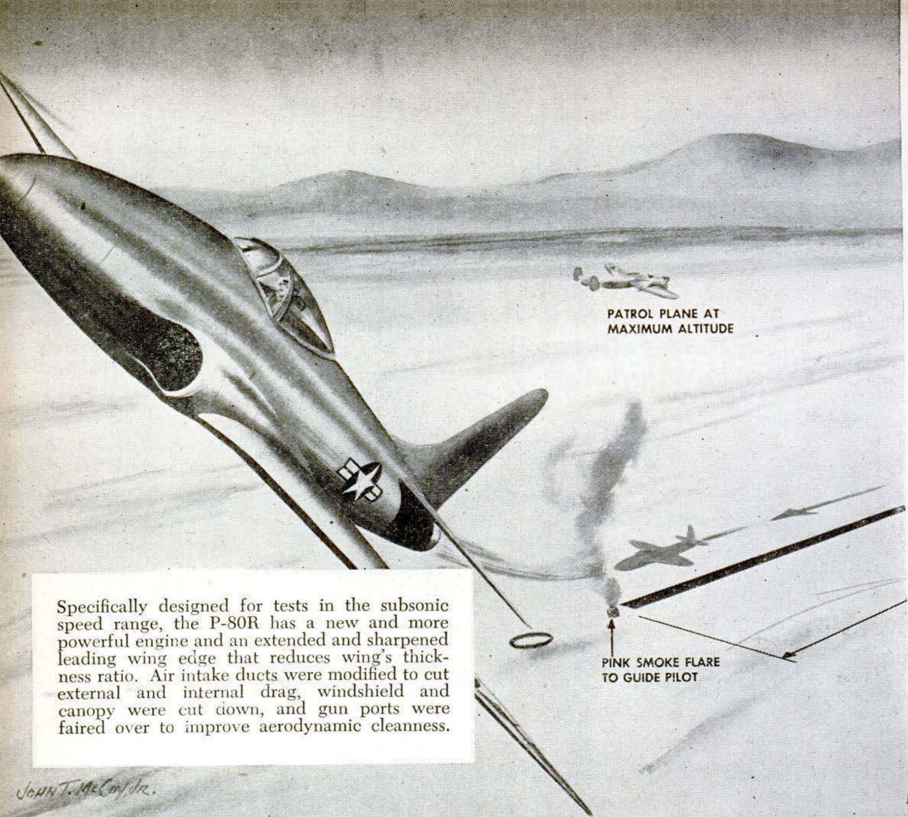
Artist's conception of conditions under which P-80R, nicknamed "Racey," set speed-mark.
