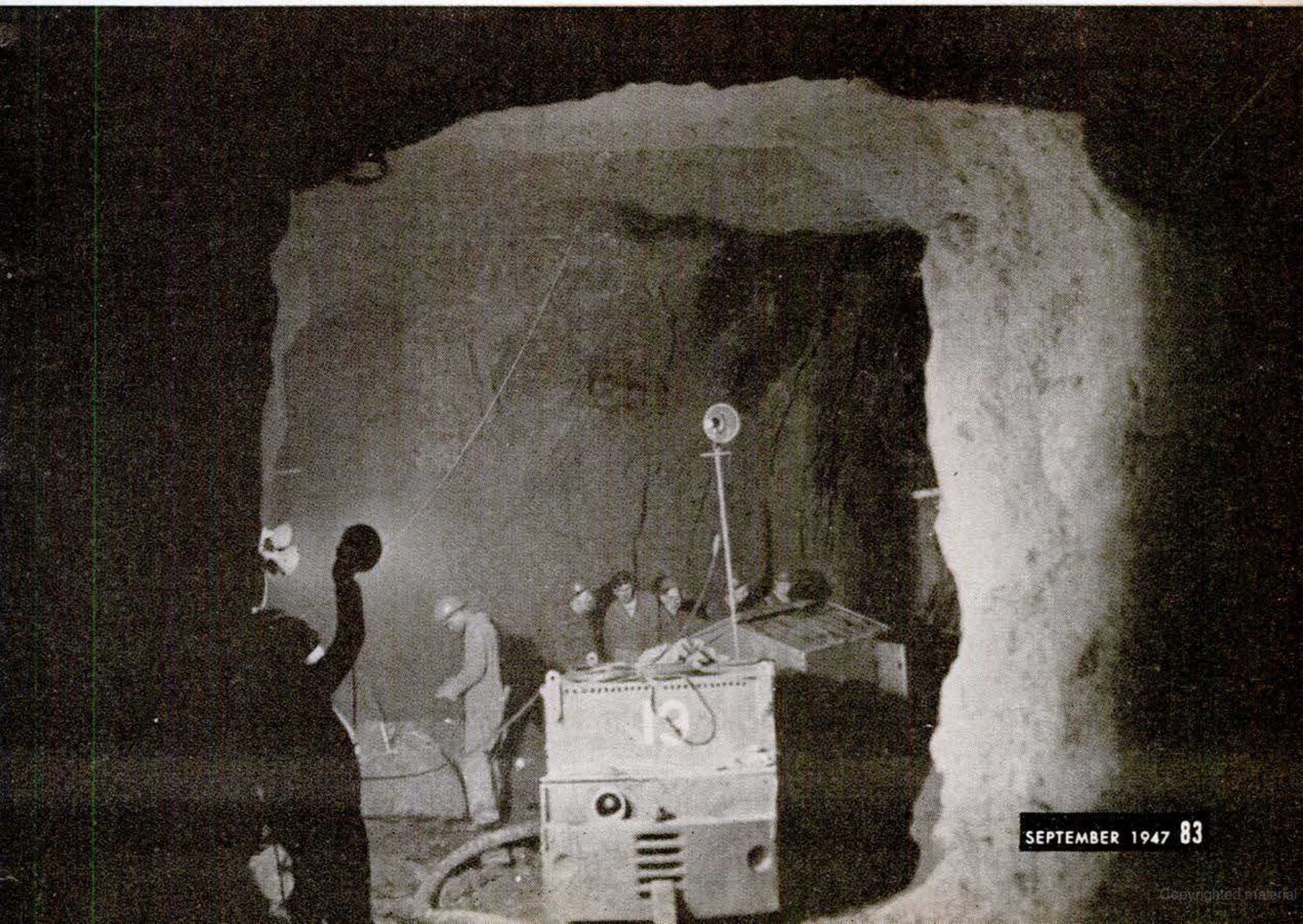
A tunnel locomotive brings up the dynamite car for a blast, in cross-drift between tubes.
