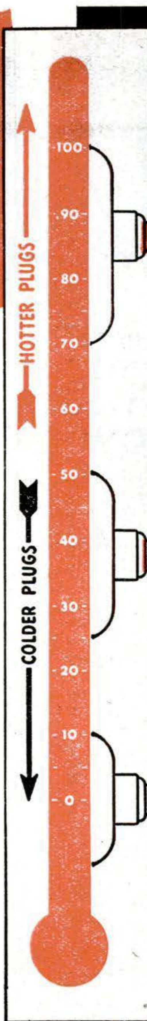
STOP-AND-CREEP DRIVING —Police cars, hearses, door-to-door delivery vehicles, etc. that have long periods of idling usually require a hot plug to prevent fouling.
