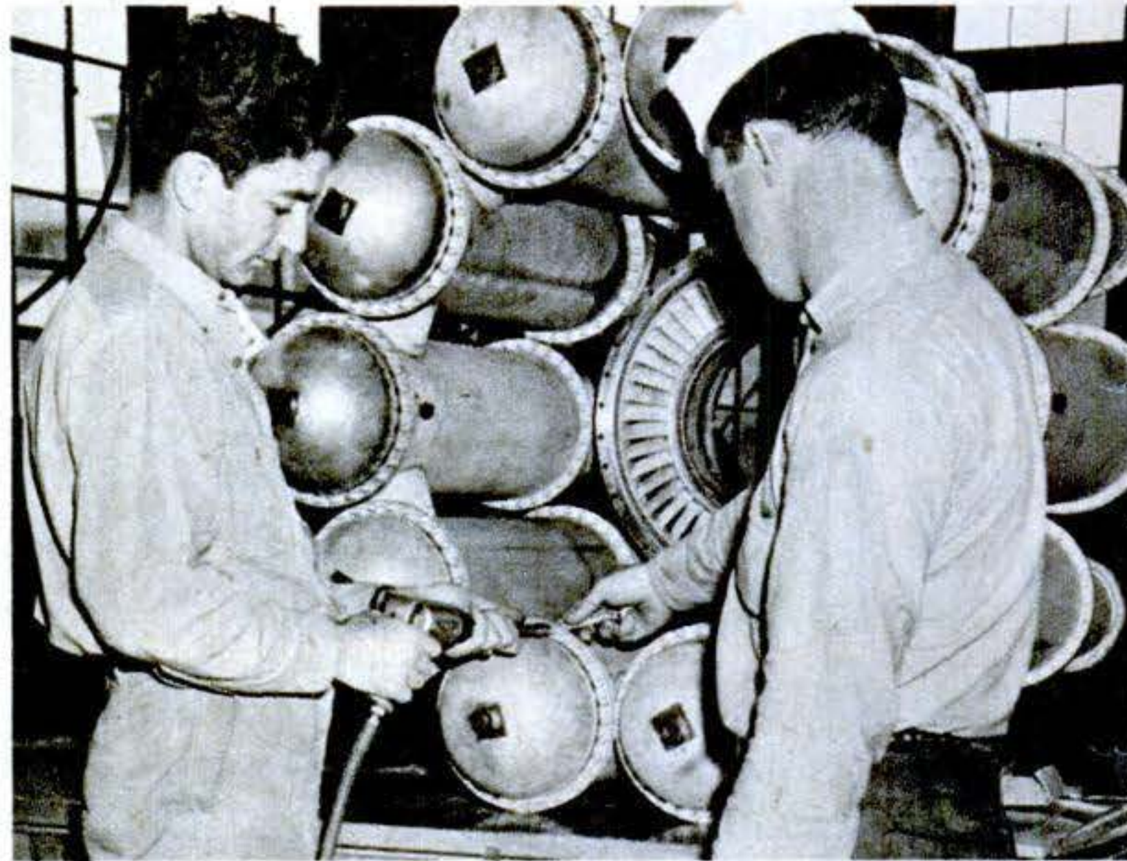
4. Power spinner is used to extract bolts, releasing combustion chamber domes. Rotor vanes are visible in the center.
