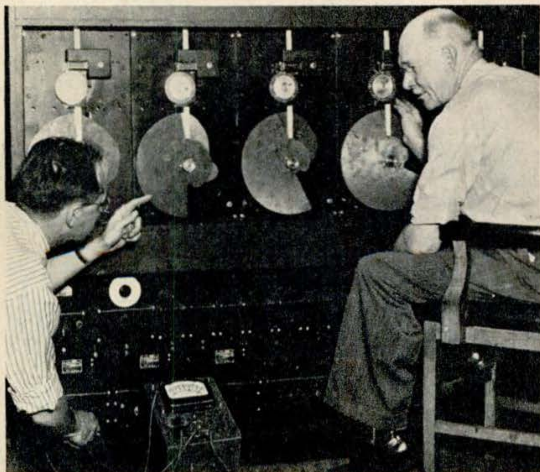
Automatic electronic equipment , governed by cams, produces imitation target "pips" on radar screens for scientifically controlled experiments with radar observation methods.
