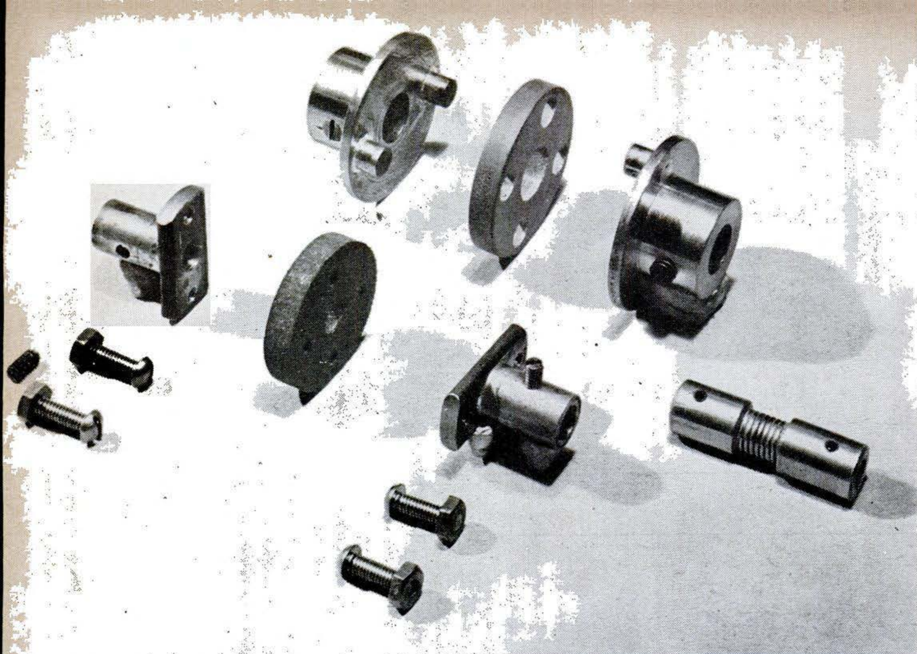
Three types of flexible coupling are seen here. Two use a flexible disk, the third (right) a coil spring.
