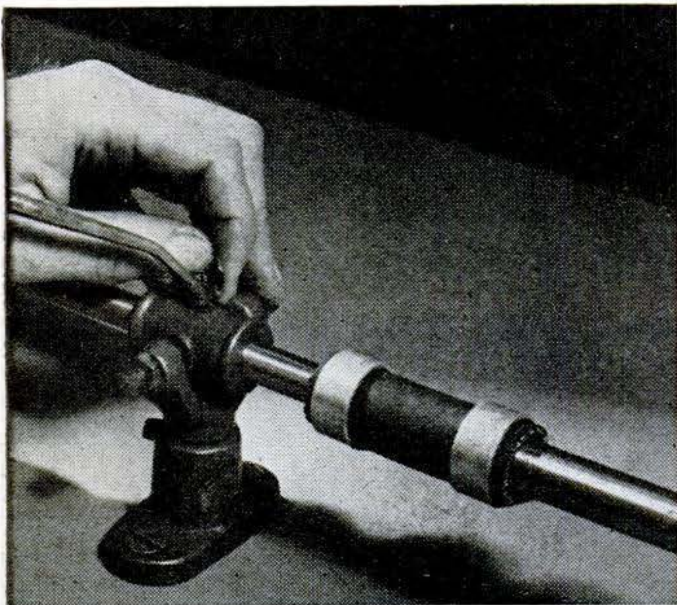
One of the simplest couplings is a piece of rubber hose clamped to the shafts. Here such a coupling is used to join two shafts of different diameters.
