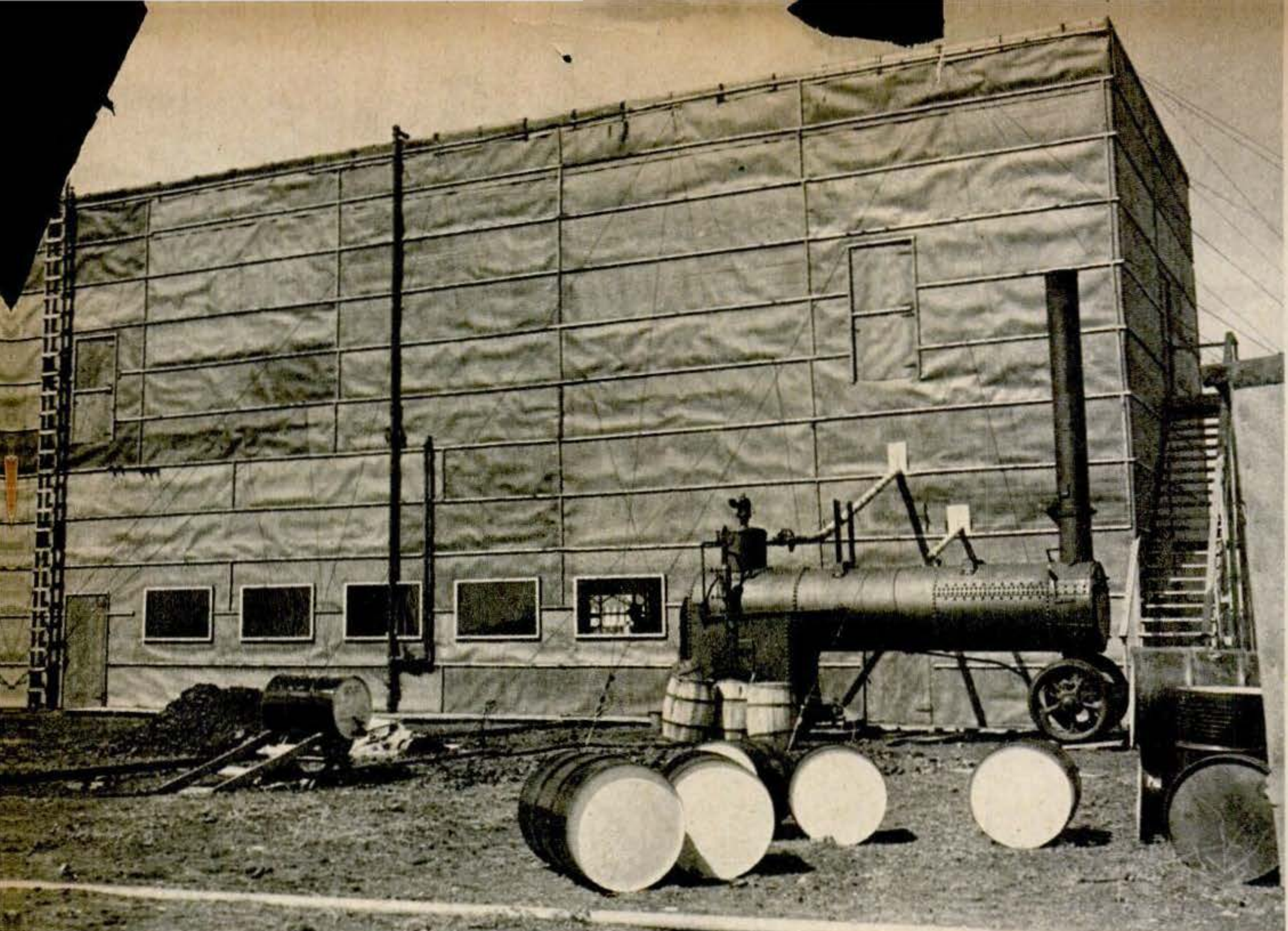
This two-story building, largely tarpaper on a tubular steel framework, was erected for tests of the new system. It contains a
