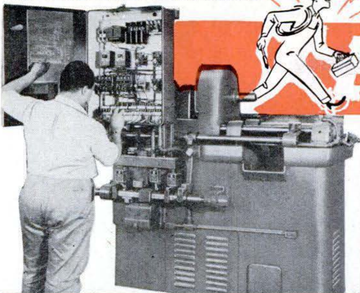
ABOVE: WIRING IN FACING MACHINE
