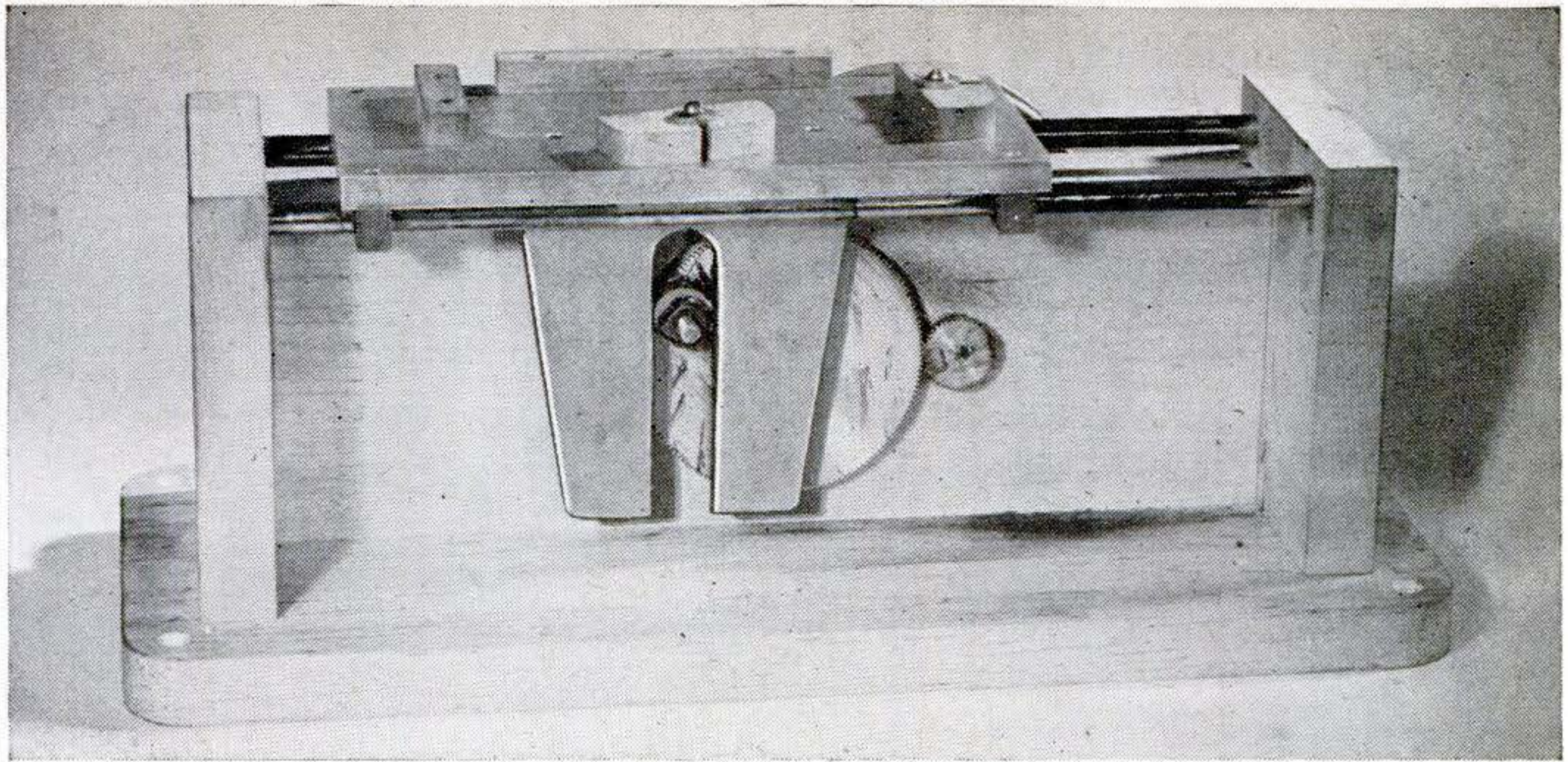
Movement of a ball bearing in a yoke operates the stone table. The bearing fits the slot without play.
