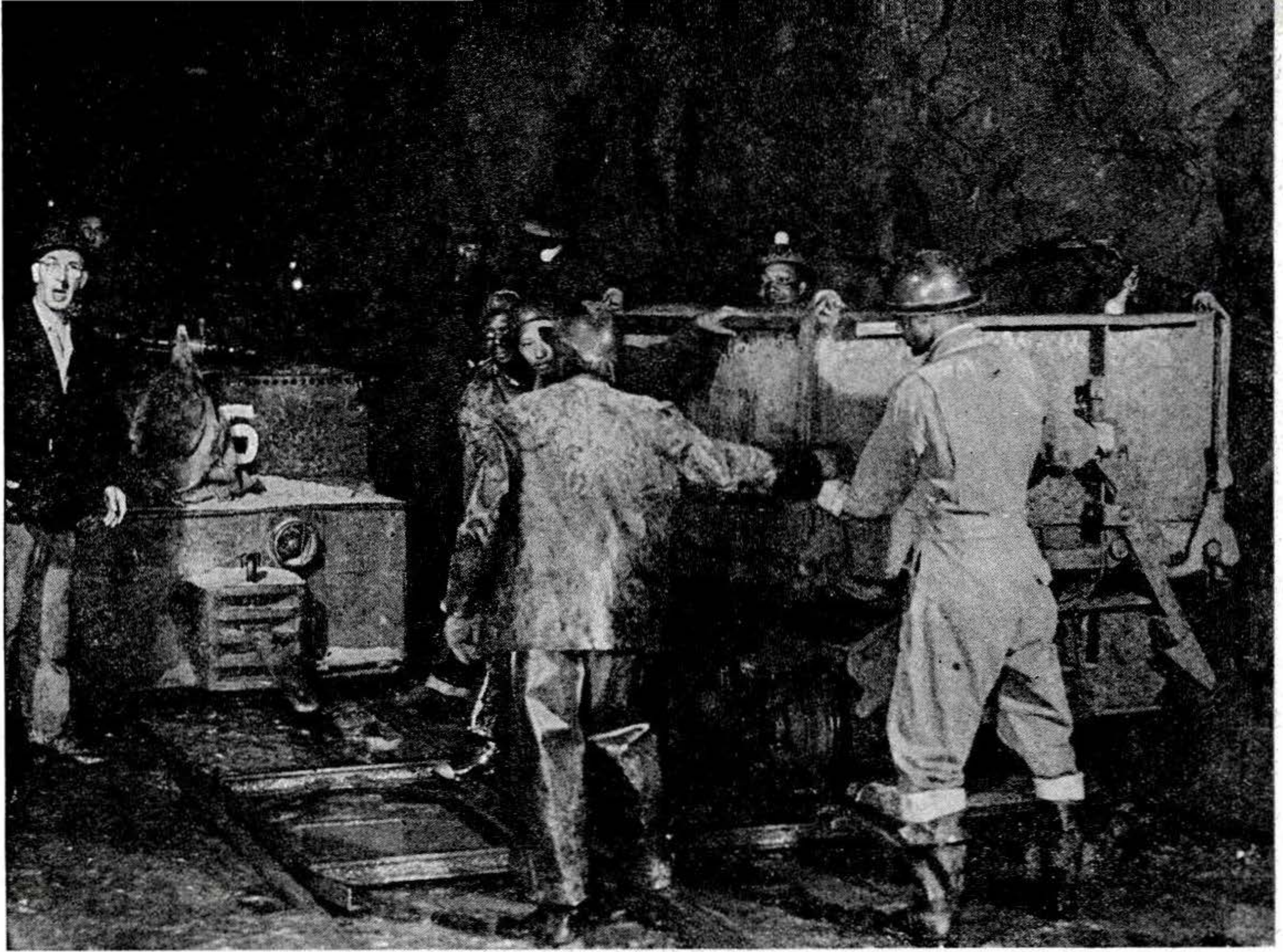
Shunting maneuvers with California switch prevent runaways on downgrade to the heading.
