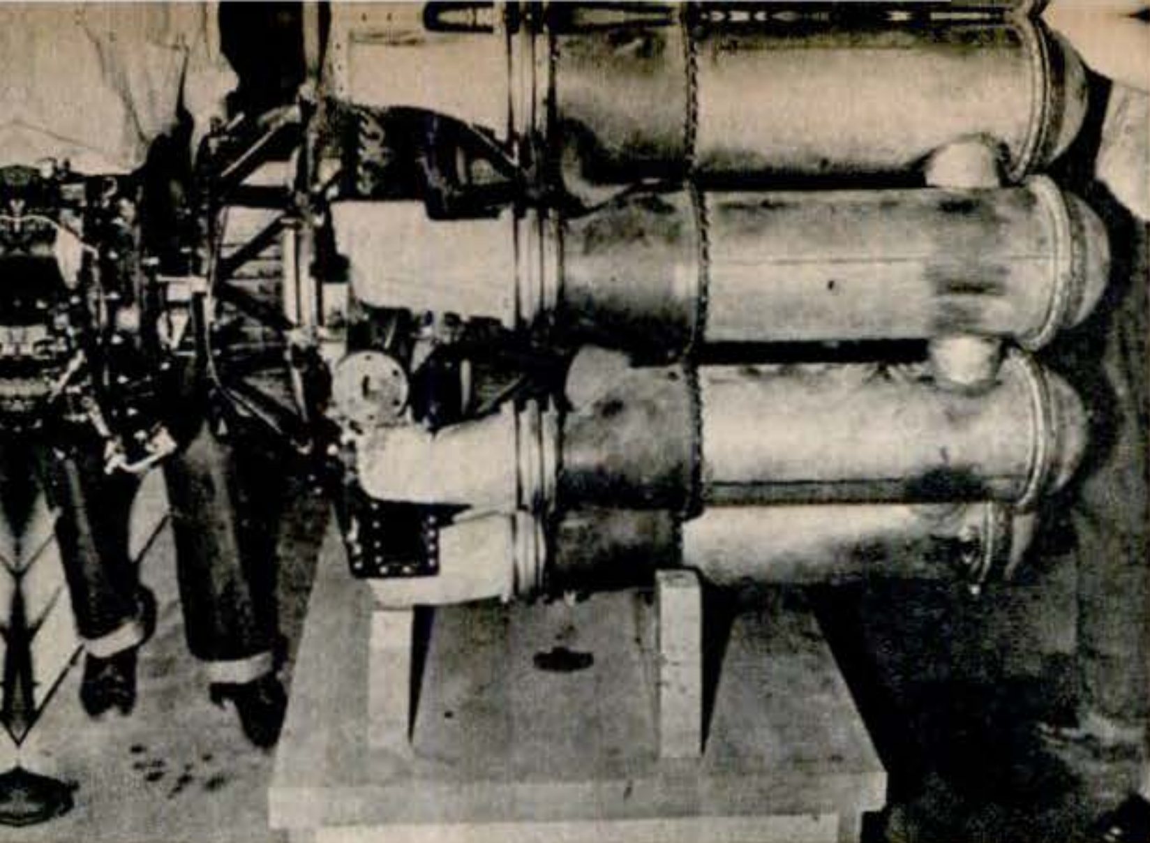
2. For first step in disassembly, engine is placed on horizontal stand and accessory case (left) removed before tear-down begins.
