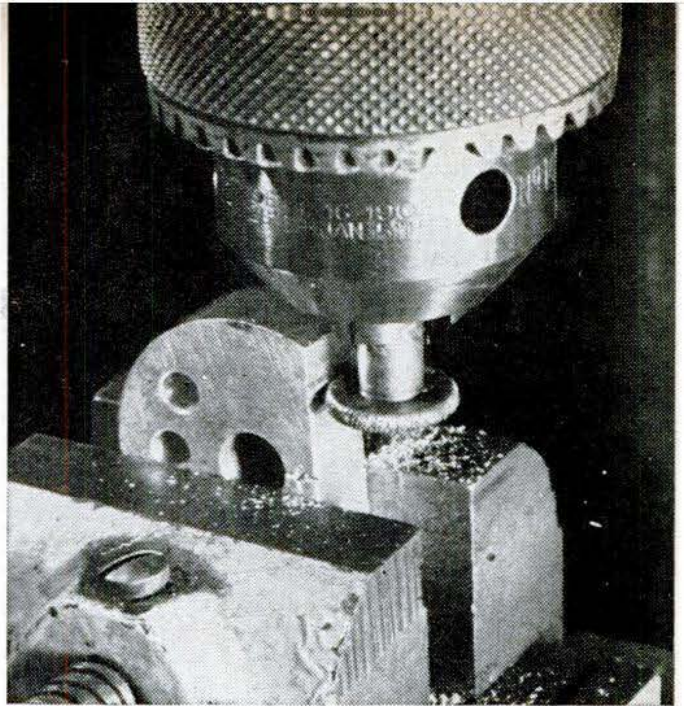
In a drill press, rotary files will shape cavities, burr or enlarge holes, and do many smoothing jobs.
