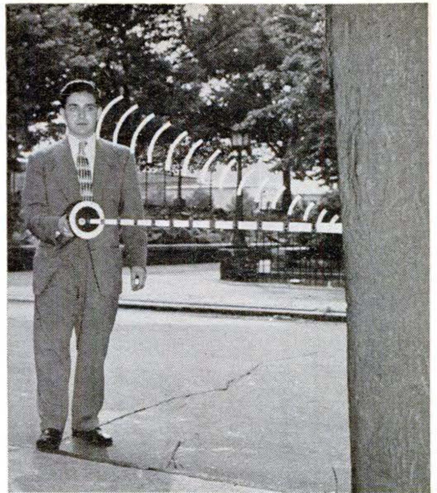
Projected beam of "sound flashlight" is shaped by the reflector, but when it bounces off tree it is audible to the user and anyone else near by.
