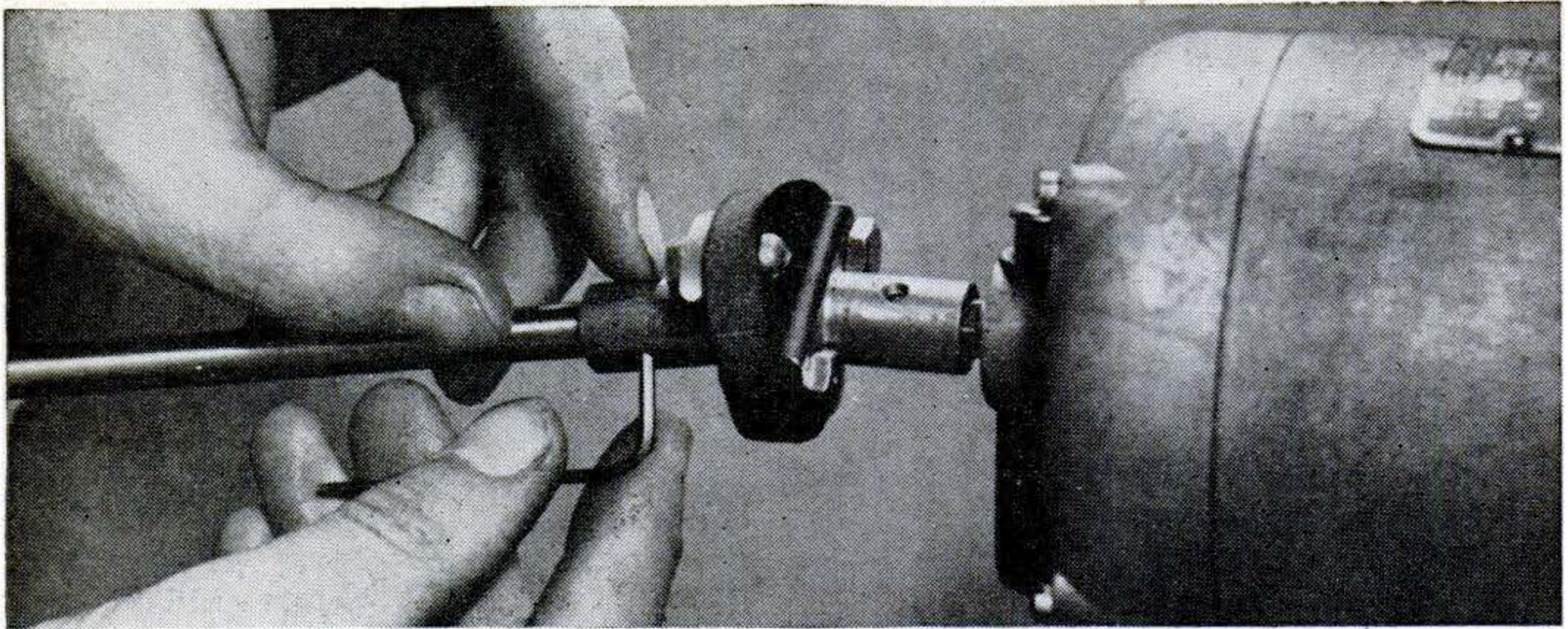
In this coupling, each end consists of a sleeve with a piece of flat stock brazed on in the form of a T.
