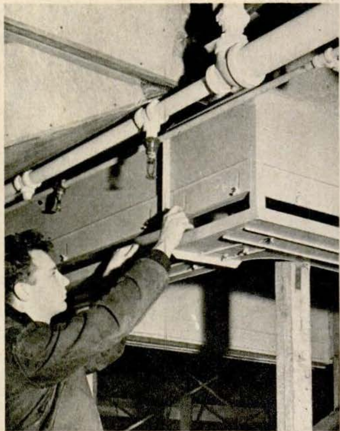
Technician examines damper in exhaust duct that circles escalator well. Through this duct smoke and fumes from fire are sucked outside building by fan, creating downward draft that blocks chimney effect of stairs.
