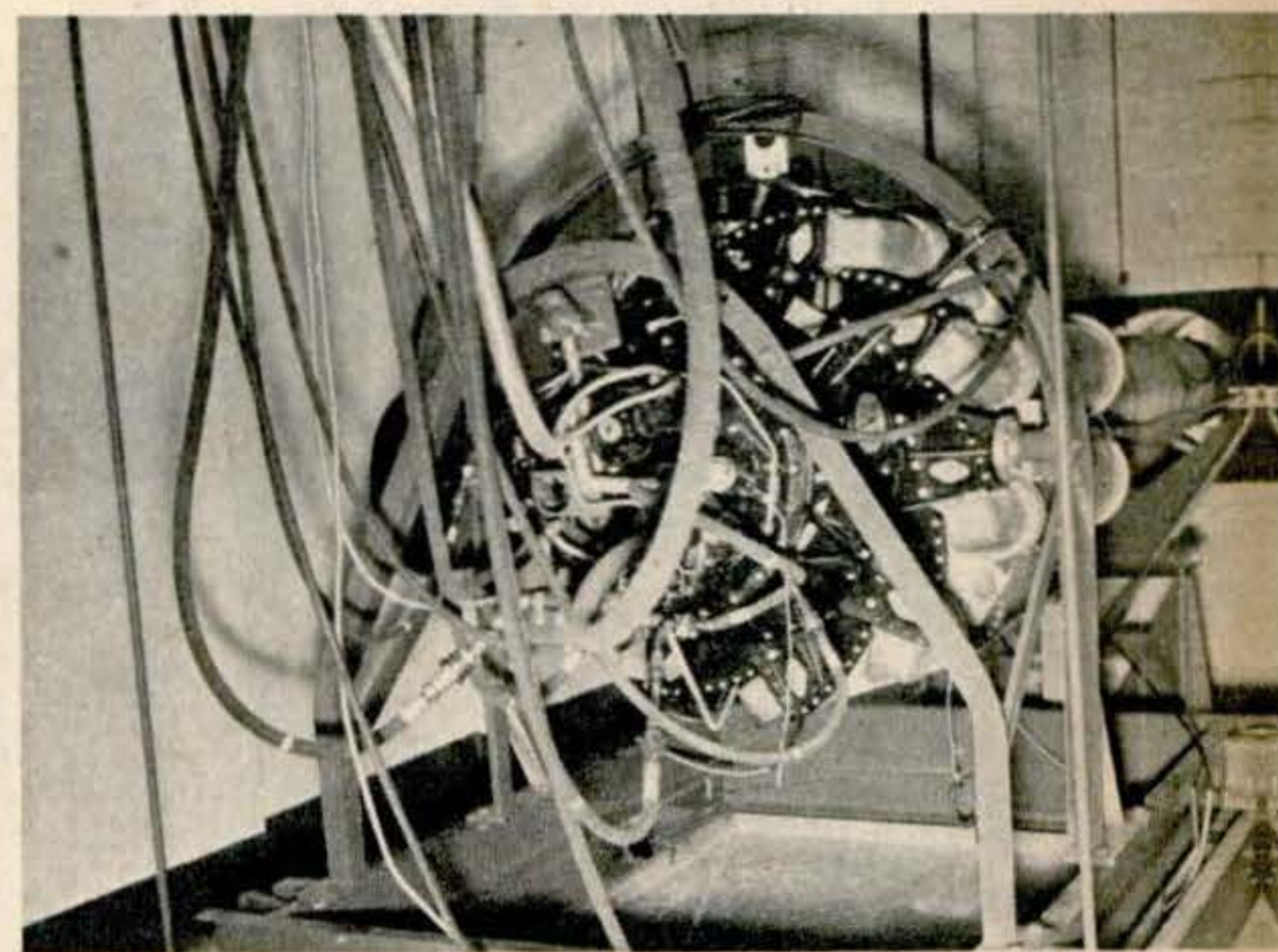
9. Reassembled engine, under power, gets final check. Run from adjoining room, jet blasts against deflector outside test cell.
