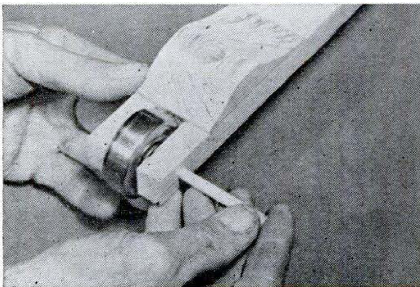
Skate wheels turn on axles cut from a hardwood dowel. Drill rod or bolts are also suitable. This wheel is set in the top of the back upright.
