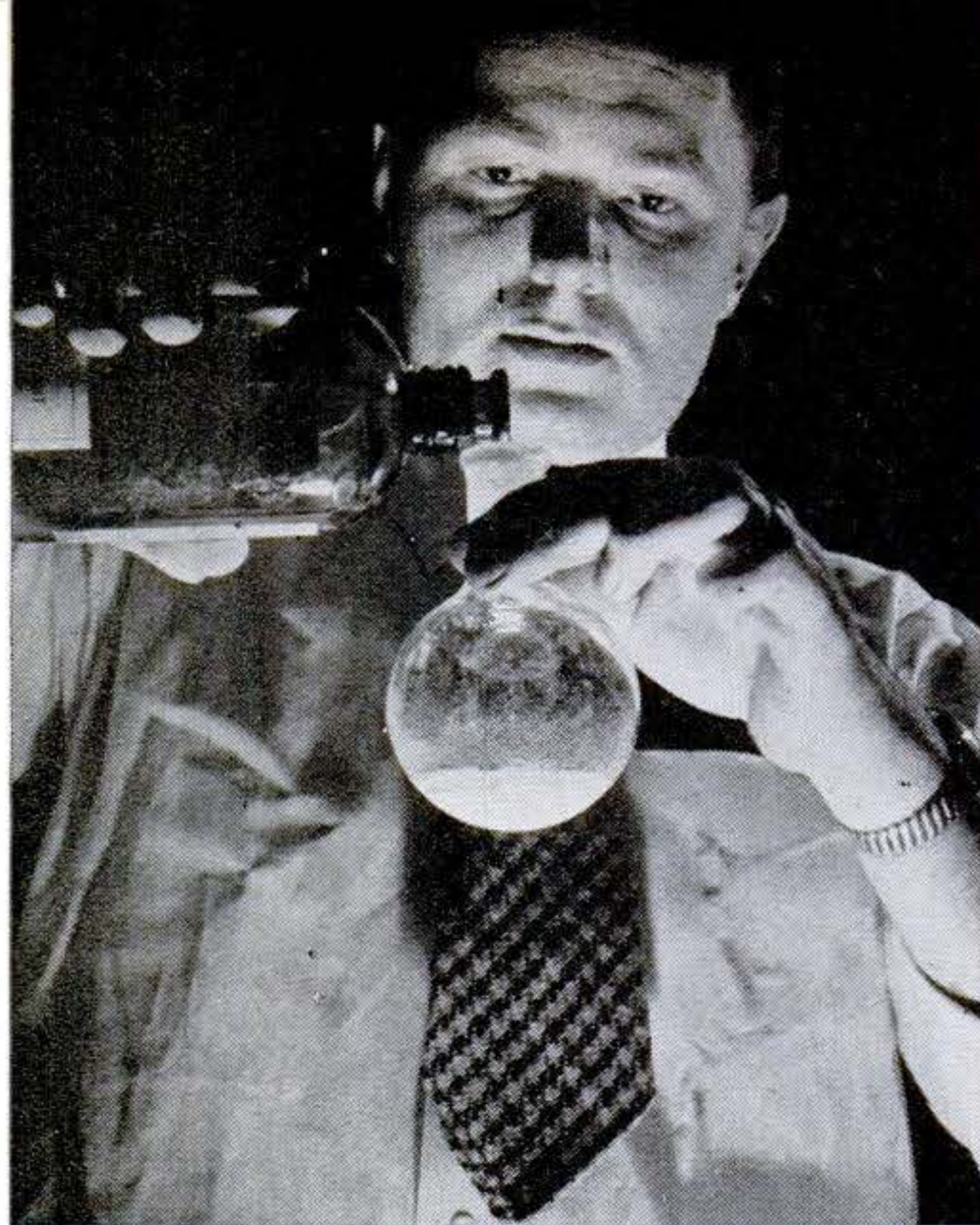
Two or more different amino-acid anhydrides are dissolved in benzene to make the solution that becomes a "protein analogue." A tiny amount of water in benzene starts the reaction.
