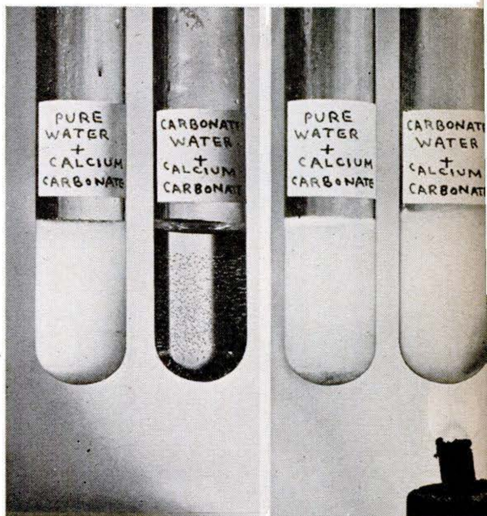
Various carbonates dissolve much more readily in water containing carbon dioxide, as at left. Such water is said to have temporary hardness because boiling, as at right, precipitates the carbonates.
