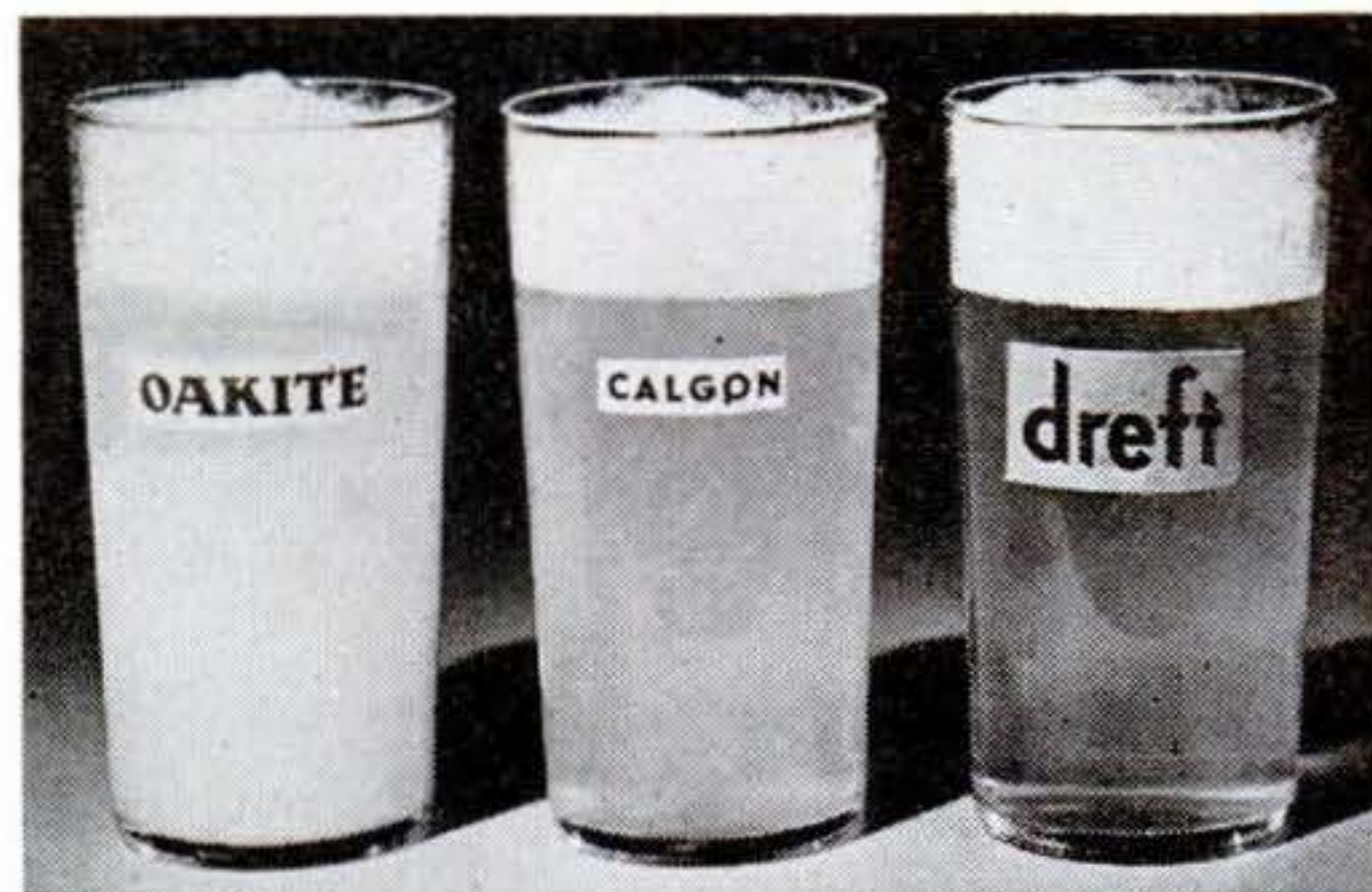
Now, however, you have a choice of such agents as these. Oakite precipitates the hardness, Calgon ties it up in complex compounds, while Dreft, one of the new synthetic detergents, just ignores it.
