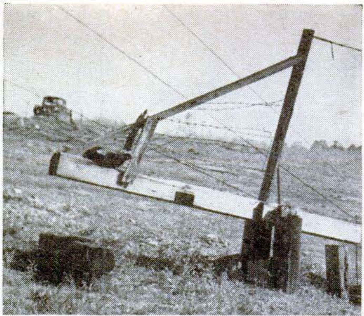
Pump rod, at extreme right, has only a short throw, but each upstroke sends a quart of water to tank, 400 feet away and 30 feet higher.
