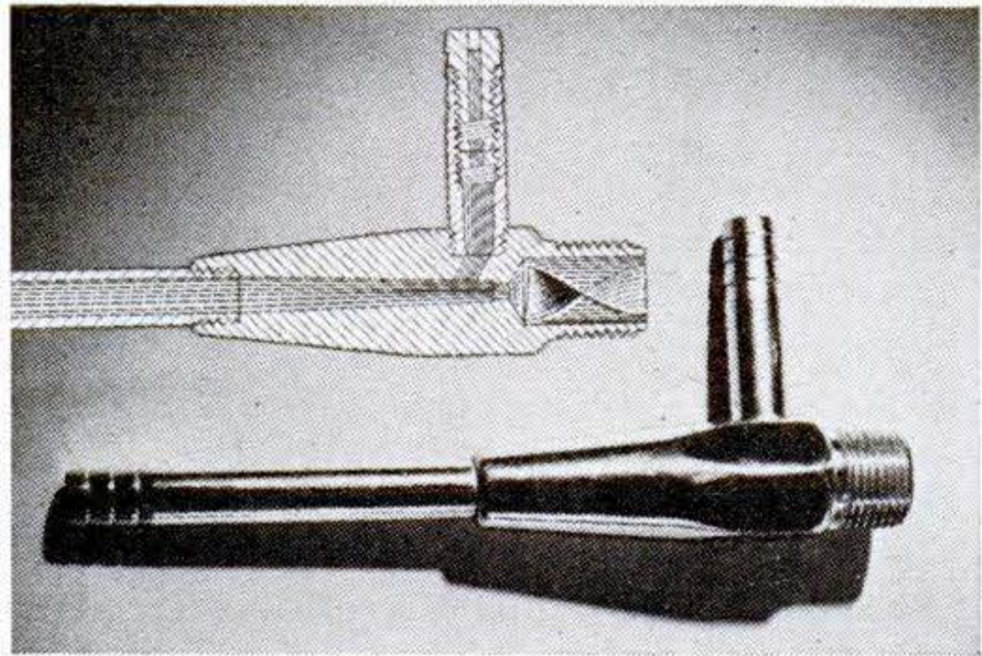
Screw the threaded end of the pump, right, into a faucet, and press rubber tubing on the short tube.
