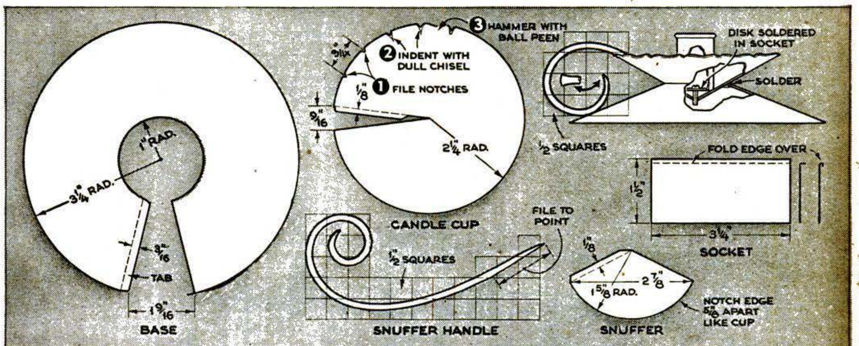
Candle sockets are easily bent around a length of rod of candle diameter. The folded edge closes to form a neat roll during the process.
