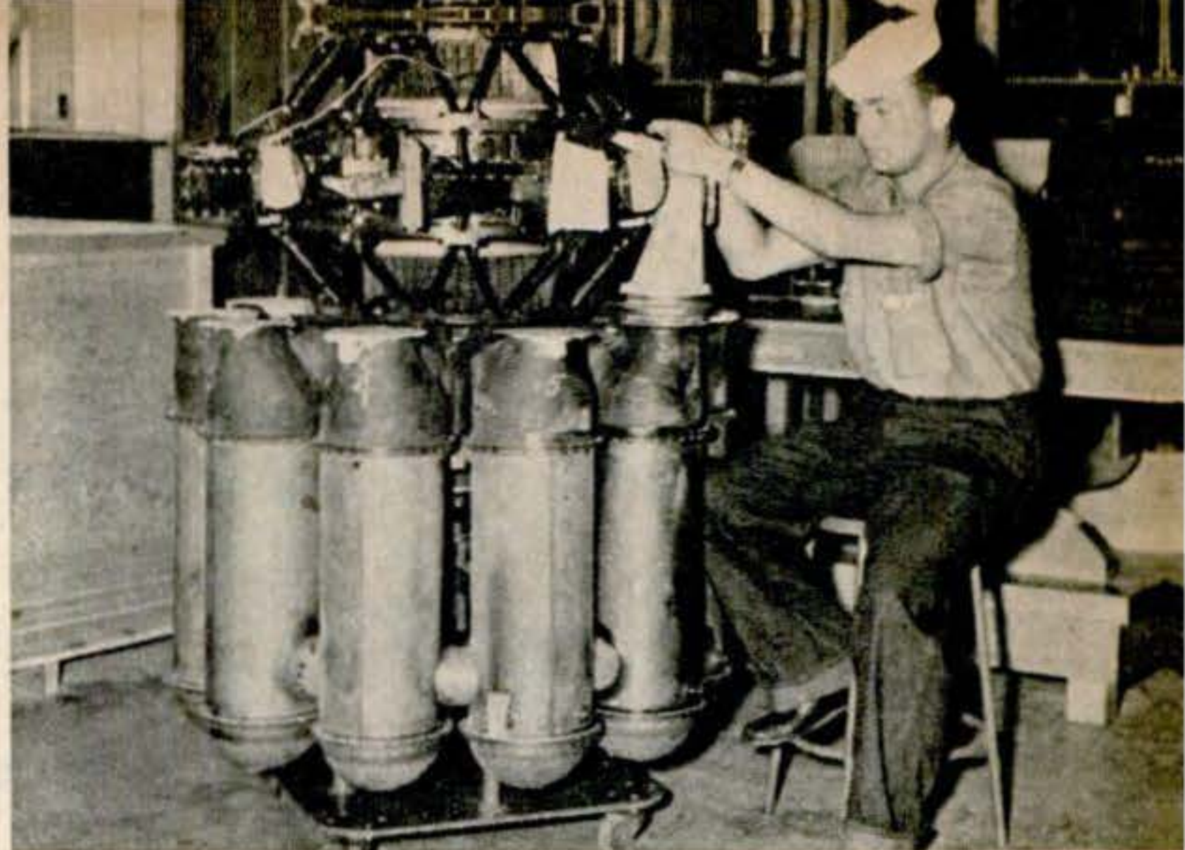
3. Engine shifted to vertical position, Navy mechanic removes the elbows. All types of Navy jet engines are handled at Alameda.
