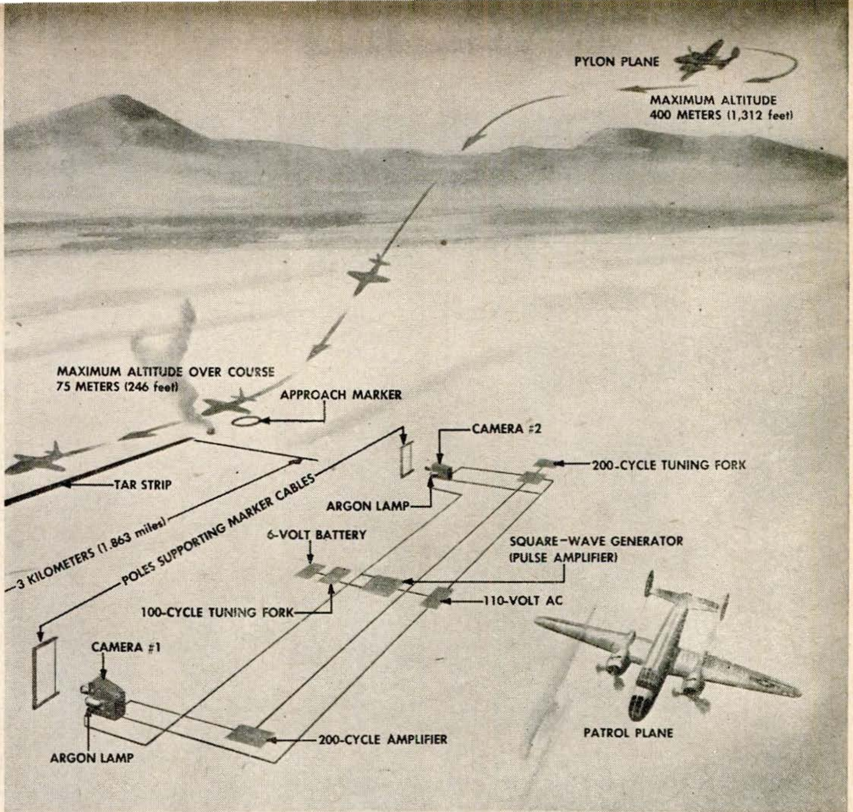
Making four passes "on the deck," at 50-foot altitude, plane flew one run at 632.5 m.p.h.
