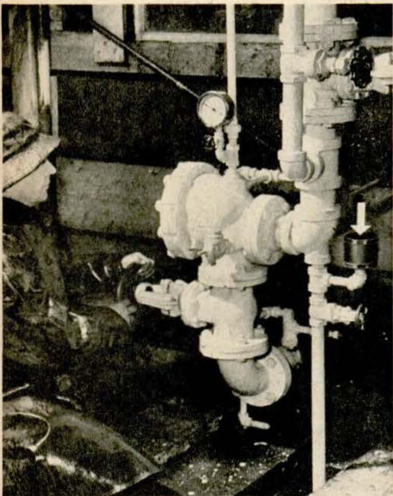
Automatic control (arrow) works by water pressure when first sprinkler is set off. It sounds alarm, stops escalators and air conditioning, starts exhaust fan, and opens dampers in exhaust duct and air intake.
