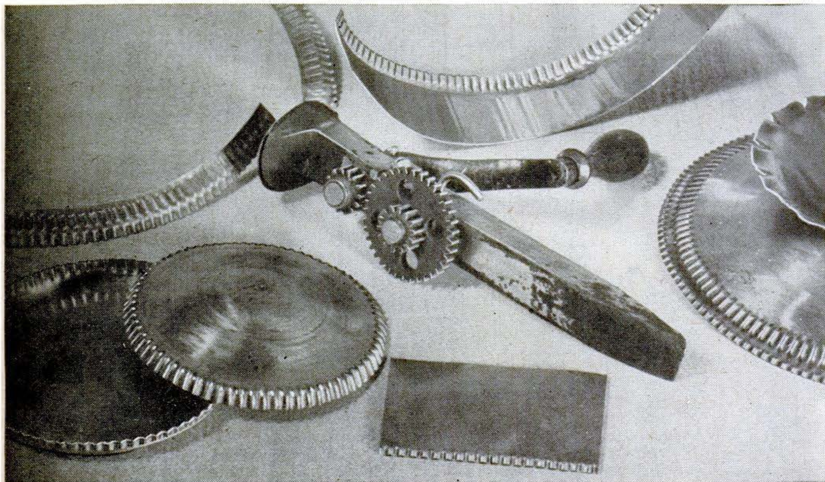
A crimper mounted on a railroad spike and some edges it makes. The handle is from a pencil sharpener.
