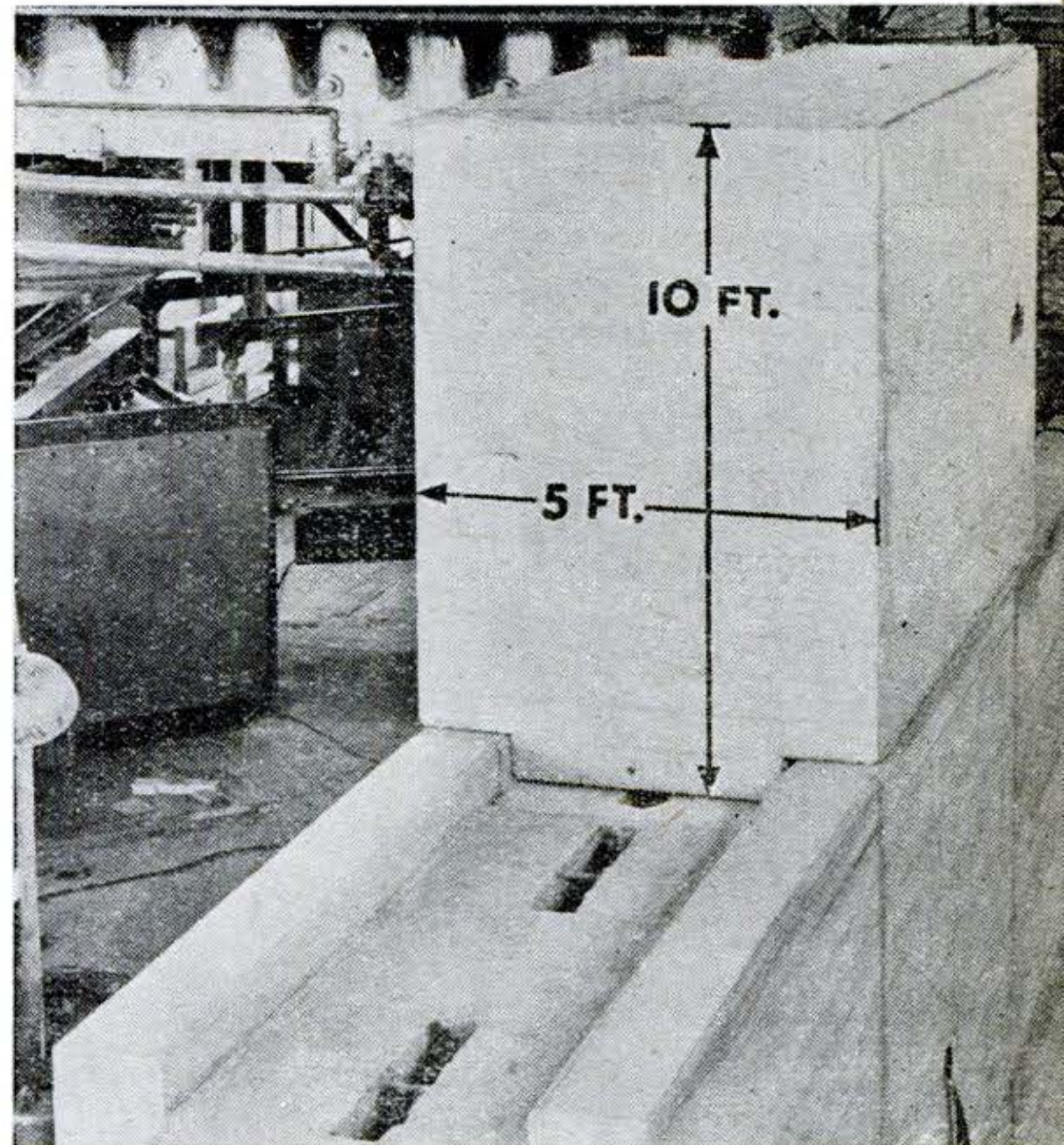
Partly completed wall shows how blocks interlock to bar possible leakage through joints.
