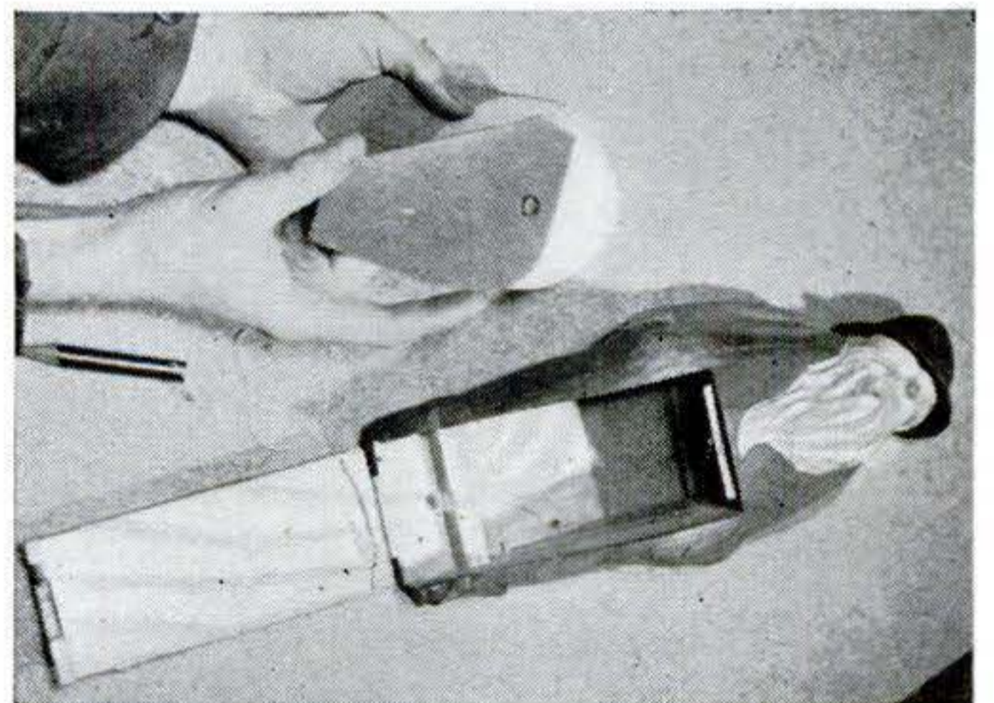
Paper-roll supports , notched and drilled for a dowel, hold the roll of adding-machine tape.
