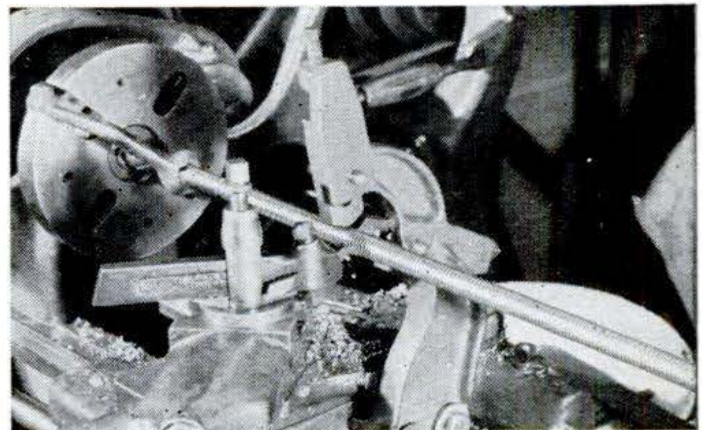
Use a follower rest in cutting threads on the longitudinal feed screw. Standard V-threads will serve for this and the other two table-control screws, but Acme threads are better.
