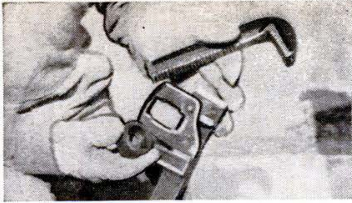
Remove the nut and jaw of a big pipe wrench to use it as a chain wrench.
