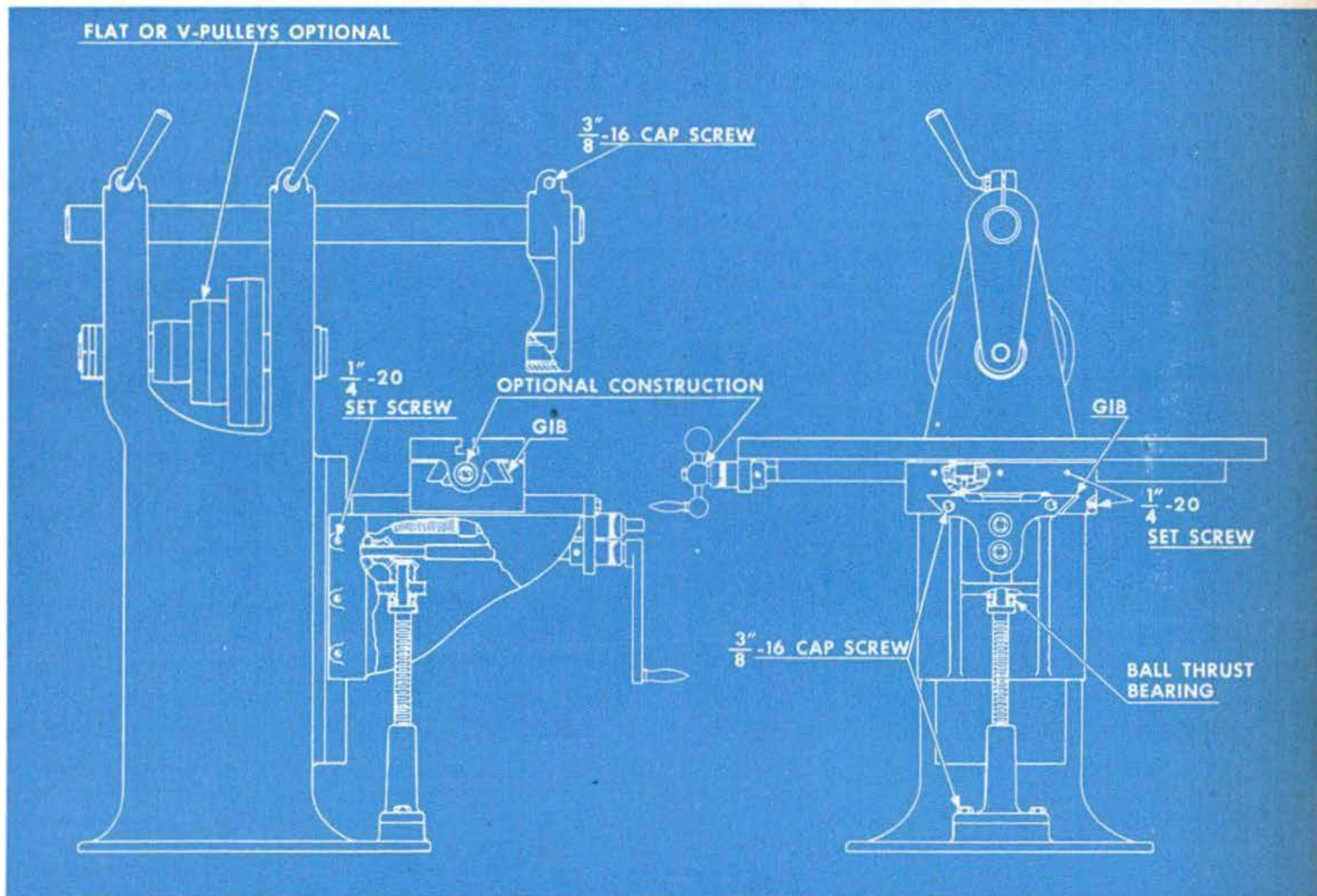
This is it —the finished mill at work. Below, an assembly blueprint furnished with castings.
