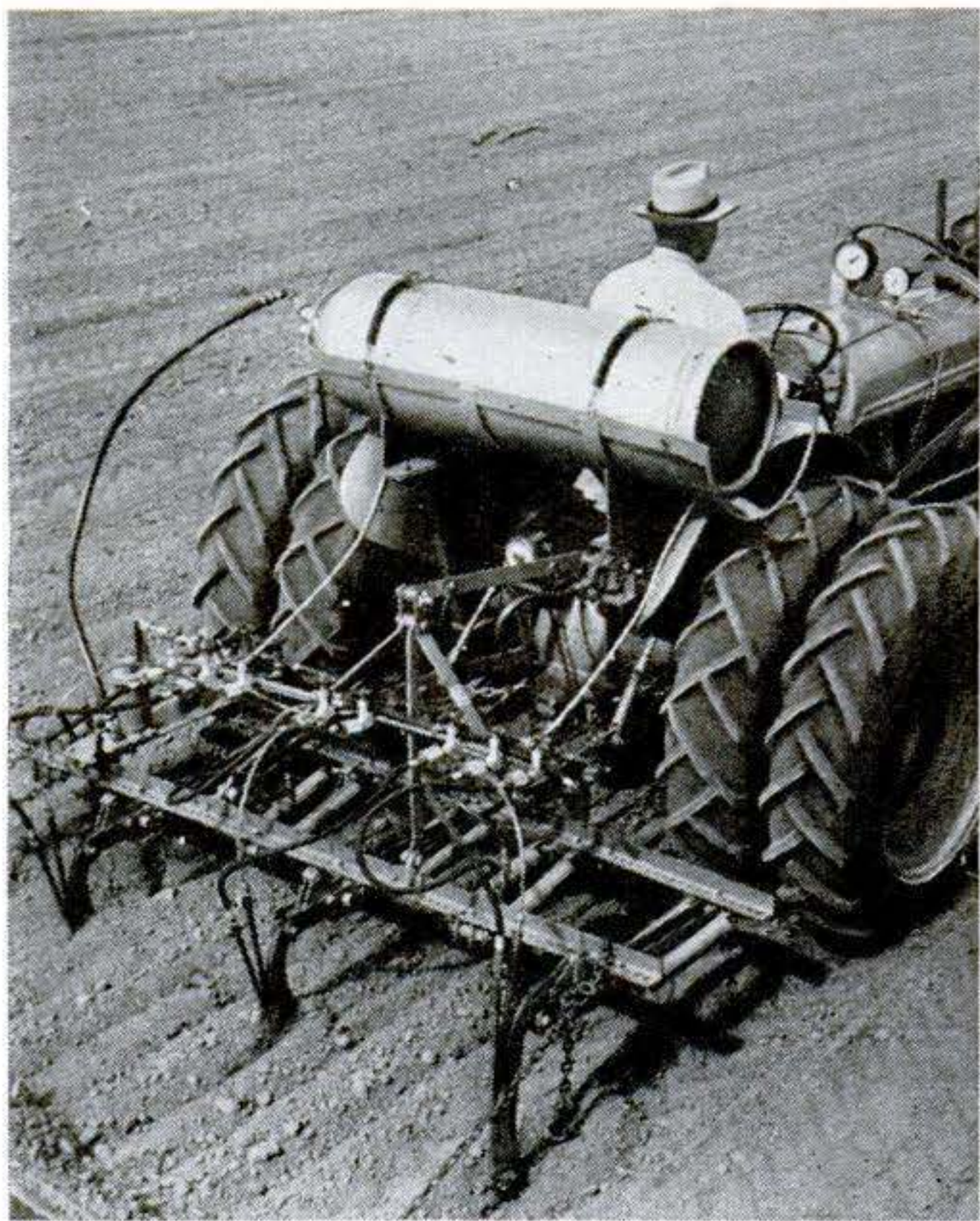
Dry method: Ammonia and D-D are piped directly into the soil. Tubes behind the blades of this tractor-drawn harrow direct the chemicals into the ground eight inches below the surface.
