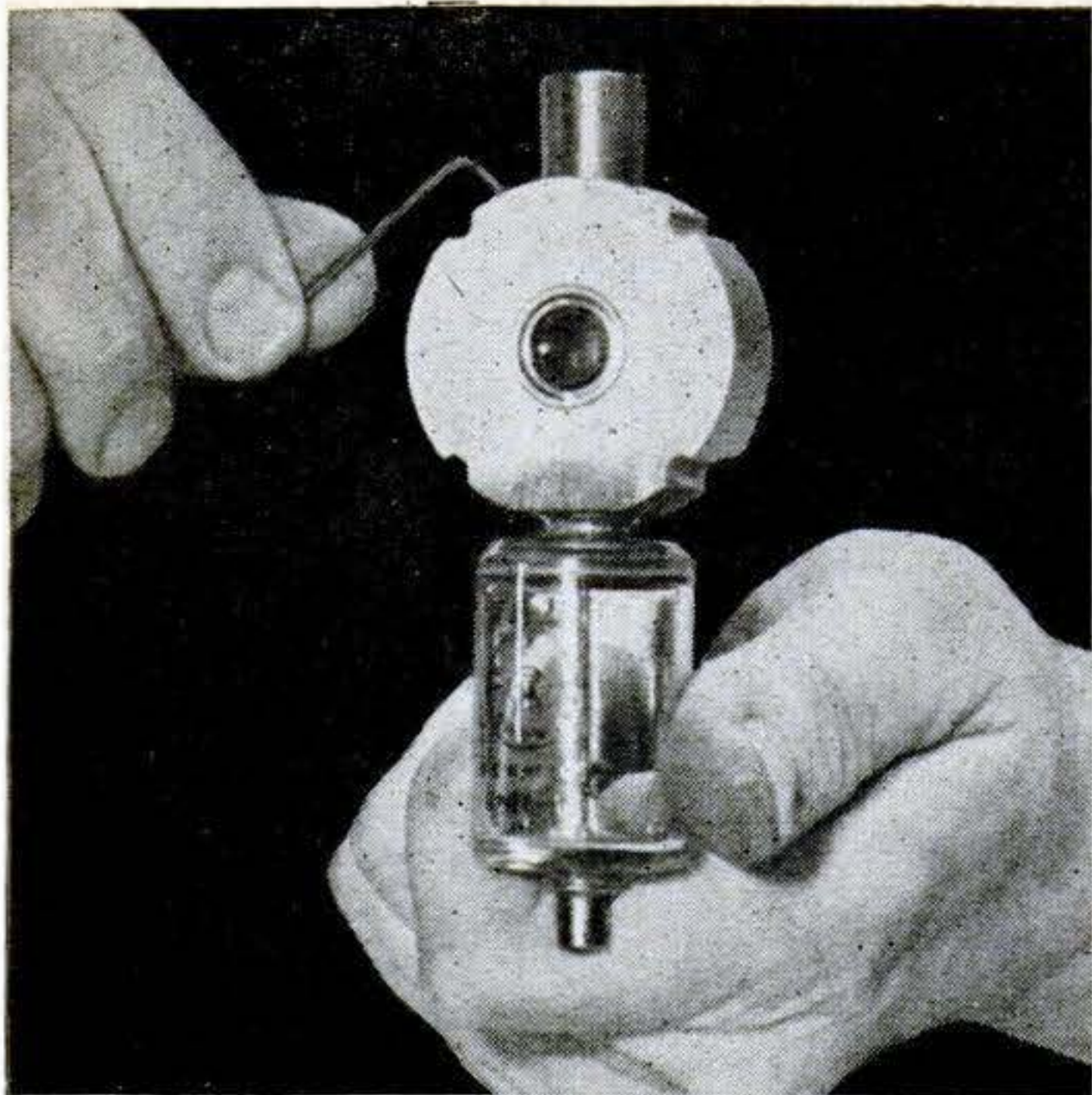
Radar sets need only one antenna, thanks to TR switch (above), which changes antenna from "transmit" to "receive" in a few microseconds.
