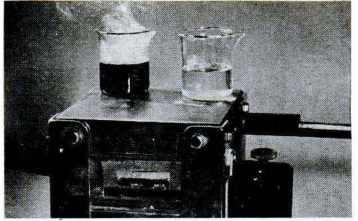
Silicone oil at right resists heat and remains clear in comparative test on hot plate. Petroleum oil, left, is decomposing, as shown by darkening and by smoke rising from liquid.
