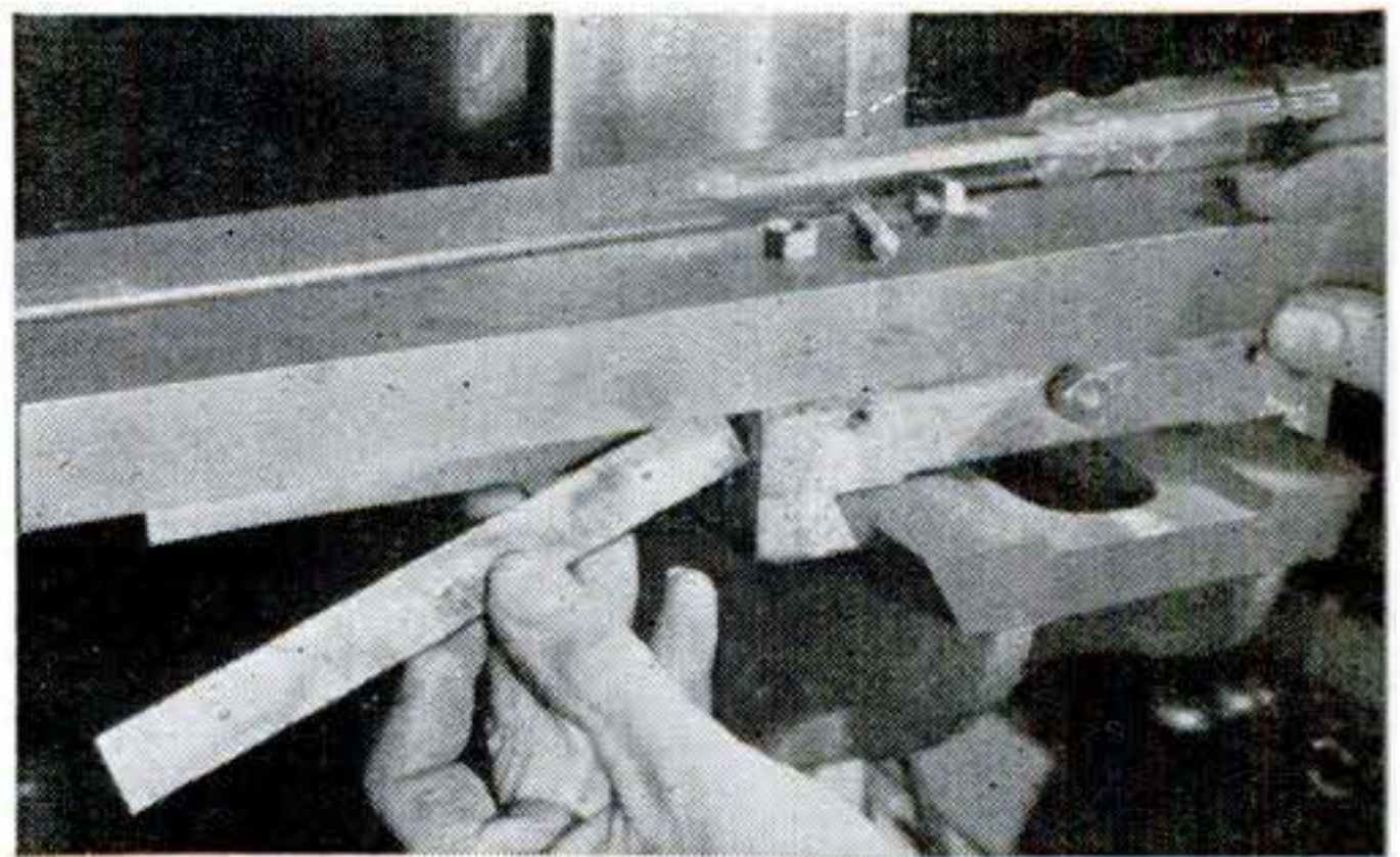
Gibs are cut to length from steel strips and their edges are beveled to match the dovetail angles. After placing the gibs in position, spot-drill each to receive the screw points.
