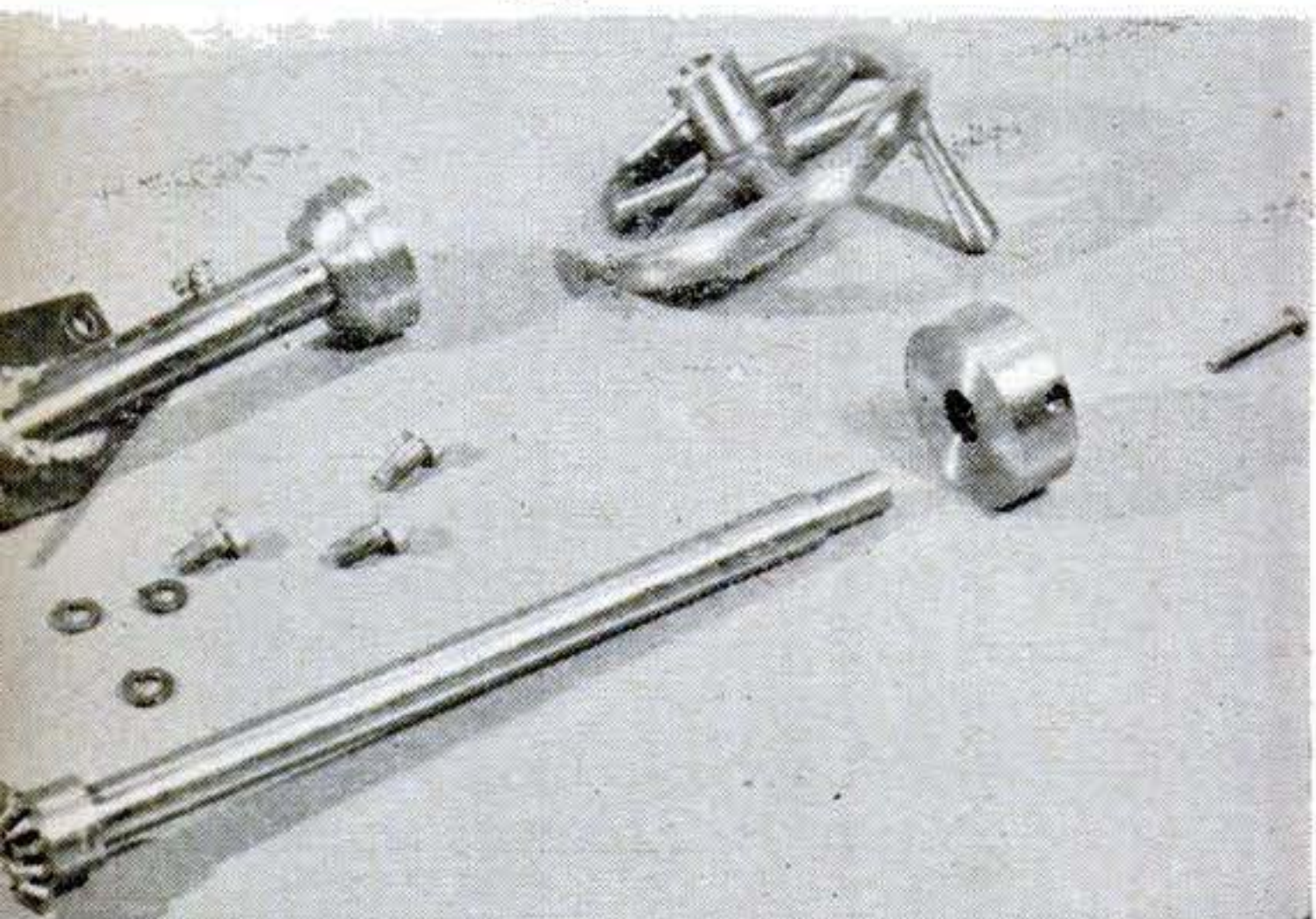
Three \frac{5}{16} " bolts attach the elevating-shaft mounting plate to the side of the knee casting, a \frac{7}{8} " diagonal hole being bored through the casting itself for the tubular housing.
