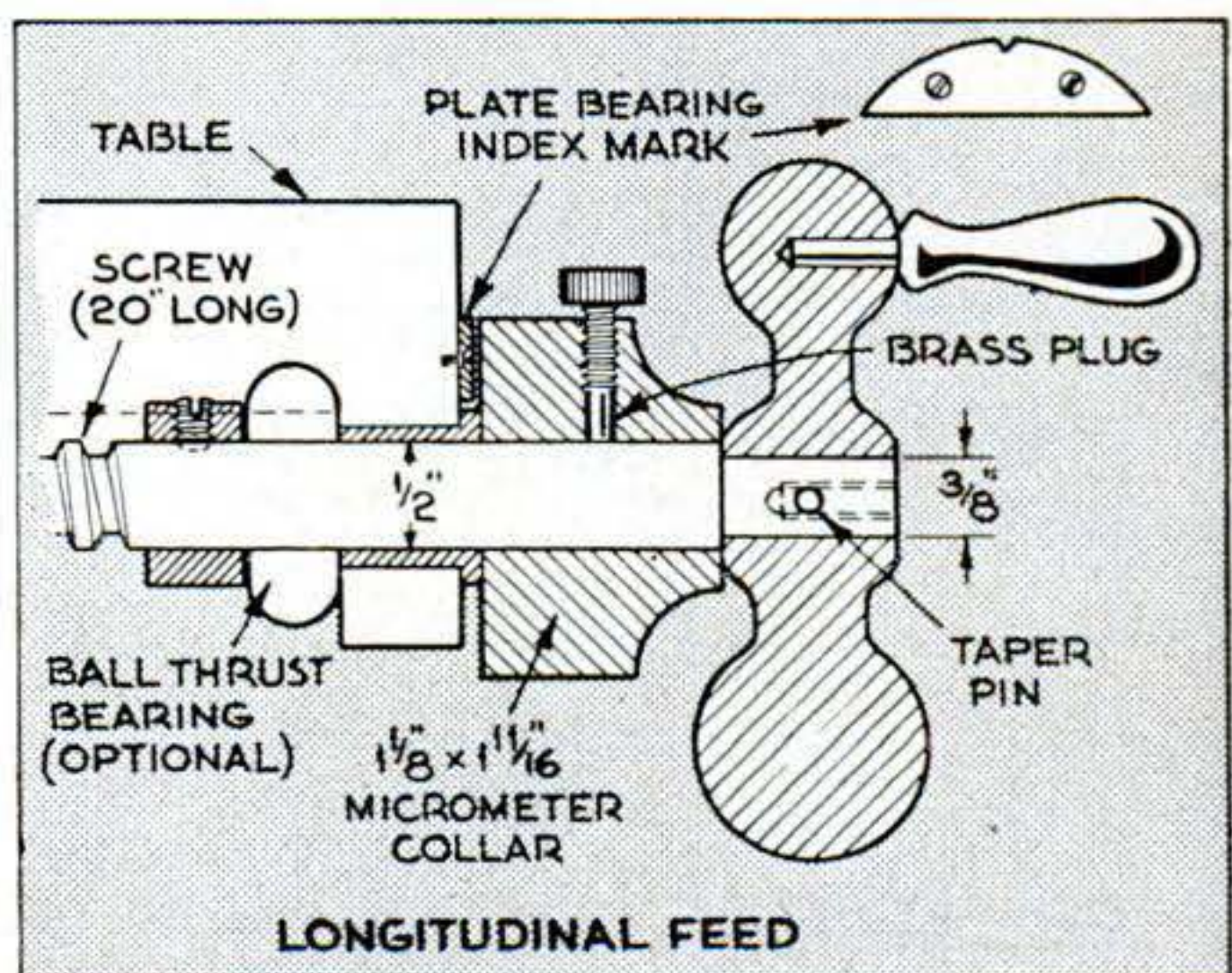
Use a follower rest in cutting threads on the longitudinal feed screw. Standard V-threads will serve for this and the other two table-control screws, but Acme threads are better.
