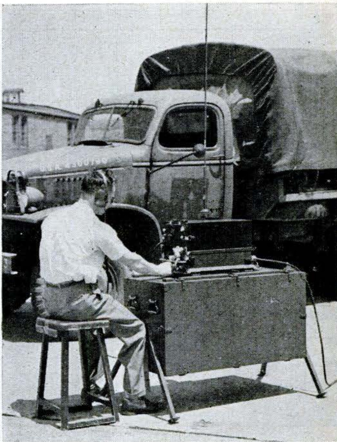
A radio-noise detector , this compact test set was developed to check suppression devices on equipment purchased by the Army. Measuring impulse noise from .15 to 40 megacycles, it will also enable repair depots to spot and eliminate interference from older-type equipment.
