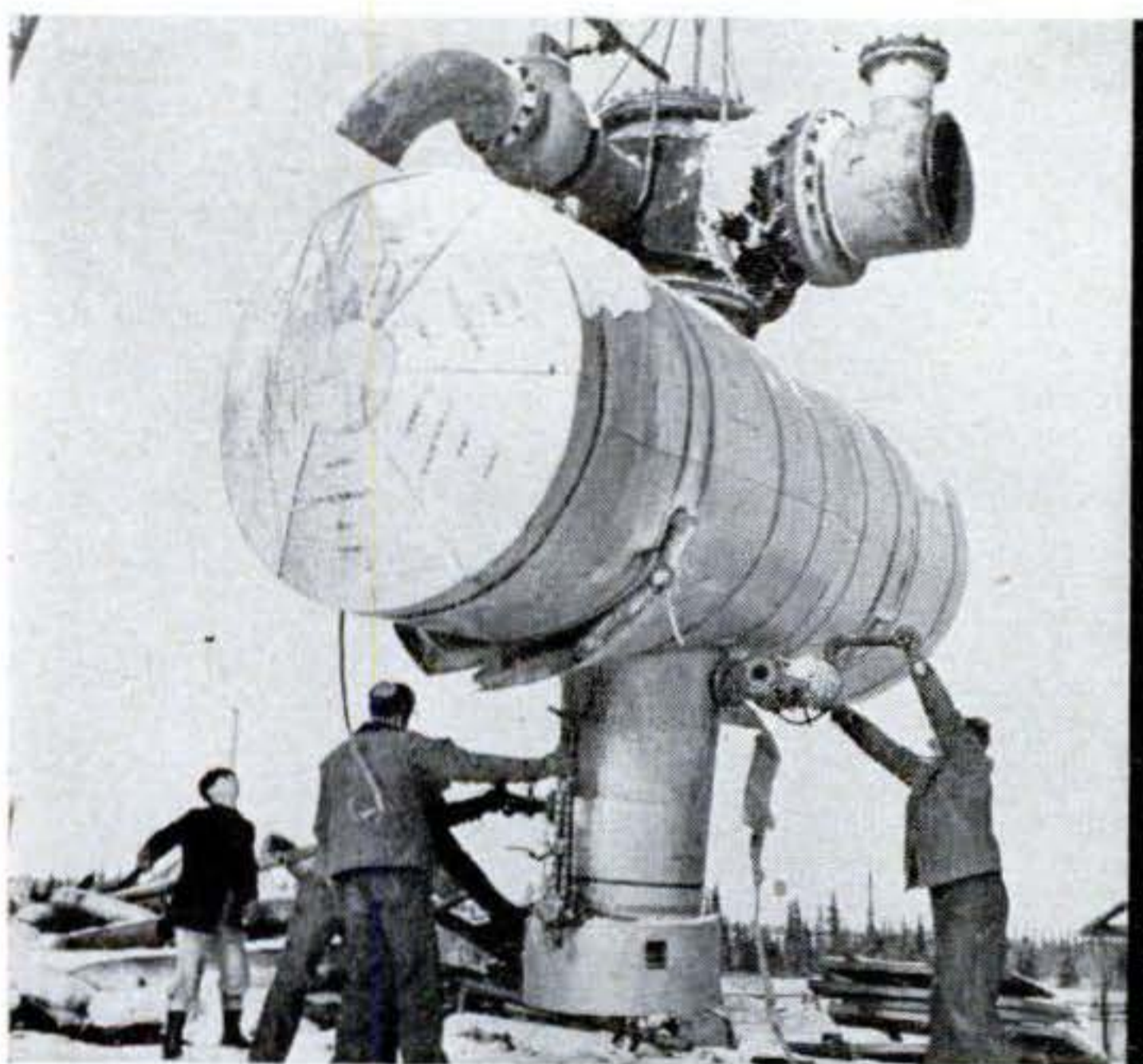
4 A huge condenser, being lowered by a crane, is maneuvered into a clearing where it was broken down for easier truck loading.
