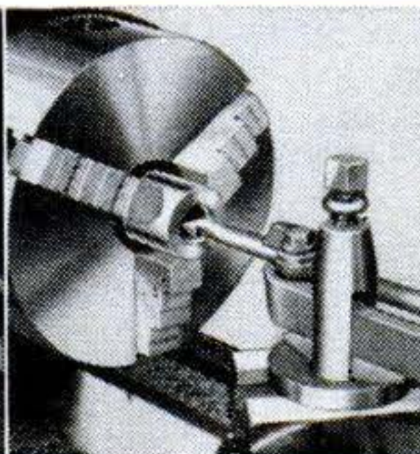
BORING
