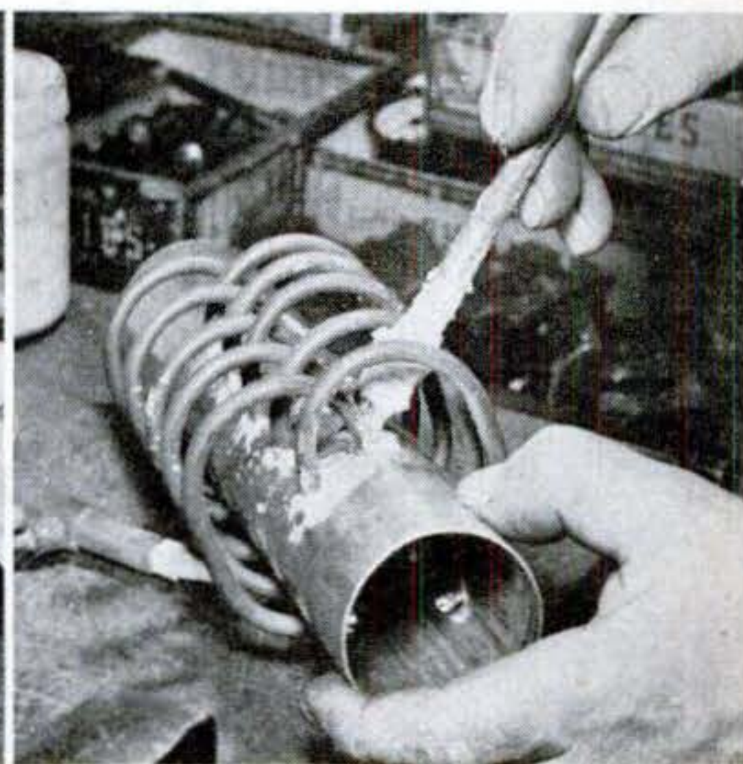
Silver-soldering flux is applied with brush. Anton Bohaboy uses commercial flux instead of borax. Note how upper ends of tubes protrude into shell. Lower ends are more nearly flush.
