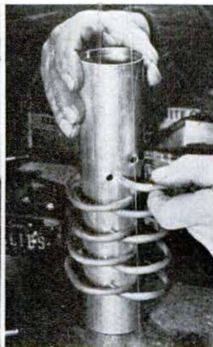
Pieces of copper tubing are bent to an open O shape on a jig. Correctly made, they have to be sprung into holes, which are cocked to suit by inserting rod, bending to position.
