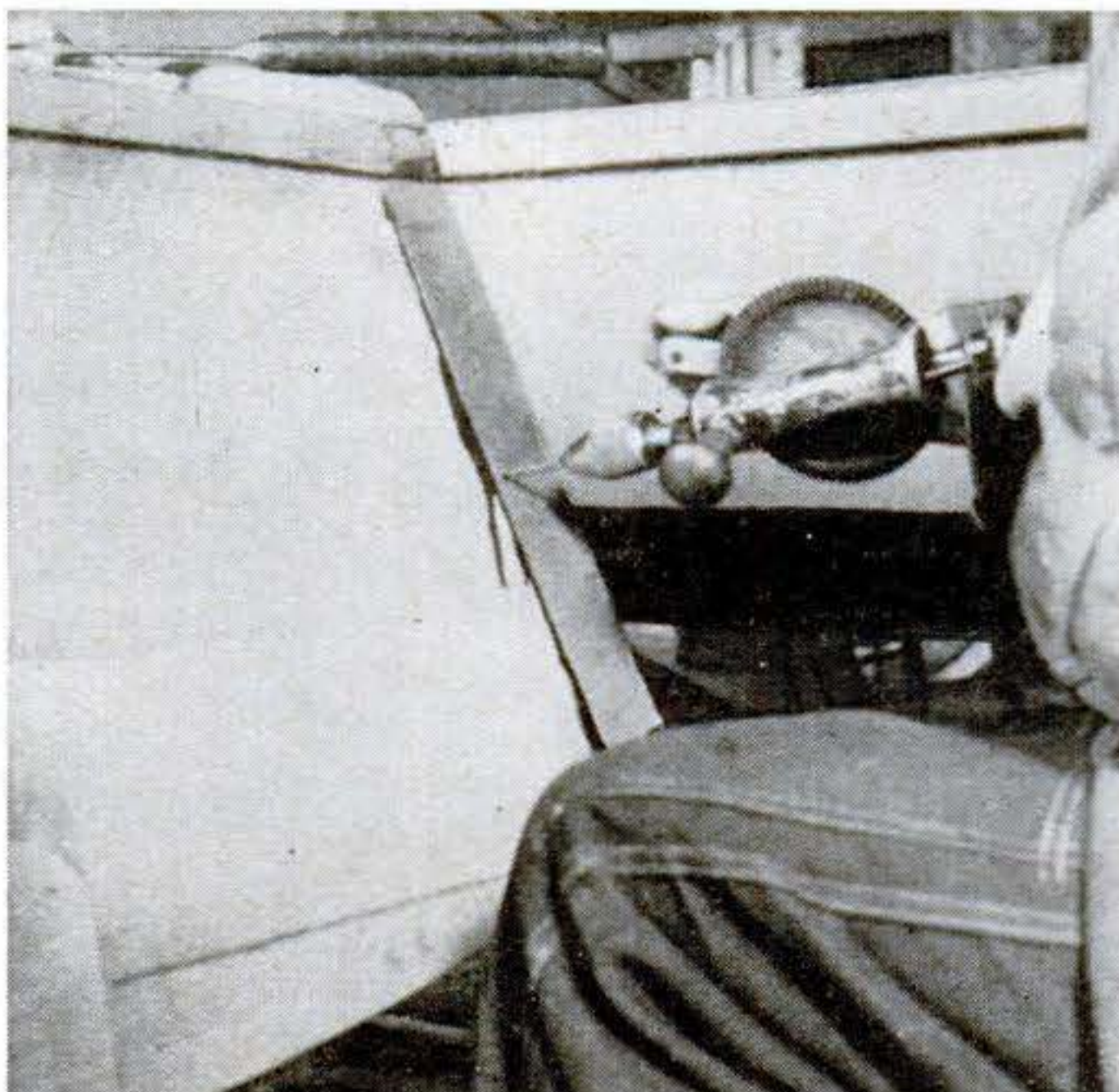
Final touch that's often overlooked is angled sheet copper on stern corners to protect them. Drill and fasten with copper nails.
