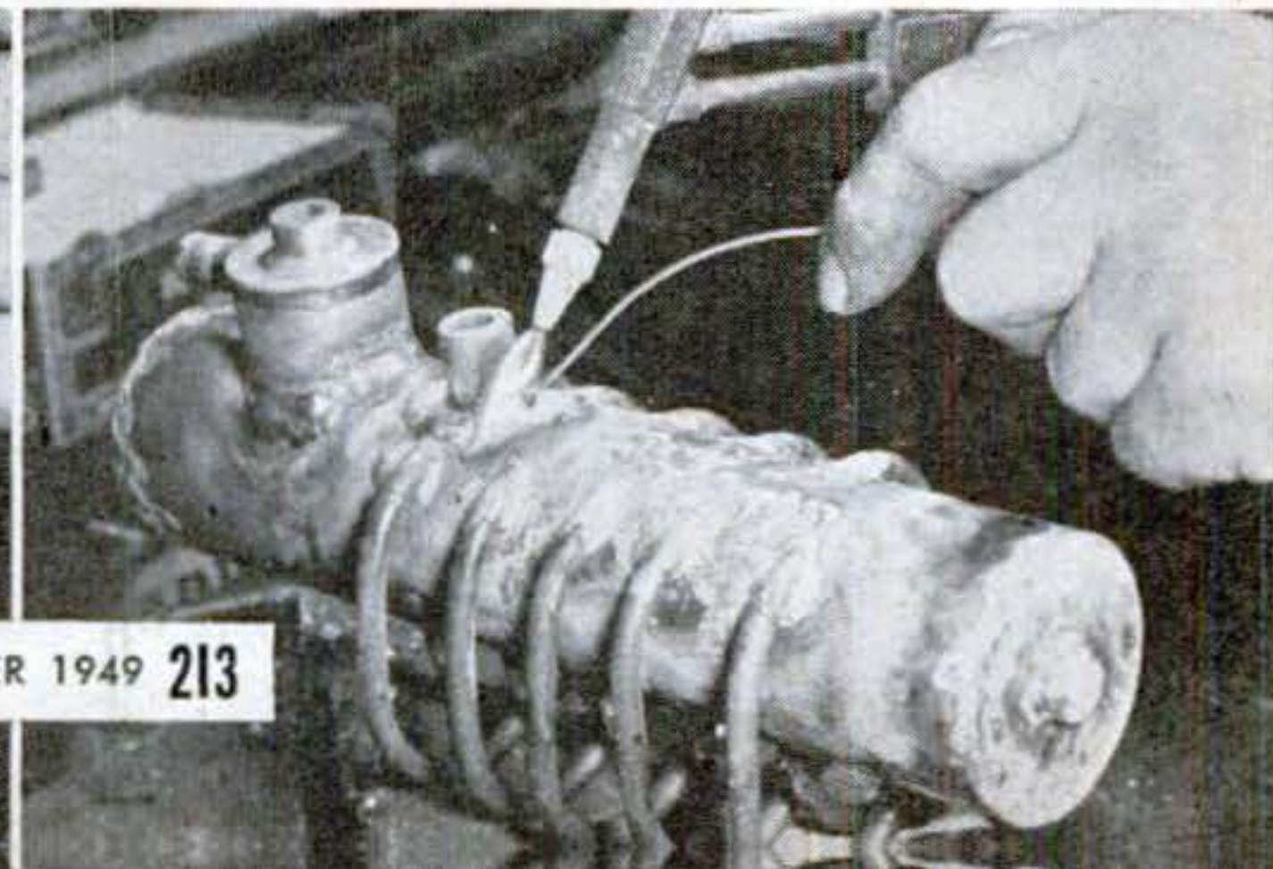
Dome, shaped saddle fashion to fit shell, is brazed over four holes. Filler nipple goes over large hole nearby. Silver solder used flows at 1,200°, and has ample strength. ➡
