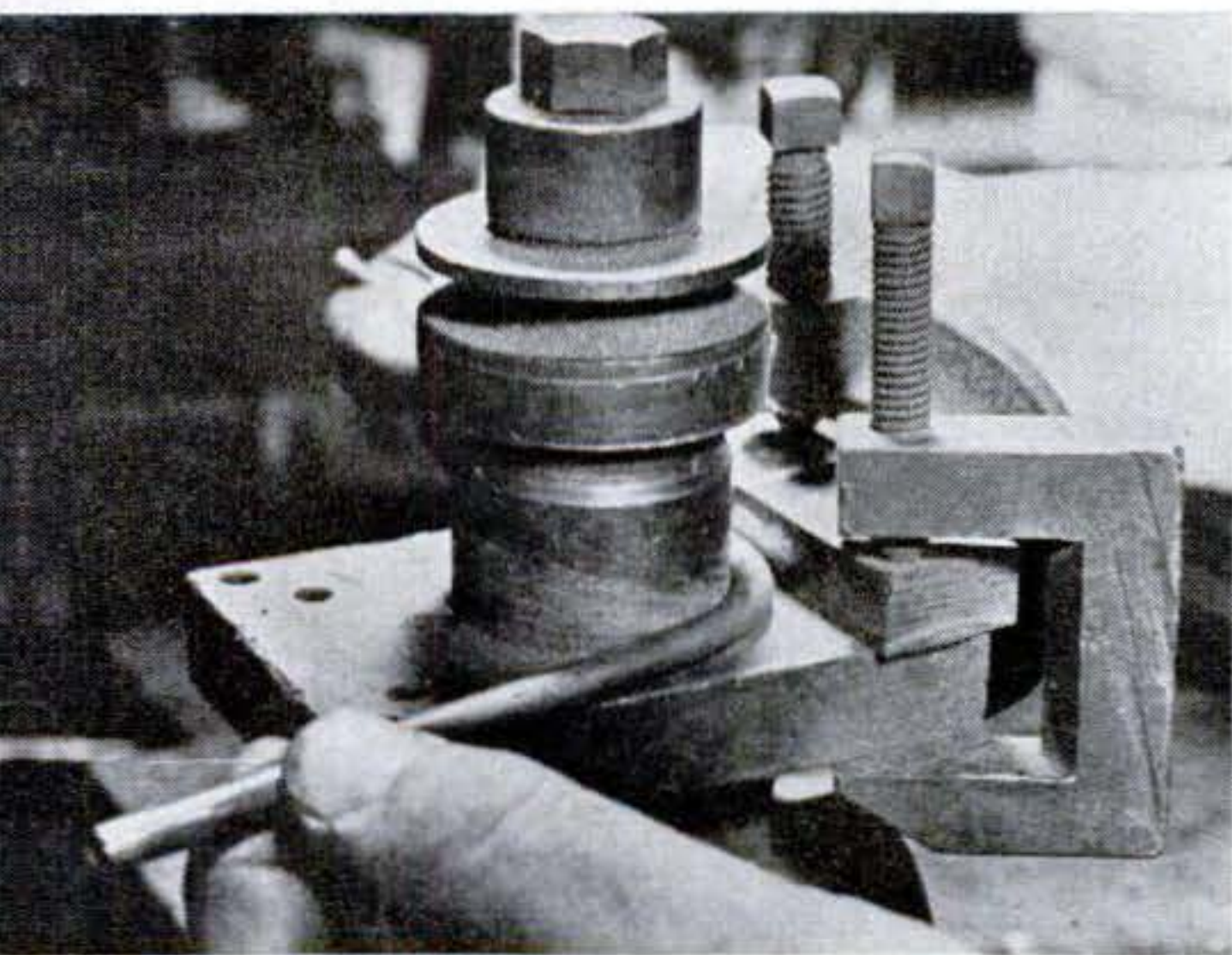
Pieces of copper tubing are bent to an open O shape on a jig. Correctly made, they have to be sprung into holes, which are cocked to suit by inserting rod, bending to position.
