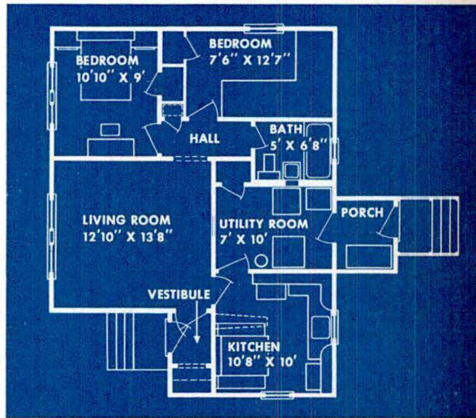
Floor plan above shows convenient layout of factory-built cabins. They are made in several sizes, with two to four bedrooms.
