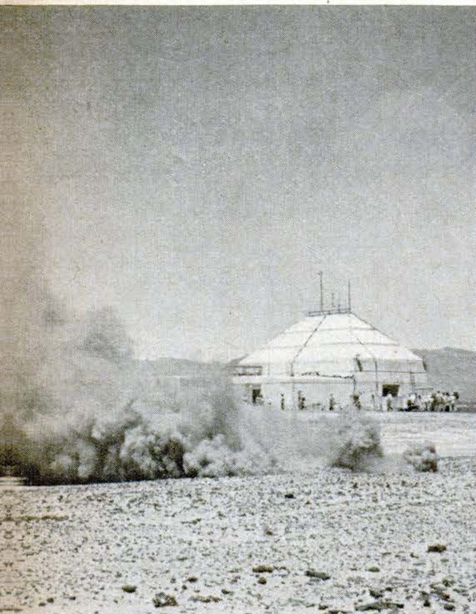
9 Fifteen minutes before launching, a red flare is shot off near the observation blockhouse, seen in the background, to alert trackers who do not have radio communication.
