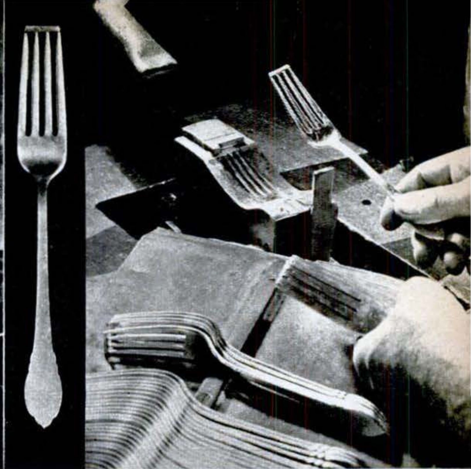
After blank has been rolled, stamped, and tined, swaging machine gives tines their graceful curves. A 600-lb. drop hammer containing male half of die forces the blank into lower, female die.
