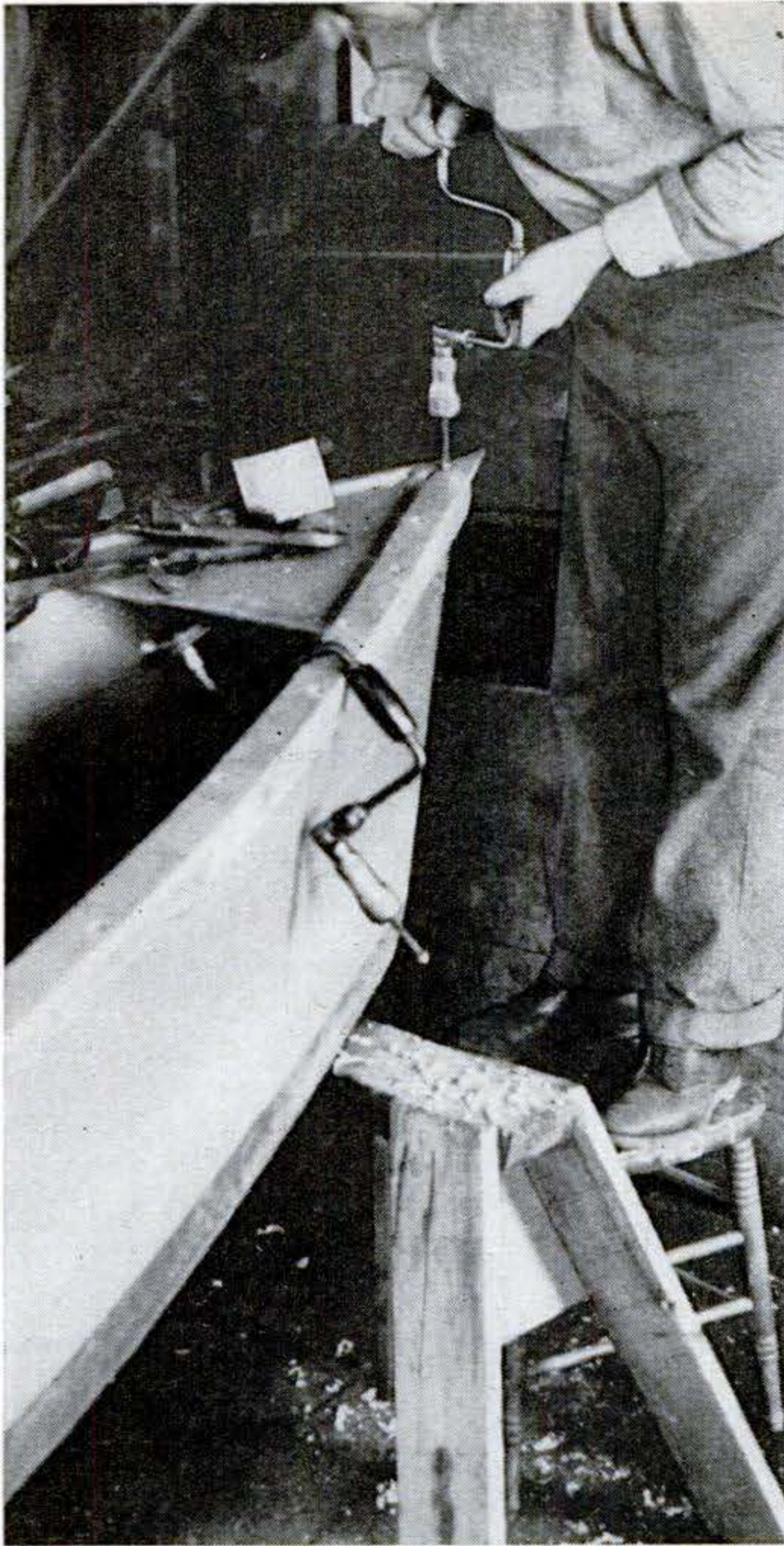
Battered top and guard rails are usually best replaced. Start at bow, bending and clamping hardwood strip in place as you drive screws.
