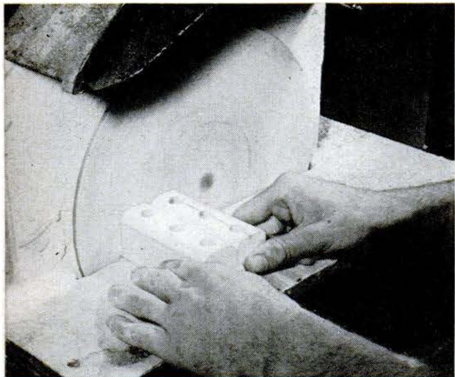
Locomotive boilers are smoothed down on disk sander. After this they are buffed to take off any sharp edges and then put under blower to remove wood dust from holes before painting.
