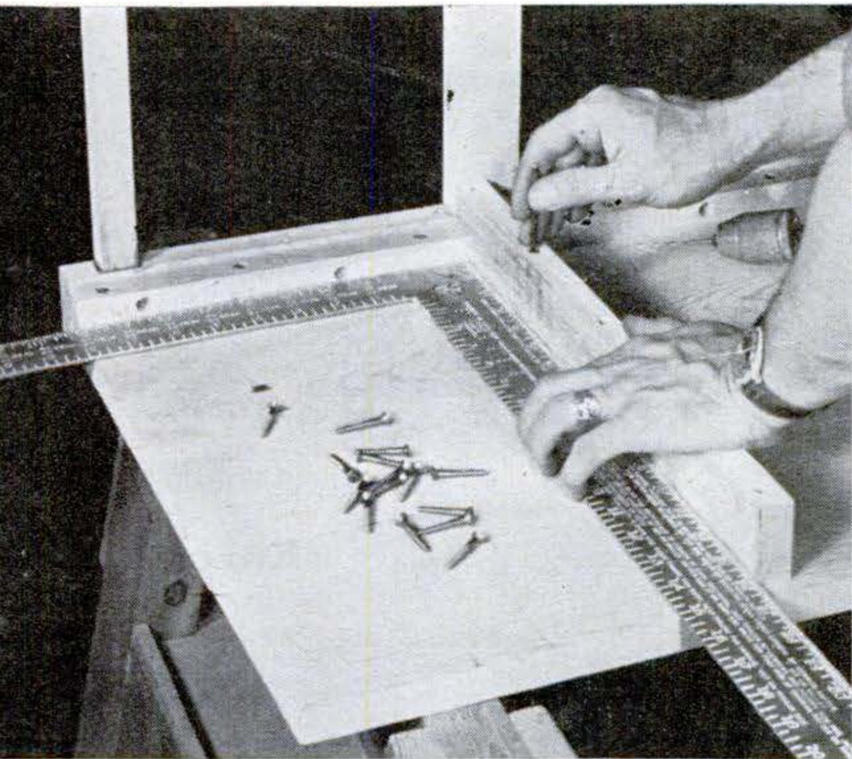
Drawer slides are screwed to sides of the cabinet. Here, a slide is squared up carefully before it is attached with countersunk screws.
