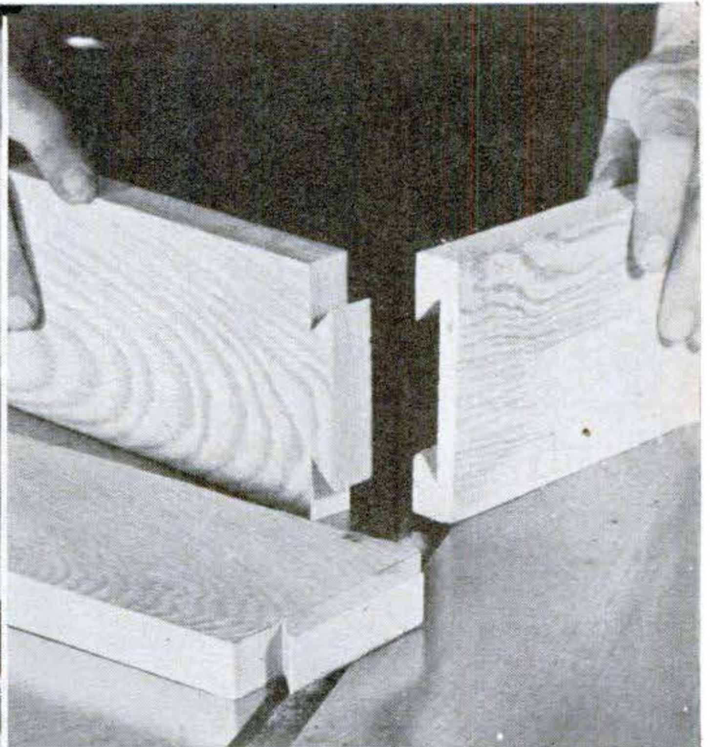
Front and sides of base are assembled with lap-dovetail joints. Rear of base is screwed into notches cut in the base sidepieces.
