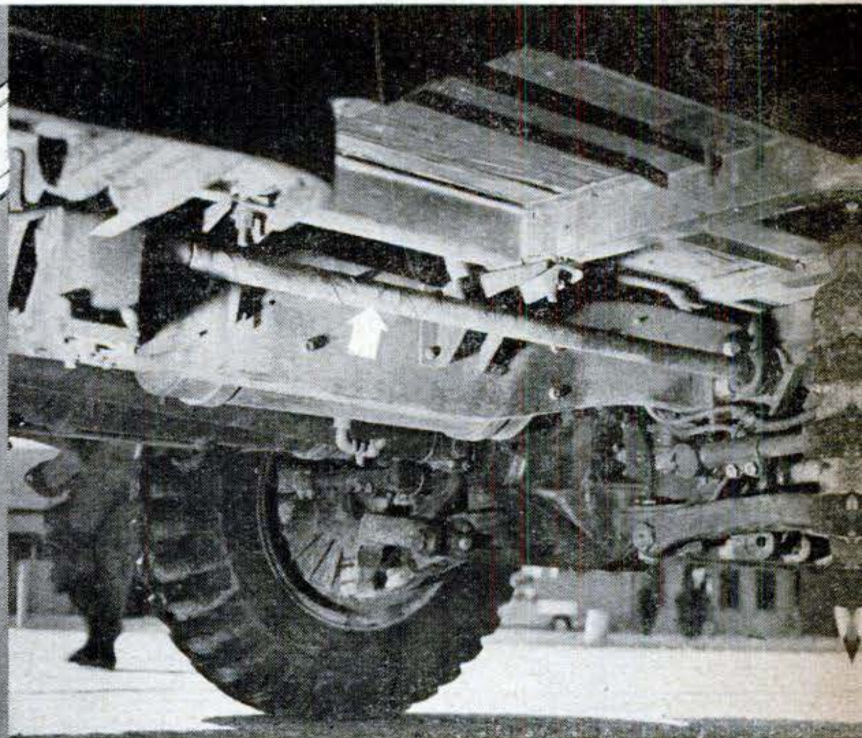
New ¾-ton cross-country truck has 187-hp. air-cooled engine, hits 60 m.p.h. on good road.
