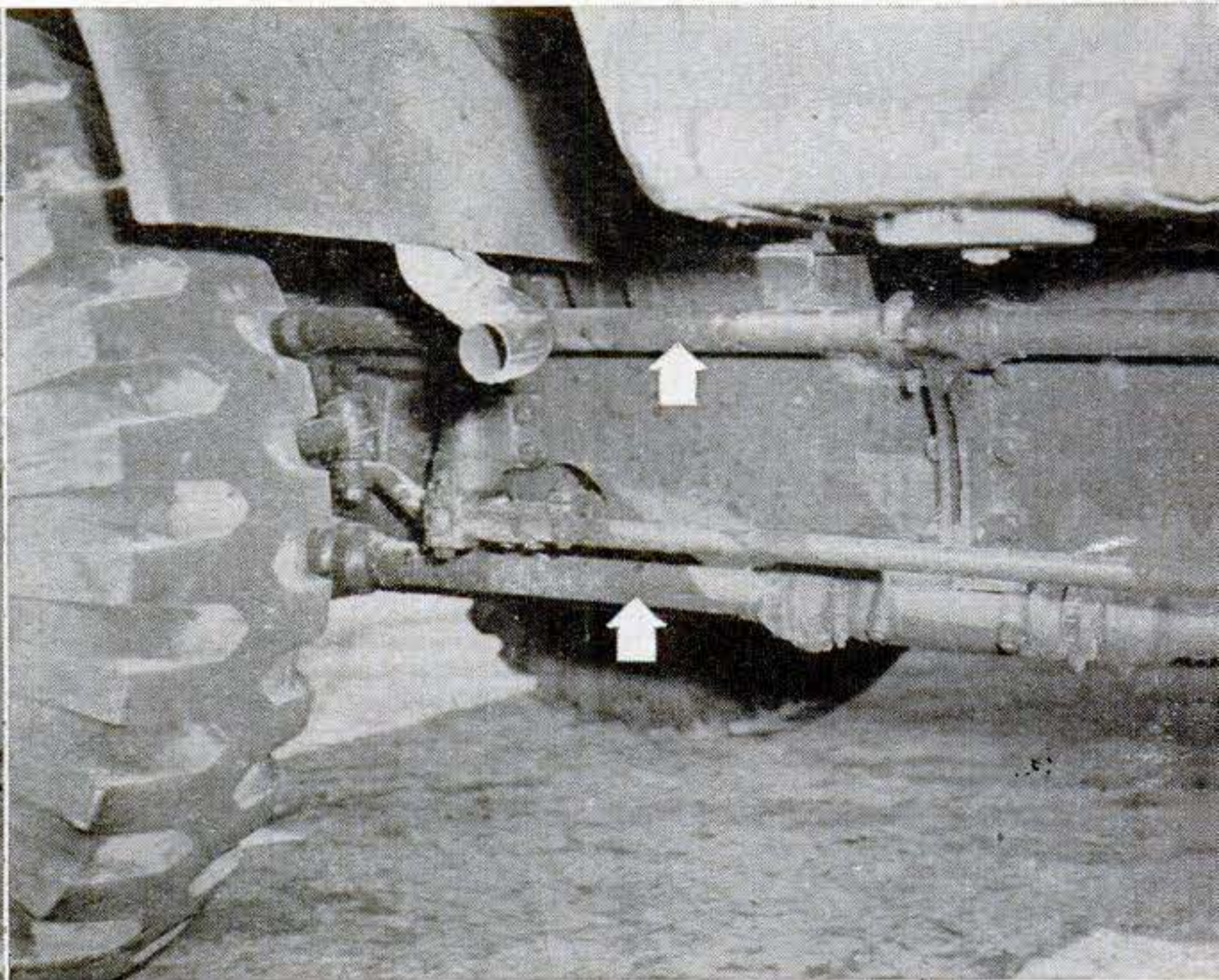
Close-up shows torsion-bar suspension (arrows) on the 5-ton truck. Twisting action of top bar takes care of ordinary road shocks. Bottom bar does same job as conventional overload springs.
