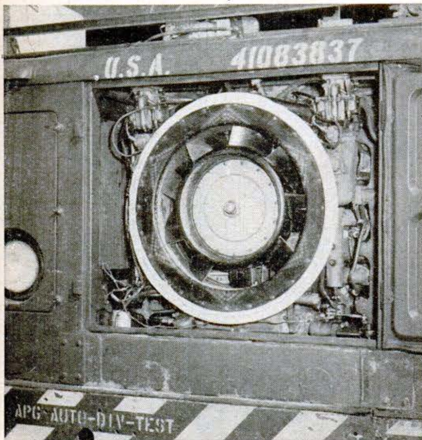
A huge cooling fan replaces the conventional radiator. The engine has eight opposed cylinders and is mounted on end with a vertical crankshaft. It develops 200 horsepower.
