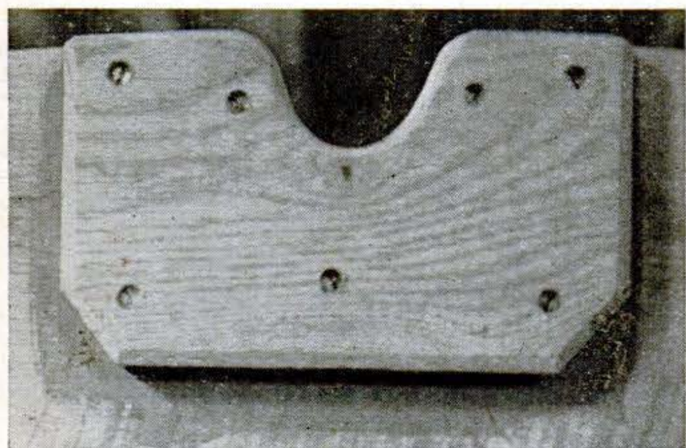
A reinforcement like this at the scull notch will save the transom from wear. Maintaining notch shape also makes sculling easier.
