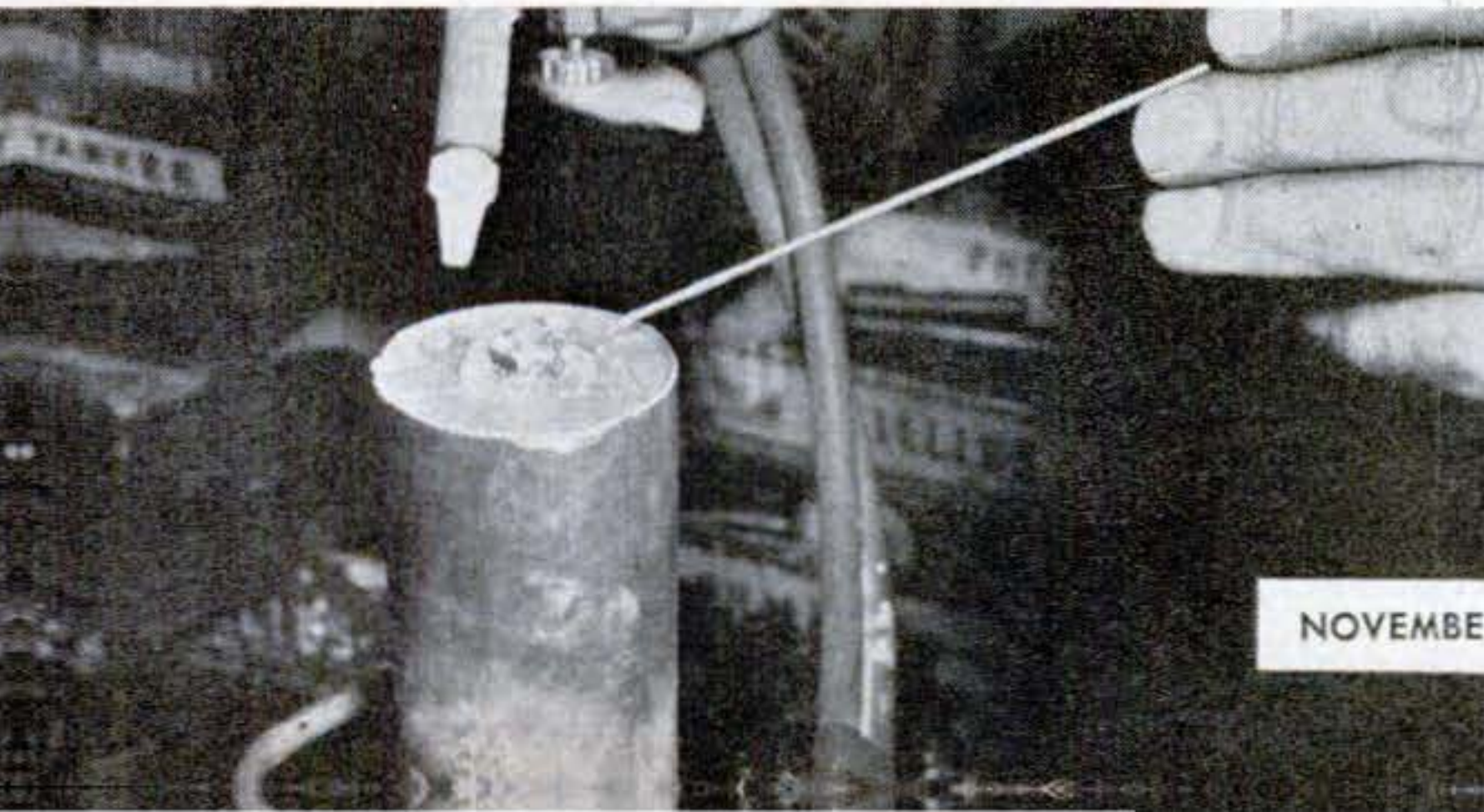
Nut is screwed on each end of stay. Then disk is silver-soldered to shell all around. Both nuts are sealed with silver solder all around and on top to prevent leakage.
