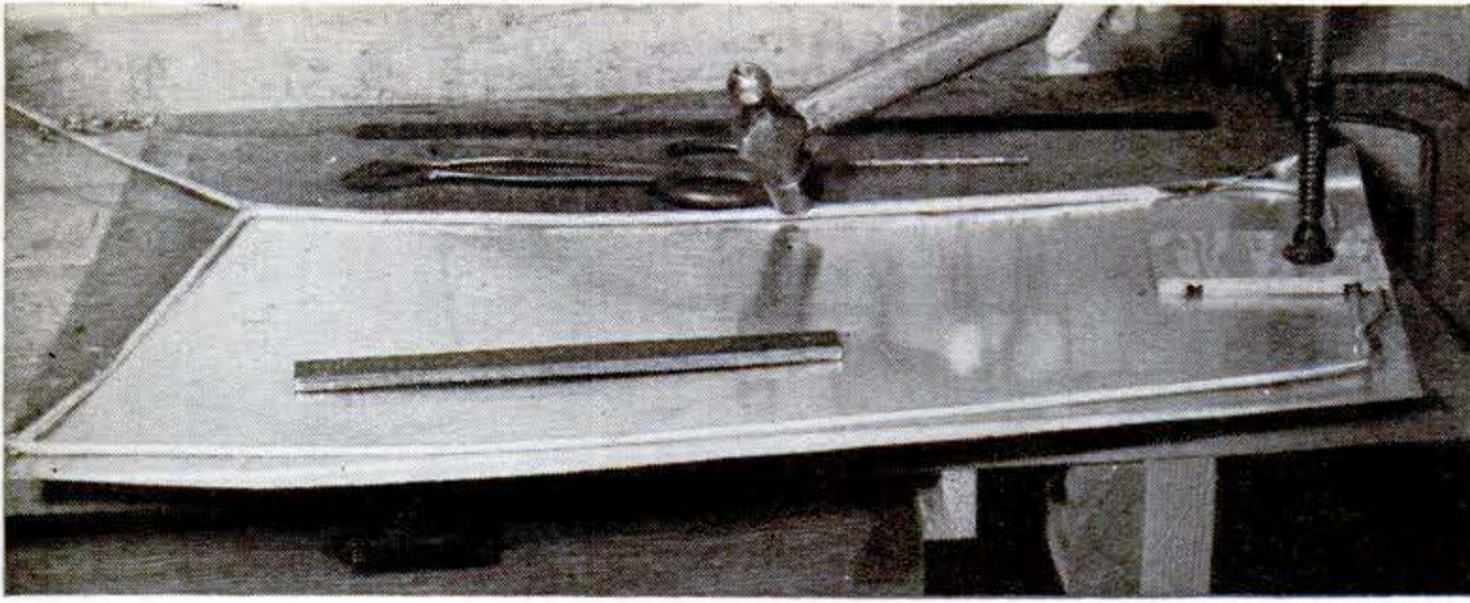
Aluminum rolls easily over the \frac{1}{4} " rod frame. Pound it down as shown here and then smooth the rolled inner edge with an iron bar like the one in foreground. Notice side bracket on the rod at the right.
