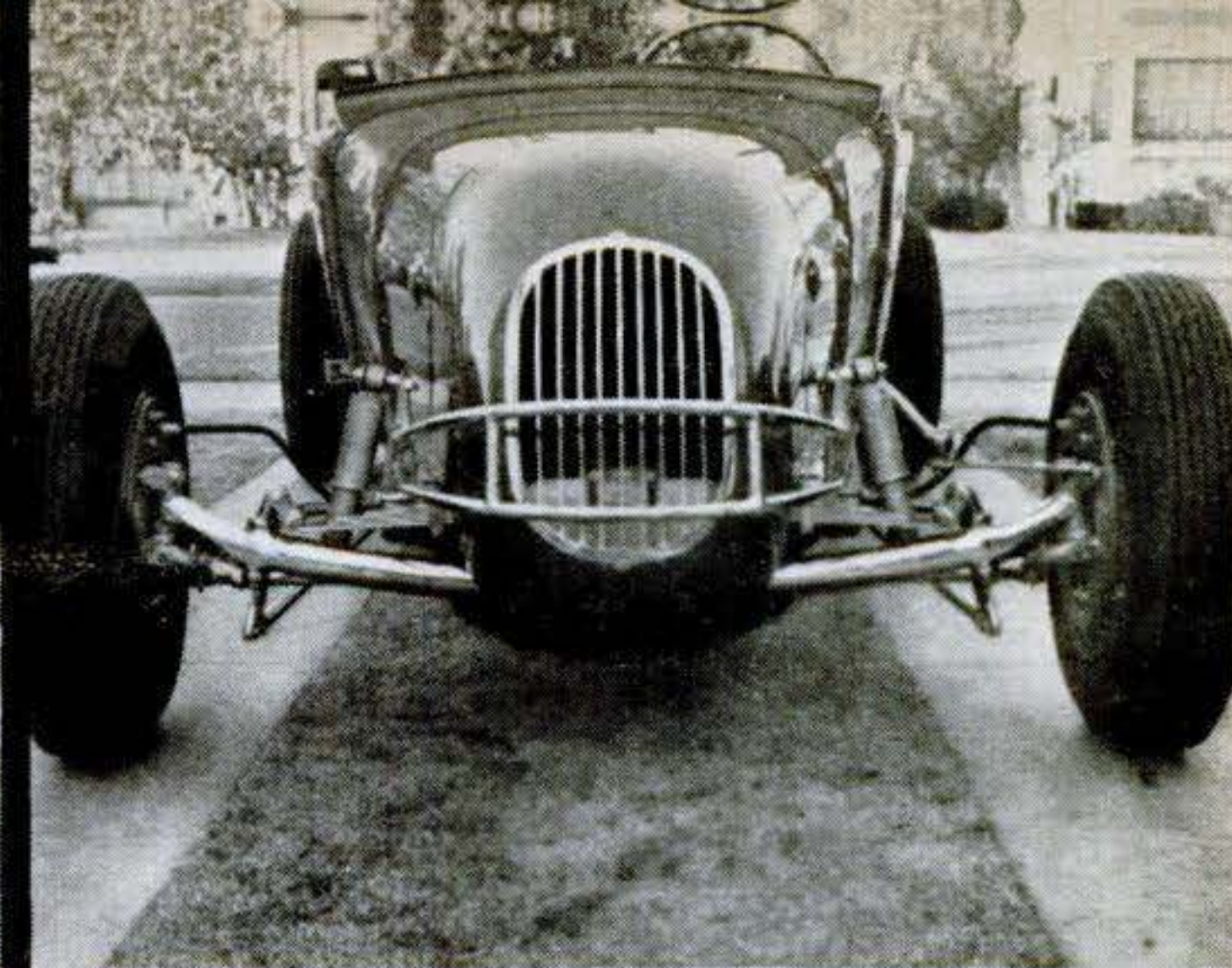
Aluminum cowl and hood , together with grille, were handmade. The front axle is from a '39 Ford, but has been fitted with earlier-model spring perches. Brakes are '41 Ford hydraulics.
