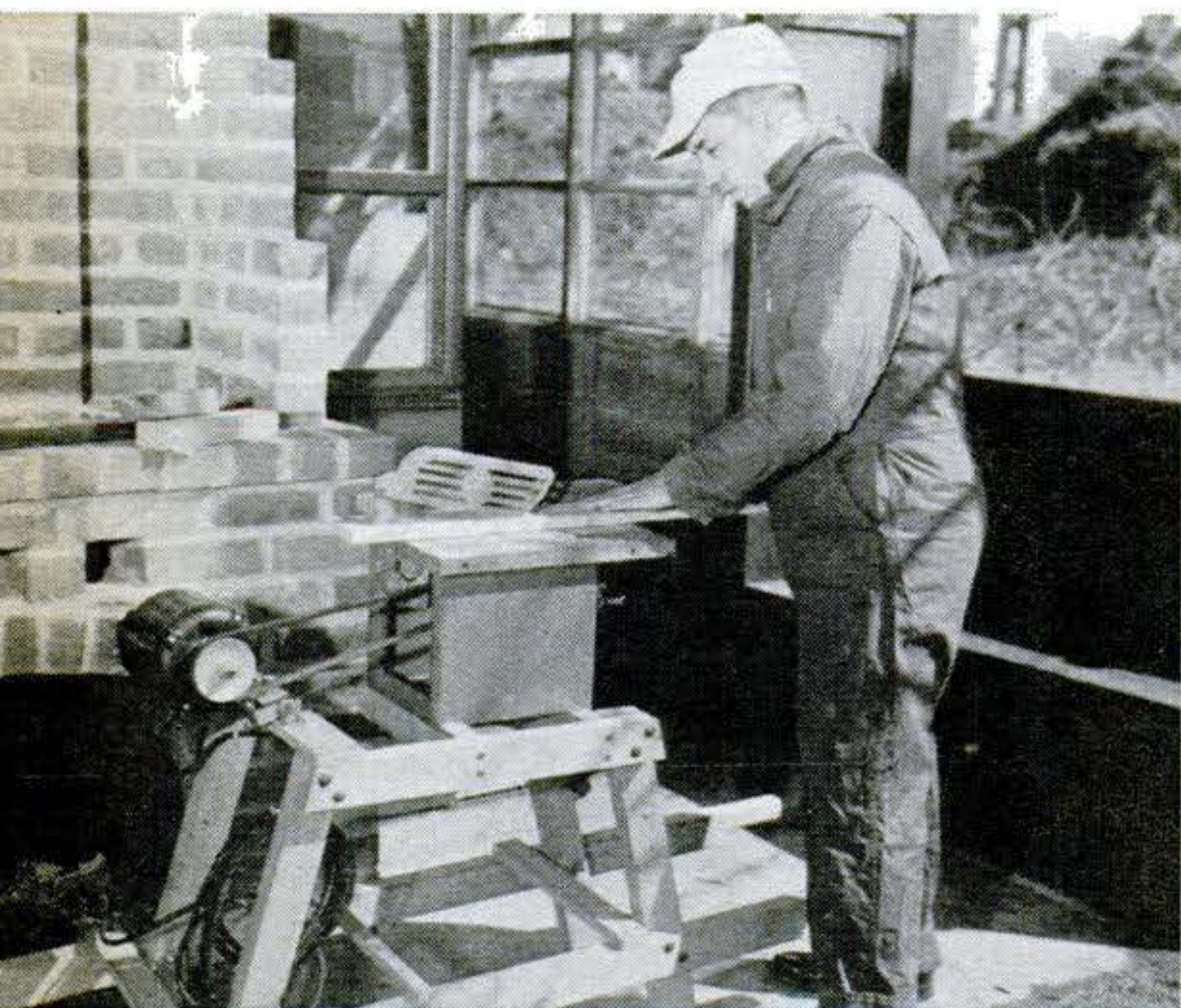
Saw in use. Even on hard surface like concrete walk, both units are heavy enough, and have legs spaced sufficiently, to be completely stable.
