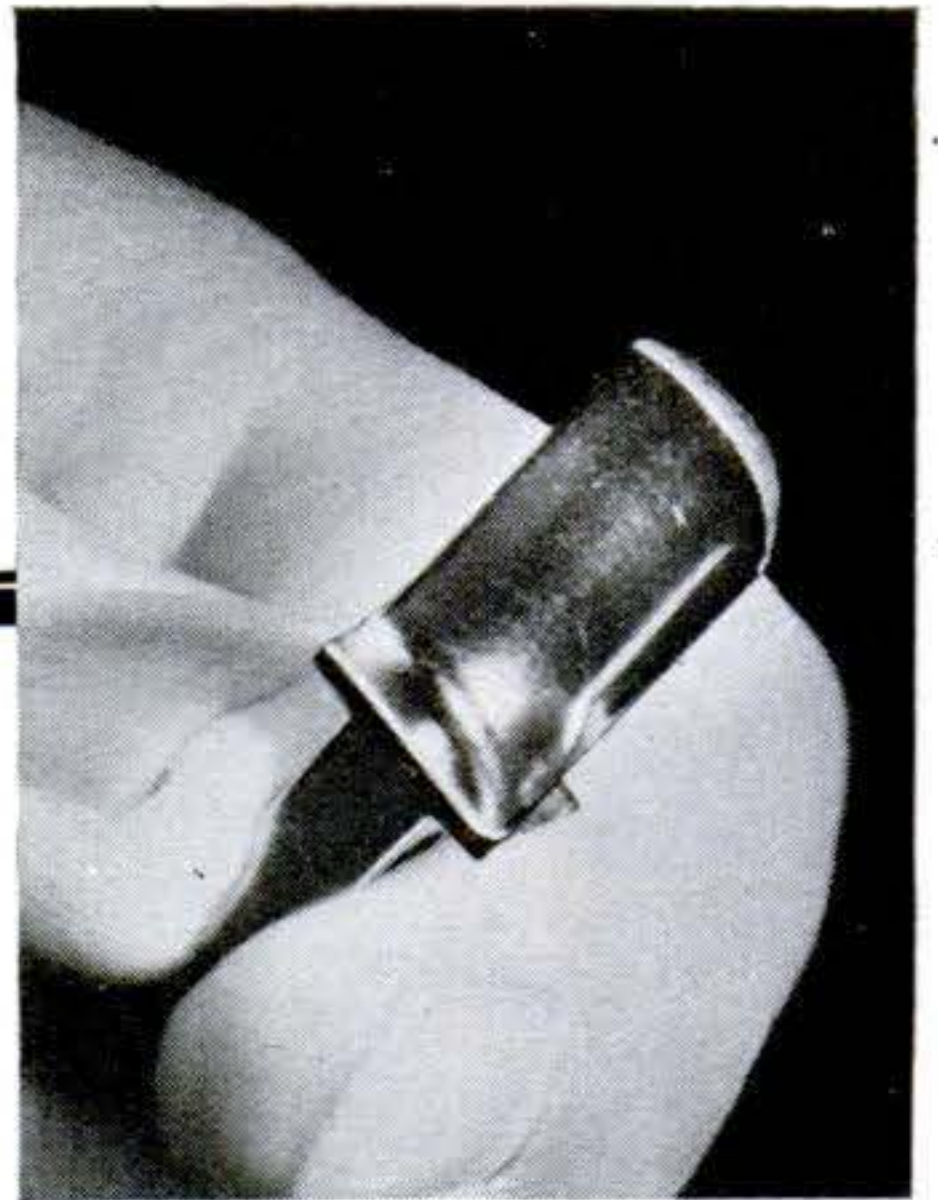
Sixty of these tiny blades are on perimeter of both compressor and power turbines of Rover engine. Made of "Ni-monic" nickel alloy steel, they must withstand constant gas blast of 1,500° F. Due to high speed, balance is big problem in turbines. Engine idles at 7,000 r.p.m., turns at 36,000 at car speed of 90 m.p.h.
