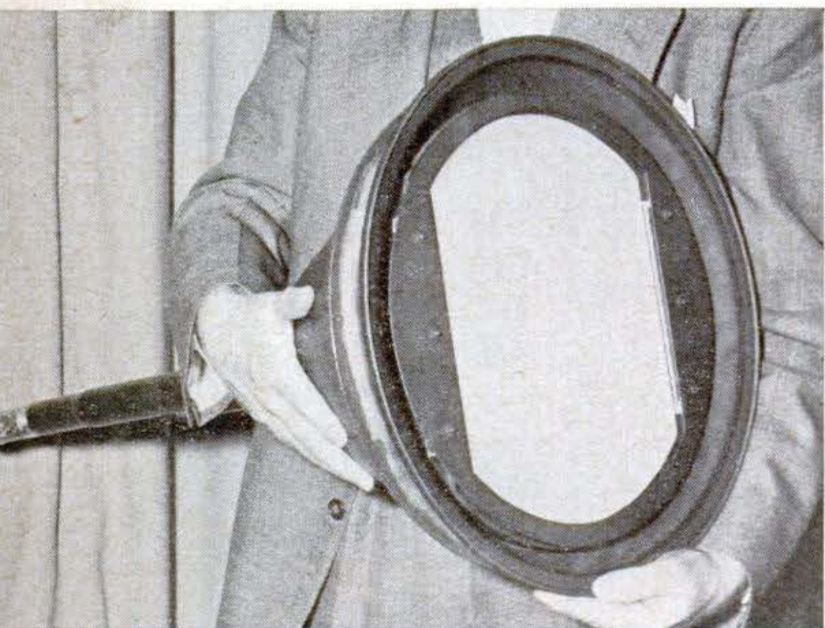
The one-gun, tri-color tube looks like this. RCA engineers are working on improved models, with more dots. Tube can be used in some standard receivers, but needs extra circuits.
