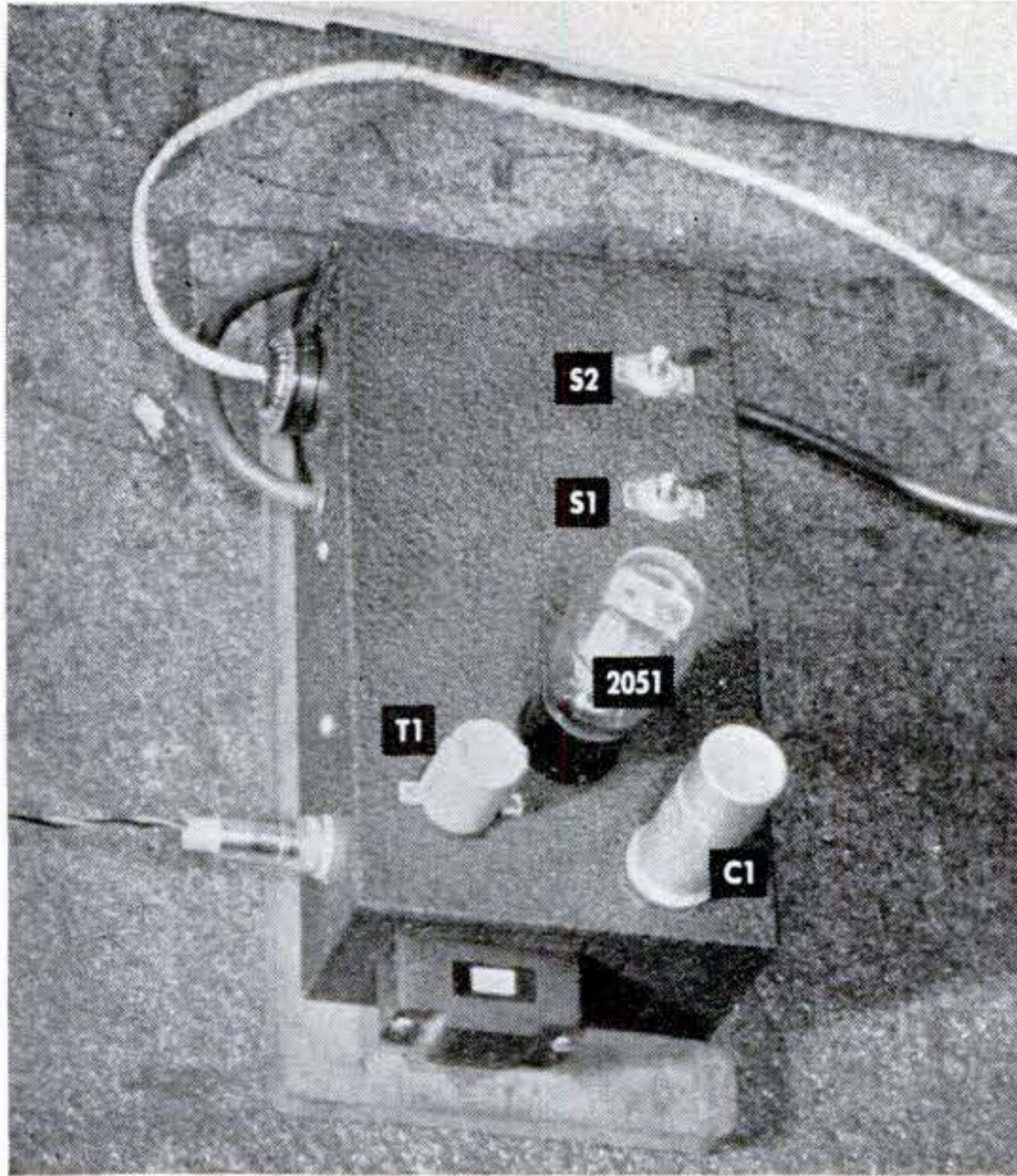
The wooden board on which the chassis rests can be screwed to a wall. The oversized chassis insures ample ventilation in tight quarters.
