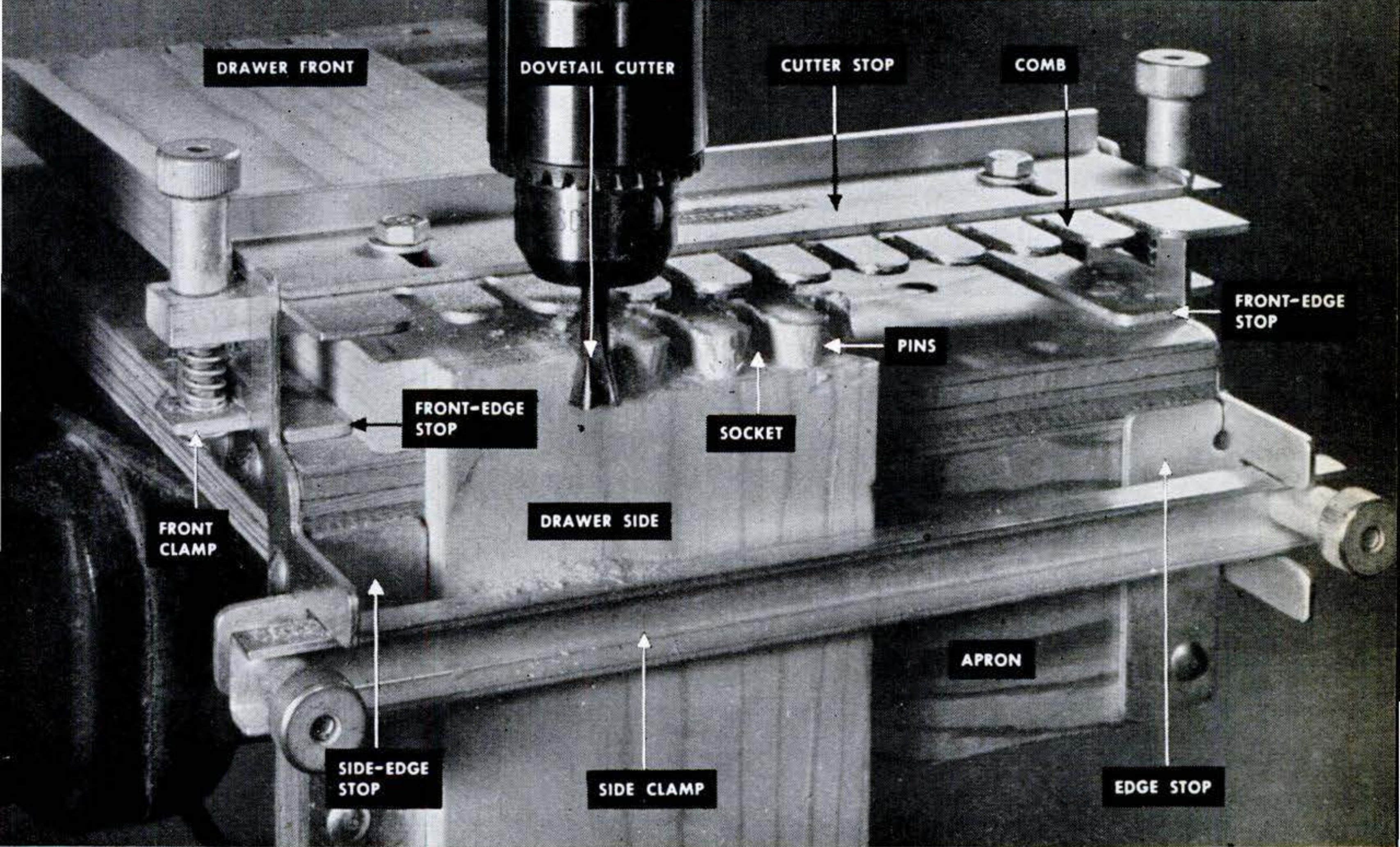
Ends of pins are undercut and rounded same as sockets. When side is flipped over, the angles match up.
