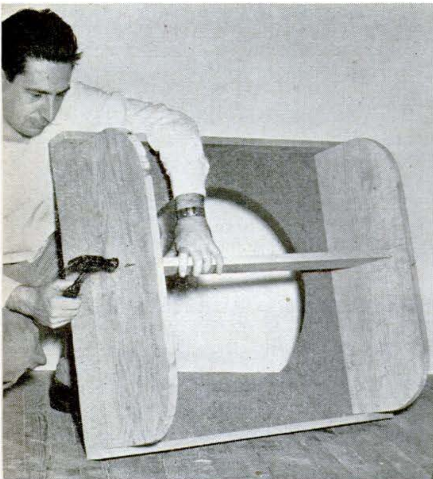
You can make a window ventilator from some lumber, a fan and arbor, a motor, and a few square feet of metal grille. Frame is made of 1" lumber; back, from composition board.
