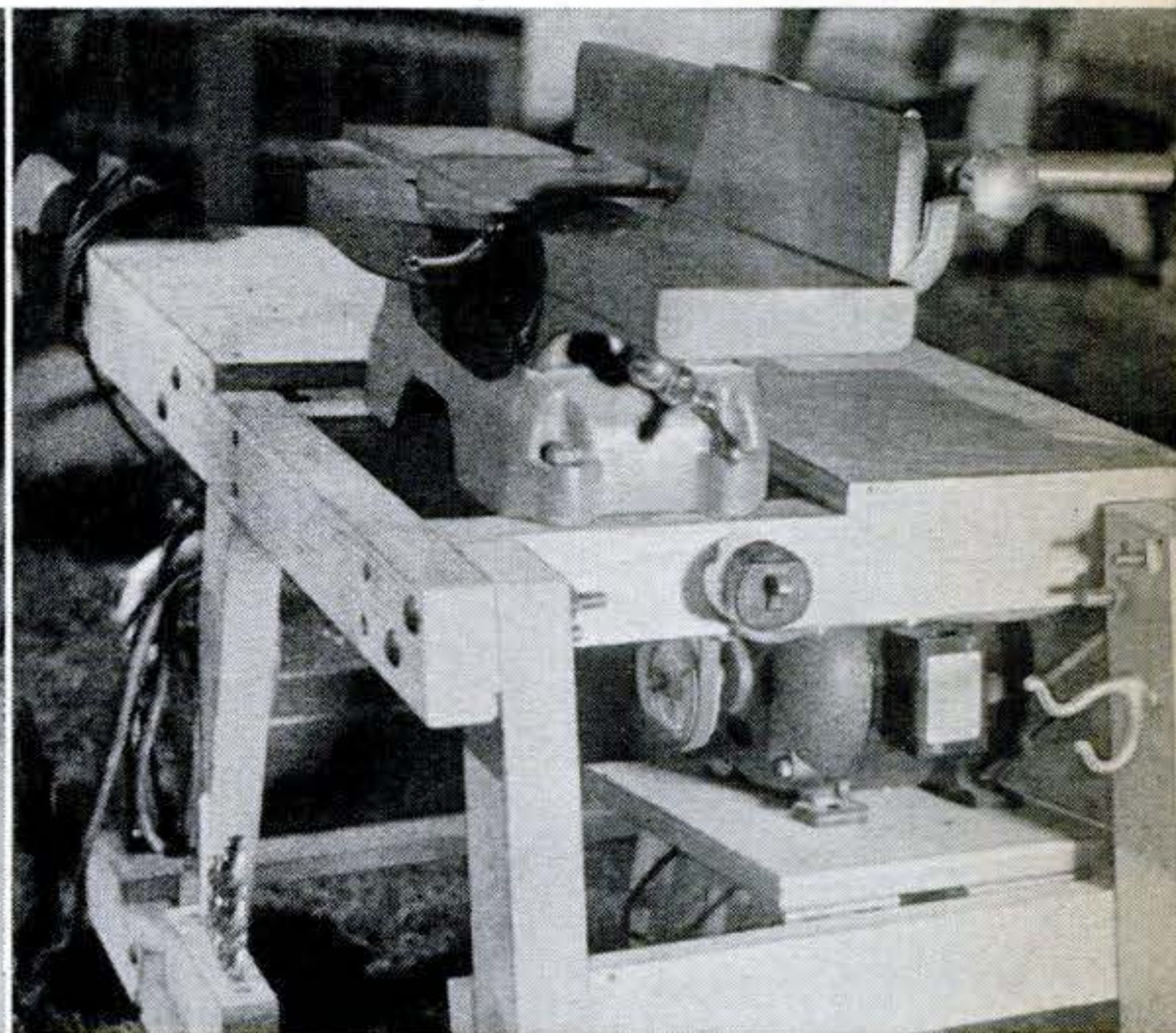
Motor of jointercart is bolted to ¾" plywood base that's hinged to crosspiece. Motor is offset for balance. Hook is for extension cord.
