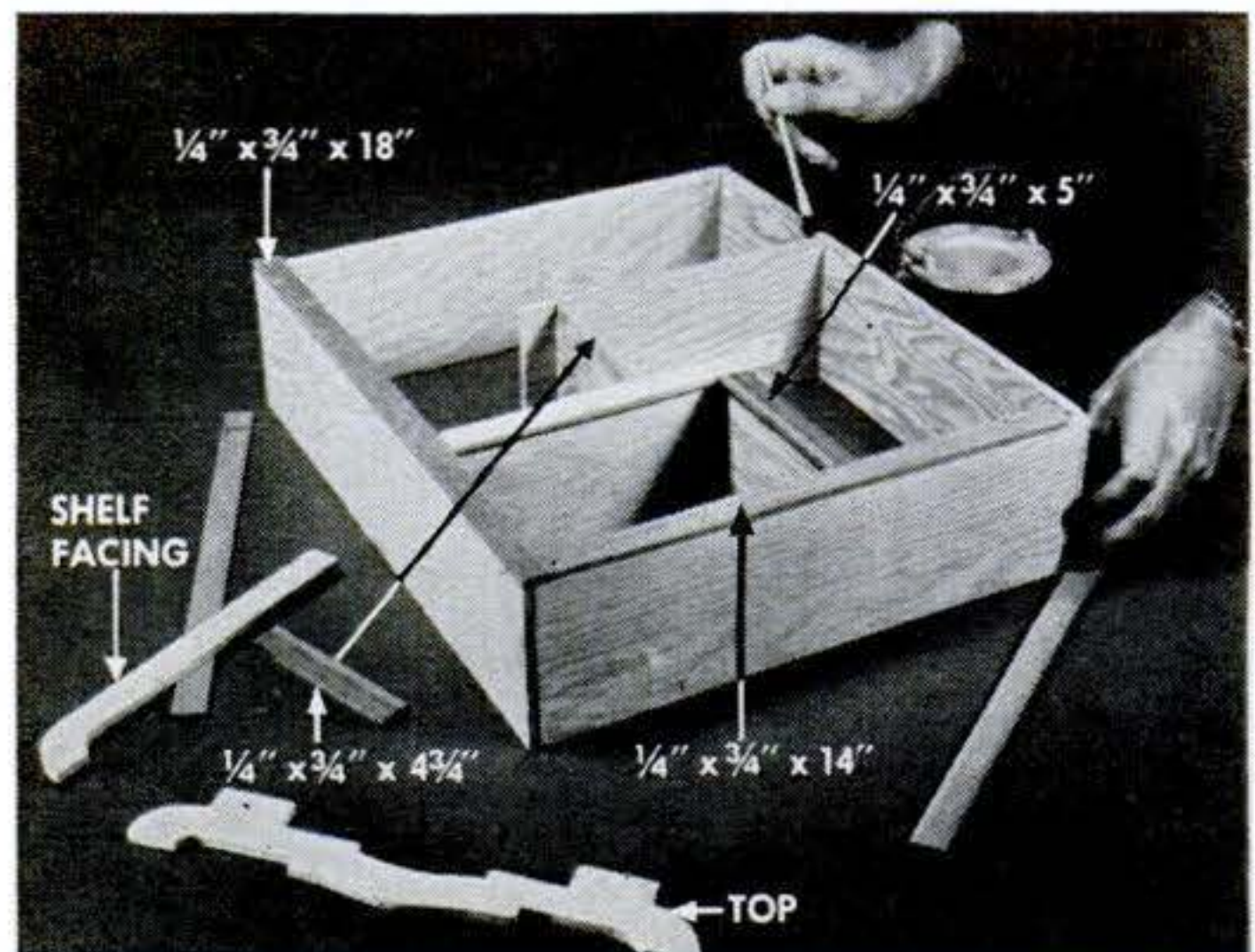
Glue is applied to the front edges of the shelves, the shelf supports, and the four sides. The framing pieces are then clamped in place.
