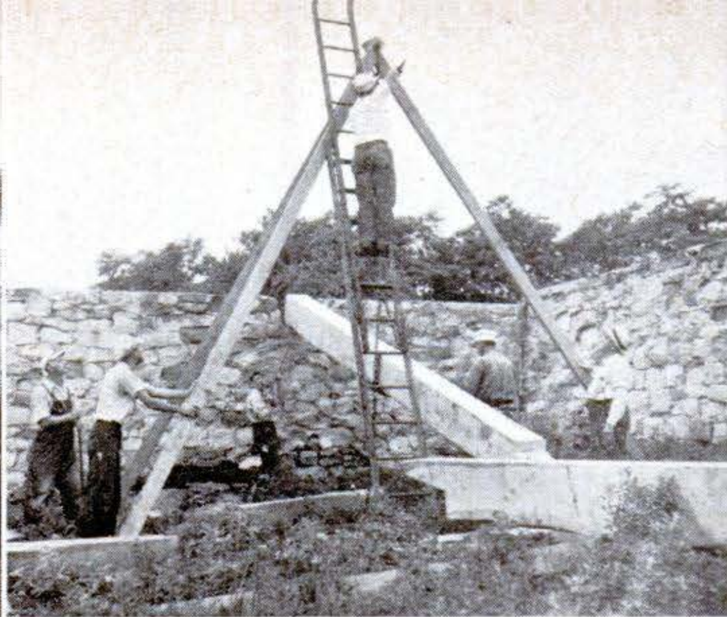
Carpenters use block and tackle to lift joists into place. These run the length of the barn, and are set into the stone foundation. Supporting posts are set in concrete on barn's floor.
