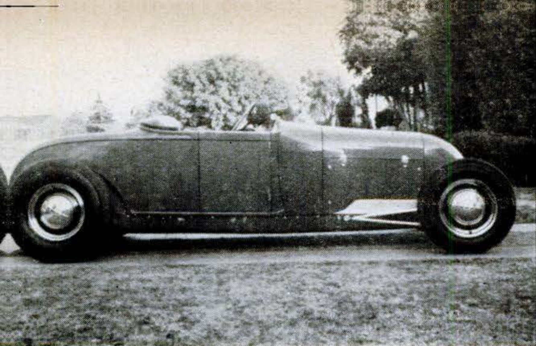
Roadster has '39 Ford rear end, with torque tube shortened 18½ in. Drive shaft is Model A. New wheelbase is 110 in. Frame rails are from '27 Essex, fitted with Model-A rear crossmember.
