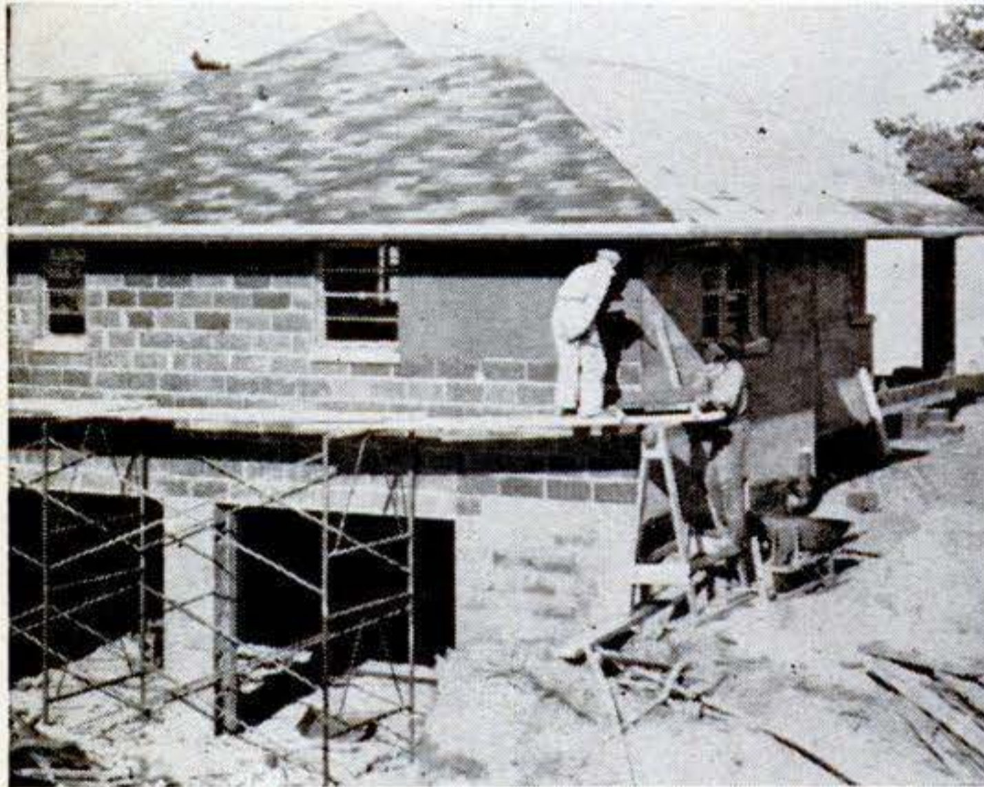
To waterproof walls, plastic cement was used inside and out. Then outside walls were finished with coating of red stucco cement.
