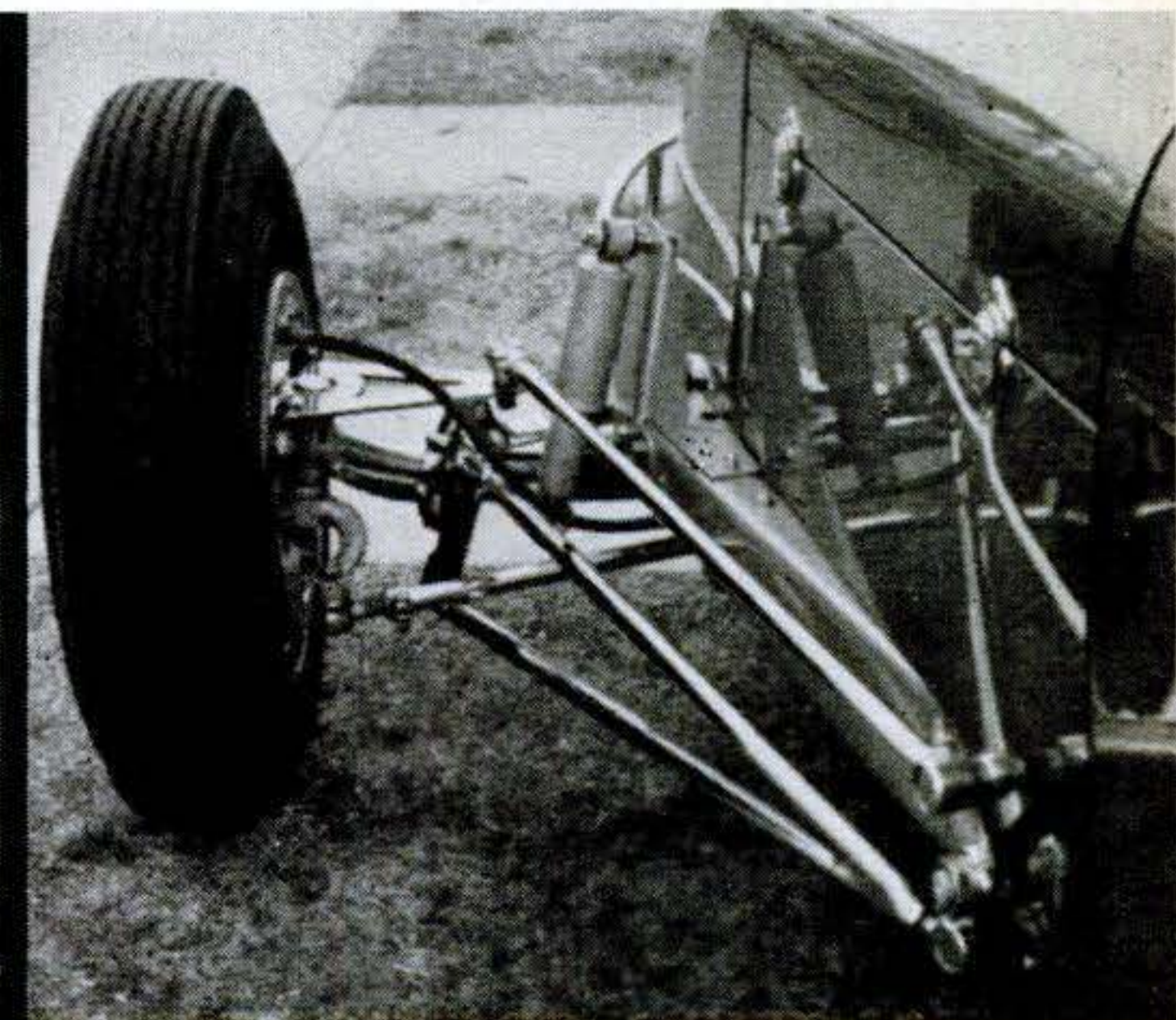
Unusual steering mechanism is '35 Ford cross-steering assembly turned on side, racer style, for ground clearance. Rear axle has teardrop fairings built around it to cut air resistance.
