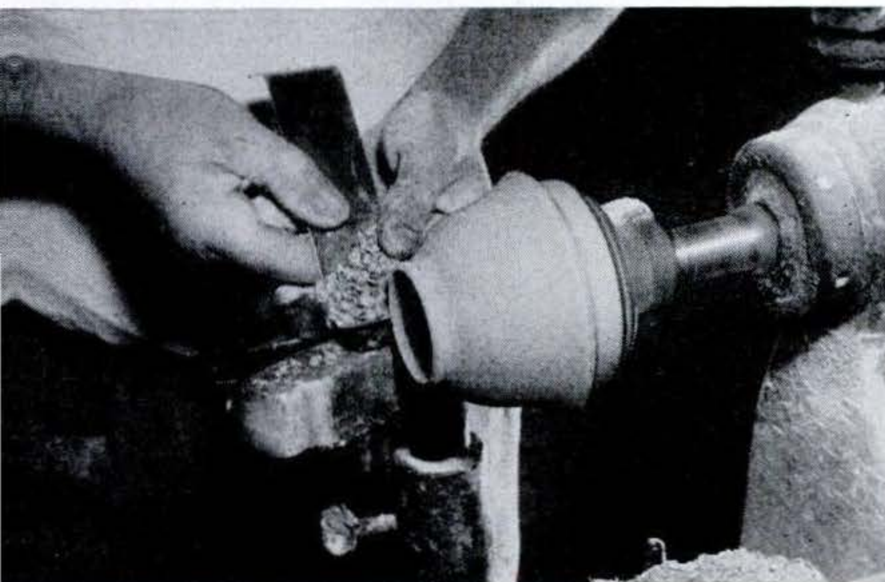
8 Cups are jiggered out in much the same way as plates. However, they must be finished on lathes. Because the body mixture contains flint, tools must be sharpened frequently.
