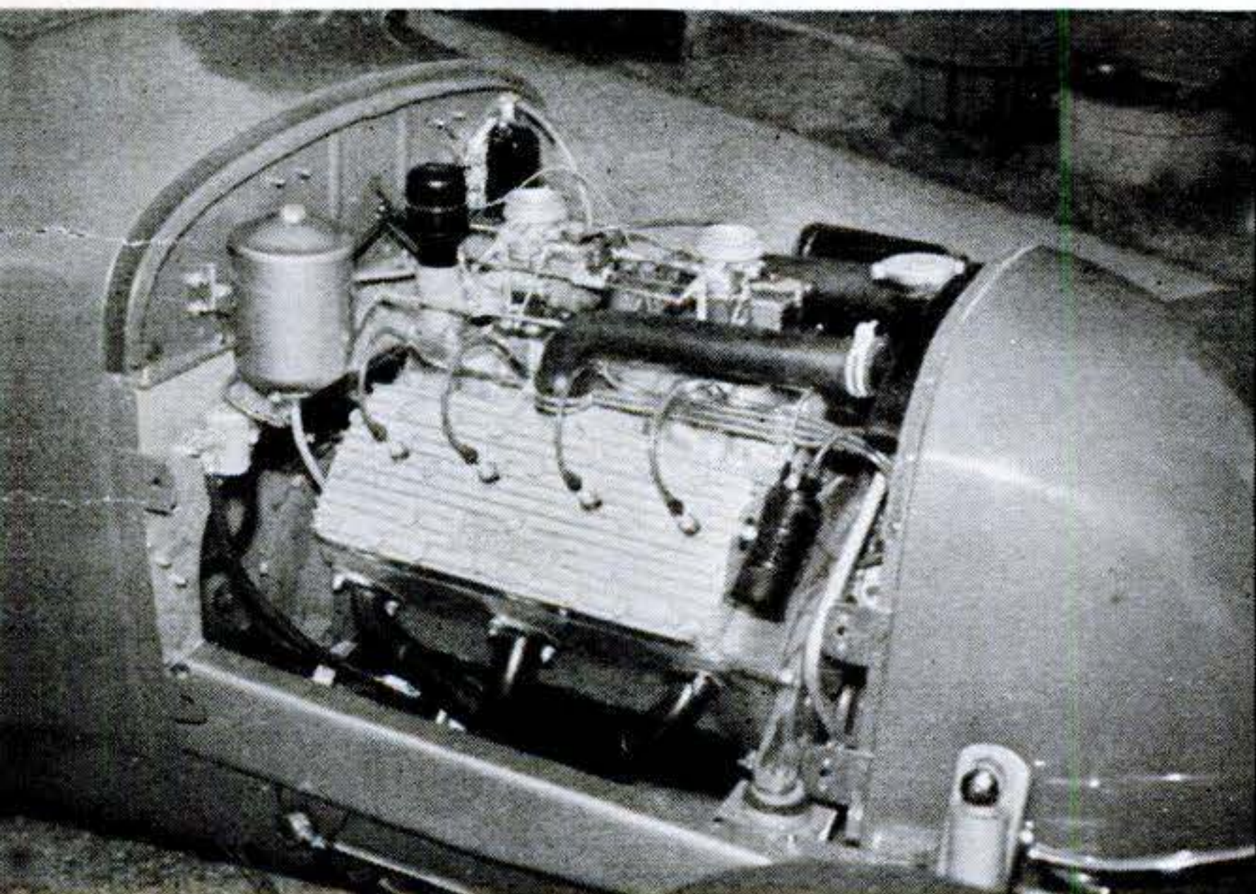
Speedy engine is '42 V-8 Mercury, of stock bore and stroke, with Evans heads, Weiand manifold, Kurten ignition, and Thompson 3-ring pistons. Rear support is Model-A crossmember.
