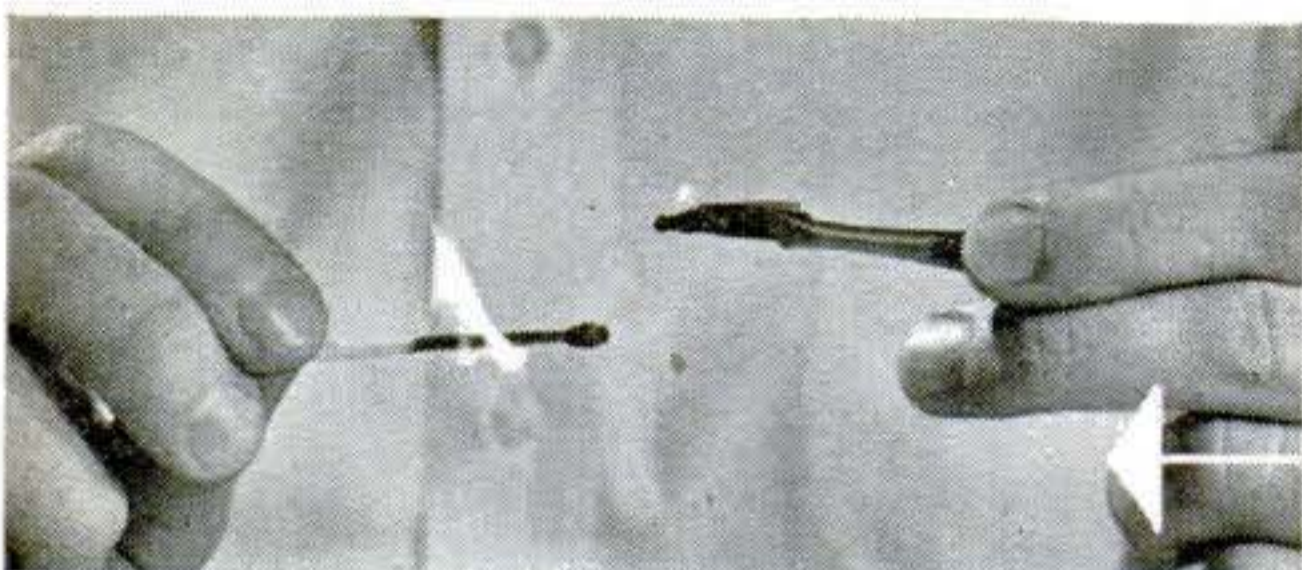
Sample burns but goes out when removed from flame. Return it just to edge of flame and note color characteristics it imparts.
