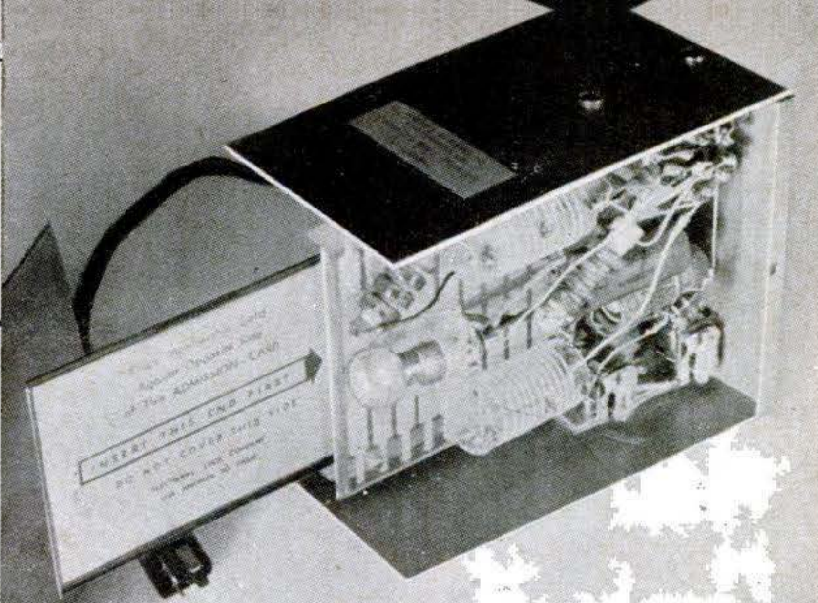
"Radar Lock" is mounted in steel box that fits inside house wall. It uses one twin-triode "peanut" vacuum tube, which is always kept warmed up. Snap-action switch turns on full power for tube when key card is inserted. Small bulb merely illuminates the key slot.
