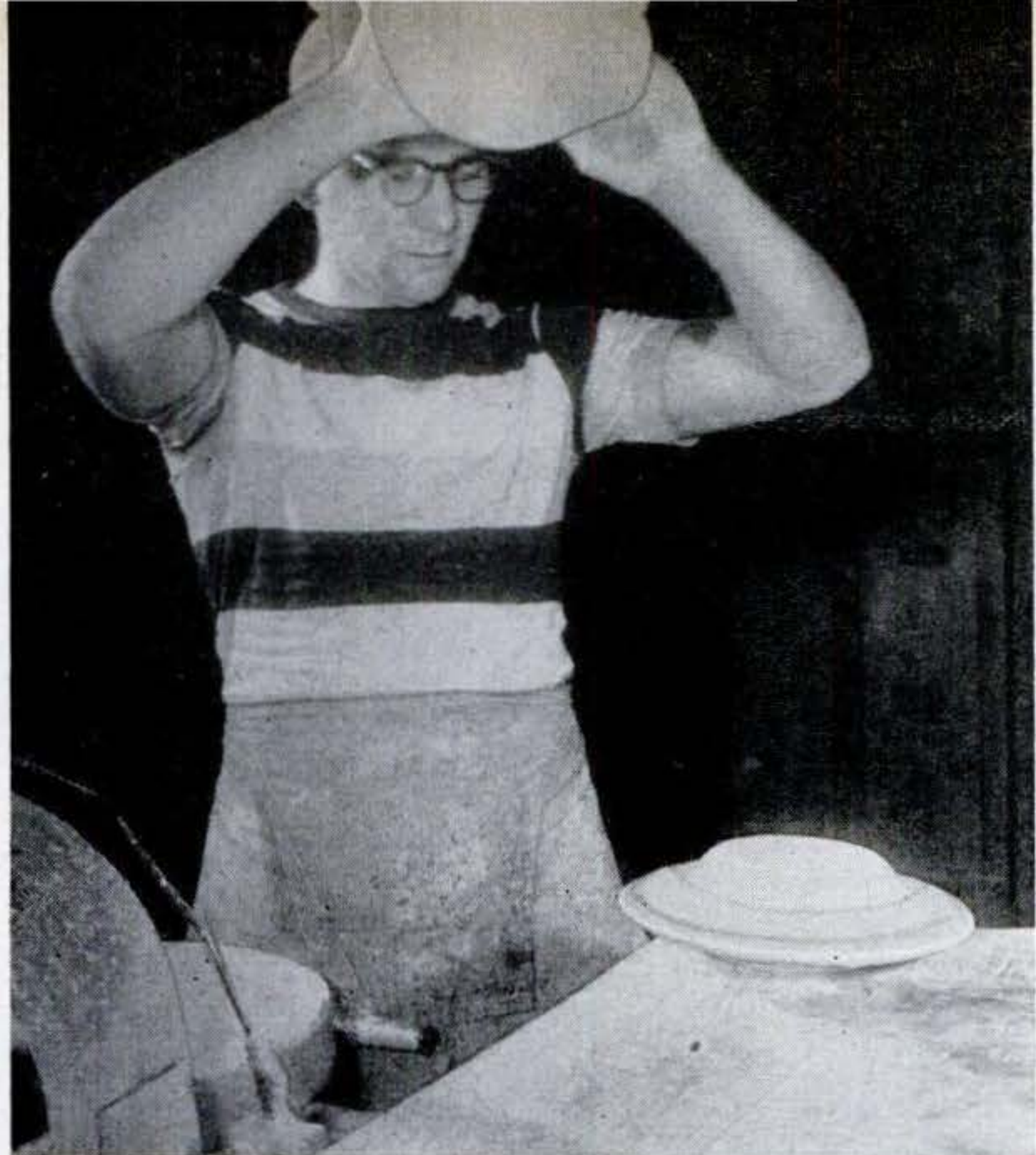
5 Batting out. This is first step in the actual making of a cup or a plate. A lump of body mixture is placed in the machine visible in lower left-hand corner of photo above, and pressed
