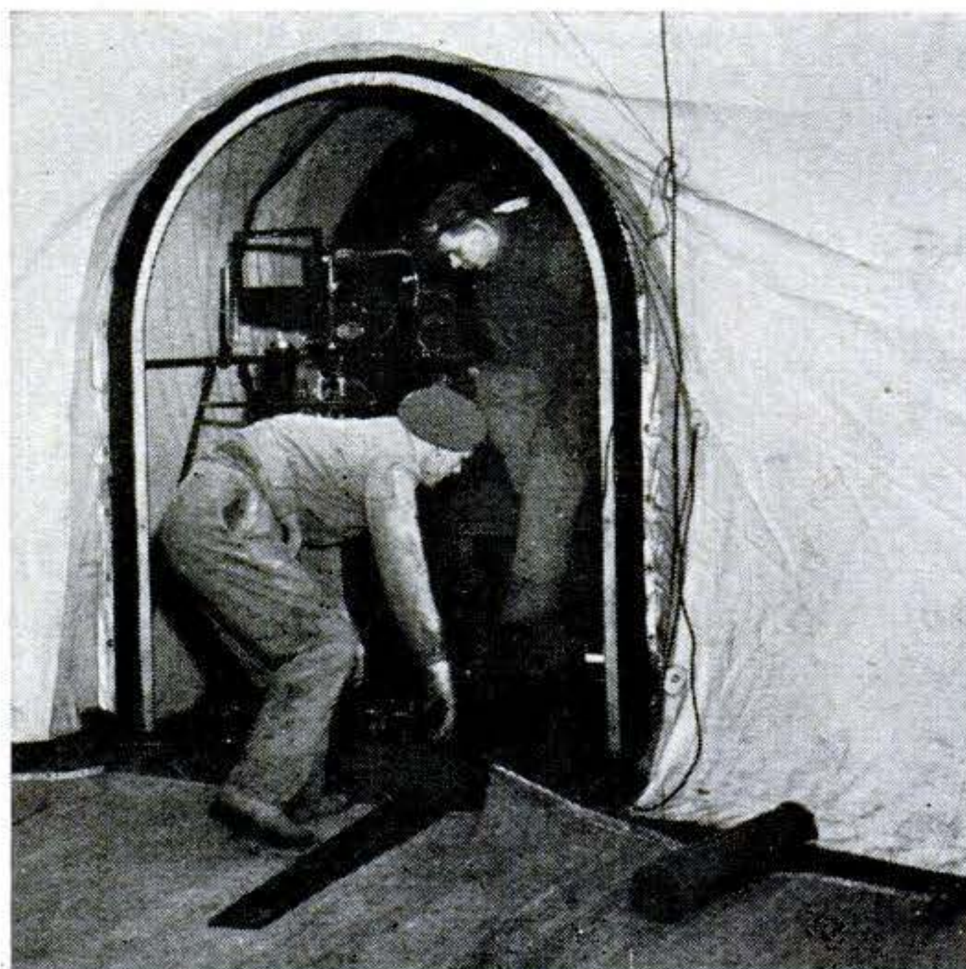
Double-door air lock lets men and equipment enter inflated dome without air escaping.
