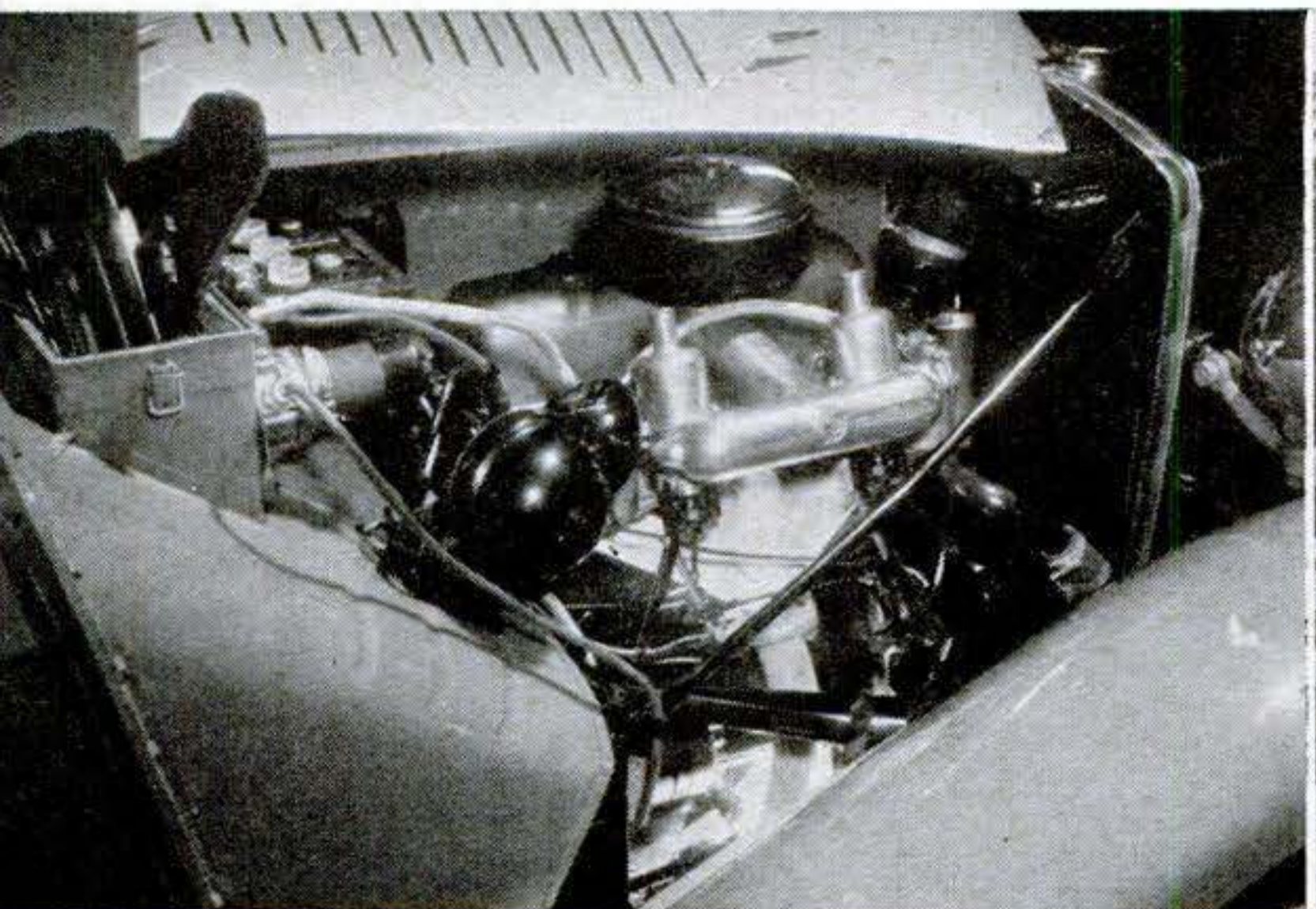
Engine is still 4-cylinder, 54-hp. , unchanged except for T-shaped air intake connecting dual carburetors with single filter. Note built-in tool chest at left, large 12-volt battery in rear.
