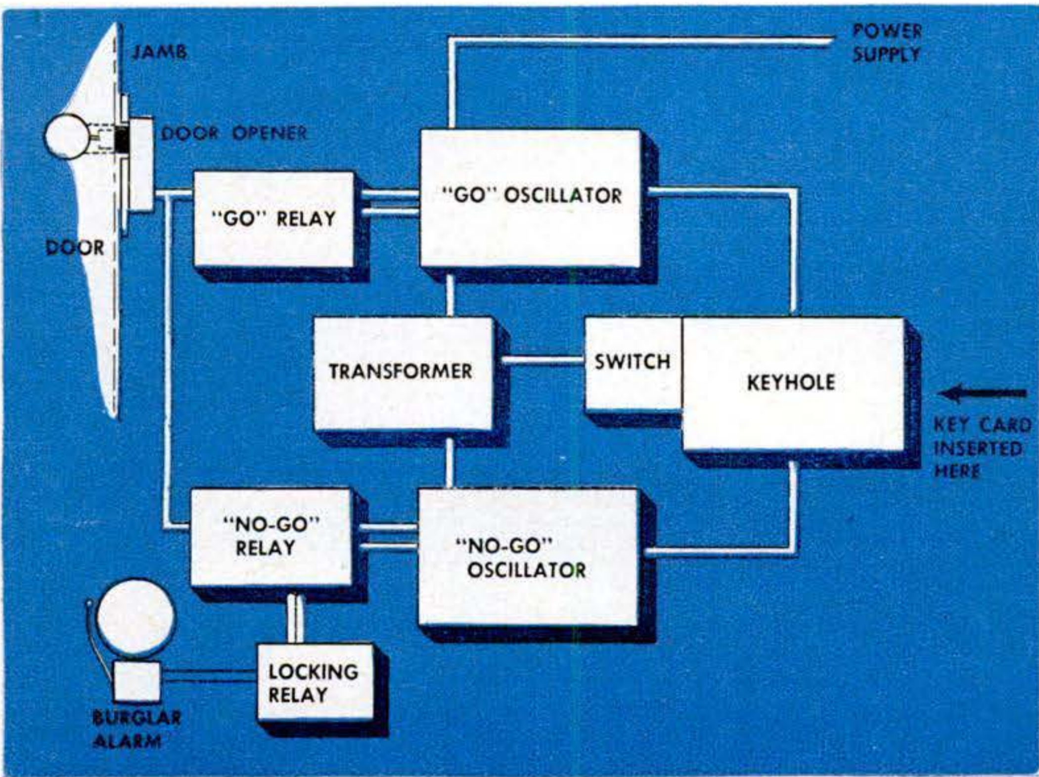
Block diagram shows components of lock made by Electronic Lock Co., Hollywood, Calif. At far right are key layers—from top down: outside sections, sheet with graphite strips, lightproof paper. Lock can be set so wrong key sets off a burglar alarm.
