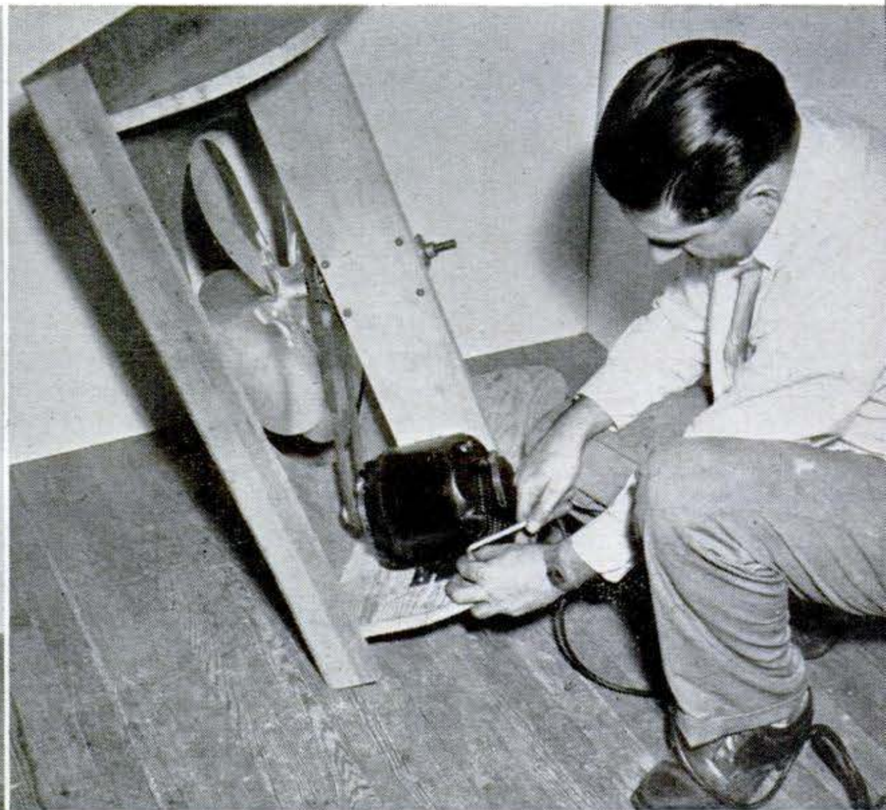
Fan and motor should be bolted in place. Rubber mountings are best. A 20" fan with 2½" pulley driven by 1/6 hp. motor with 1½" pulley will circulate air in small house.
