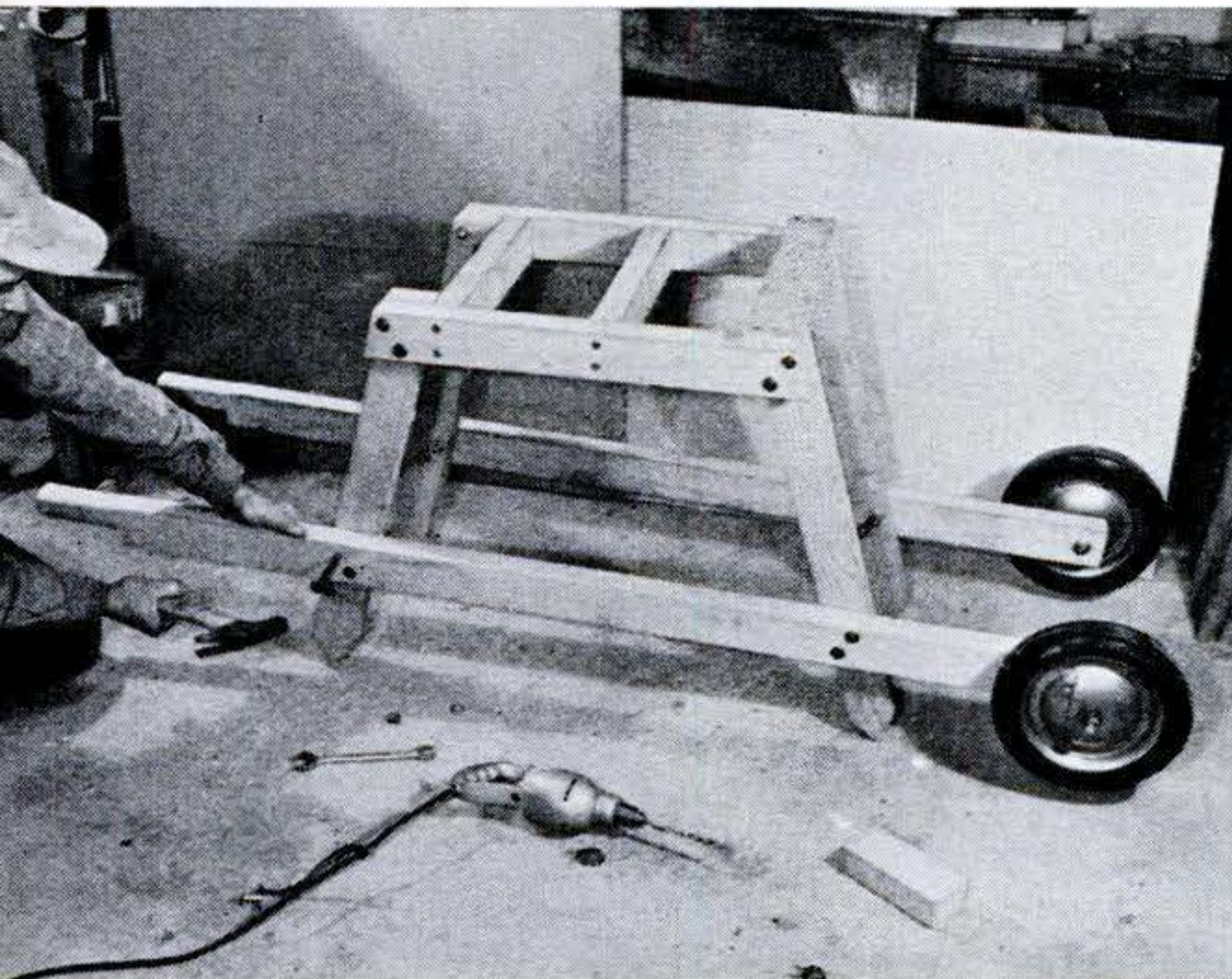
Details of sawcart construction are shown above. Crosspieces are held by wood screws 3½" long. Distance from grip to leg is 18".
