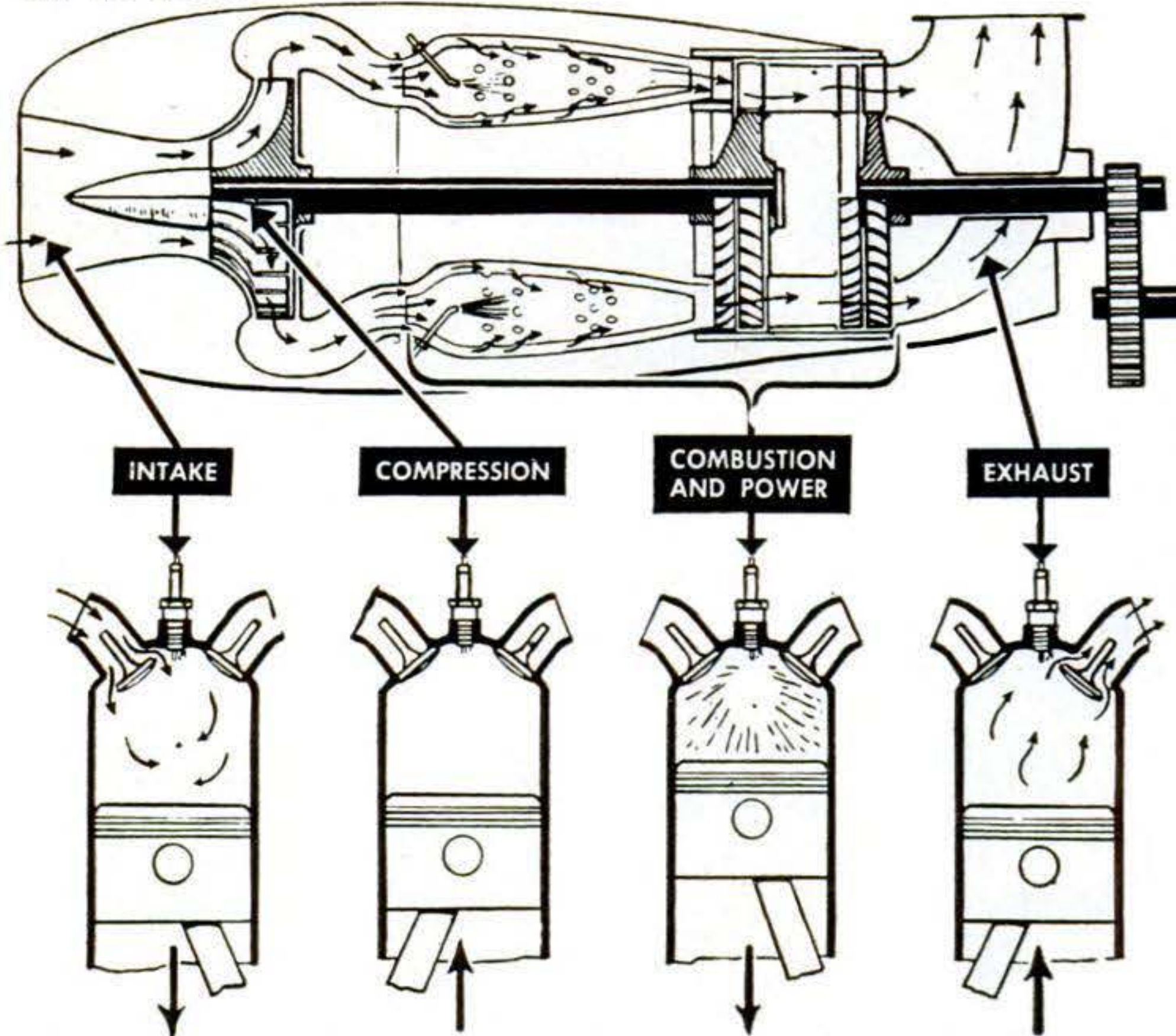
Gas turbine can be compared this way with piston engine.
