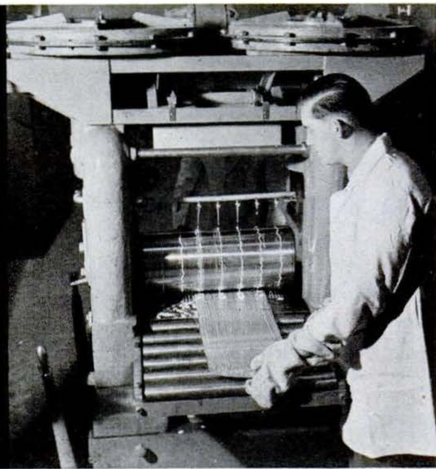
4 Operator above pulls aluminum sheet out of machine, whose rollers squeeze with a pressure of 700,000 lb. A full-size mill uses 2,000,000 lb. of pressure to flatten a 5,000-lb. ingot.
