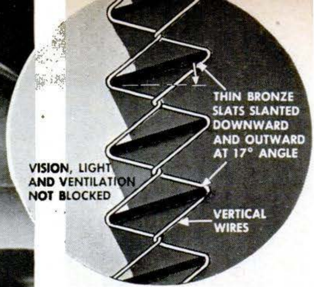
Special window screens will keep out direct rays, as well as insects, without interfering with view. Tiny horizontal slats placed at angle stop rays. Photo at left shows how sunlight passes unscreened window but is blocked by slats.
