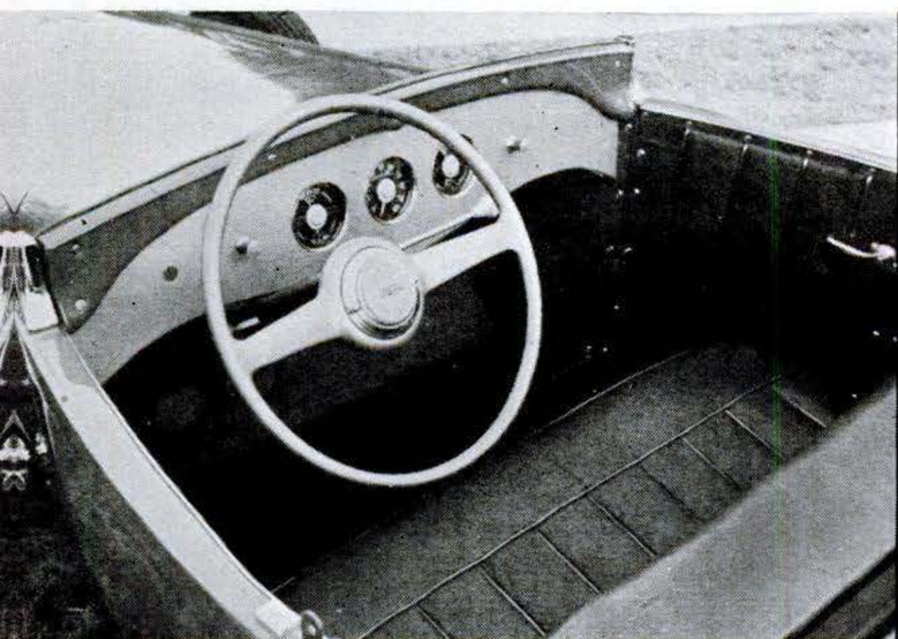
Dashboard is clean and simple, with '49 Plymouth instruments grouped in center. Steering-column gear shift and transmission are from '49 Ford. Headlights are added for night driving.
