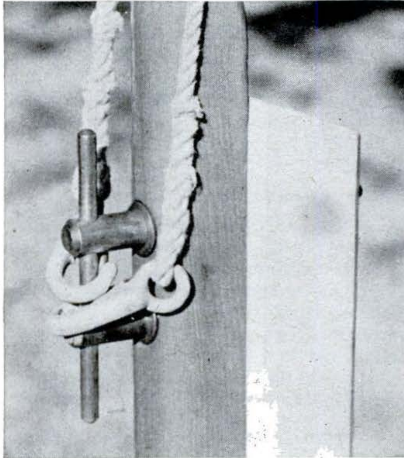
Snap fasteners, hooked into special cleat, hold flag up. They can also be snapped to cleat after flag is lowered to keep wind from banging them against pole. Drawing shows cleat details.
