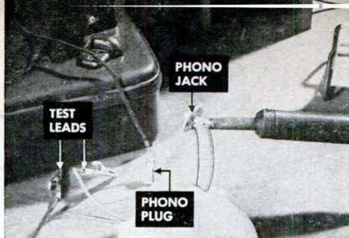
Making the test leads
