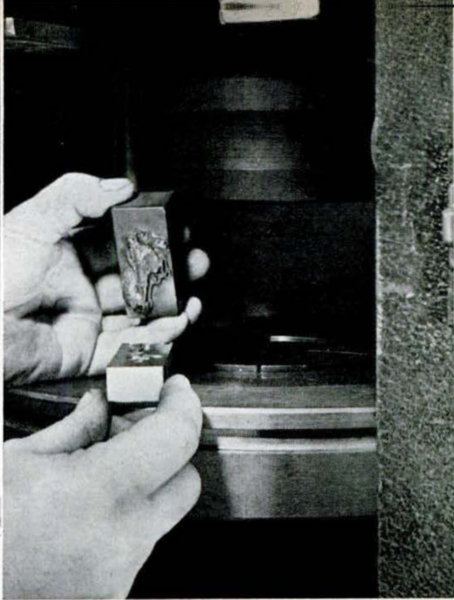
Under pressure of 100 to 300 tons, the hob is squeezed into soft steel blank (lower block). This reverse image, called a "cavity," is used as mold of figure into which plastic is injected.
