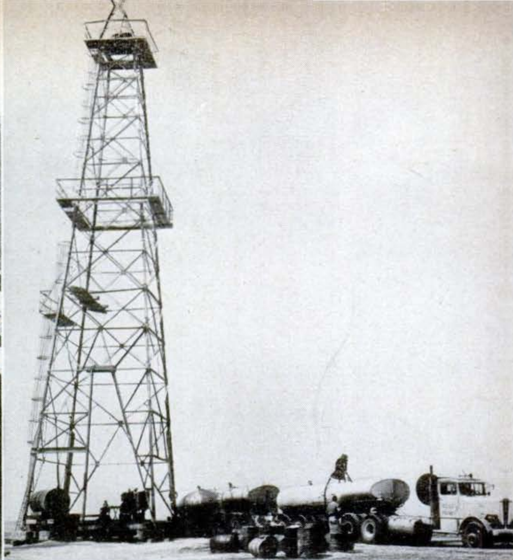
Tank trucks load up with fresh water at one of 40 wells drilled along pipeline route to supply construction crews. Man-made oases have become centers of new Bedouin settlements.
