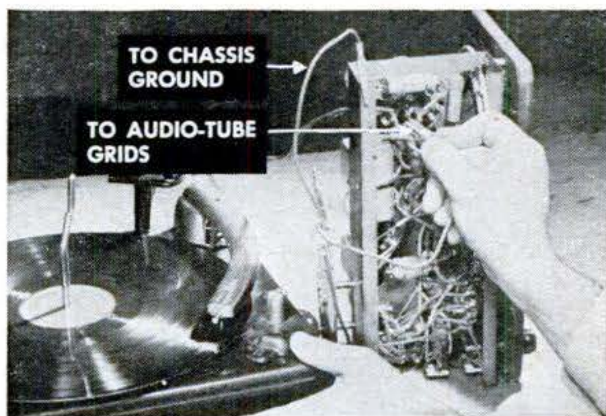
Checking the audio circuits
