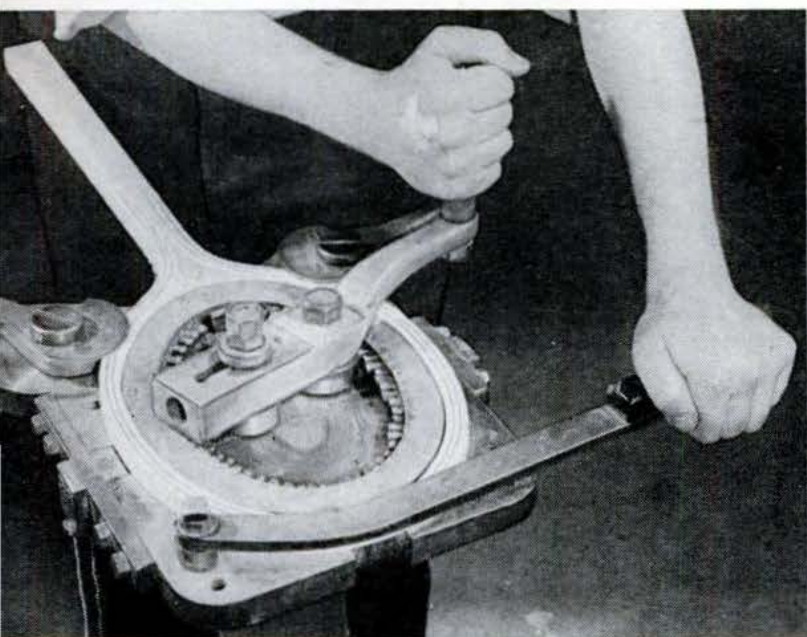
7 The locations of the string holes are marked in this jig. When frame is clamped in place, turning the handle on top of the jig forces pins out to mark inside of the bow.
