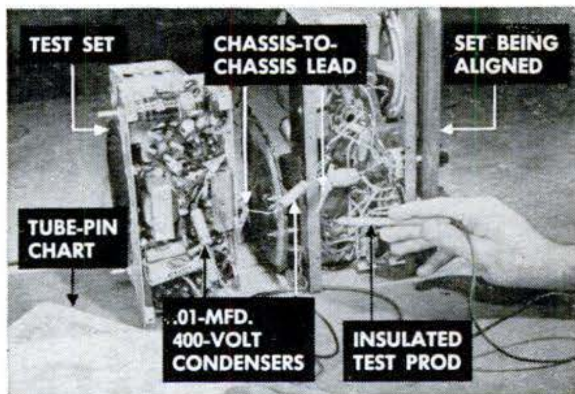
Feeding an I.F. signal
