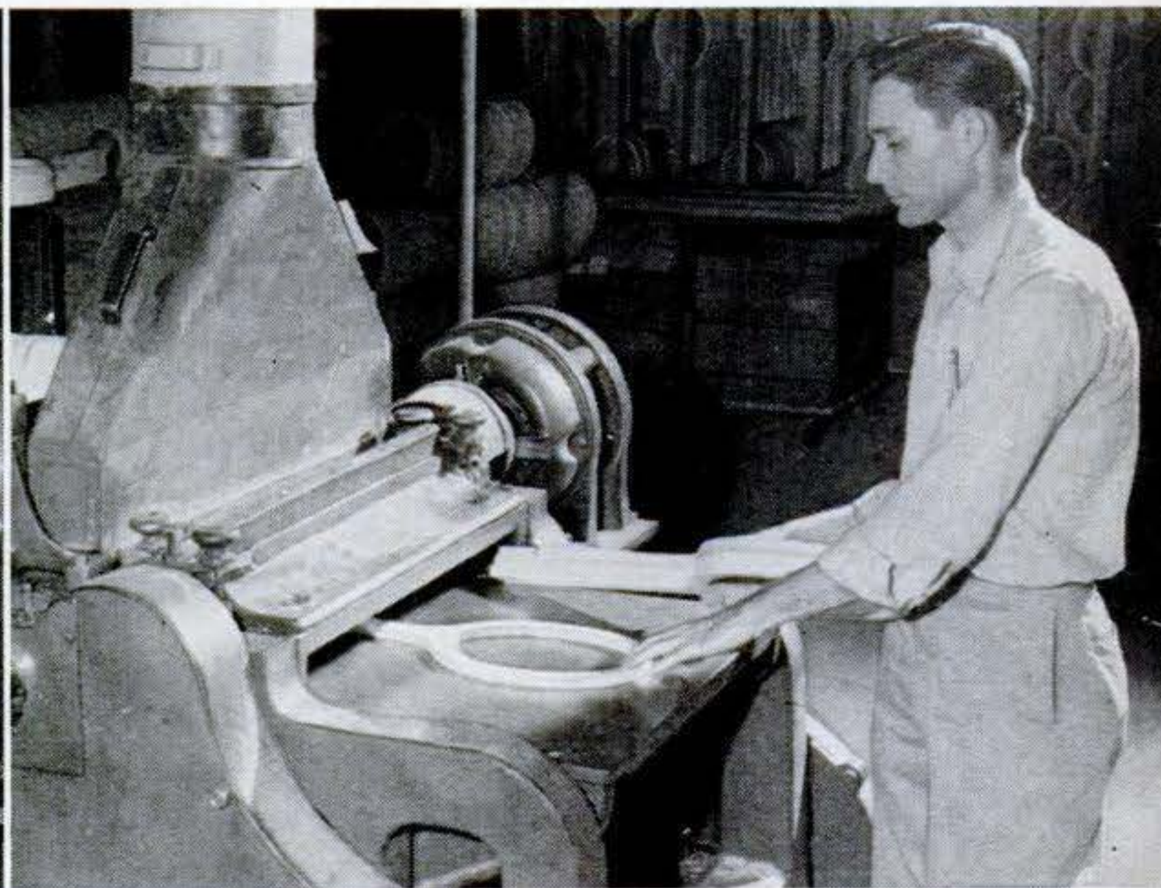
6 First, one side of each frame is machine-planed to provide a smooth working surface. Then the second side is machine-planed down to the proper frame thickness.
