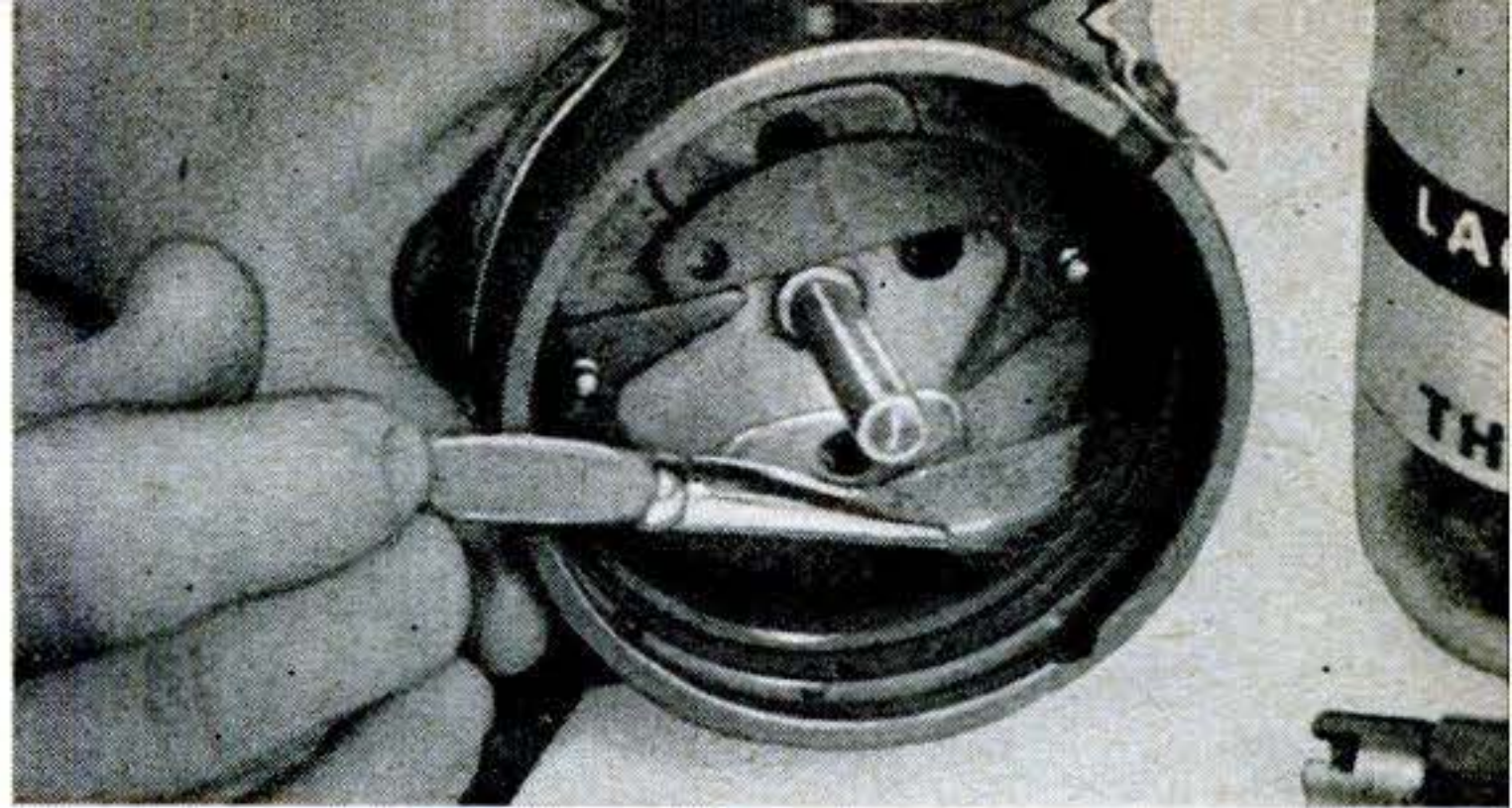
Wash out distributor with lacquer thinner and soak small parts in jar. Sticky deposits stop free movement of breaker plate and other parts.
