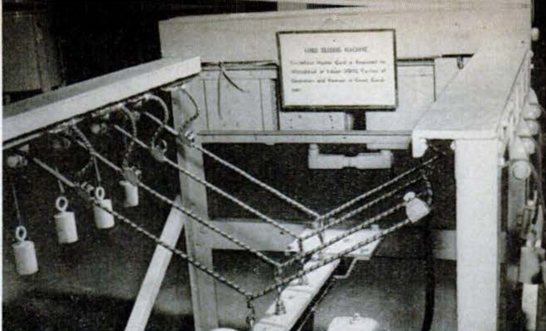
Extension cords , held taut by weights, are twisted and untwisted 3,000 times to make sure the insulation won't break down, exposing the wire and creating danger of fire or shock.
