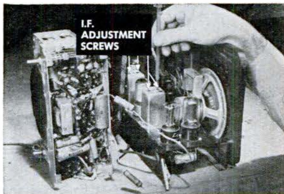
Adjusting the I.F. trimmers
