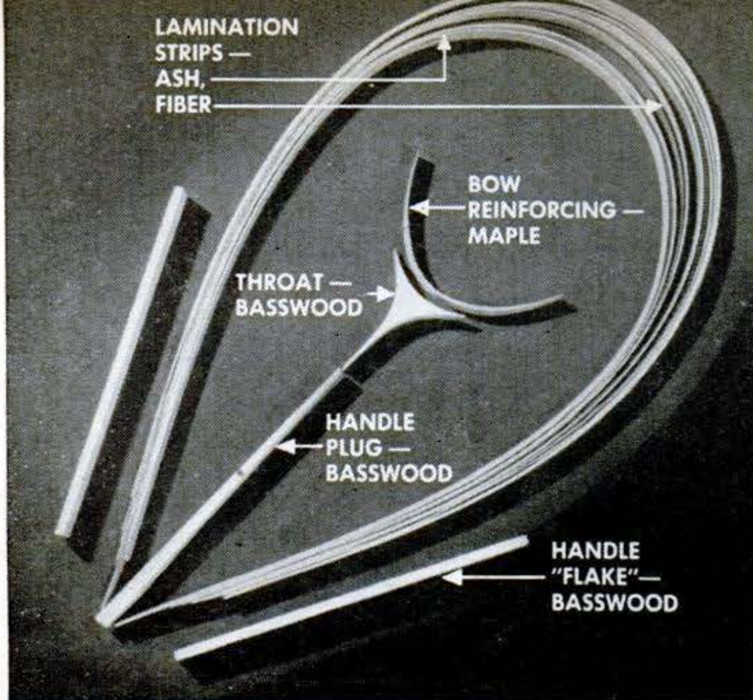
1 Here are basic parts that go into a tennis racket. The wood laminations are 64-in.-long strips cut freehand with the grain from clear, second-growth mountain-ash boards.
