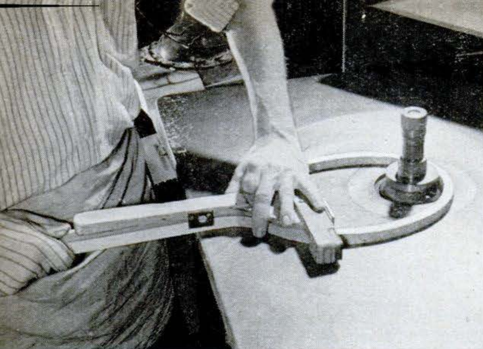
10 A vertical shaper is used to form rounded edges on the inside and outside of the bow. A guide under the revolving cutter determines how much wood can be removed.
