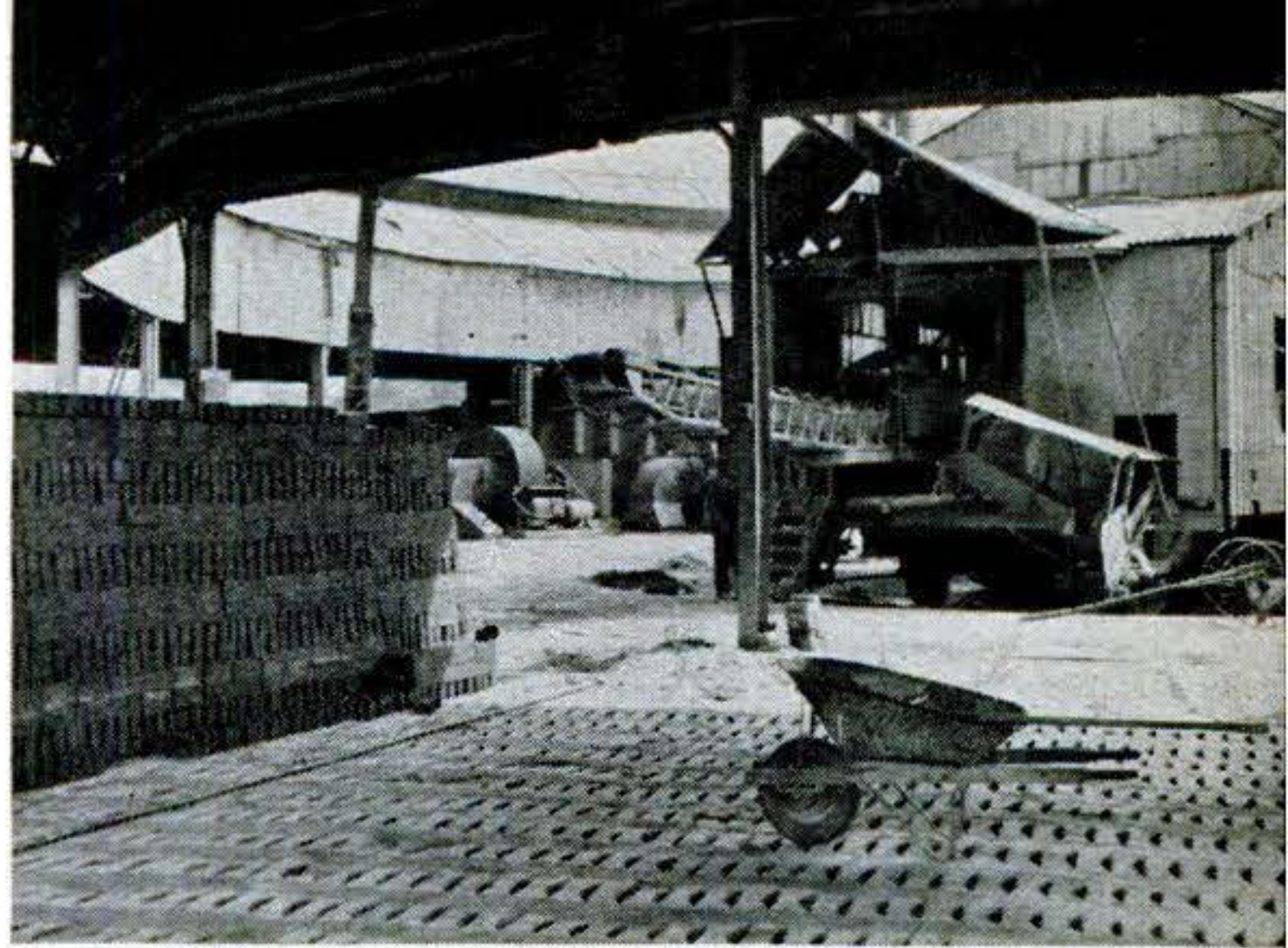
Lower conveyor of central building retracts to clear roof columns as building revolves. Then it extends to deliver raw bricks to workers, who stack them in piles as at left.
