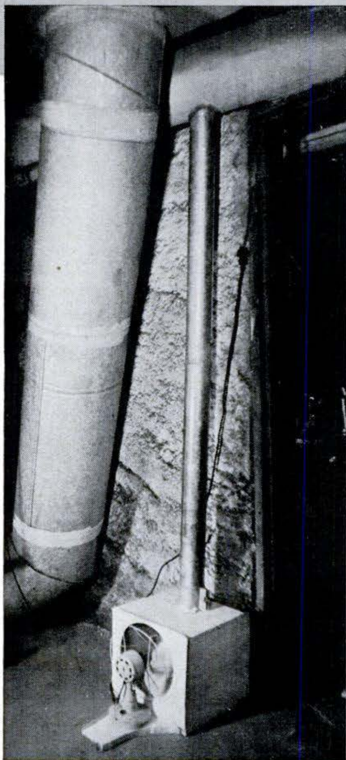
HOT-AIR FURNACE
