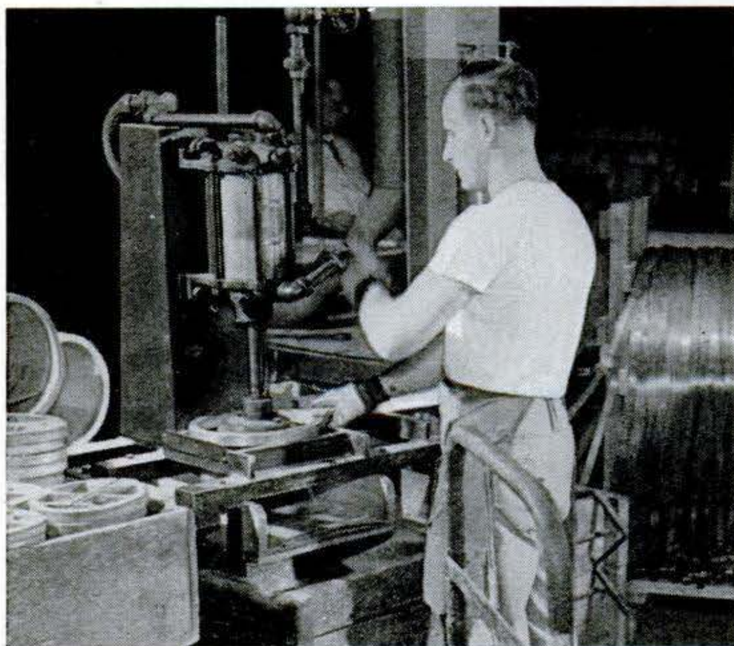
5 After 4 hours of kiln drying and 8 of air drying, the clamped form is removed and the basic glued laminated racket frame starts down the woodworking production line.
