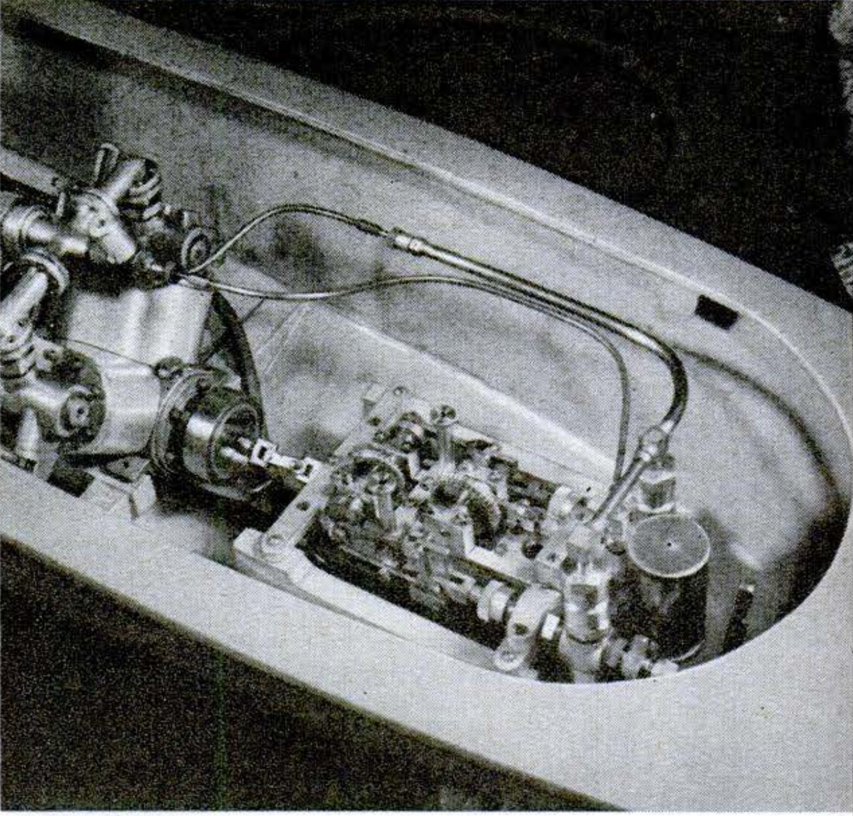
3 Speedboat hull like this is crammed with power plant. Boiler consists of yards of tubing heated by a gasoline blowtorch. Four-cylinder, single-action piston-valve engine is at left above. Oil and water pumps of Lacey's design are to the right of the engine.
