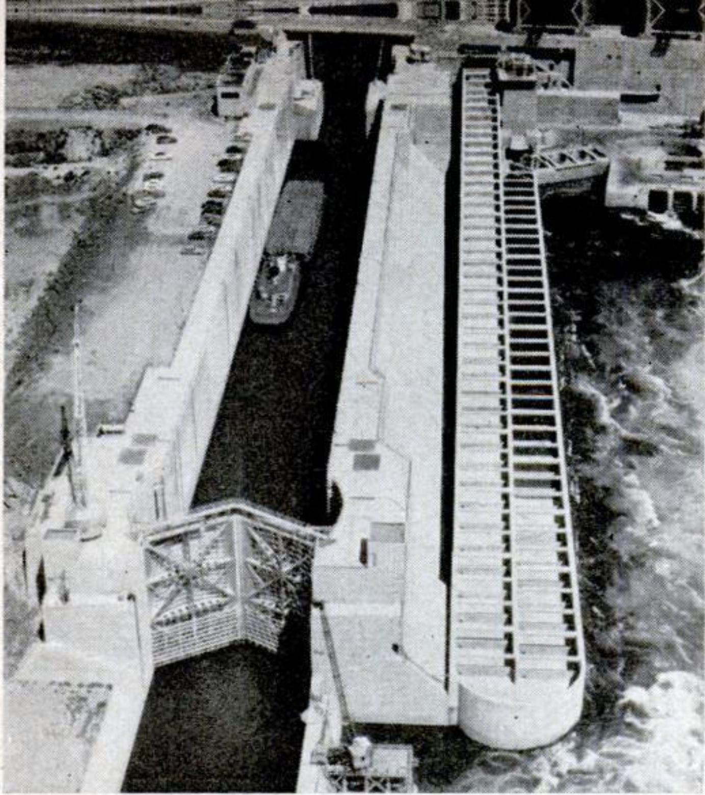
LOFTIEST LOCK in the world is this one at brand-new McNary Dam on the Columbia. Measuring 56,000 square feet in area, it hoists ocean-going tugs and barges 92 feet.
