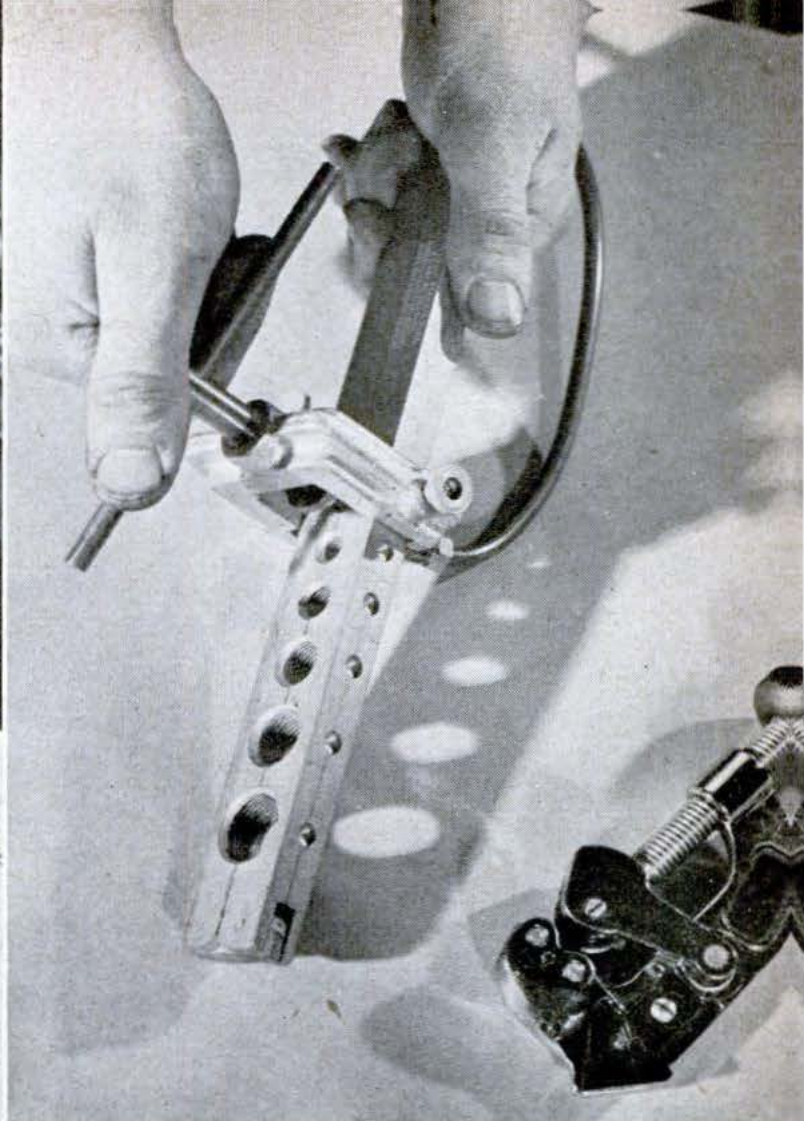
HAVE TUBING FLARED , at a reliable garage, for making the hydraulic connections. Remember, these lines must hold 800 lb. of hydraulic pressure. Failure can be serious. Don't forget to slip fittings on before flaring.
