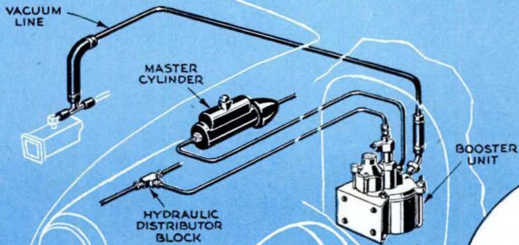
CONNECTIONS to be made in installing a power-brake unit for your car are one vacuum line and hydraulic lines in and out.
