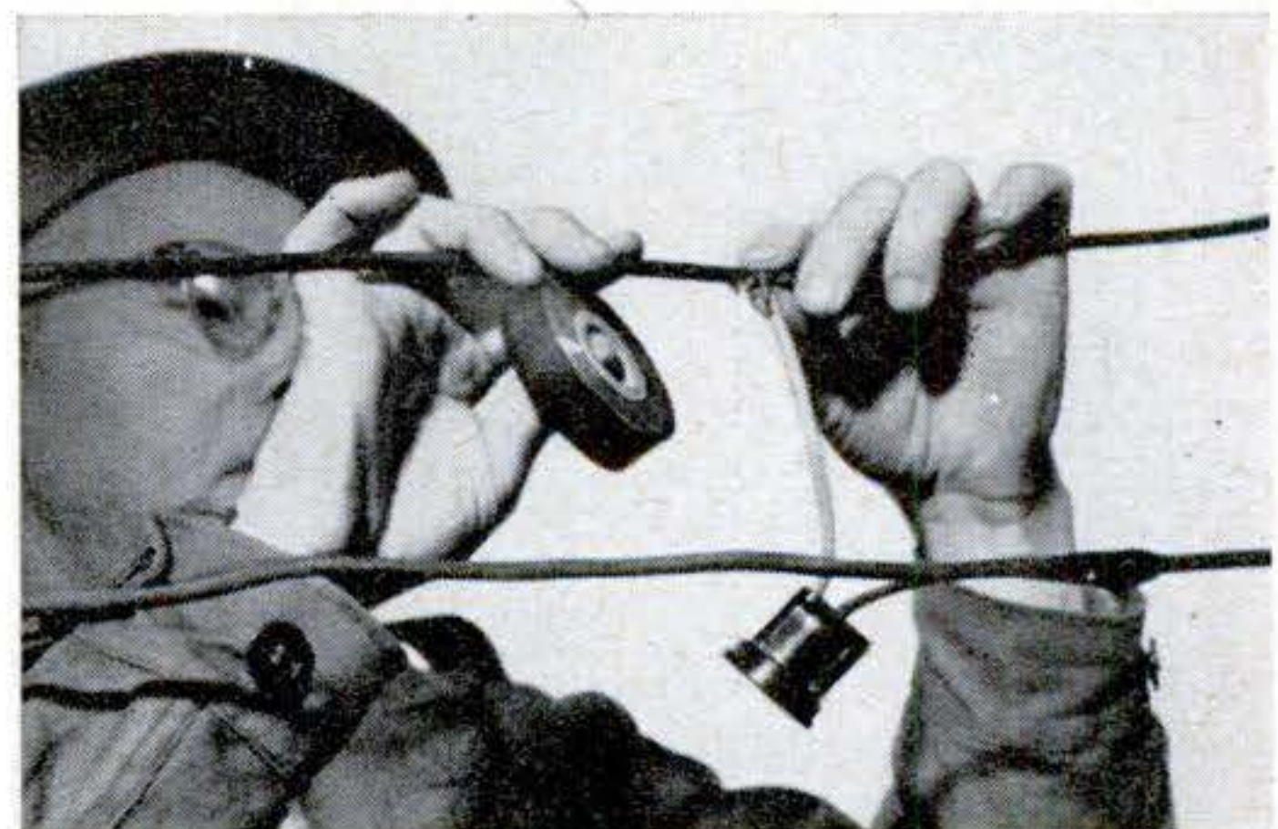
SIMPLEST ALL-WEATHER LIGHTING consists of weatherproof wire and socket tapped in where wanted. Bare the wire, make connection, insulate with plastic electrical tape.
