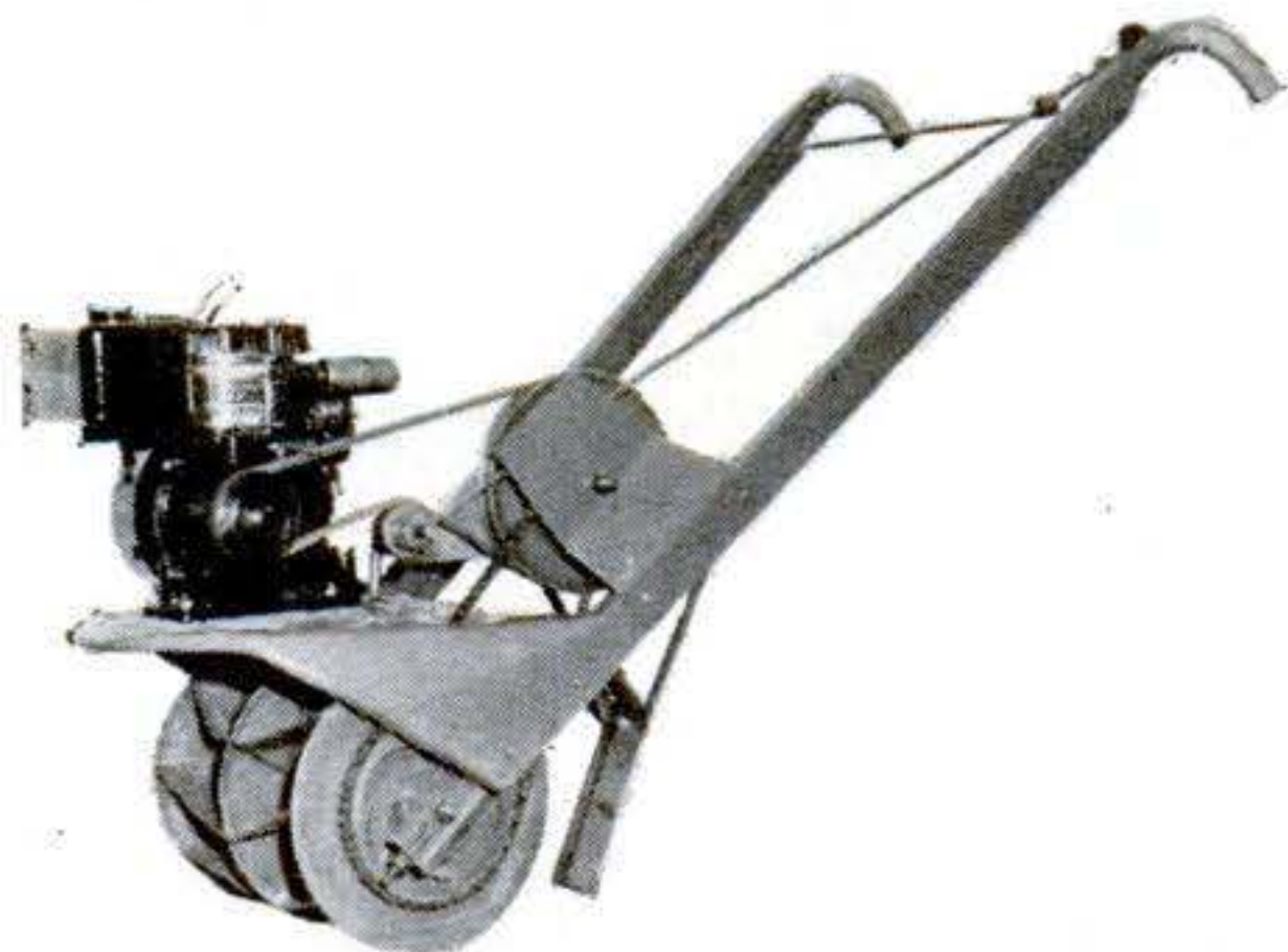
ONE WHEEL does all the work in this powered Hull hoe. Bladed drum acts both as drive wheel and pulverizer to break up earth. It takes plows, other attachments.
