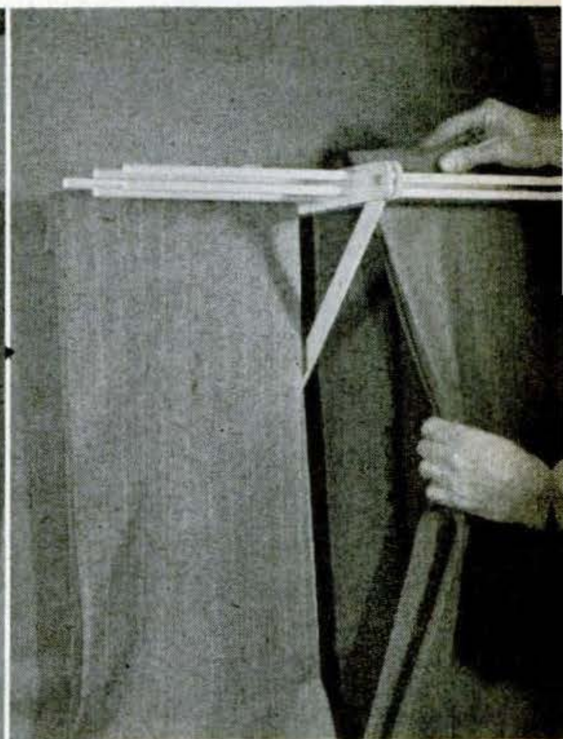
JIG SPACES HOLES right if dowels are all the same length. Drill holes near both ends with the stop close in. Move it away to drill the two inside holes. Thread cord as at left.
