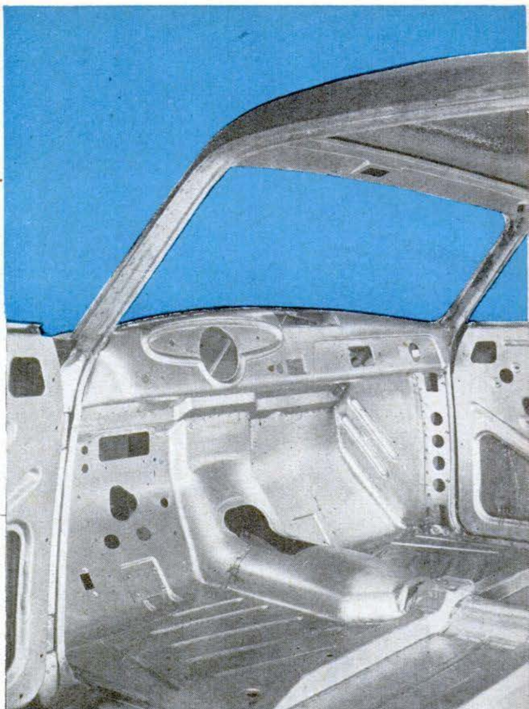
ABOUT 8,000 SPOT WELDS are needed to put together the five main parts of a unitized Aero Willys body. This interior view shows how skillfully the welding job is done.
