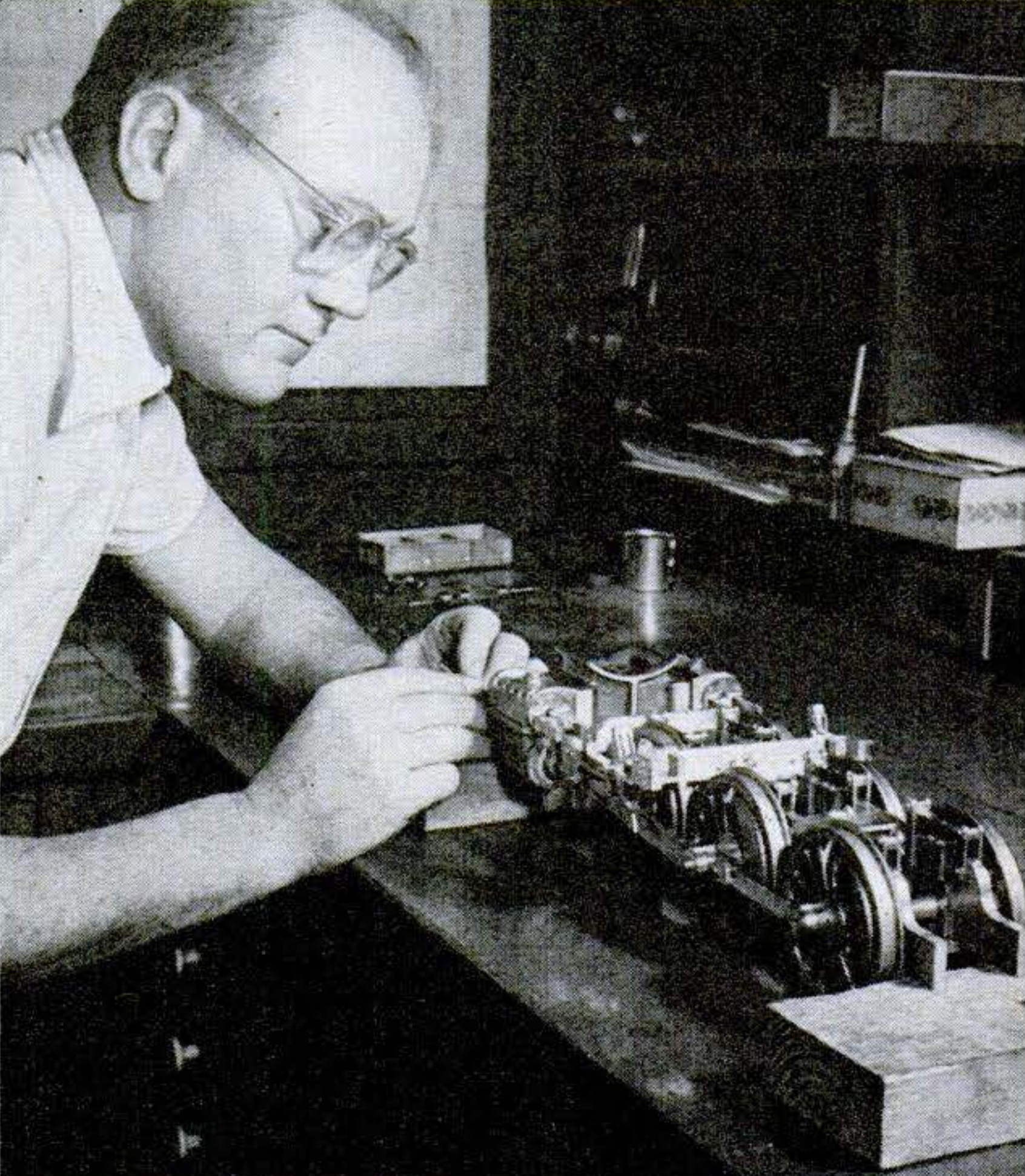
1 Running gear of this 1/2"-scale (2 1/2"-gauge) Pacific locomotive shows precision work. To be driven by live steam, the engine will have Walschaert valve gear (just like a real locomotive's). Cylinders are 1" bore, 1 1/4" stroke. The rods are milled from solid steel.
