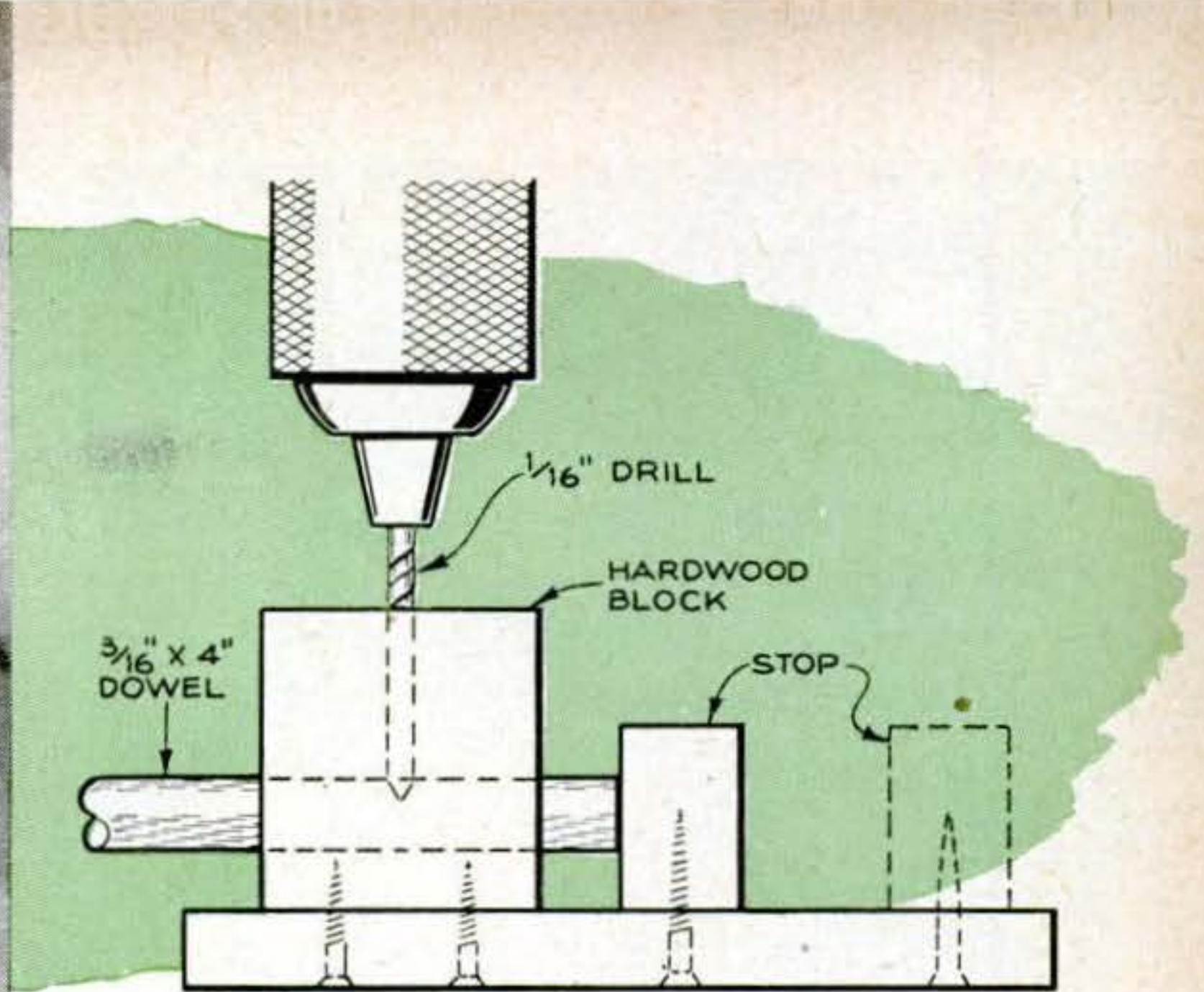
JIG SPACES HOLES right if dowels are all the same length. Drill holes near both ends with the stop close in. Move it away to drill the two inside holes. Thread cord as at left.
