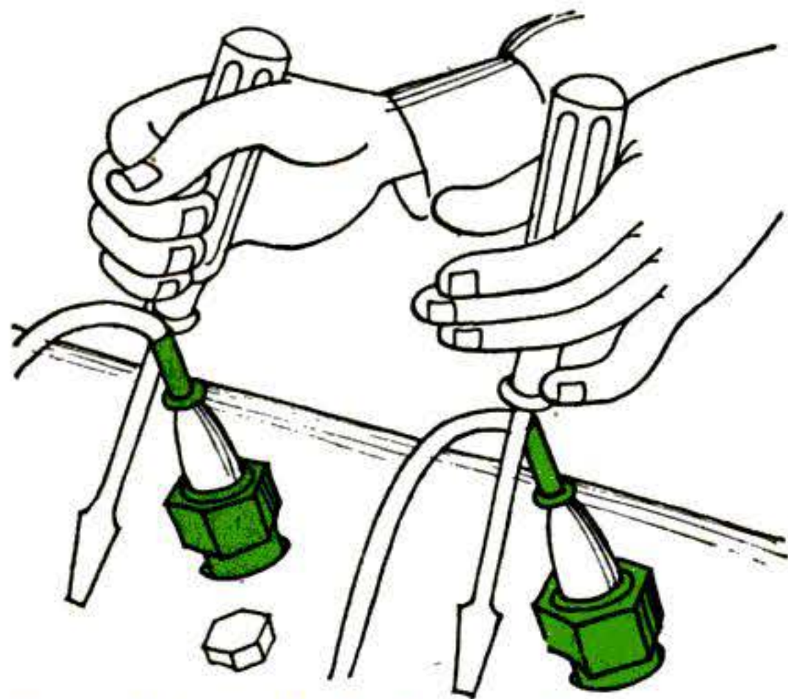
Screwdrivers check plug performance
