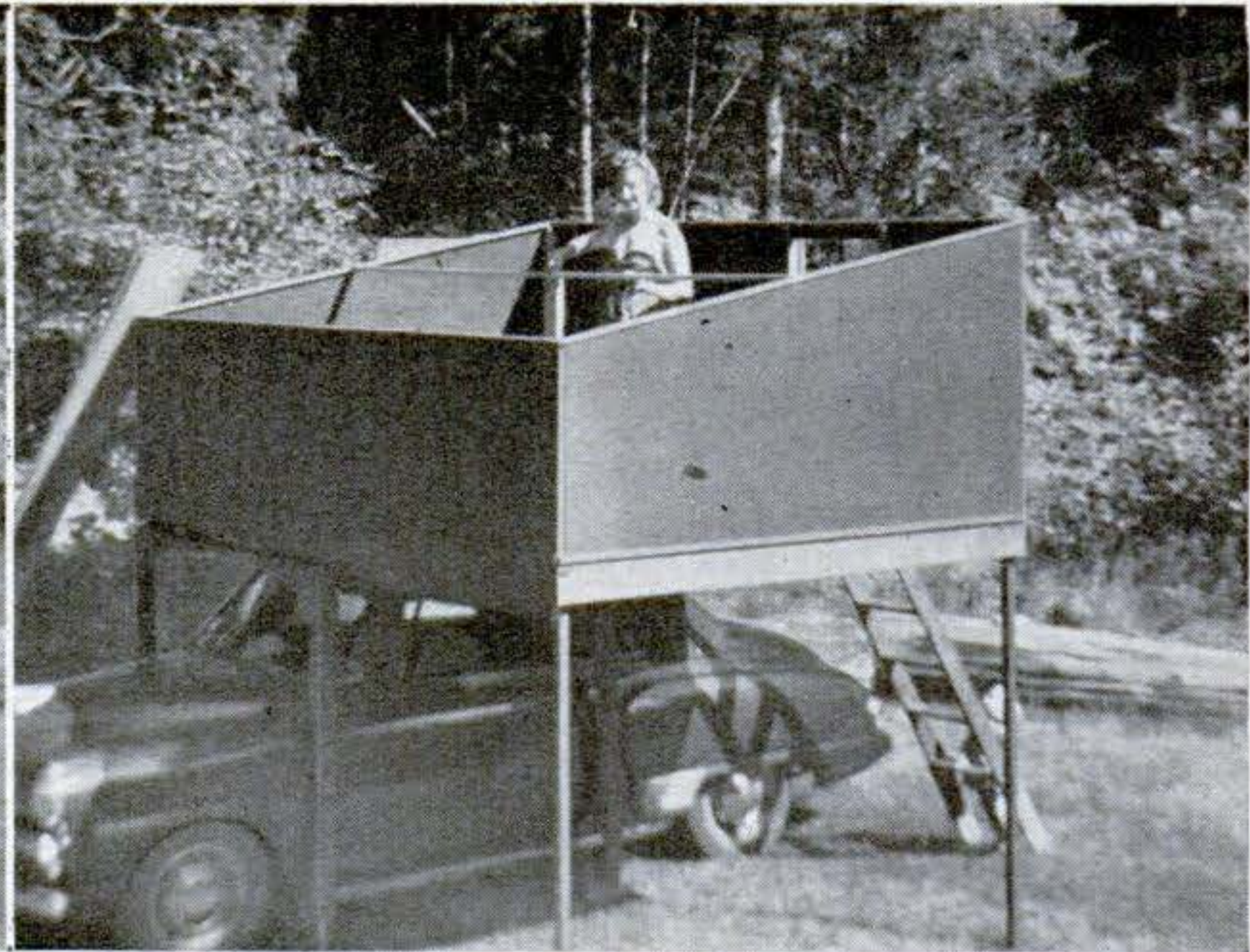
Bolted-together walls hold roof support . . .
