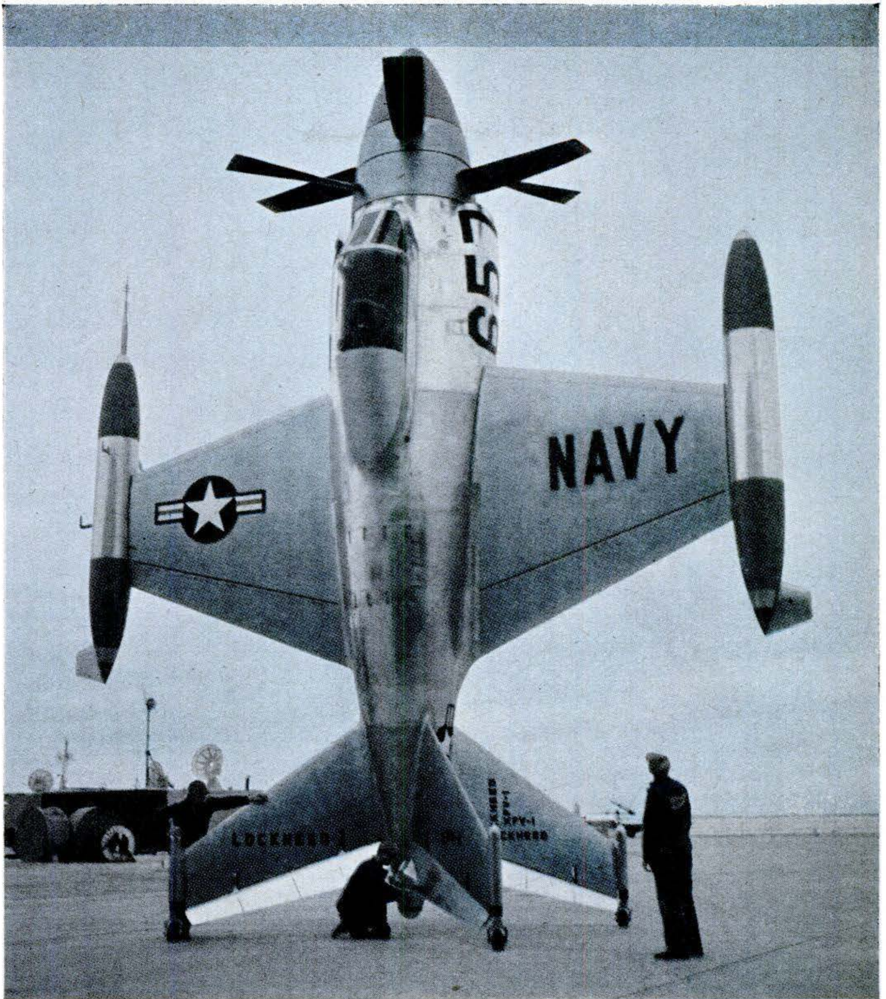
Four-pointed, X-shaped tail is landing gear of Lockheed XFV-1, shown in take-off position.
