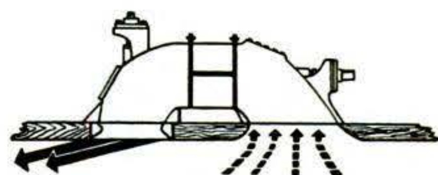
WATER JET. Engine of this British boat is an inverted U pipe, open at its two ends. A built-in pump sucks in water at the front, ejects it rearward to propel the craft through obstructed or shallow waters. Deflector vanes provide steering.
