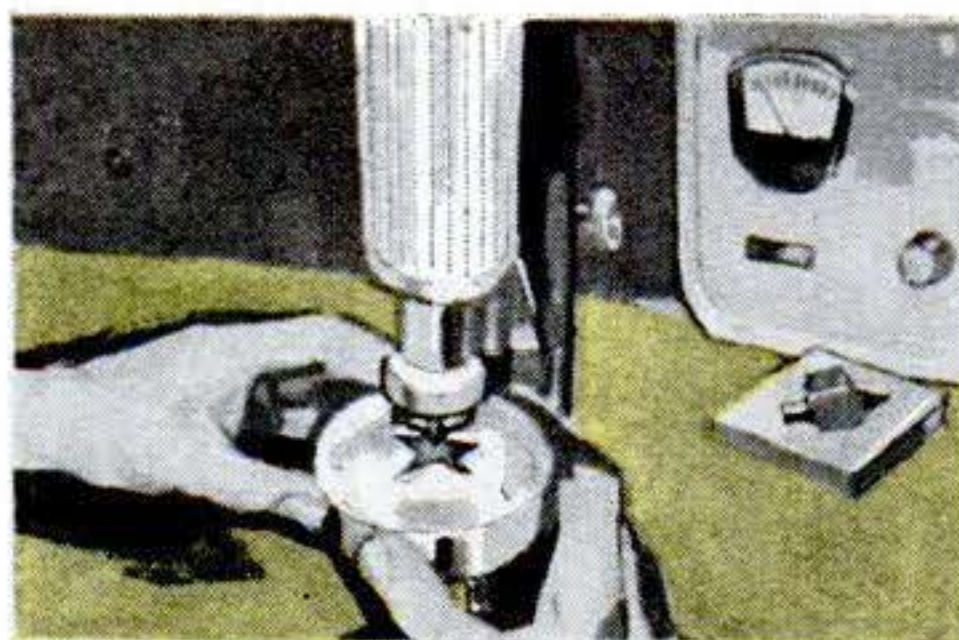
DRILLING HOLES. Sound generator "bit" vibrates abrasive to cut through hard materials. Hole copies shape of the bit.
