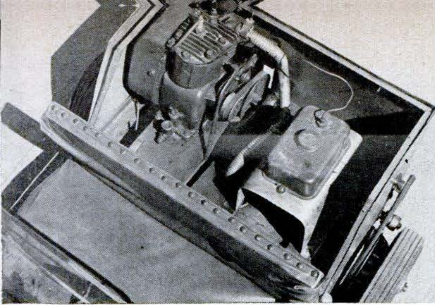
BOXED-IN ENGINE of Capt. Sparks' jeep drives a jackshaft extending over the drive wheel. The rear axle is mounted on half lengths of auto leaf springs. Spring-tensioned idler keeps the belt taut. Pushed forward, the control tightens a band brake on the other (nondriven) wheel.
