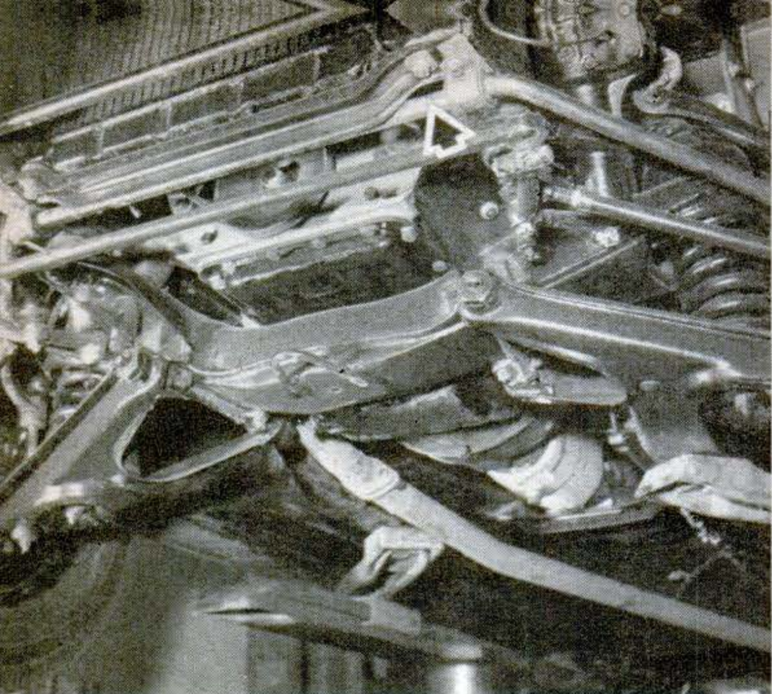
FRONT WHEELS ARE SPRUNG on conventional wishbones and coil springs, with an anti-sway bar across them (arrow). The engine, wheels and transmission are all mounted on the heavy crosspiece shown, and can be removed as a unit.
