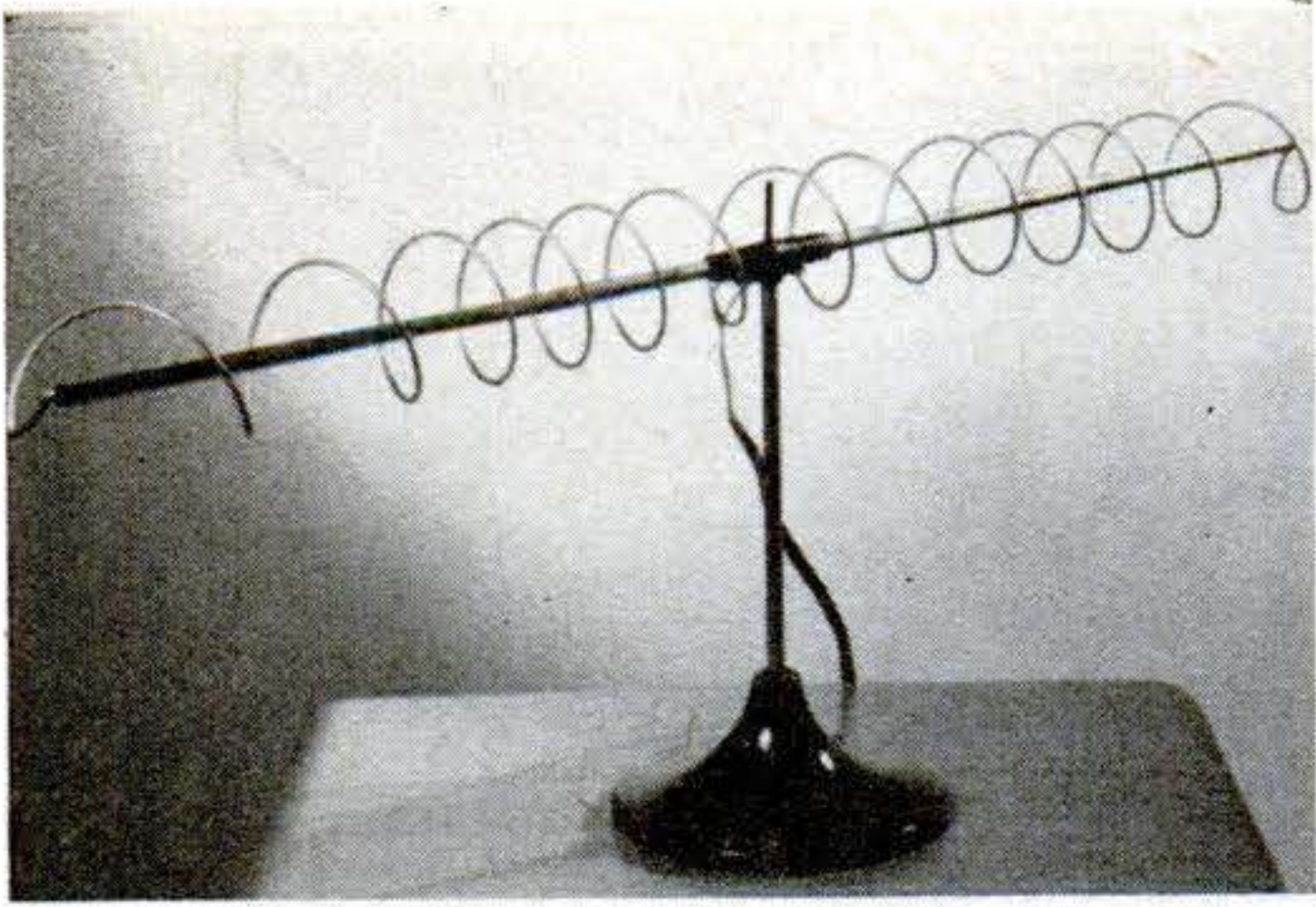
SPIRALING the long, low-channel element of this "Hi-Lo" antenna around the shorter high-channel element is said to give the same effective reception as a long straight-line dipole.
