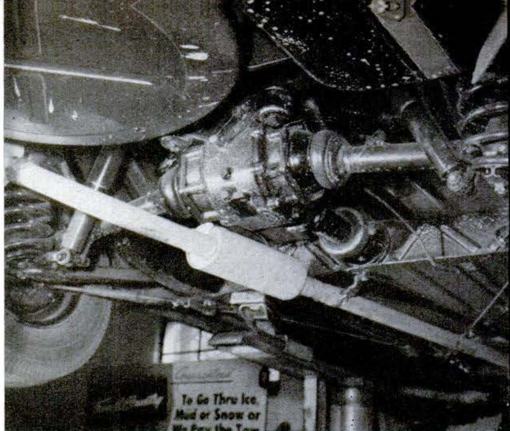
MOUNTED ON RUBBER but firmly fixed to the body-chassis, the differential drives the rear wheels through short swing axles, with radius arms taking the torque thrust. Gas tank is visible at top right, spare-wheel well at left.
