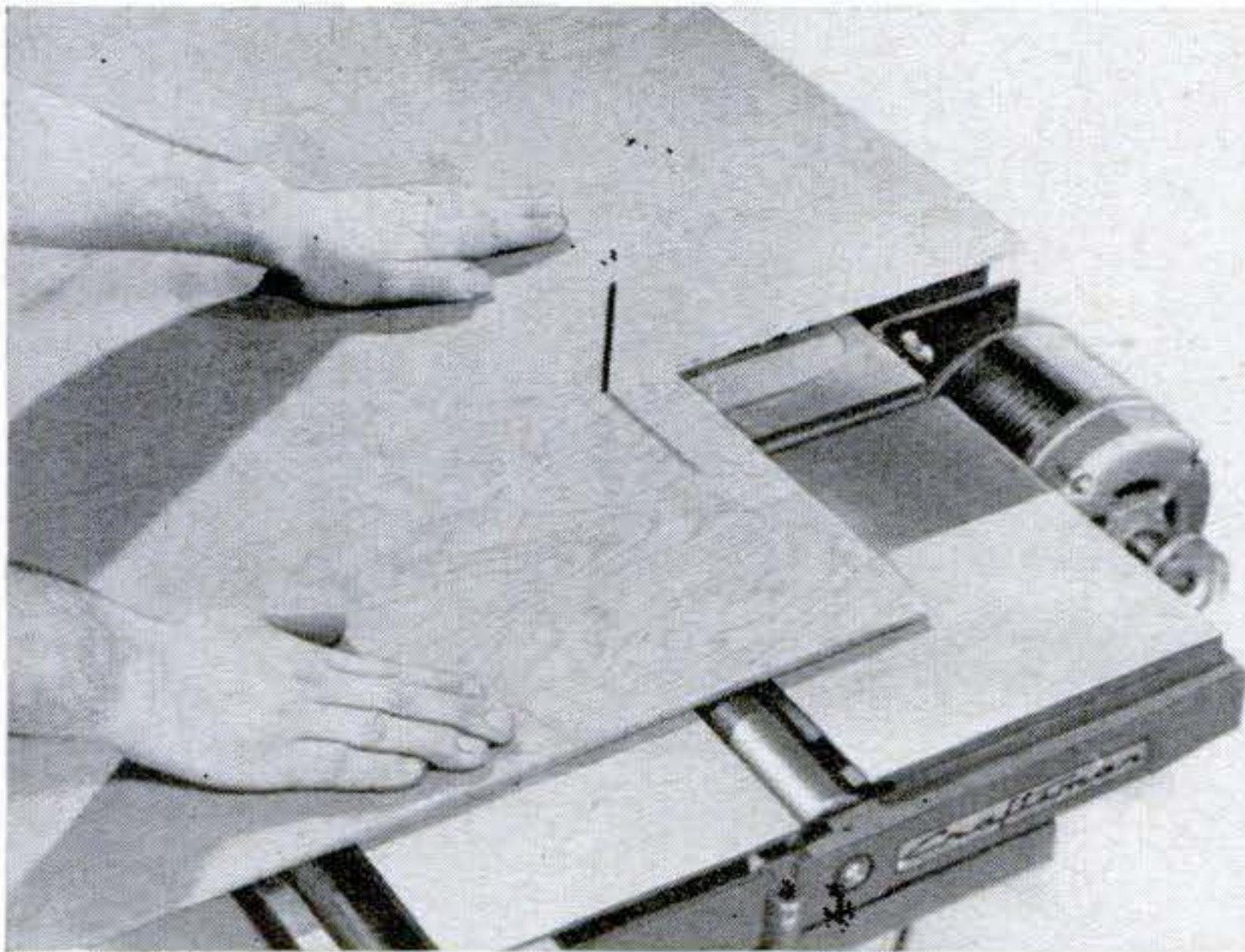
FIVE-IN-ONE-TOOL is Sears, Roebuck's new entry in the multipurpose field. Basically an 8" tilting-arbor bench saw, it sets up as a saber saw (above), jigsaw, disk sander and 4 1/8" jointer-planer. Center pedestal makes it easy to reach. Price: $5 down, $189.88 total.
