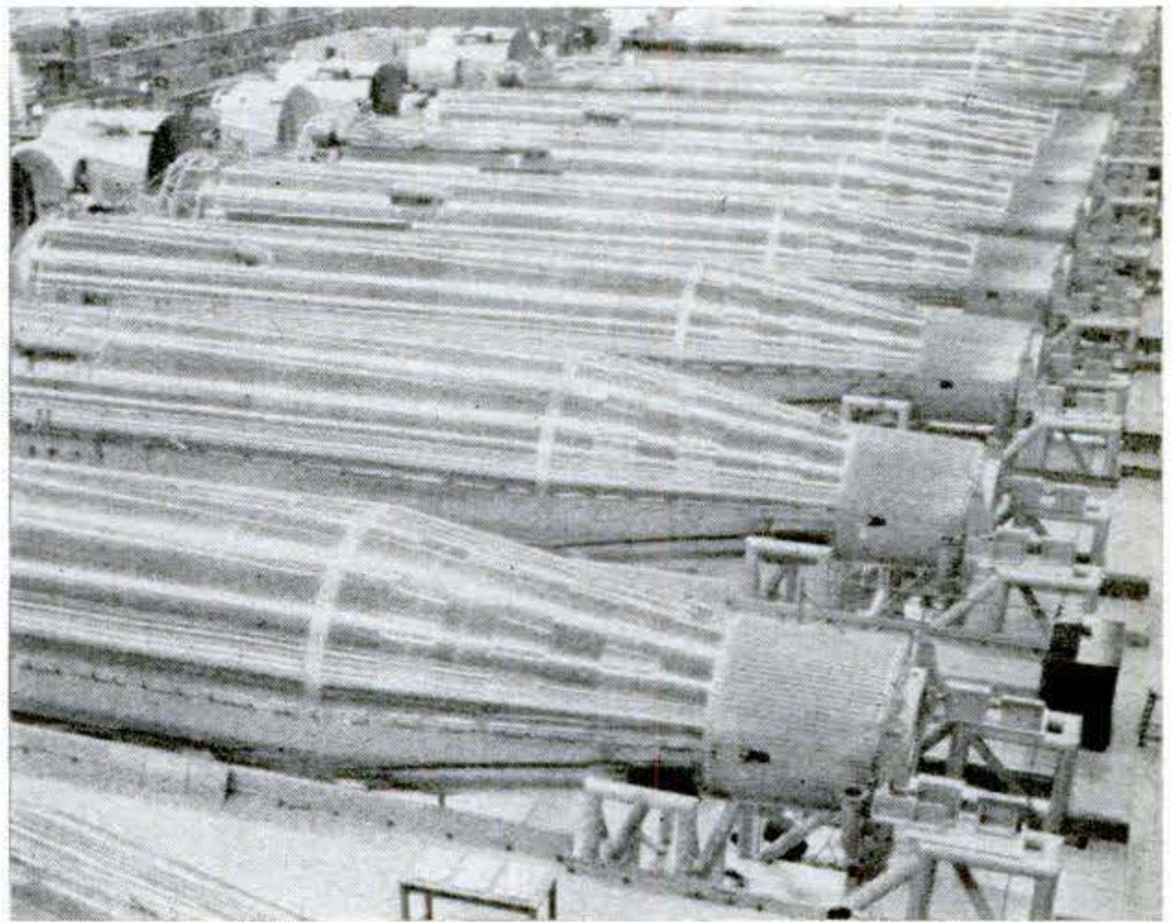
ATLAS PRODUCTION LINE. Air Force intercontinental ballistic missiles are assembled here before delivery to test sites and operational squadrons. The 75-foot stainless-steel rockets rest in test racks at Convair's San Diego plant.
