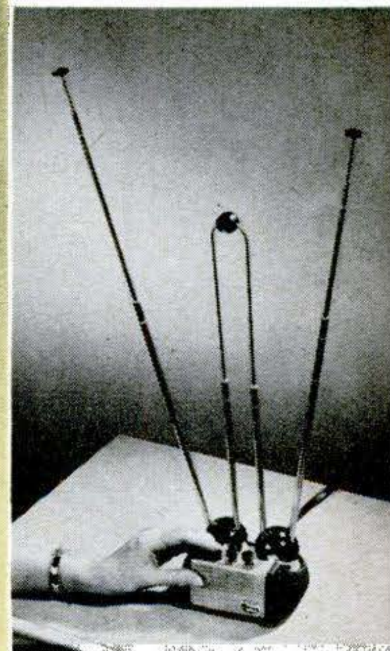
PUSHBUTTONS take place of rotary switches on these modified rabbit ears. Telescoping center loop is said to aid tuning and adjustment.
