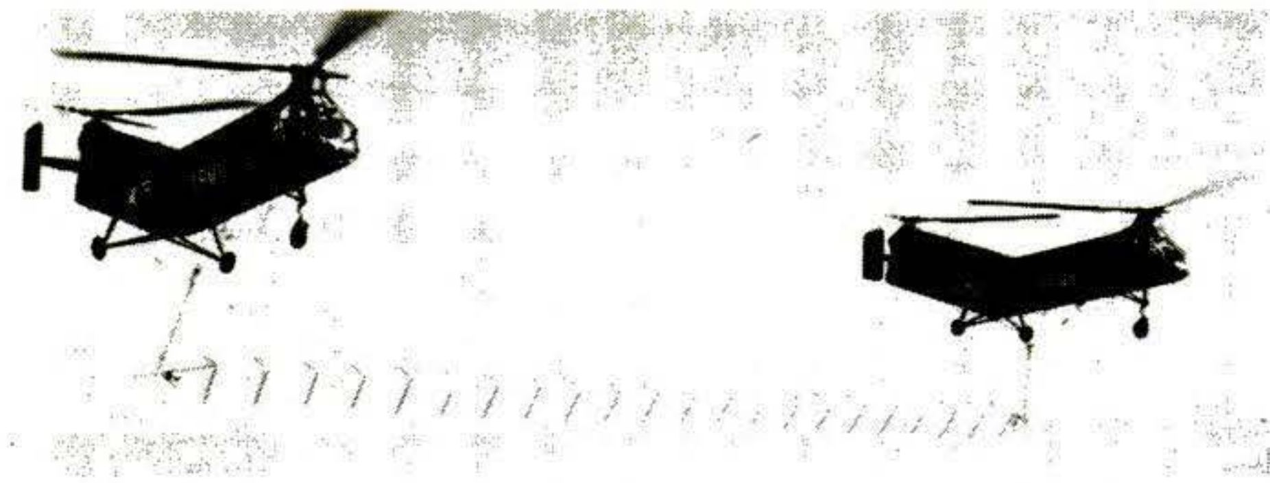
WHIRLYBIRD HARNESS. The aluminum-alloy frame slung under helicopters above was built by Vertol for combat hauls. Teamed as in the drawing, four or more could lift a big Army truck too heavy for one.
