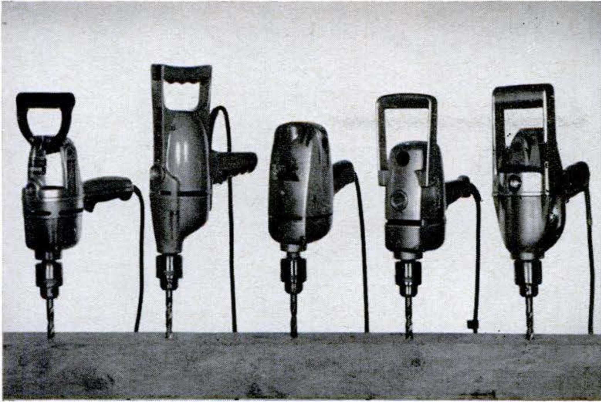
SLICKED UP, SLIMMED DOWN: New 1/2" electric drills, once considered strictly pro, are styled with a new eye on the home-shop market. Some weigh as little as eight pounds, sell for less than $50. Left to right: Black & Decker, Millers Falls, Remington, Sunbeam, Thor.
