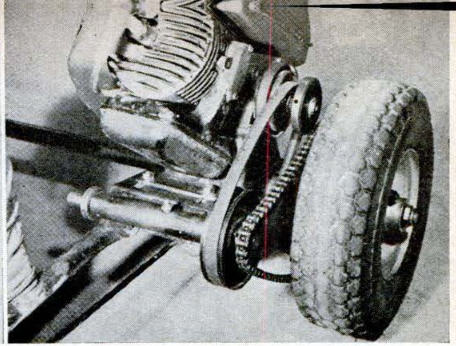
SLICKLY PROFESSIONAL is this two-step reduction drive engineered by V-Plex Clutch, of Hagerstown, Ind. The jackshaft turns in a tubular crosspiece mounted on one frame member. As the engine revs up to 1,800 r.p.m., the centrifugal clutch engages the belt. END
