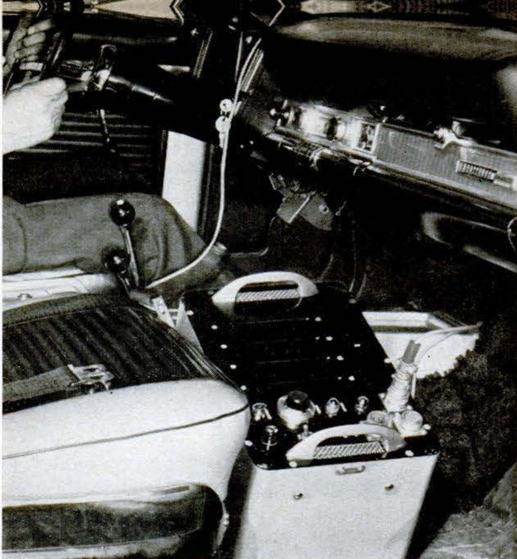
Brain-box for braking test turns on ready light at 60 m.p.h. When brake is applied, stoplight switch on brake starts electronic counter, which runs until car stops.
