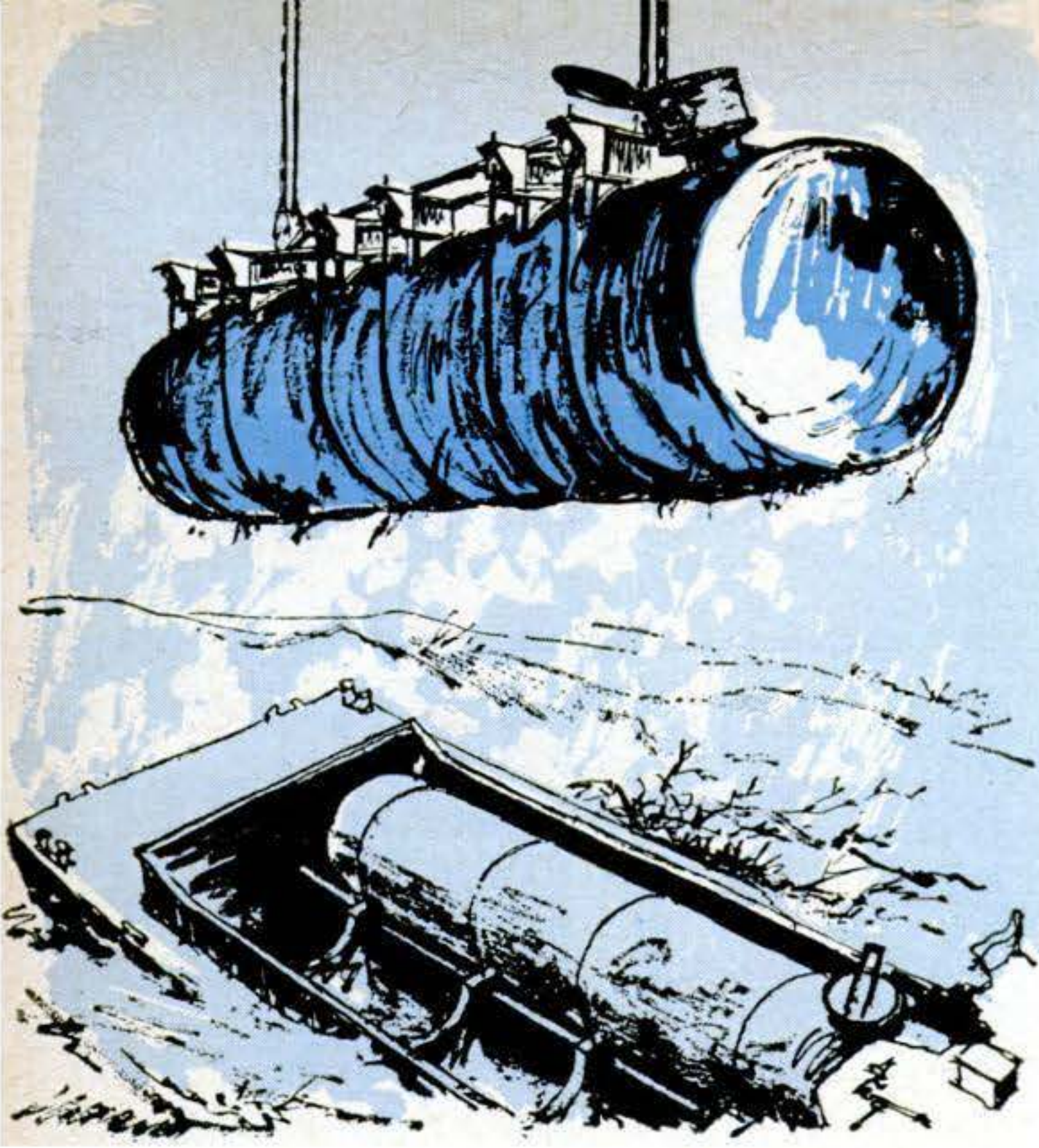
Strongback , a 30-ton strait jacket lashed to the tank, was lifted gingerly. Critical moment came when tank "readjusted" itself in its cables from slanting position to horizontal.
