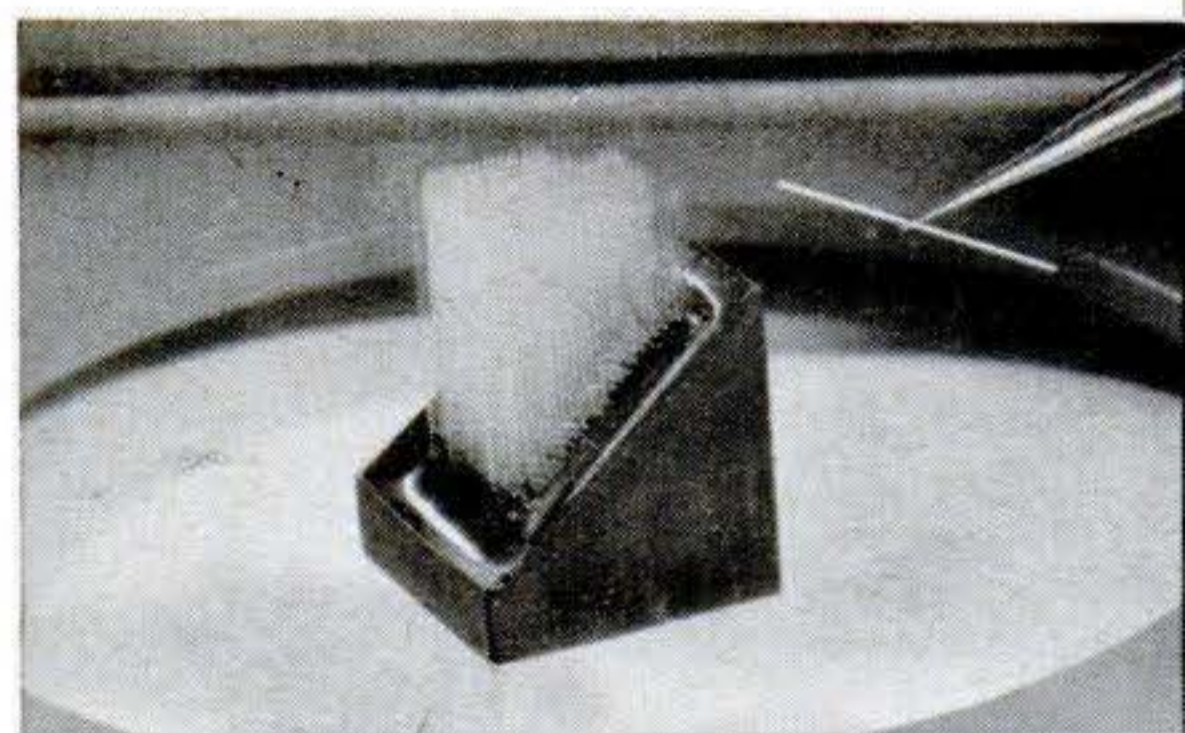
Heart of Sceptron is tuft of quartz fibers, like one held in forceps. Fibers vary in length, and different frequencies, blended in an incoming signal, make different ones vibrate.
