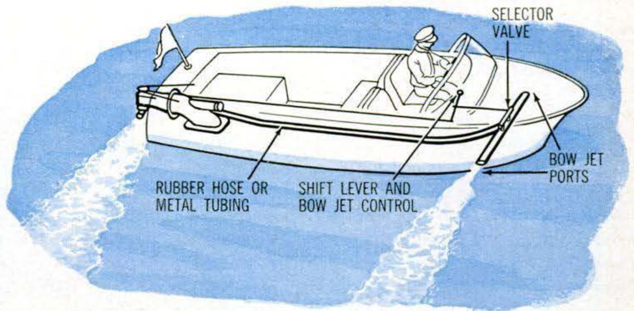
Bow steering system for low-speed maneuvering uses auxiliary jets on either side of the bow. Water under pressure is supplied through a rubber hose or metal tubing from an outlet on the side of the jet pump. Operating pressure is applied to this line when the control gate is in the reverse or neutral position.
