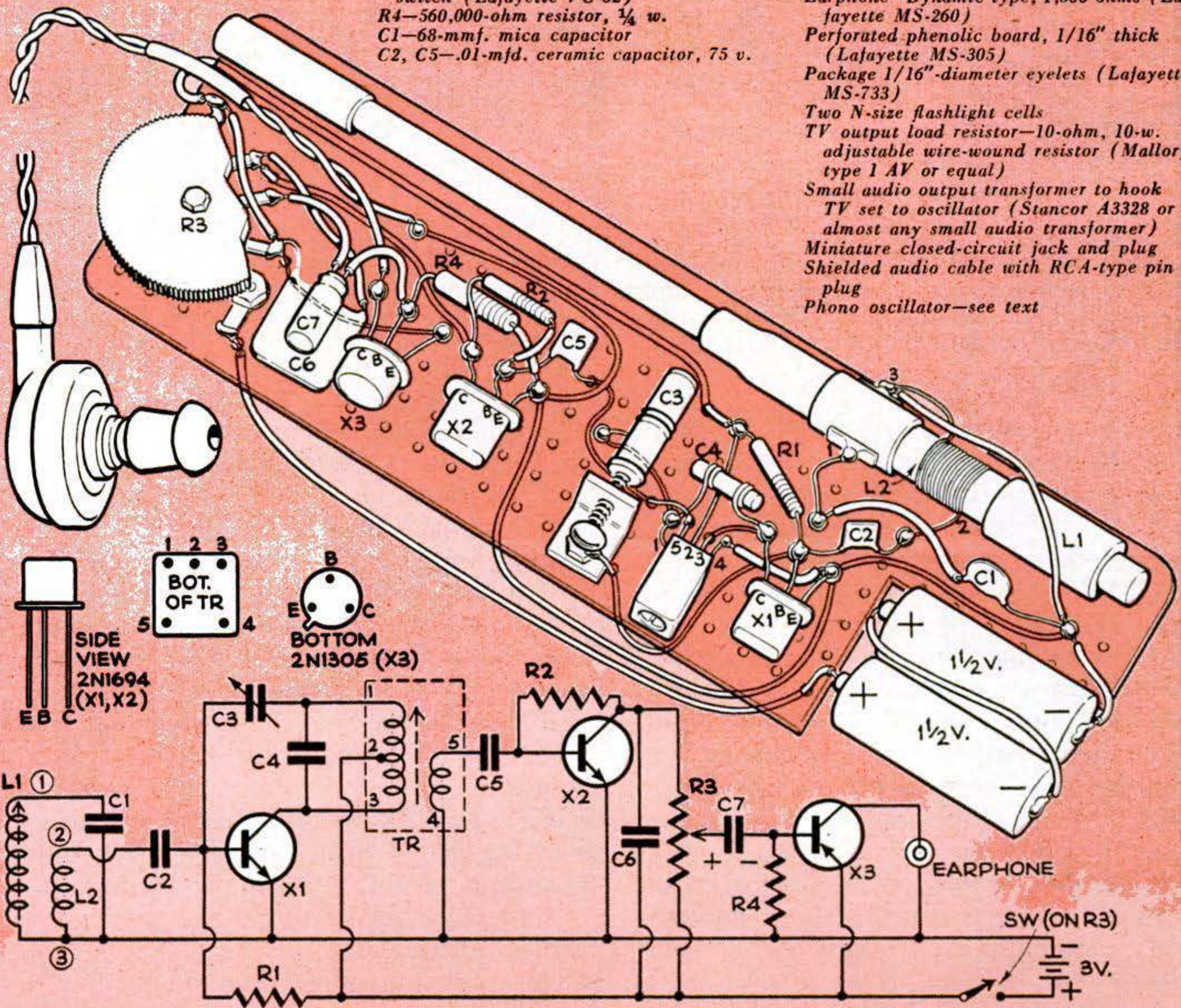
TOTAL CURRENT DRAIN—ABOUT .6 MA.
