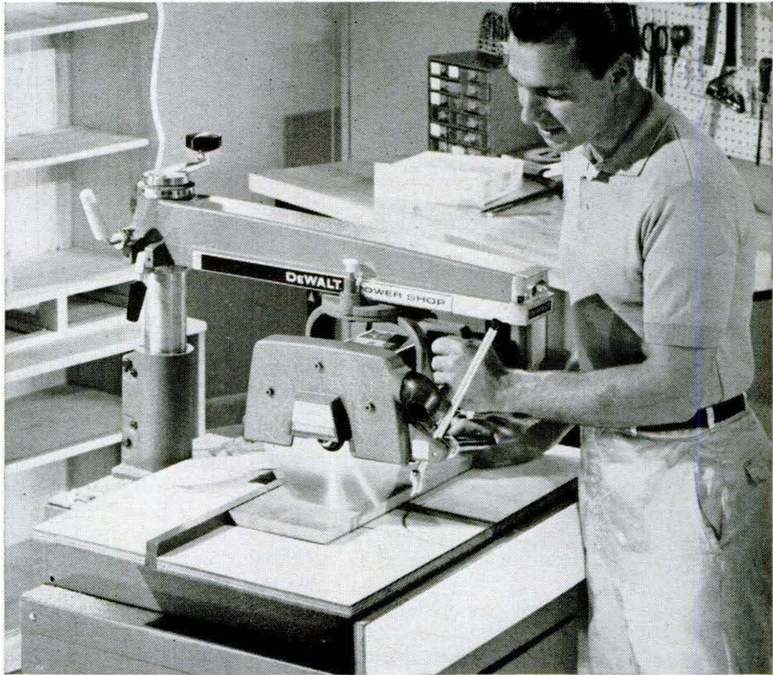
Radial Power Saw
