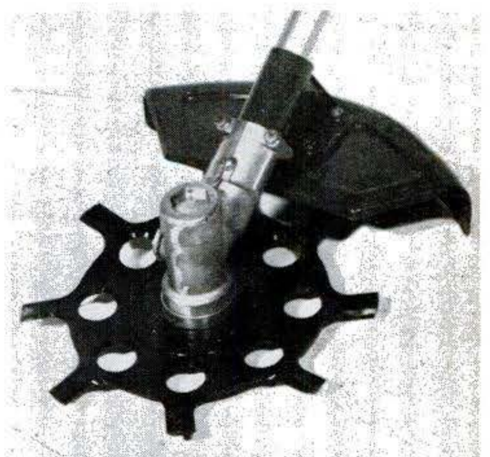
Aggressive design of flexible plastic cutter blade from John Deere enables it to handle heavy weeds and even light brush. Yet the plastic cutter head is safer than rigid steel blades for the same job.
