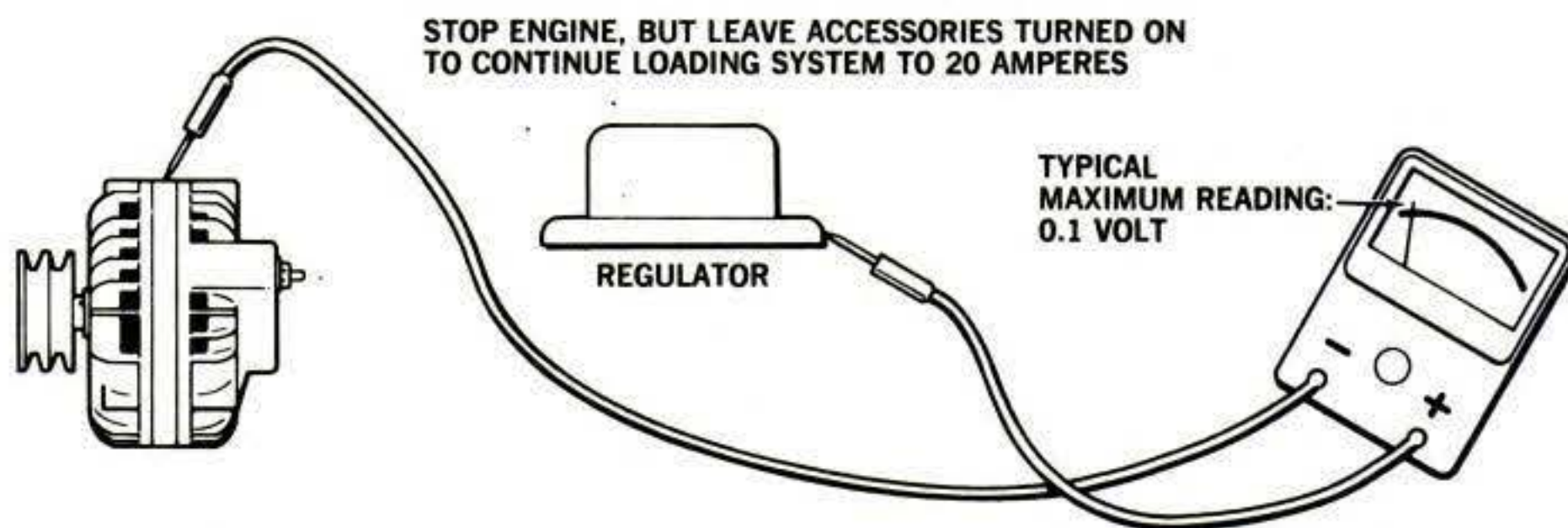
VOLTAGE DROP—ENTIRE GROUND CIRCUIT
