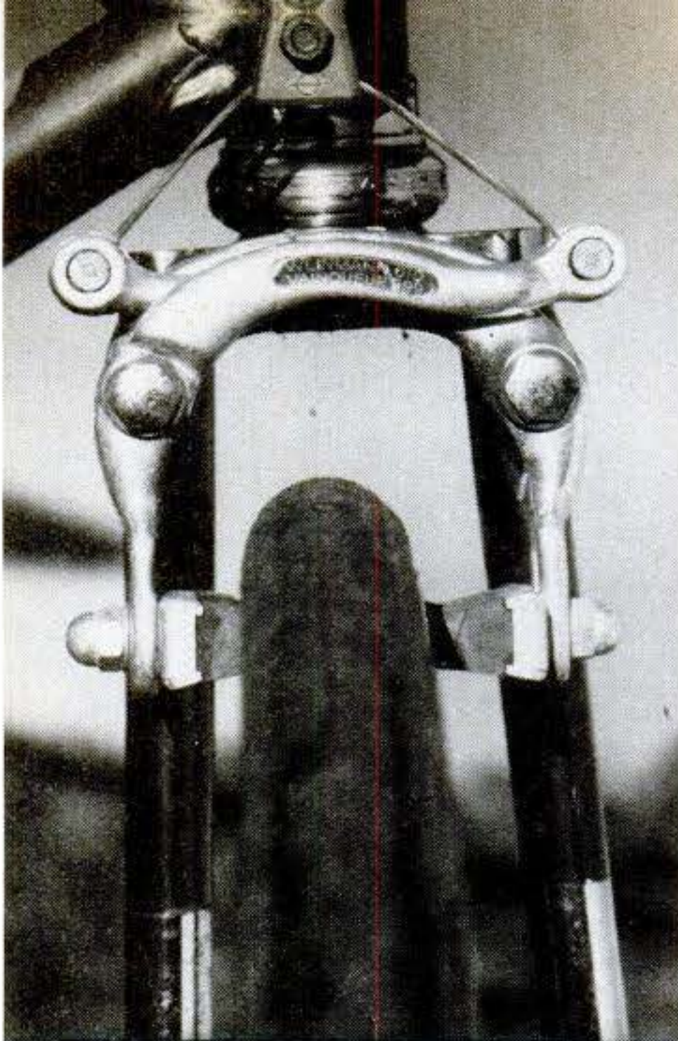
Lightweight alloy center-pull brakes are found on many low- and mid-priced 10-speeds. This type brake is easy to adjust and capable of safe, reliable stops. Brake shoe should be positioned close to rim.
