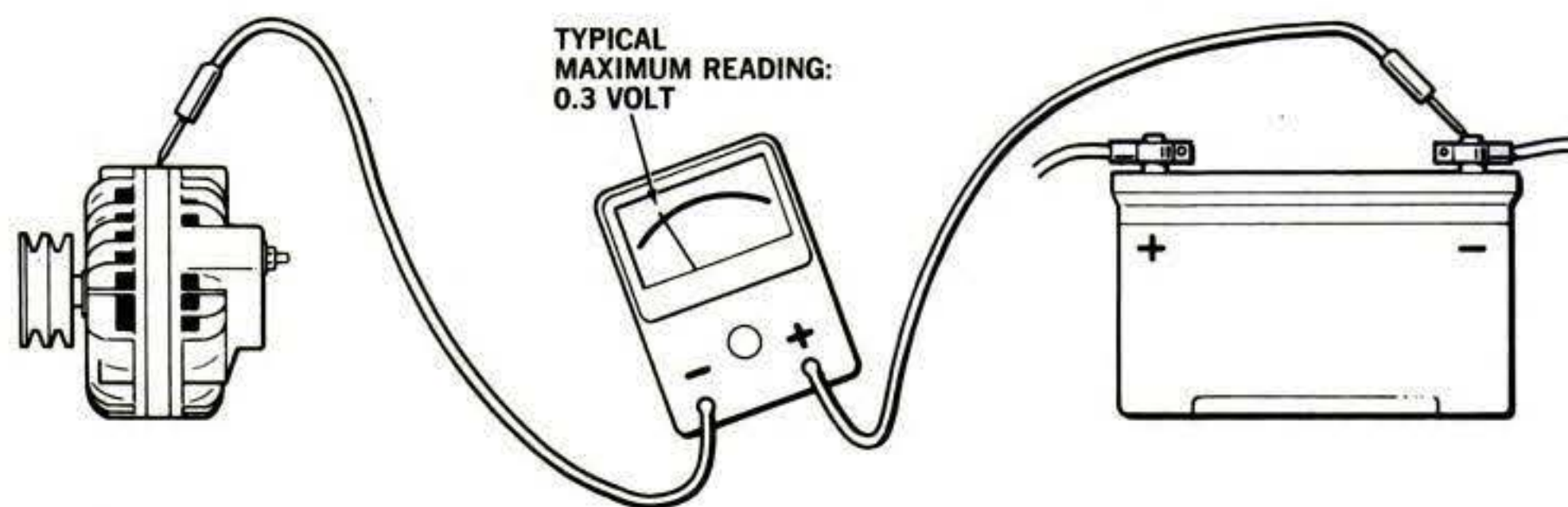
VOLTAGE DROP—GROUND CHARGING CIRCUIT
