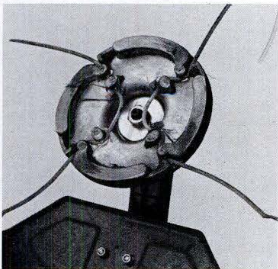
Rugged, 1/8-inch nylon line is about twice as thick as normal cutting line. Too heavy for spools, line must be clipped manually into its Toro head. Lines shown have trimmed heavy weeds for 15 minutes.
