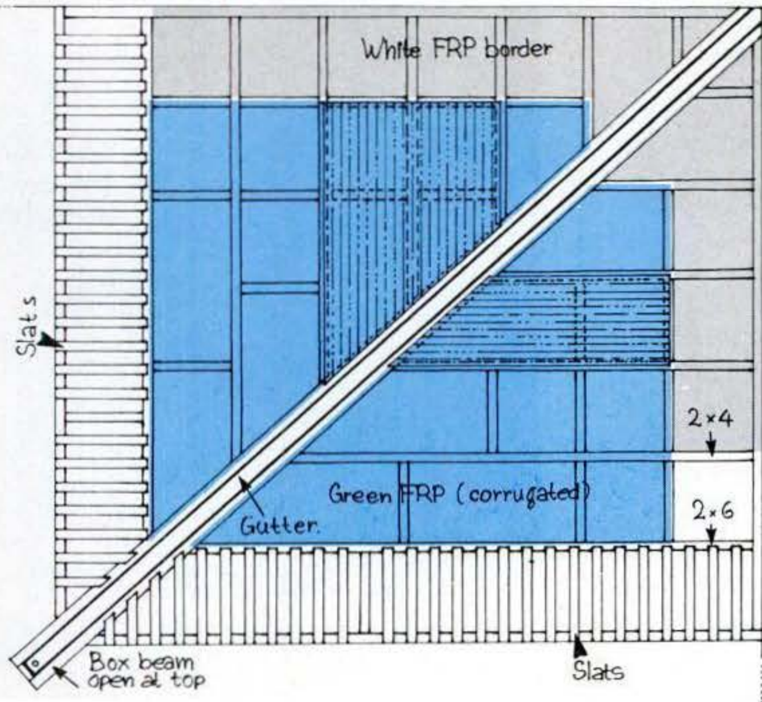
Detail of box beam and chain drain
