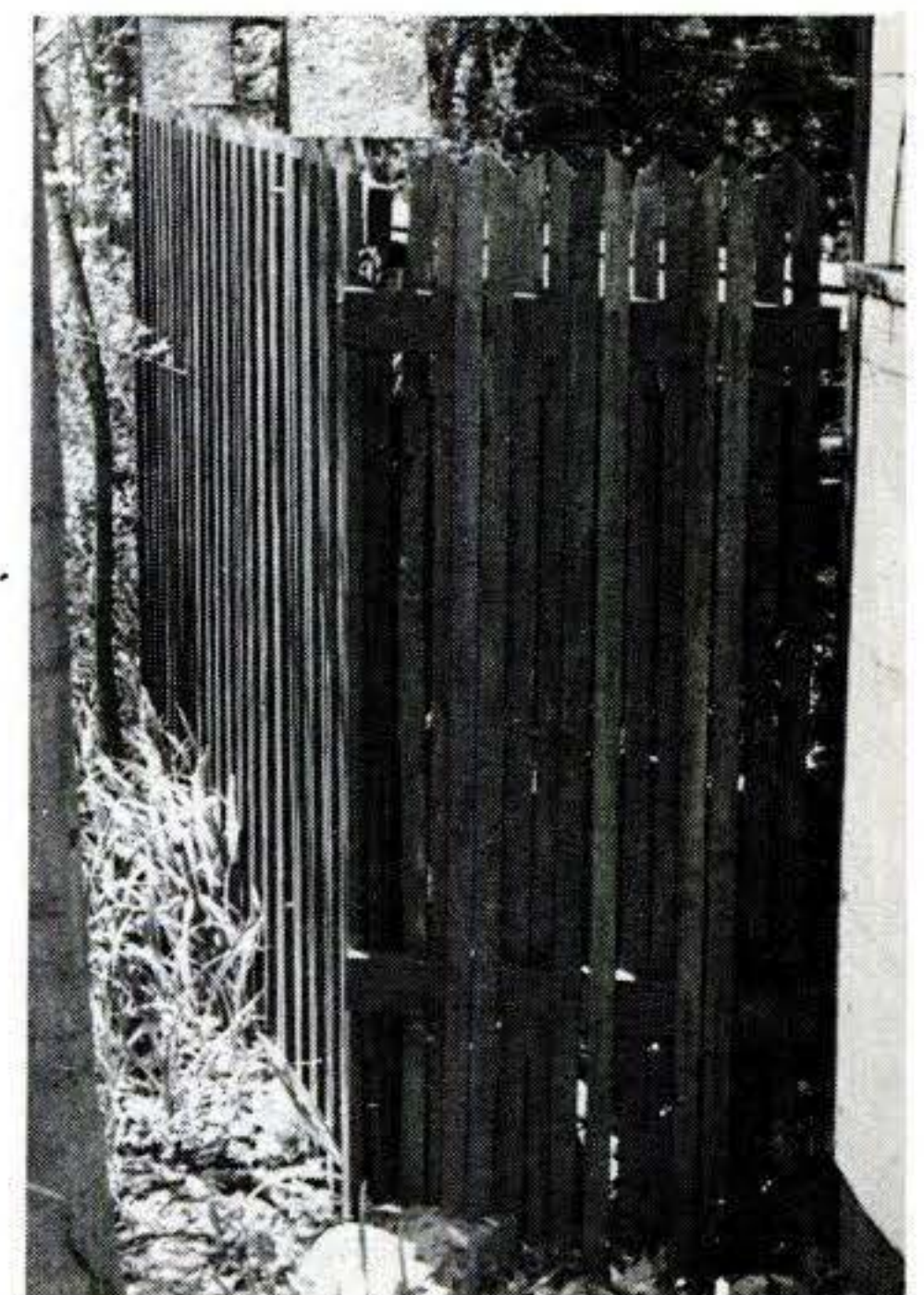
Use a level to keep slats true (top). Staggered slats provide good air circulation. Finished fence has birdhouses atop posts (above); they handily shed snow and rain.
