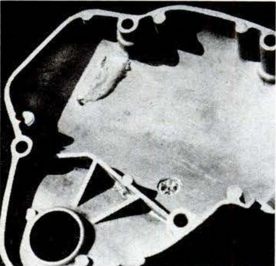
Cast-aluminum repairs should be filled and ground smooth after hardening.
