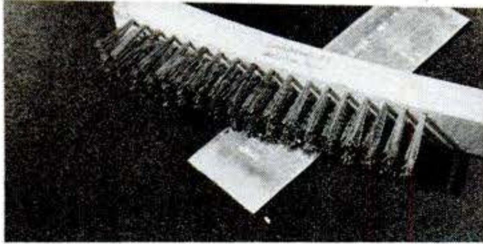
Stainless-steel wire brush is essential to the Lumiweld process, but it must be kept uncontaminated by dirt or other metals.
