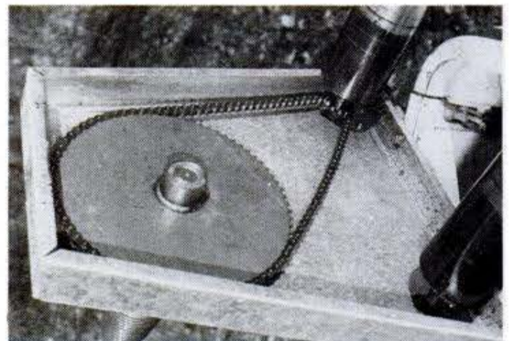
Heavy motorcycle chain transmits power from roller to screw, as this view with the cover removed shows.
