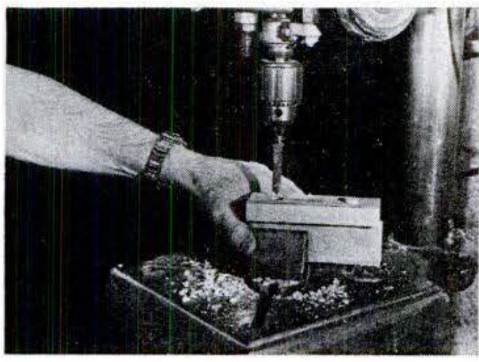
Flat bit, with upper counterbore and stop, prepares hole for dowel and sleeve.
