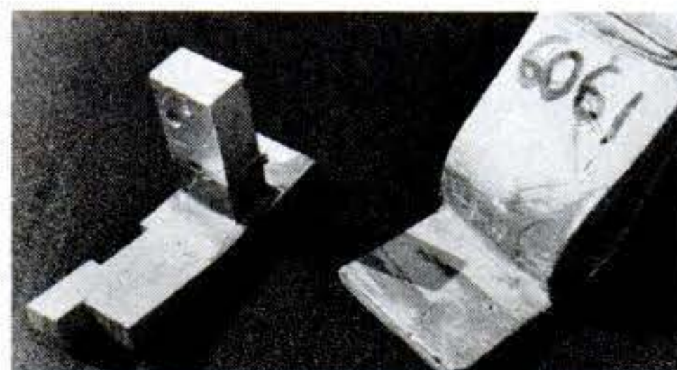
Lumiweld stands up to bend tests on heavier gauges, too. Oxygen-assisted torch may be needed to bring heaviest gauges up to rod-melting temperature.
