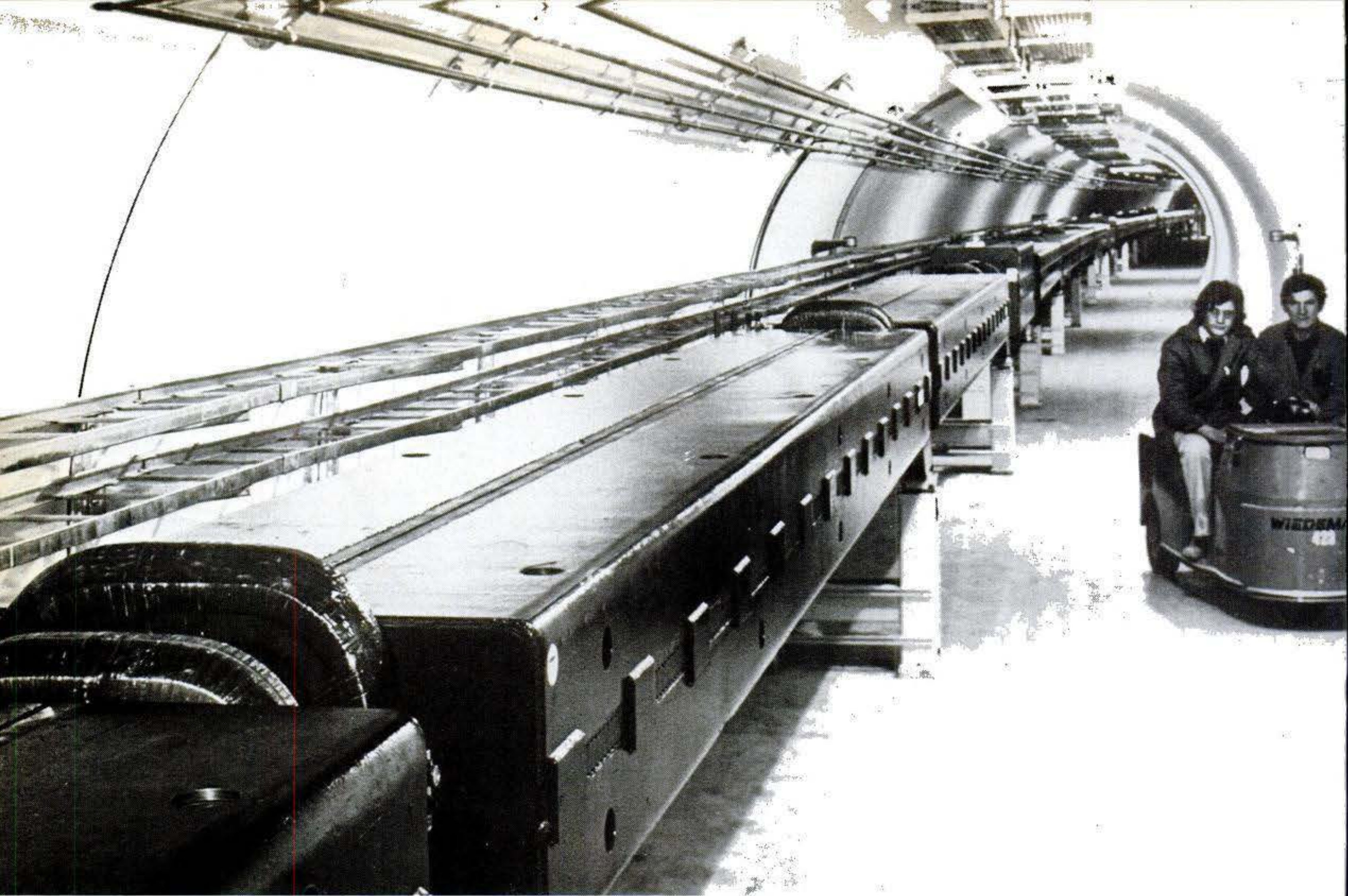
Protons and antiprotons will speed in opposite directions inside single ring in CERN tunnel that crosses national borders.
