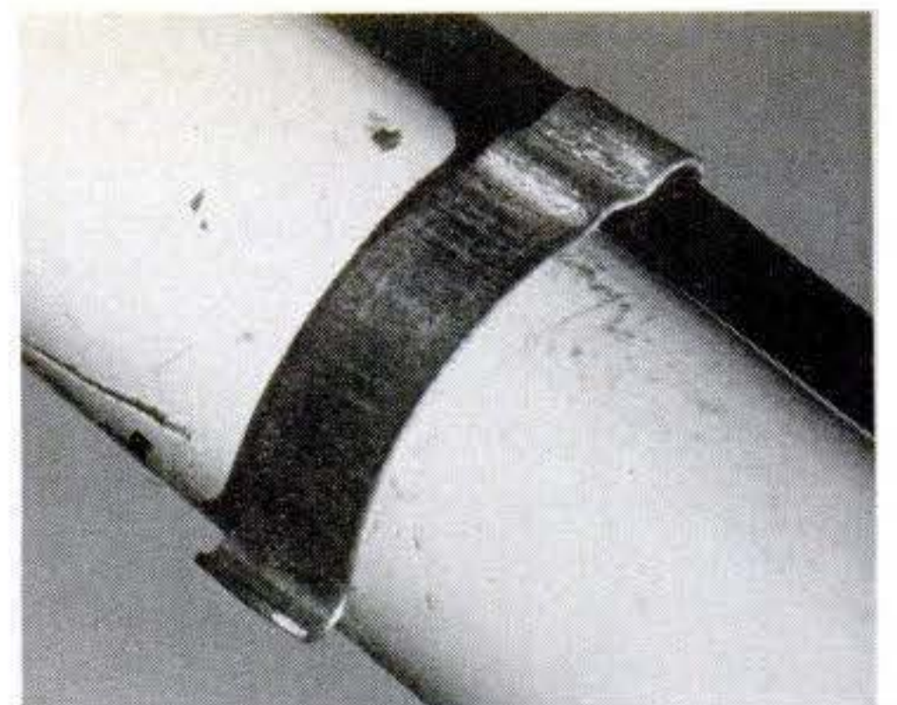
Most manufacturers use metal or plastic clips to secure brake and derailleur cables to the bicycle's frame. Brazed-on guides (preceding page) look neater, won't scratch the frame, or loosen.
