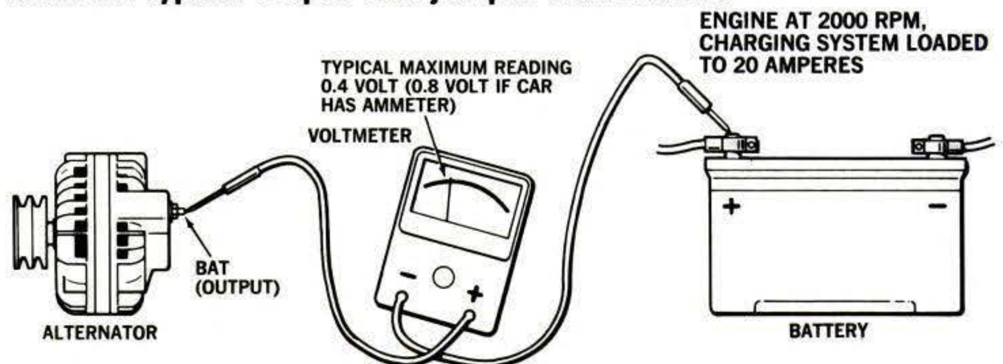
VOLTAGE DROP—INSULATED CHARGING CIRCUIT
