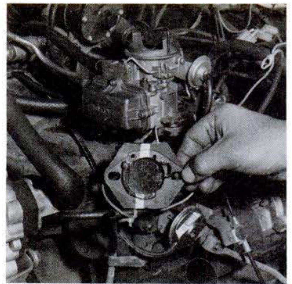
Electric grid between car's carburetor and intake manifold provides extra heat to improve methanol vaporization.
