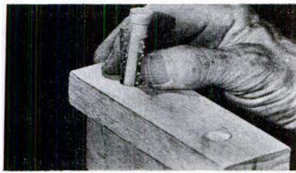
Gripper strip is folded and dropped in, followed by dowel, which drives in snugly.
