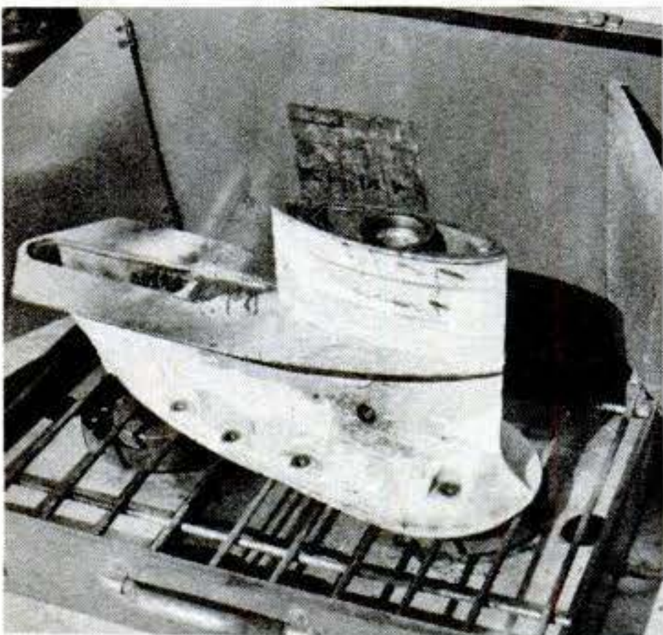
To use Lumiweld on larger castings , the home craftsman needs a propane camp stove or other heat source to help keep the work up to melting temperature of rods.
