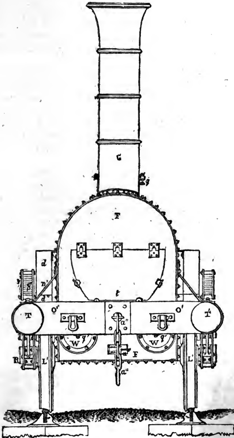
ELEVATION OF THE FOREMOST END OF A LOCOMOTIVE ENGINE.
