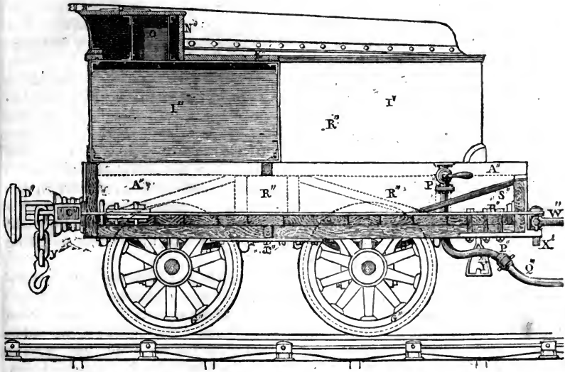
LONGITUDINAL VERTICAL SECTION OF THE TENDER.
