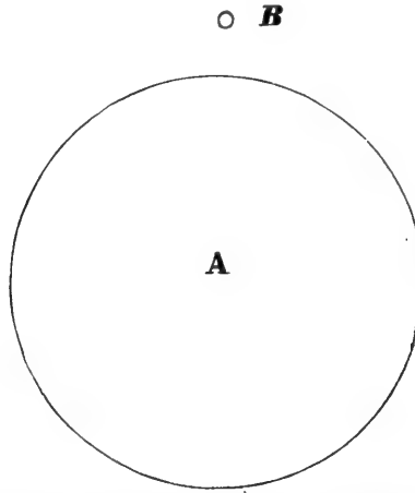
A—SIZE OF EARTH WHEN IN THE NEBULOUS PERIOD, COMPARED WITH ITS PRESENT DIAMETER, AS SHOWN BY B.
