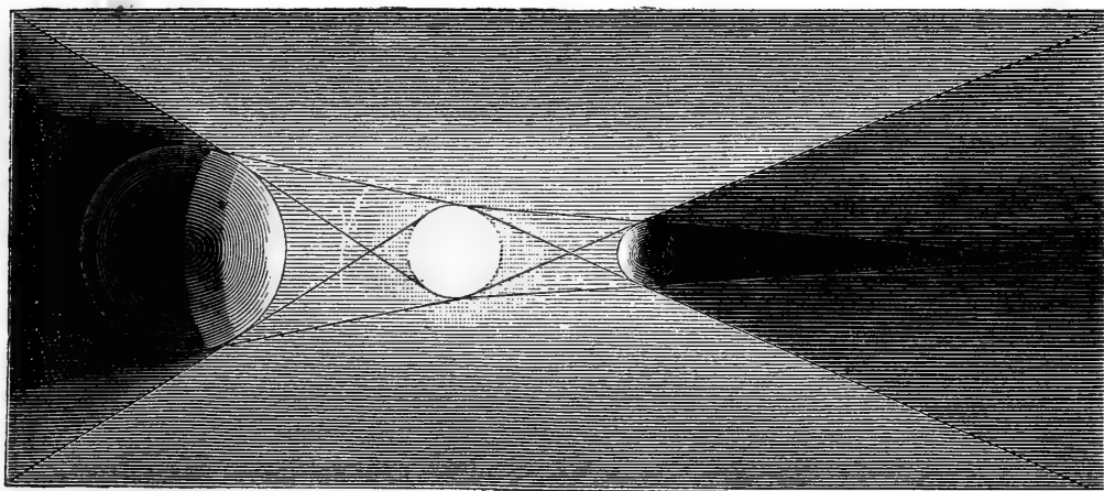
UMBRA AND PENUMBRA.
