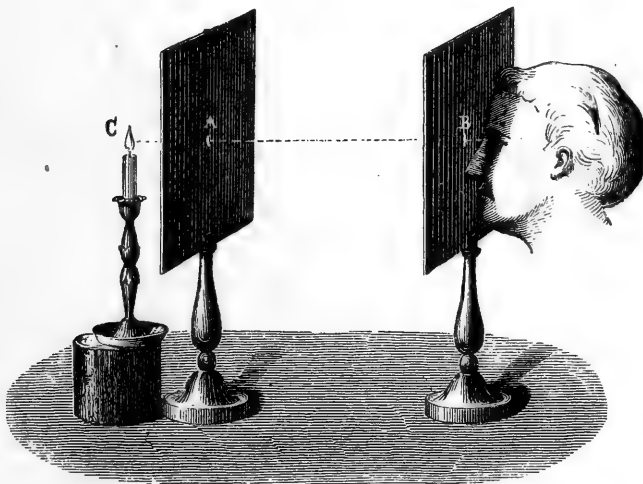
RECTILINEAR PROPAGATION OF LIGHT.
