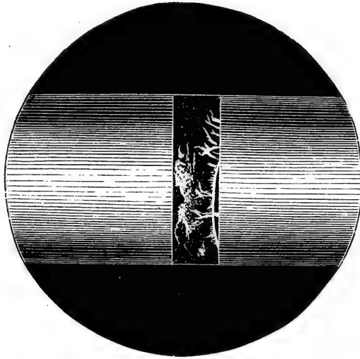
SPECTROSCOPIC ASPECT OF A PROMINENCE.
