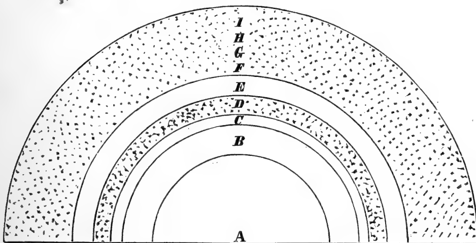
ZONES IN THE EARTH AND ATMOSPHERE.
