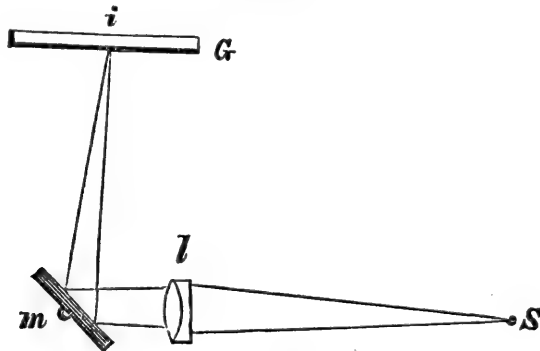
REVOLVING-MIRROR ARRANGEMENT.
