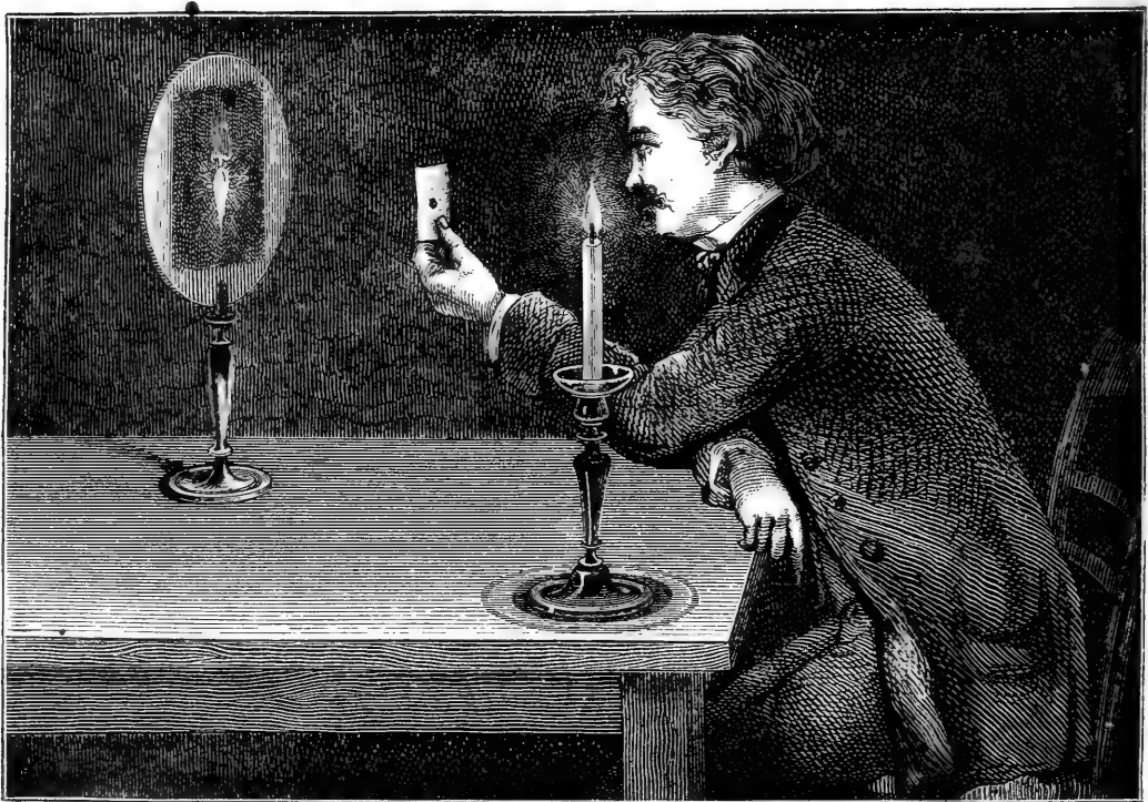
IMAGE FORMED BY A HOLE IN A CARD.
