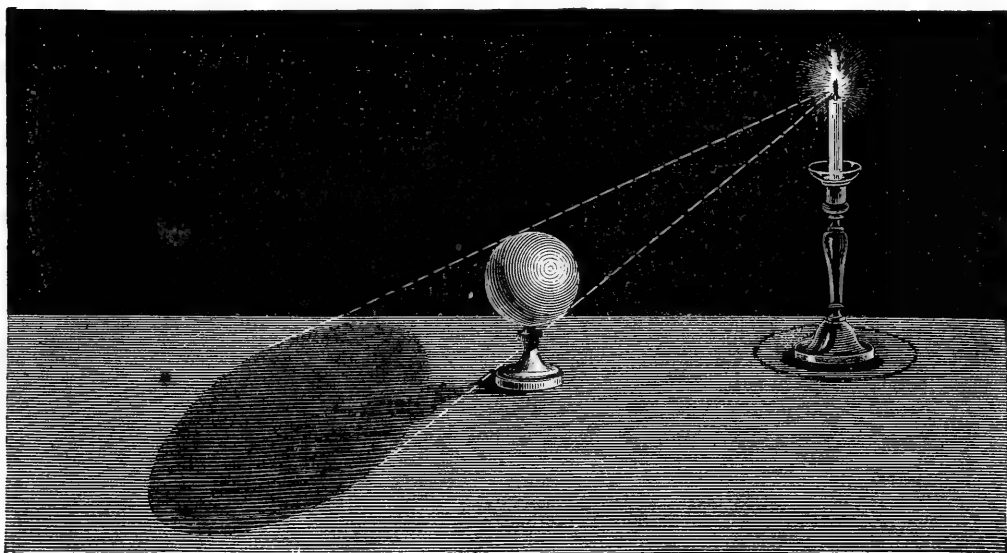
FORMATION OF A SHADOW.
