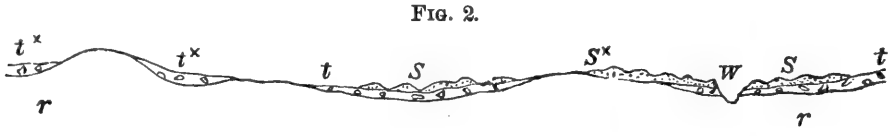
DIAGRAMMATIC SECTION, SHOWING RELATIVE POSITION OF TILL tt^x AND OVERLYING SAND AND GRAVEL SERIES SS^x . W . = RIVER VALLEY.
