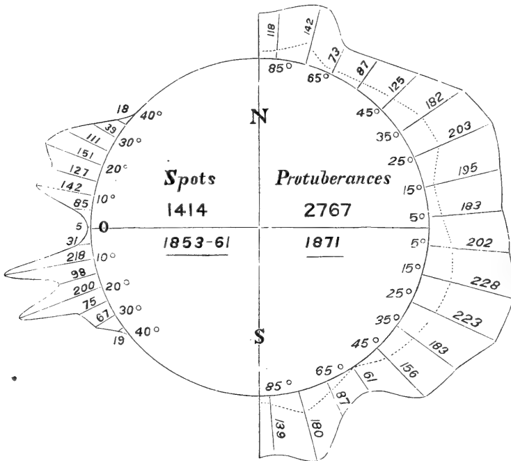
RELATIVE FREQUENCY OF PROTUBERANCES AND SUN-SPOTS.
