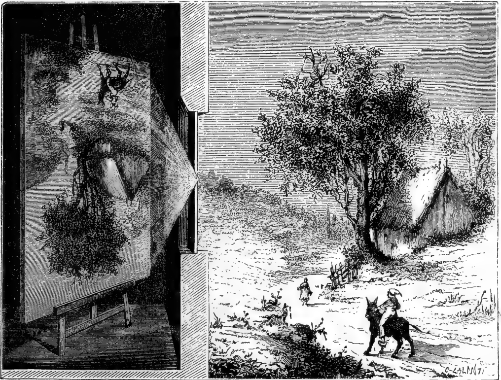
INVERTED IMAGE OF LANDSCAPE.
