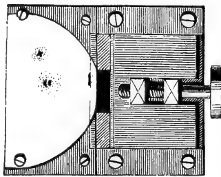
OPENED SLIT OF THE SPECTROSCOPE.
