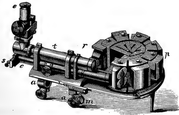
SPECTROSCOPE, WITH TRAIN OF PRISMS.
