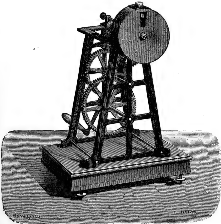
BECQUEREL'S PHOSPHOSCOPE.
