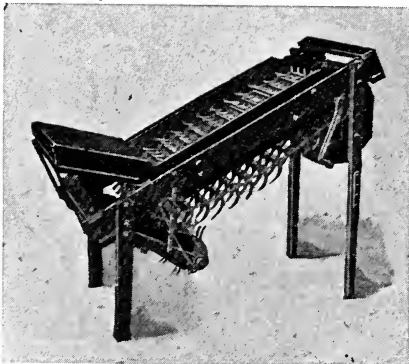
Fig. 29. A potato-sorter (courtesy of Aspinwall Canadian Machinery Company).
