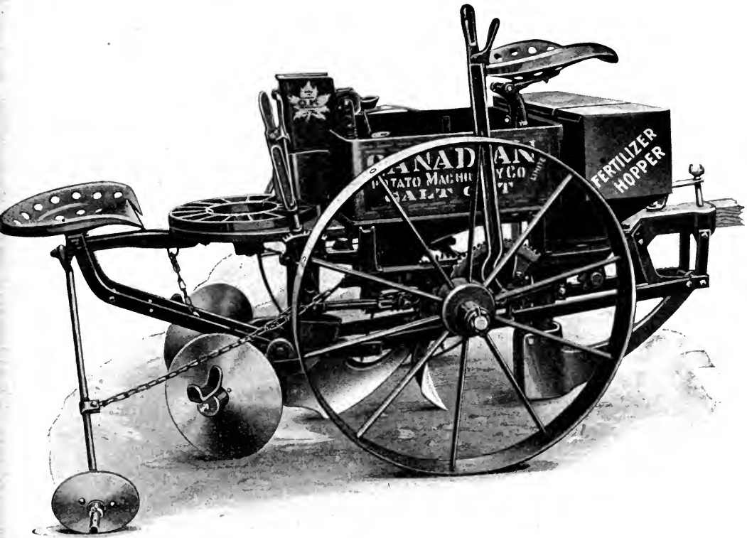
Fig. 21. A two-man type of planter.
