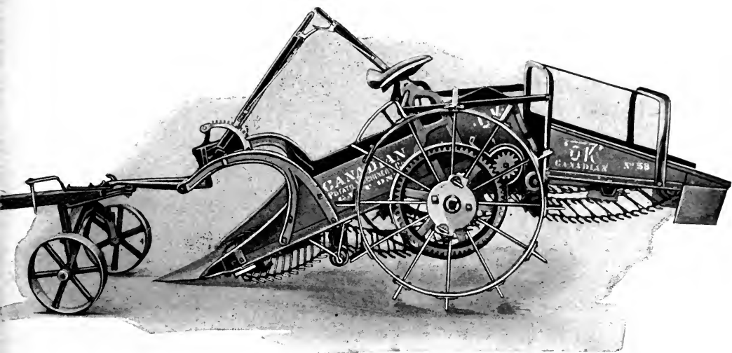
Fig. 26. Side view of a steel-nose potato-digger.
