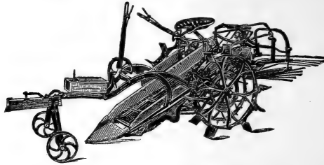
FIG. 44—THE HOOVER DIGGER
