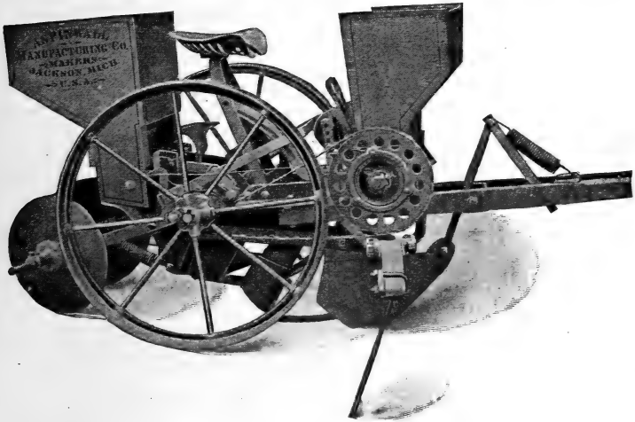
FIG. 27—ASPINWALL POTATO PLANTER (SIDE VIEW)
