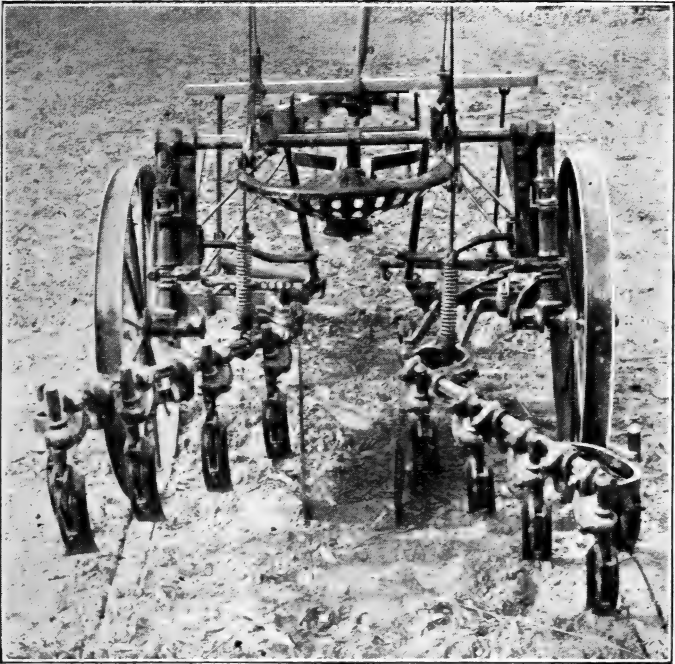
FIG. 32—A USEFUL TWO-HORSE CULTIVATOR A requisite wherever large areas of potatoes are grown.
