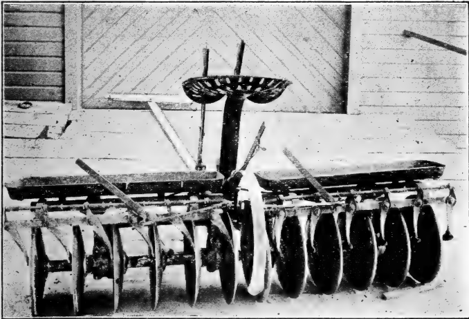
FIG. 8.—AN EFFICIENT PULVERIZER; THE DISK HARROW
