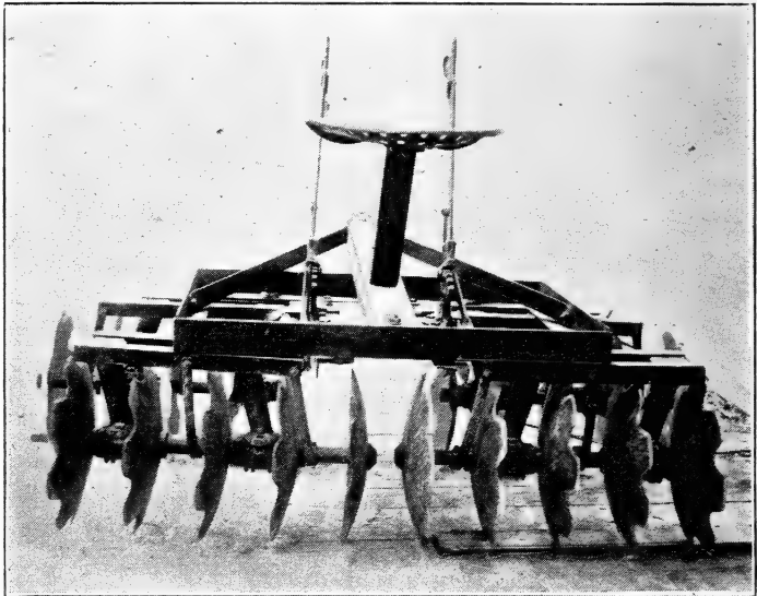
FIG. 9—DOUBLE-ACTION CUTAWAY HARROW
