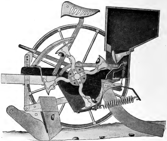
FIG. 26—SECTIONAL VIEW OF ASPINWALL PLANTER
