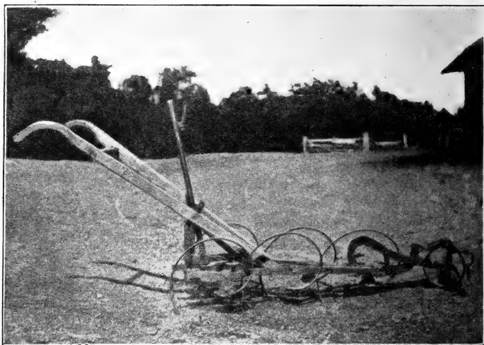
FIG. 33—ONE-HORSE SPRING-TOOTH CULTIVATOR An excellent tool for the later cultivations.
