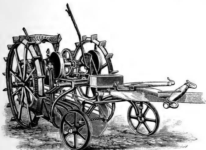
FIG. 43—THE REUTHER POTATO DIGGER
