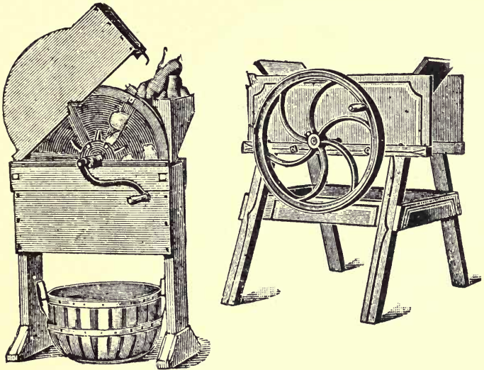
FIGS 36—37: ROOT CUTTERS
