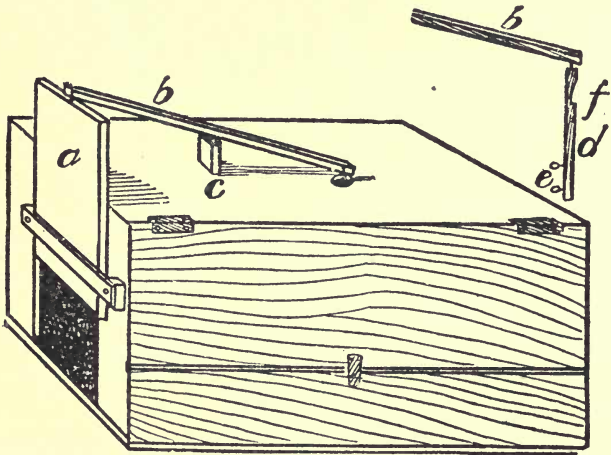
FIG 92: SKUNK TRAP
