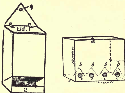
FIGS 8—9: AUTOMATIC FEEDERS
