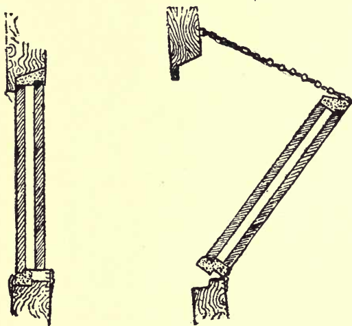
FIG 61: DOUBLE WINDOWS
