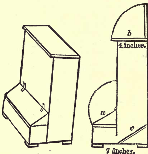
FIG 5: FEEDING HOPPER
