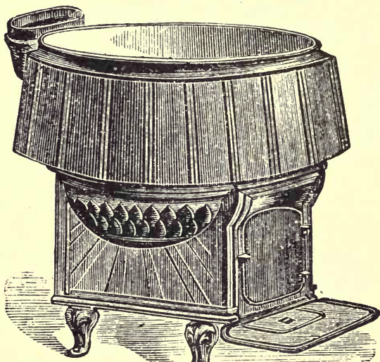
FIG 107: FEED COOKER
