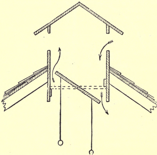
FIG 97: GOOD VENTILATION
