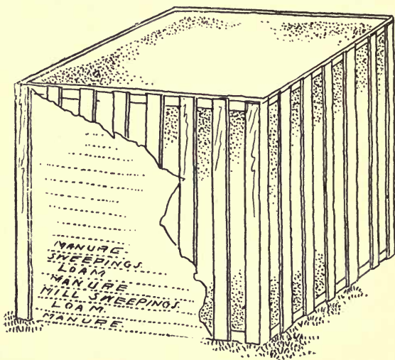
FIG 109: WORM BOX
