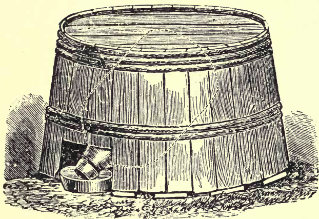
FIG 23: NON-FREEZING FOUNTAIN
