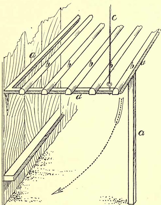
FIG 42: IMPROVED ROOST
