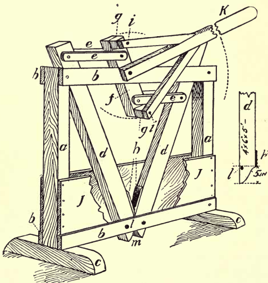
FIG 41: GRIT MILL
