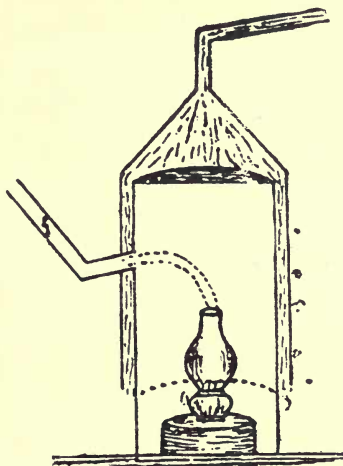
FIG 106: LAMP HEATER
