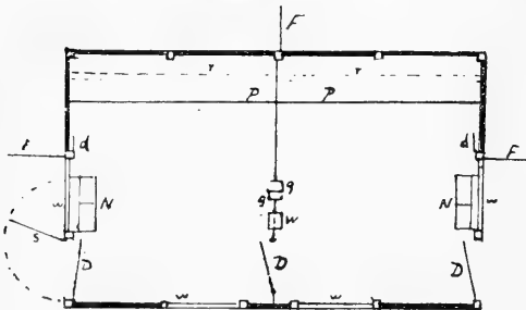
Fig. 7. Two-Pen Poultry House. P P, droppings boards; r r, roosts; N N, nests; D D, large doors; d d, small doors; w w, windows; W, water dish; g g, grit box; s, screen door; F F, fences.
