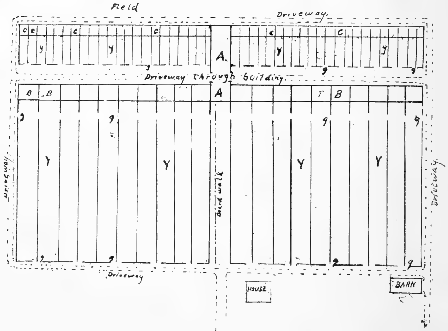
Fig. 23. Plat of Plant Arranged so that Work may all be done Under Cover in Stormy Weather.—A, central building; B B, laying houses; C C, brooder or brooder and surplus stock houses; Y y, yards; gg, gates.
