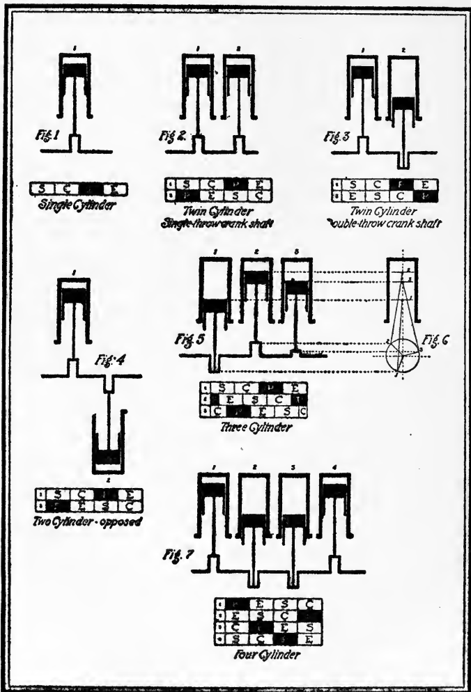
Types of crankshaft
