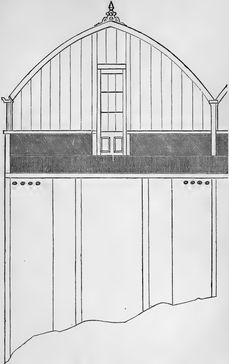
Fig. 45.—END VIEW AND PLAN OF ROSE-HOUSE.
