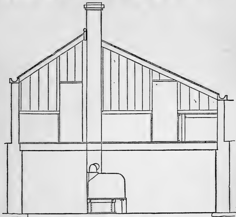
Fig. 16.—END VIEW OF FORCING HOUSE.
