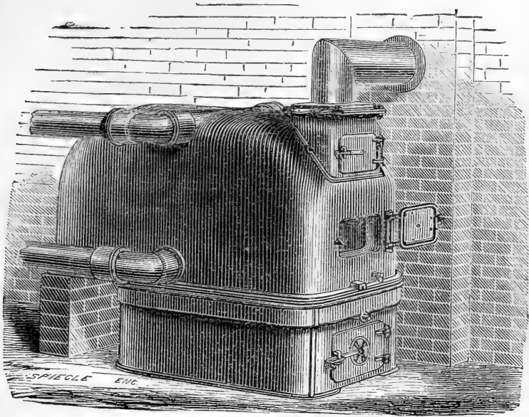
A.—Elevation of Boiler.
