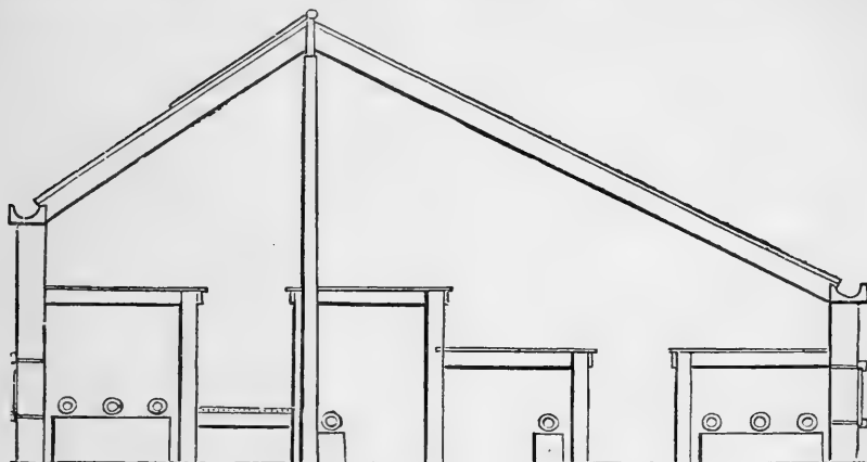
Fig. 19.—INTERIOR OF FORCING HOUSE.
