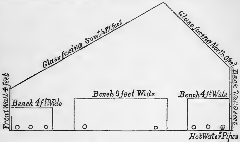
Fig. 44.—END SECTION OF ROSE-HOUSE.
