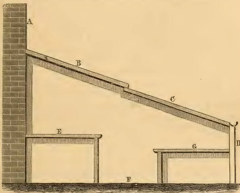
Fig. 20.—SECTION OF A CHEAP GREENHOUSE.
