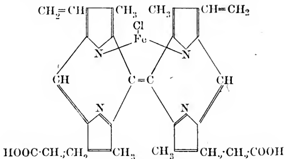
Haemin, C_{27}H_{30}N_4O_4FeCl .
