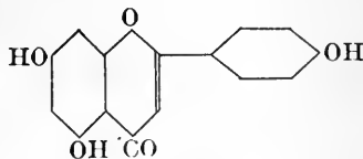
Apigenin or 1, 3, 4'-trihydroxy- flavone.
