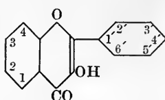
Flavonol or hydroxyflavone.
