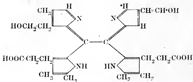
Haematoporphyrin, C_{33}H_{28}O_6N_4 .
