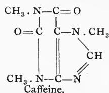
or 1, 3, 7-trimethylxanthine.
