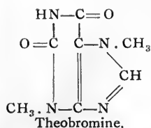
or 3, 7-dimethylxanthine.
