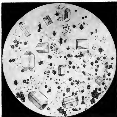
FIG. 82.—Deposit of triple phosphate (am. mag. phosphate) and ammonium urate. (After Funke.)
