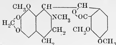
Narcotine.
