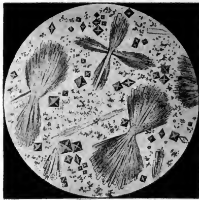
FIG. 83.—Deposit of uric acid, sodium urate and calcium oxalate. (After Funke.)
