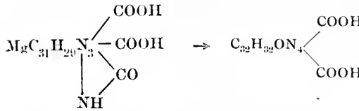
Isochlorophyllin a .
