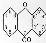
Xanthone.
