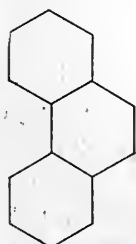
Phenanthrene.
