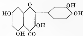
Quercetin or 1, 3, 3', 4'-tetrahydroxy- flavonol.
