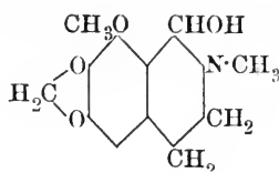
Cotarnine.
