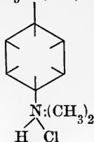
Colourless leuco base.
