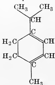
\alpha -Terpinene
