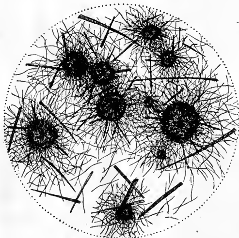
FIG. 40.—Lactosazone.
