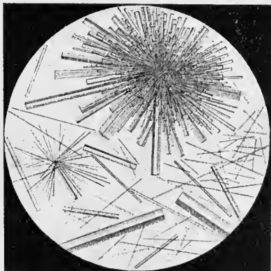
FIG. 53.—Glycocholic acid. (After Funke.)
