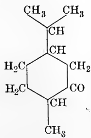
Carvomenthone.
