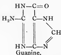
or 2-amino, 6-oxy-purine.
