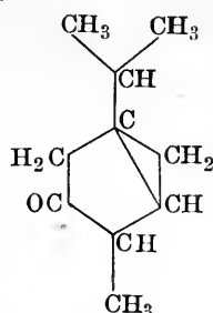
Thujone.
