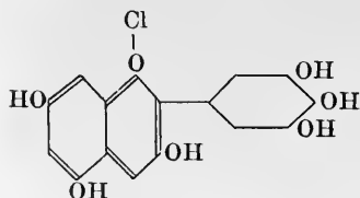
Delphinidin.
