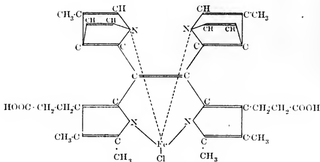
Haemin, C_{33}H_{32}O_4N_4FeCl .
