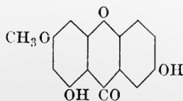
Gentisin or 4-methoxy- 2, 3'-dihydroxy- xanthone.
