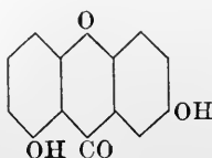
Euxanthone or 2, 3'-dihydroxy- xanthone.
