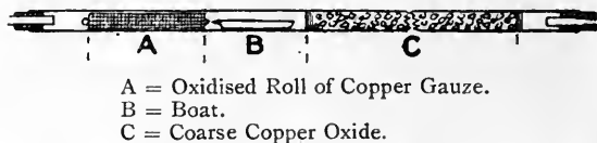
FIG. 16.—From Price and Twiss' "Practical Organic Chemistry".
