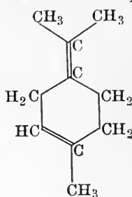
Terpinolene, not natural.
