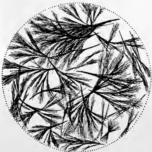
FIG. 39.—Glucosazone.
