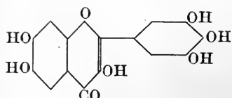
Myricetin or 1, 3, 3', 4', 5'- pentahydroxy-flavonol.
