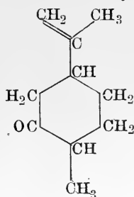
Dihydrocarvone.
