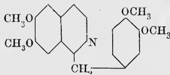
Papaverine or tetramethoxybenzylisoquinoline.
