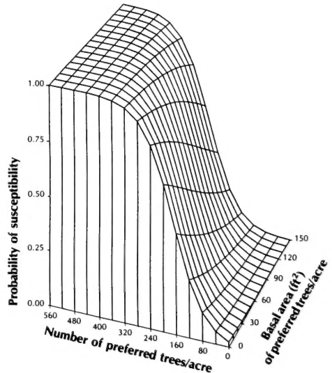
FIGURE 1. Plot of the logistic regression equation used to predict the susceptibility of forest stands to gypsy moth defoliation.
