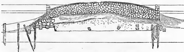
Section of a Crannoge in Ardakillin Lough, Roscommon.
