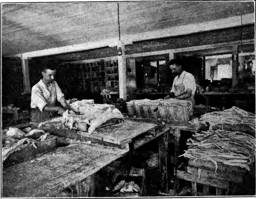
FIG. 2.—Cutting fish for tablets or fish cakes. (The miter box is used by one cutter and the slitted table top by the other.)
