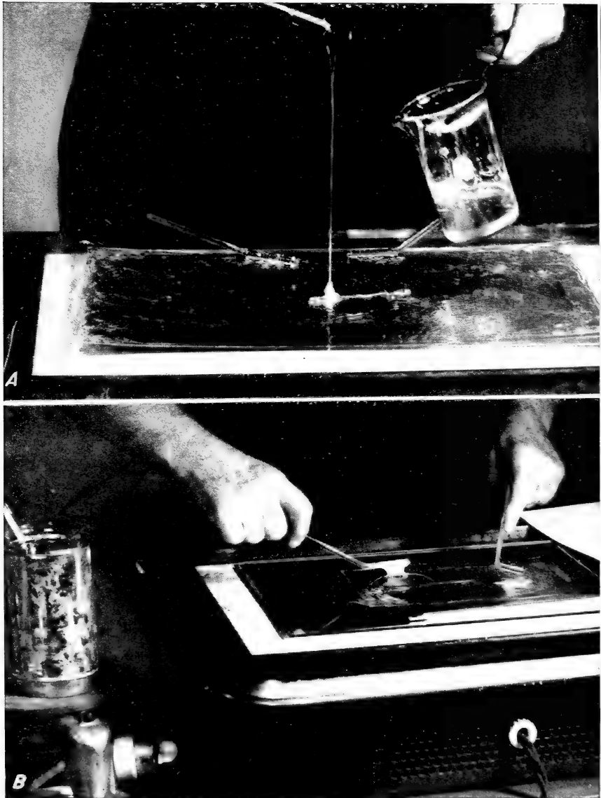
FIGURE 8. The thermoplastic cementing resin, previously heated to 110^{\circ} C. ( 230^{\circ} F.), is applied while fluid (A); it is then spread over the surface of the mount with a glass rod bent like a hockey stick (B).
