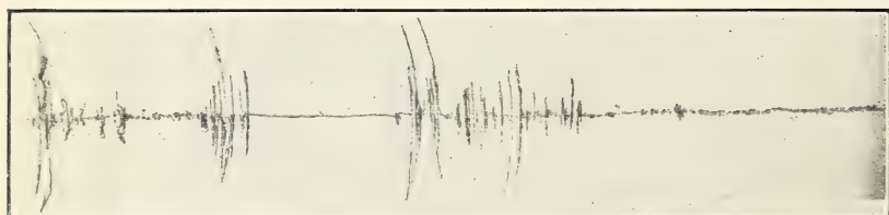
FIG. 3.—YARD SHIFTING.
