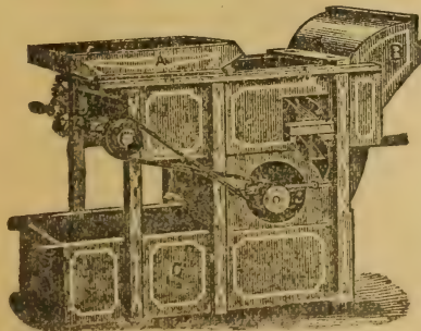
a, Hopper; b, Dust Spout; c, Grain or Seed Box. Weight, 150 lbs. Price, $2.50.
