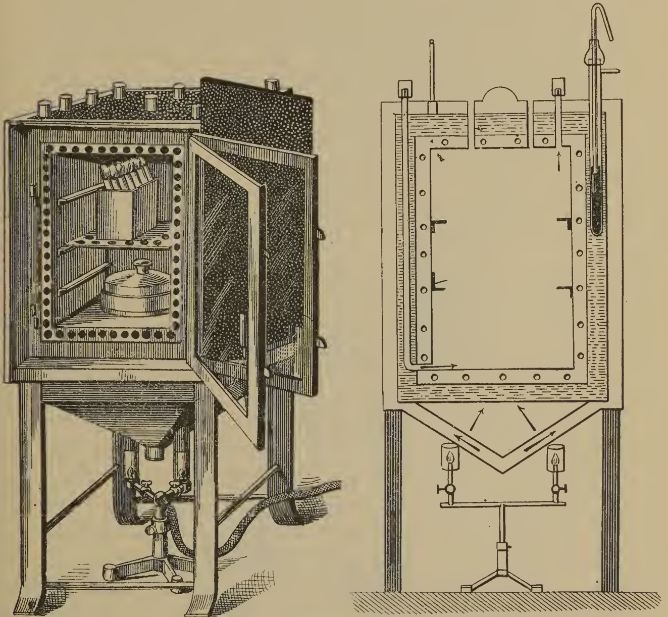
Incubator used in bacteriological work.
