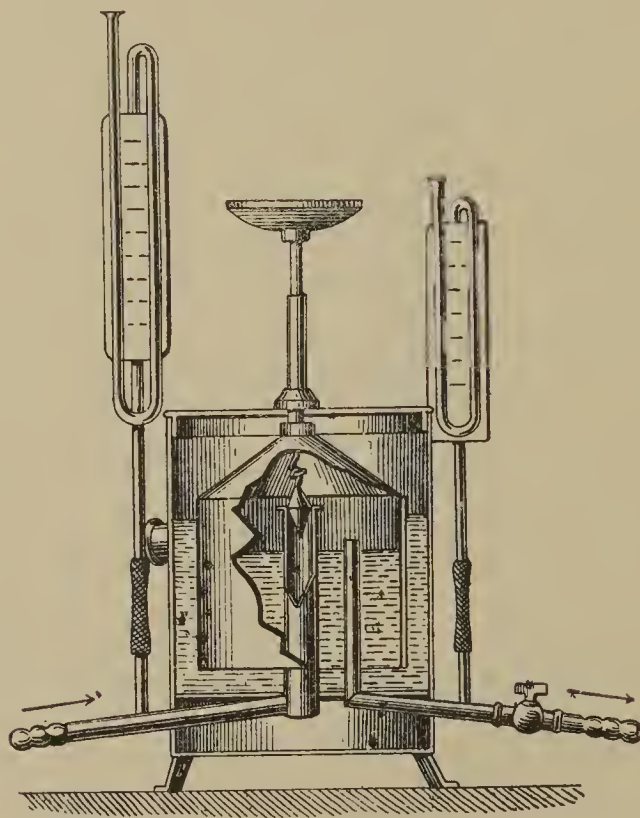
Moitessier's gas-pressure regulator.
