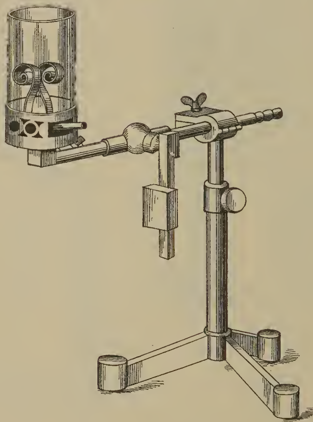
Koch's safety burner.
