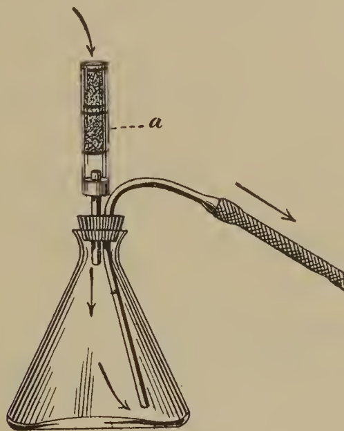
Petri's apparatus for bacteriological analysis of air. The tube packed with sand is seen at the point a .
