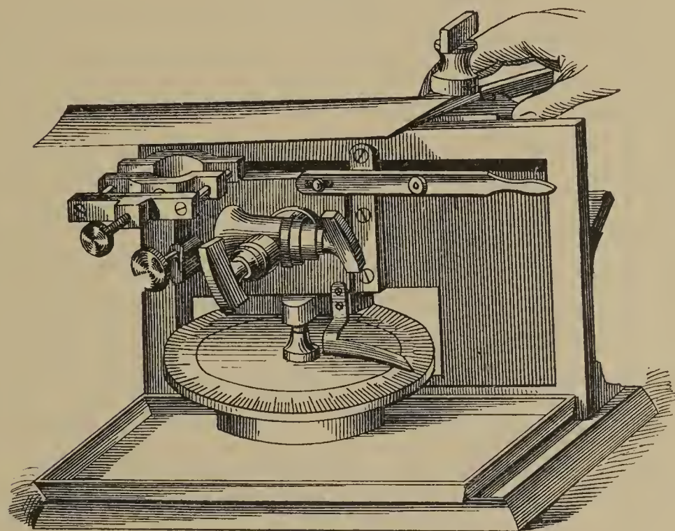
Schanze's microtome.
