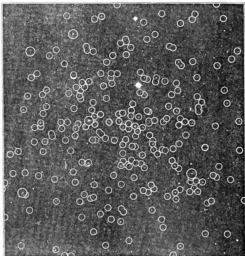
FIG. 2. Region of many small nebulae at 12^{\text{h}} 55^{\text{m}} + 28^{\circ} 30' . 249 small nebulae in an area 38' \times 30' .
