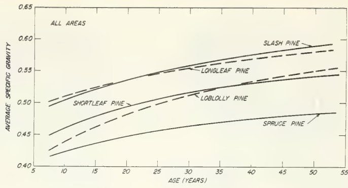
Figure 2. Relationship between age at breast height and core specific gravity for five species of pine in Mississippi.
