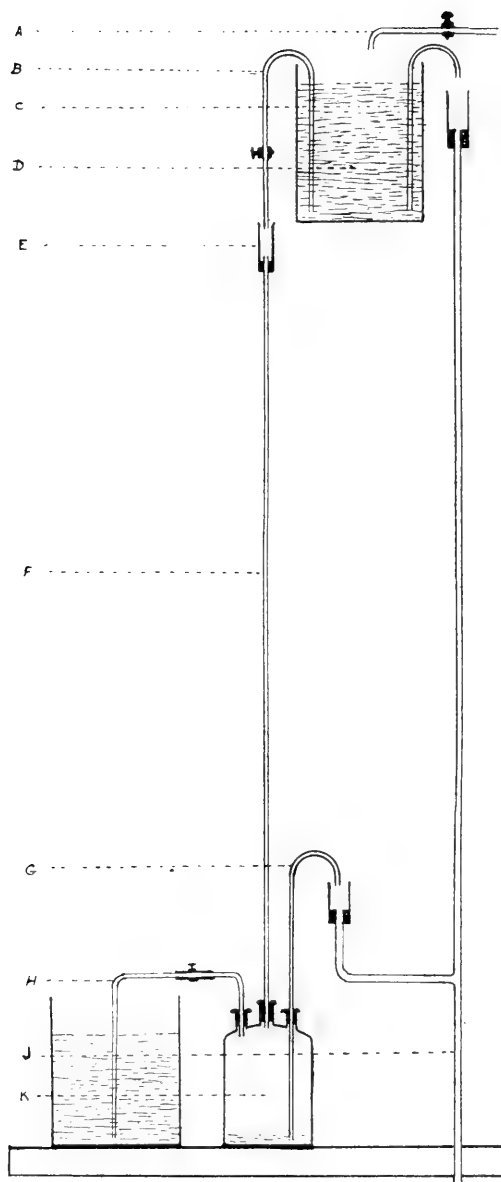
An Apparatus for Aerating Culture Solutions.
