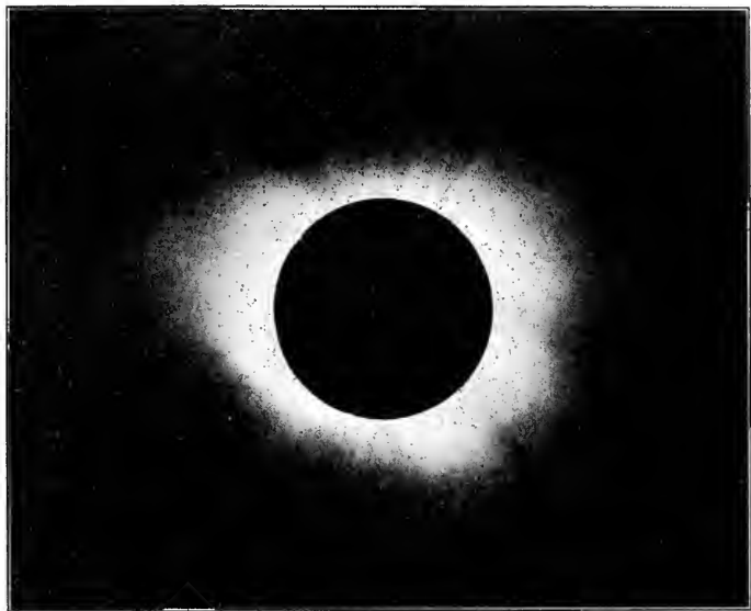
FIG. 133.—Plate No. 1. Exposure one second; 5^{\text{h}} 23^{\text{m}} 57^{\text{s}} to 5^{\text{h}} 23^{\text{m}} 58^{\text{s}} .
