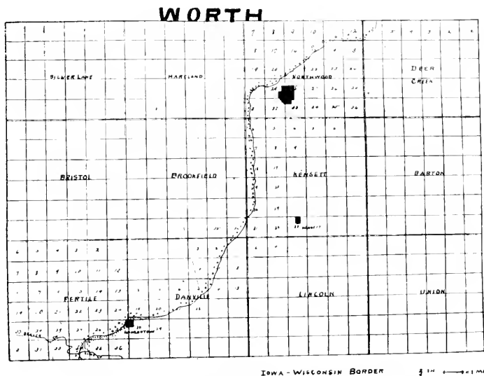
FIG. 104. Map of the Iowan-Wisconsin border in Worth county.
