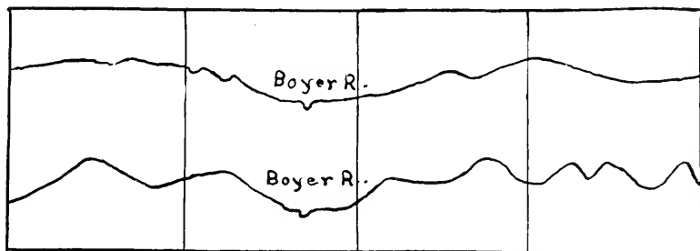
FIG. 123.—Profiles of Boyer valley. Upper profile, west of Lake View, Sac county. Lower profile, at Ells, Crawford county. Horizontal scale, one inch equals five thousand feet. Vertical scale, one-fourth inch equals one hundred thirty feet.
