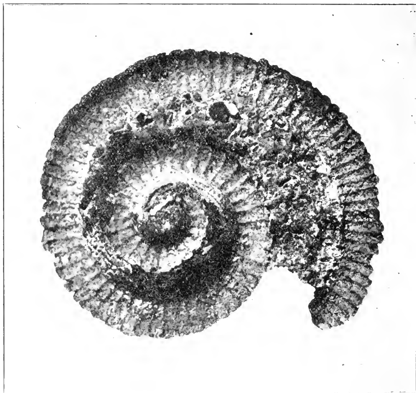
FIG. 121.—An illustration of a specimen of Salter's genus Herpetocrinus from the Niagaran dolomitic limestone near Monticello, Iowa. Total length 83 millimeters; greatest diameter across the coil, 20.6 millimeters, shortest, 16.0 millimeters. Length of the distal missing part of the stem unknown. Magnification a little more than four and one-half times.
