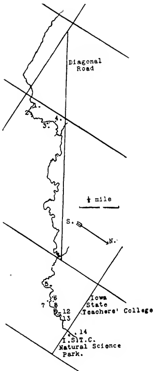
FIG. 10.—Map showing course of Dry Run for the upper three miles.
