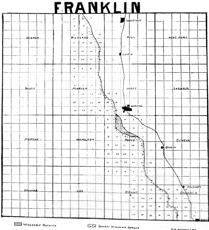
FIG. 105. Map of the Iowan-Wisconsin drift border in Franklin county.
