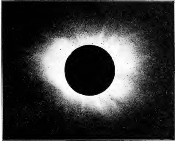
FIG. 134.—Plate No. 2. Exposure five seconds, 5^{\text{h}} 24^{\text{m}} 03^{\text{s}} to 5^{\text{h}} 24^{\text{m}} 08^{\text{s}} .
