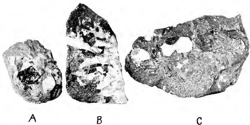
Fig. 2. Specimens illustrating the metasomatic replacement of quartz by sphalerite.
