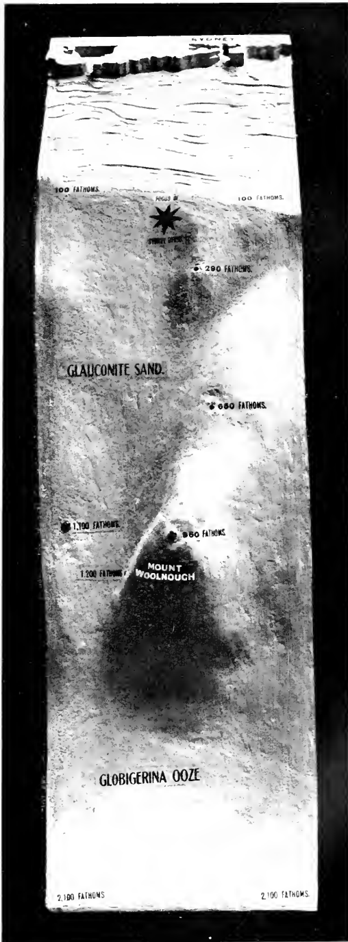
Full-face View of Model of the Submarine Slope off Sydney
