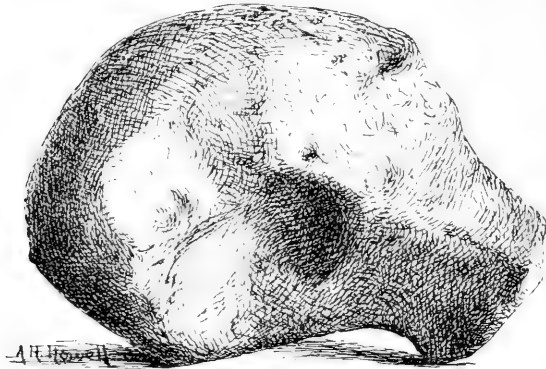
WELLAND METEORITE. (One-third natural size.)
