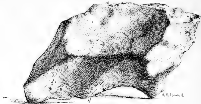
PUQUIOS METEORITE. (One-third natural size. The line a, b, indicates where section was made.)
