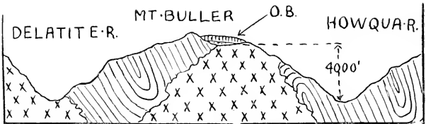
Fig. 8.—Diagrammatic section from North to South through Mt. Buller (6911 feet).
