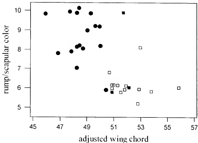
Figure 19 Scatterplot for Cistothorus palustris deserticola and coastal southern California Marsh Wrens of the two variables in which they differ most, wing length and rump/scapular color. So that the sexes could be considered together in one statistical process, the wing chords of females were multiplied by 1.06, the factor by which the average male Marsh Wren exceeds the average female. ■, core (August/September) specimens of the breeding population of the Colorado Desert ( deserticola ); □, additional October–February specimens from the Colorado Desert inferred as deserticola (see Figure 4); ●, specimens of the breeding population of coastal southern California.
