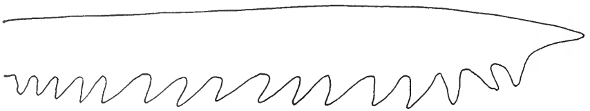
FIGURE 2.— Corydoras treillii Steindachner. Pectoral fin spine of lectotype, ventral view, left spine.
