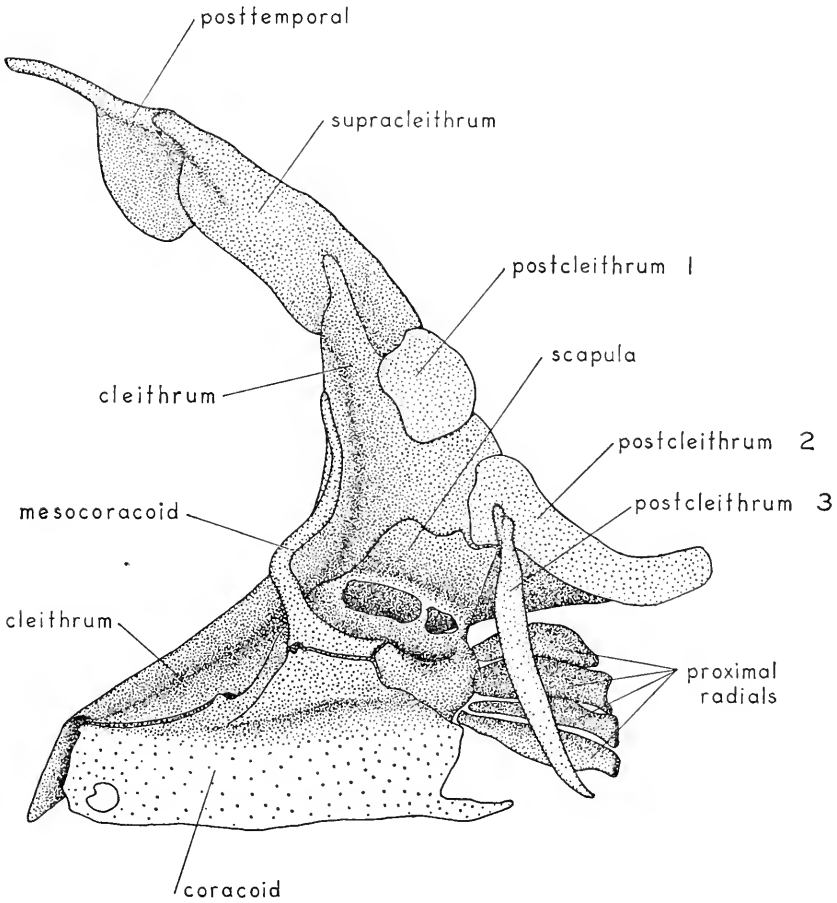
FIGURE 10.—Right pectoral girdle of Poecilibrycon harrisoni (median view). The fin rays have been removed.
