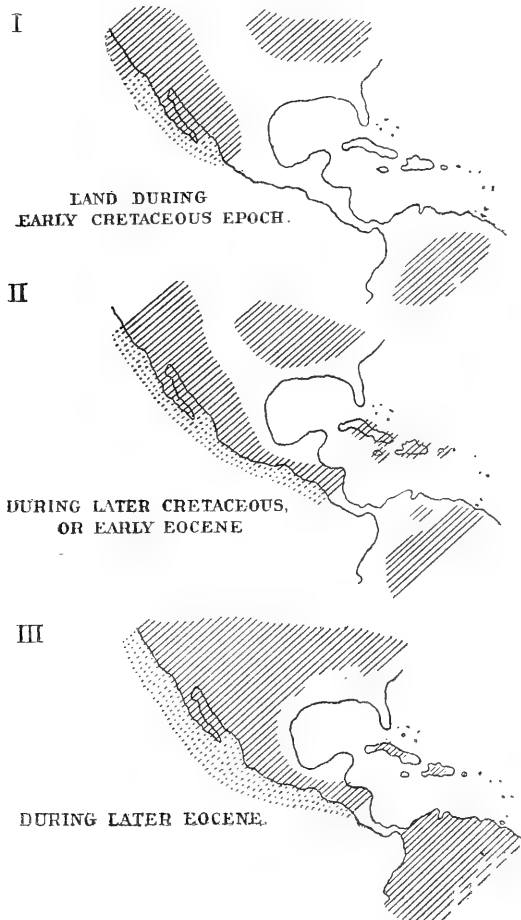
Diagrams to illustrate the contours of Mexico at different geological ages.
