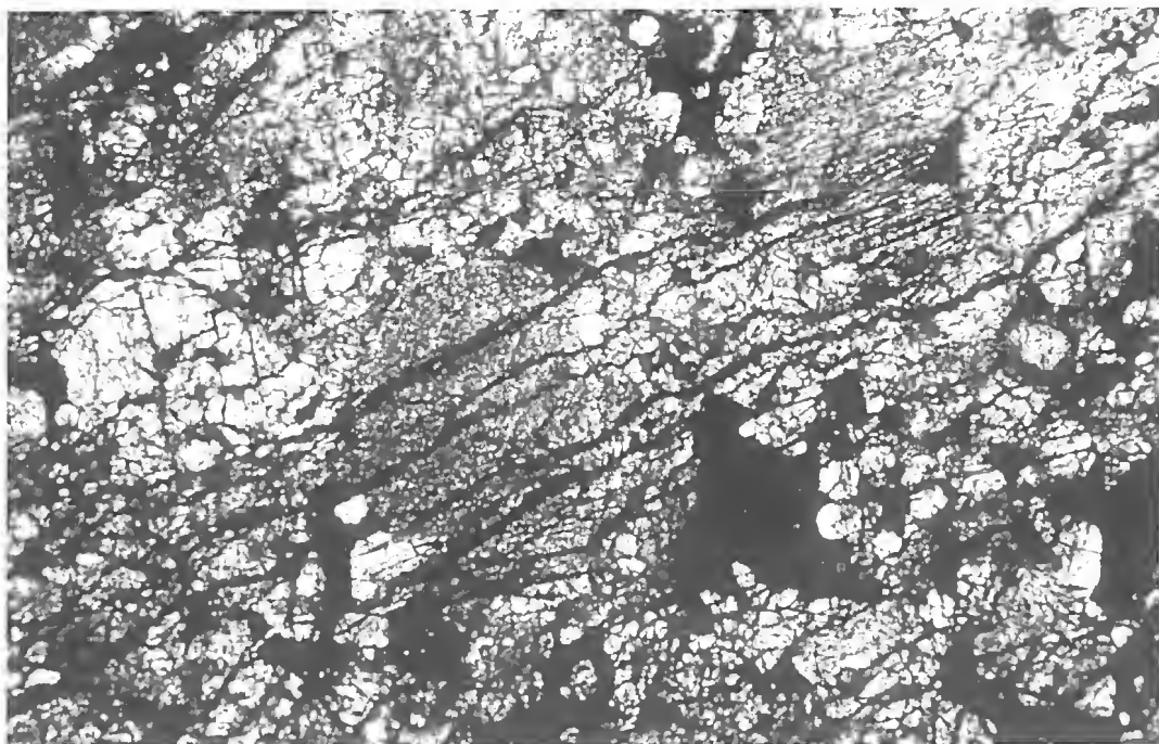
Fig. 7. Highly fractured texture in the Pigeek meteorite. Note the pervasive system of sub-parallel fractures (field of view 3 mm across).
