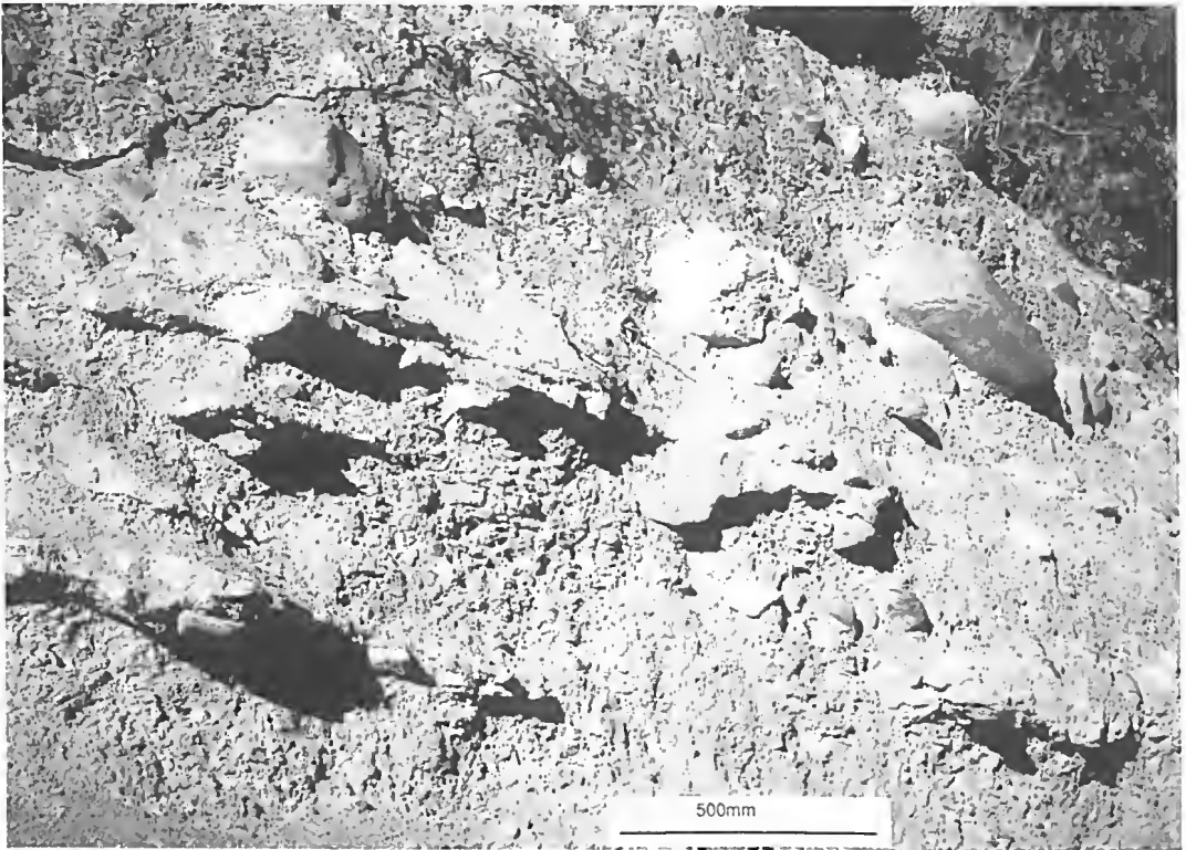
Fig. 4. Diamicite exposed on the eastern bank of the Lerderderg River, revealing imbricated boulders and dip to the southwards.
