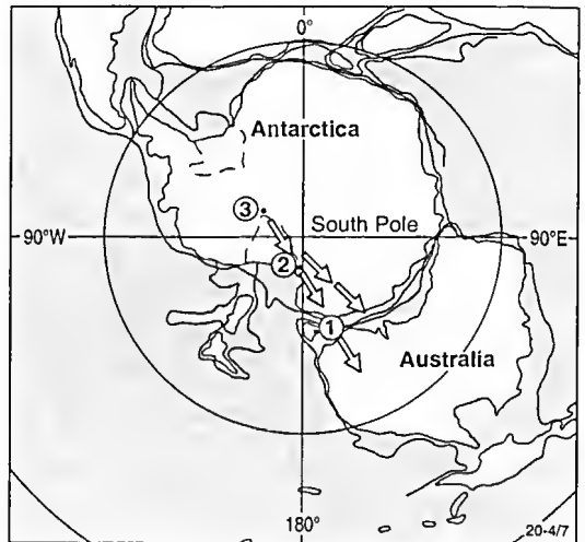
Fig. 7. Early Permian (Sakmarian) palaeogeographical reconstruction showing locations of possible palynomorph-bearing Devonian source rock in Tasmania and Antarctica and the path of ice transportation to south-eastern Australia. 1, north-eastern Tasmania (Eugenana beds); 2, south Victoria Land (Aztec Siltstone and Terra Cotta Siltstone); 3, Transantarctic Mountains, Ohio Range (Horlick Formation). Reconstruction after Truswell (1991).
