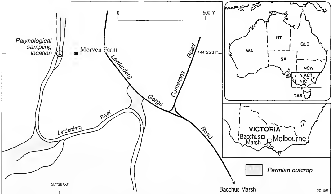
Fig. 2. Geological map of the Early Permian Bacchus Marsh Formation diamictite, Lerderberg River, Swing Bridge Section.
