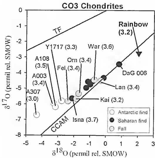
Fig. 6. O-isotopes for Rainbow and other CO3 meteorites (modified slightly from Grossman et al. 2000). Abbreviations: TF = terrestrial fractionation line; CCAM = carbonaceous chondritic anhydrous minerals mixing line; SMOW = standard mean ocean water; A003 = Allan Hills (ALH) A77003; A108 = ALH83108; A307 = ALHA77307; DaG006 = Dar al Gani 006; Fel = Felix; Kai = Kainsaz; Lan = Lancé, Orn = Ornians, War = Warrenton; Y1717 = Yamato 791717. Unlabelled Saharan meteorites include Acfer 202 and 243, Dar el Gani 023 and 025, and Hammadah al Hamra 043.
