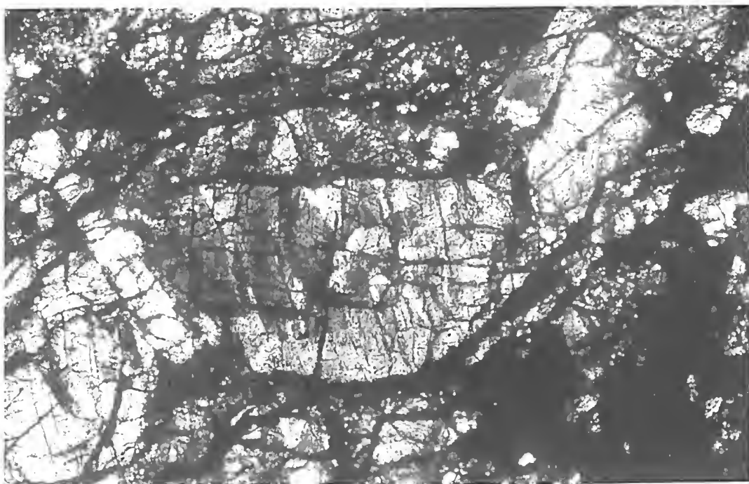
Fig. 8. Shock features in the Pigeek meteorite. The large olivine grain shows undulose extinction and there are also poorly developed planar fractures, for example in grain to lower left (field of view 1.2 mm across).
