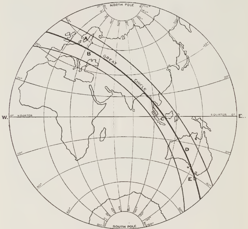
Map on Stereographic Projection showing Great Circle \gamma_{20^\circ} with belt on each side of it 10^\circ wide, indicating that all the known tektites of the World lie approximately on the same Great Circle.
