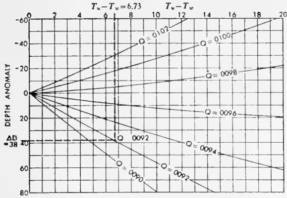
Figure 10.—Graph for determining thermometric depth anomalies from corrected thermometer readings, T_w - T_w , and thermometer constant, Q .
