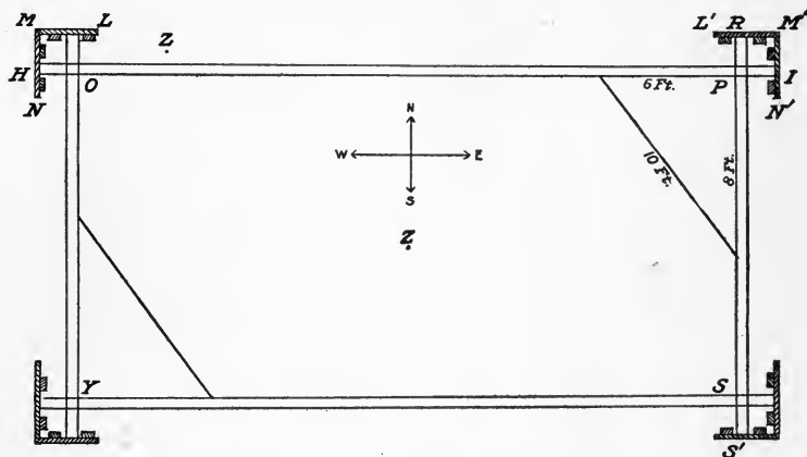
FIG. 80.—Diagram showing method of laying out foundation. (See text for directions.) The foundation cannot be laid out too carefully.
