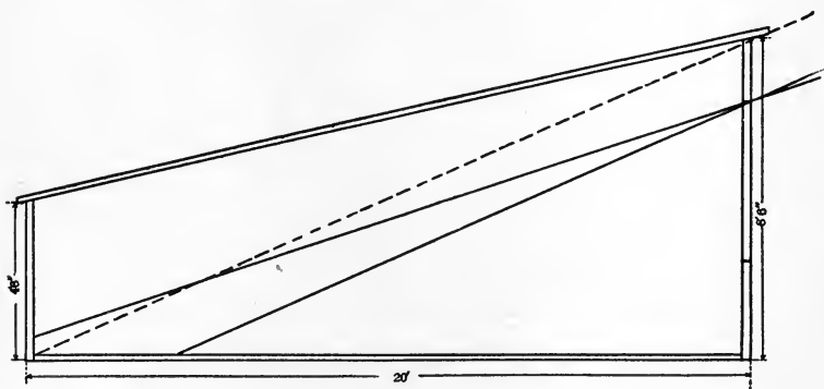
FIG. 69.—Diagram showing lines of sun's rays in September and December. The front of the house is 8 ft. 6 in. high and the back 4 ft. 6 in. high, with a width from front to back of 20 feet.
