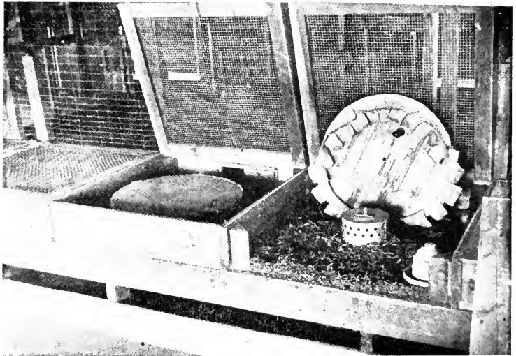
FIG. 164.— A , Interior of long house with double-pen brooders. B , Single compartment and its hover. (Courtesy of Hall and Candee Companies.)
