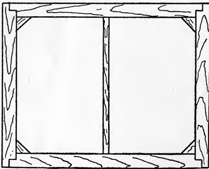
FIG. 78.—Two plans for constructing frames for muslin curtains.
