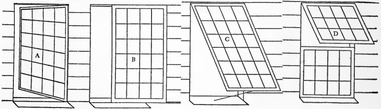
FIG. 77.—Types of poultry windows. A, Hinged at the side and opening inward, the method preferred; B, sliding window; C, hinged at the top and opening outward; D, upper sash hinged at the top and opening outward and lower sash stationary.
