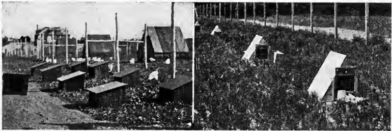
FIG. 151.—Two common types of sitting coops.
