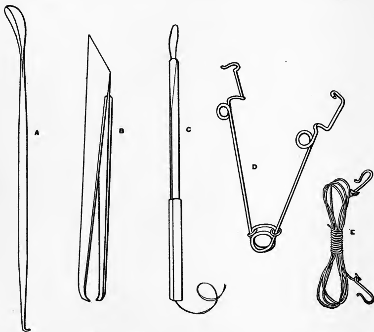
FIG. 181.—Caponizing instruments. A, Spoon and hook; B, forceps and knife; C, cannula threaded with horsehair; D, spreader; E, cord and hooks.
