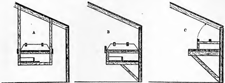
FIG. 93.—Arrangement of nests, perches, and dropping boards. A, suspended; B and C, attached to back wall.
