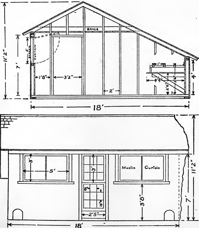
FIG. 88a.—End and front views of a part of laying house with two-thirds span roof.
