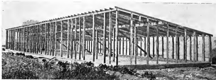
FIG. 73.—A well-framed poultry house.
