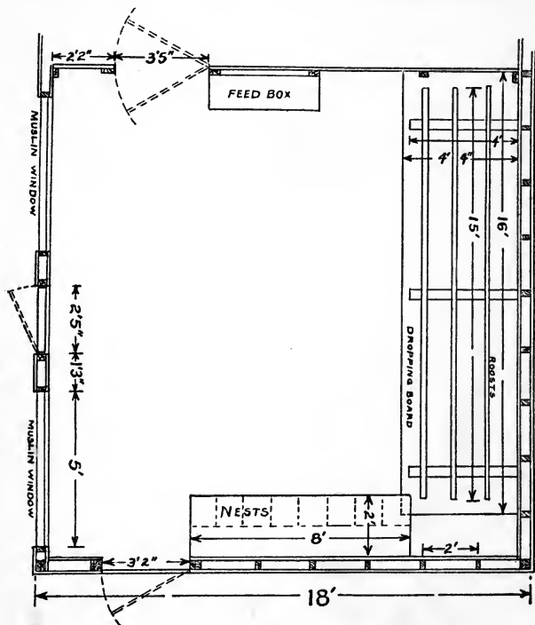
FIG. 88b.—Working plans of laying house with two-thirds span roof.—Floor plan of one section.
