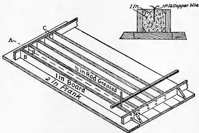
FIG. 108.—Forms for making concrete fence posts.
