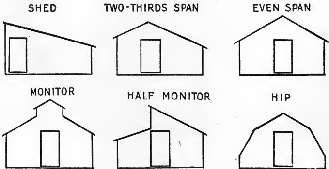
FIG. 72.—Six types of roofs for poultry houses. The shed roof is most common and is the best.
