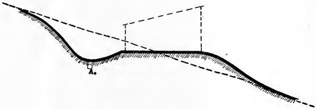
FIG. 79.—Cross section of hillside, showing manner of grading before laying out foundation. The long dotted line shows original slope and the heavy black line shows the surface graded for the poultry house. The house is shown in outline. Drain tile may be placed at A to carry water below the house.
