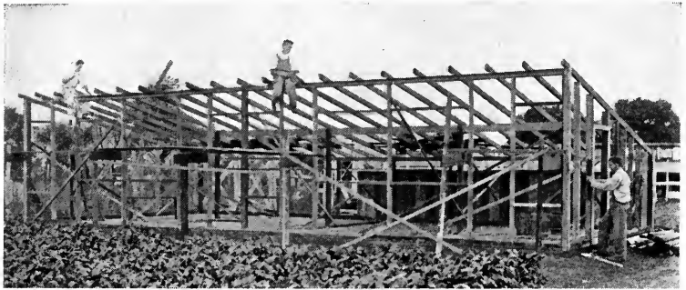
FIG. 84.—Frame of standard multiple-unit laying house—light, cheap, yet durable.
