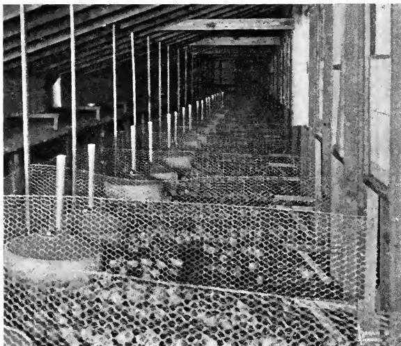
FIG. 165.—Portable indoor hovers make it possible to use the laying houses for brooding purposes. (Photo by Rancocas Poultry Farm.)
