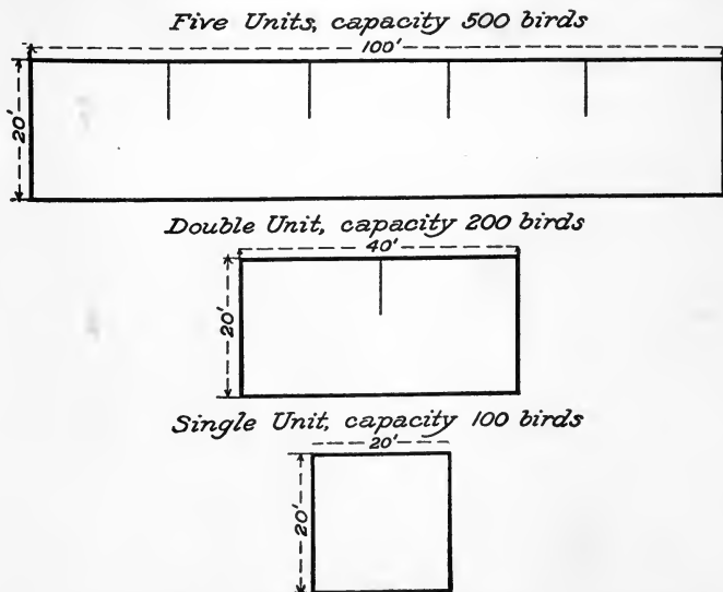
FIG. 71.—The possible growth of the multiple-unit plan,—single, then double, and an indefinite future increase.
