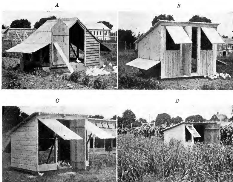
FIG. 173.—Four types of summer developing houses. A , Fresh-air house so constructed that both side walls hinge and open upward, allowing an unlimited circulation of air; B , shed-roof colony house; C , a wide-open house; D , a portable summer chick shelter, showing a luxuriant vegetation furnishing an abundance of green feed and shade.
