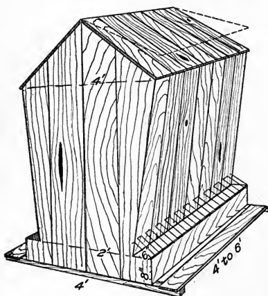
FIG. 102.—A home-made dry-mash hopper, feeding from both sides, for large flocks.
