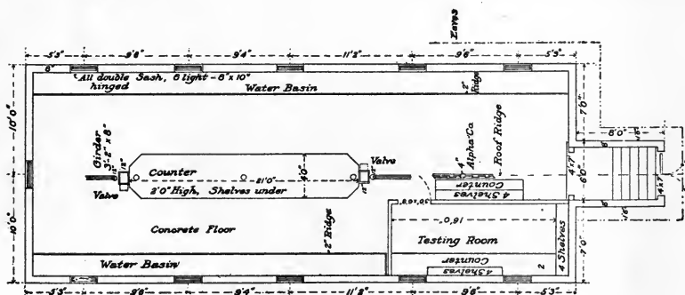
FIG. 155.—Working plans for incubator cellar.
