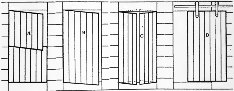
FIG. 75.—Four styles of doors for poultry houses. A, Brooder house door, cut in the centre so that the top half only need be opened, providing ventilation but preventing floor draft; B, door hung to swing both ways; C, double doors for use where overhead trolleys are used; D, sliding door.
