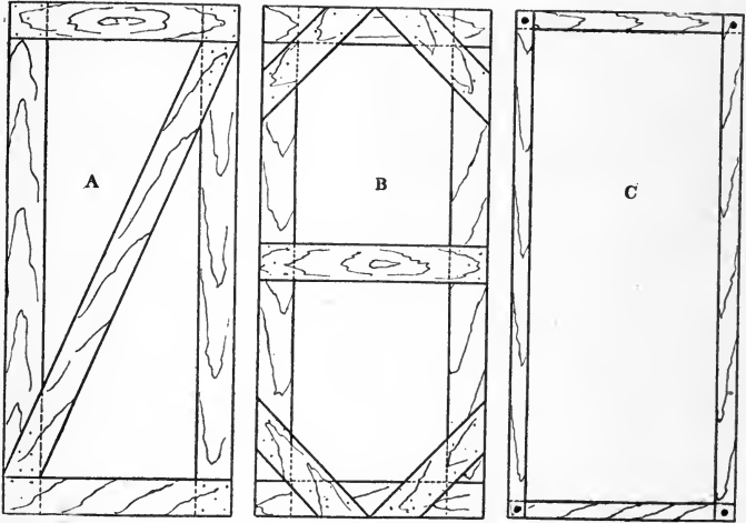
FIG. 112.—Types of gate construction. A, Best type, 1 x 6 inch white pine is used; B, same material with different bracing; C, corners mortised and bolted, 2 x 3 inch material used.
