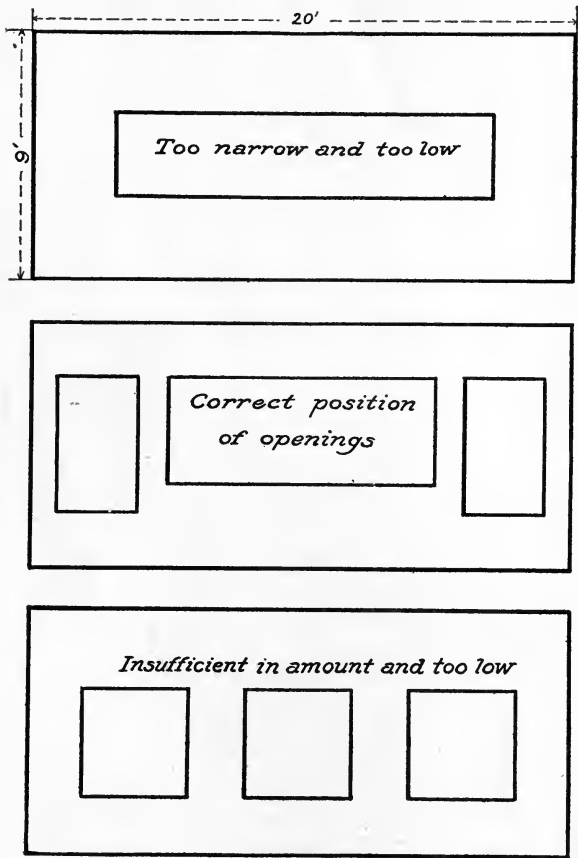
FIG. 76.—Three plans for placing openings in front wall of poultry houses.
