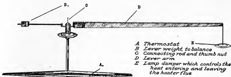
FIG. 159.—A complete self-regulating device for incubators heated by lamps.
