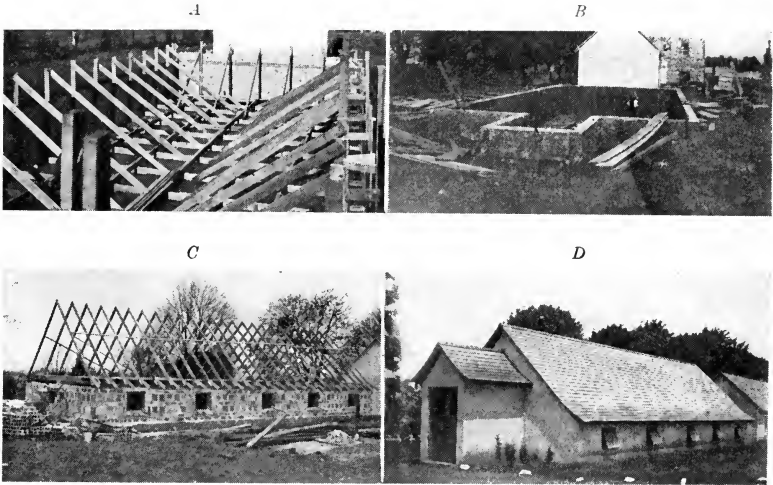
FIG. 156.—Four views showing construction of hollow-tile incubator cellar. A, Forms ready for pouring concrete foundation wall; B, forms removed; C, hollow-tile construction, and manner of framing roof; D, completed cellar.
