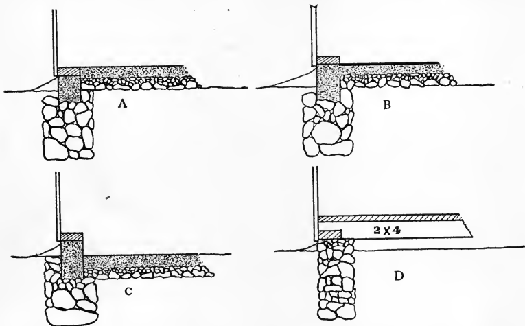
FIG. 74.—Four plans for foundation and floor construction. A, Floor flush with top of sill; B, finished floor flush with bottom of sill, the latter being laid in cement; C, foundation wall extending above floor level; D, construction suitable for board floor.
