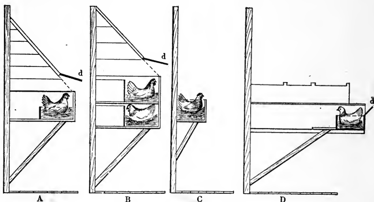
FIG. 95.—Four ways of locating nests,—end boards are removed to show construction. Eggs are taken out from the covered nests by raising the door, d .
