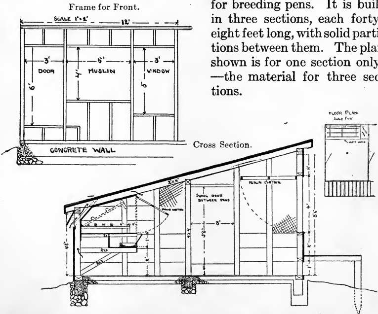
FIG. 86.—Working plans of small-unit laying house. (See text for description.)
