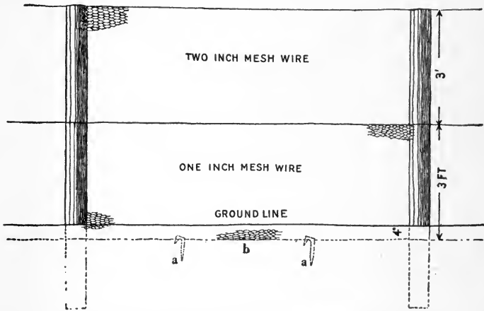
FIG. 110.—A common type of fence construction. a , Manner of anchoring wire under ground; b , wire buried a few inches under ground.
