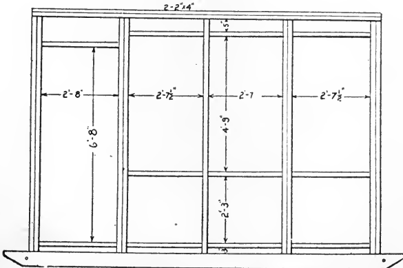
FIG. 92a.—Portable laying house: Working plans.
