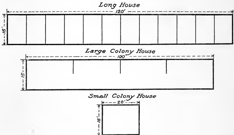
FIG. 68.—Three types of laying houses. The long house is used for small-unit flocks with intensive methods for breeding purposes. The large colony house is for large flocks for market eggs. The small colony house is used for breeding in small flocks.
