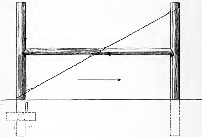
FIG. 109.—Manner of bracing a corner fence post (a). The pull is in the direction of the arrow. The cleats on the bottom of the corner post prevent its turning or twisting.
