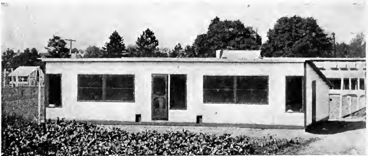
FIG. 85.—Double-unit house completed. Note the combination door and window, and the arrangement of openings for light and ventilation.
