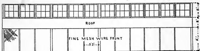
Fig. 91a.—Half-monitor type of laying house: Working plans.
