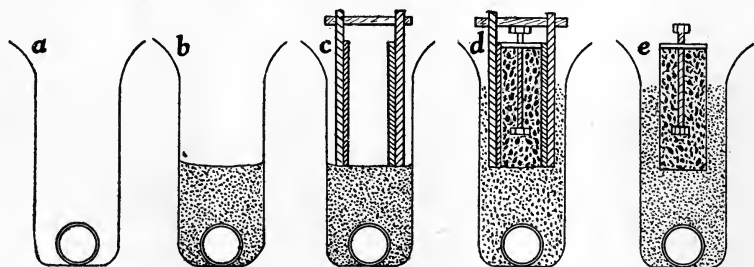
FIG. 81.—Five steps in the construction of a concrete foundation. a , Tile in the bottom of trench; b , tamped cinders over drain tile; c , forms ready for pouring concrete; d , forms filled with concrete, sill bolt in place; e , forms removed, foundation completed, and cinders filled in on both sides.
