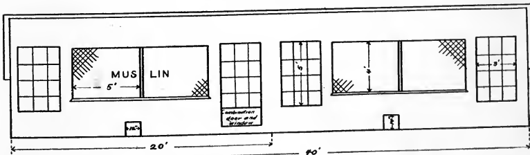
FIG. 83.—Working plans of a double-unit laying house. Each unit 20 x 20 feet, with a capacity of 100 birds.
