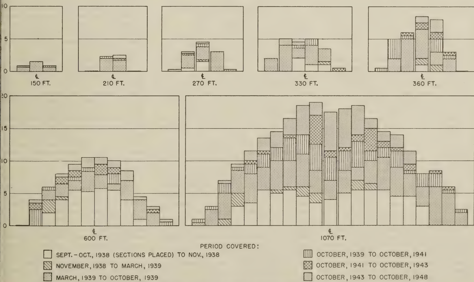
Figure 19.—Distribution of cumulative cracking per 50 feet of section length in the first 10 years of pavement life.
