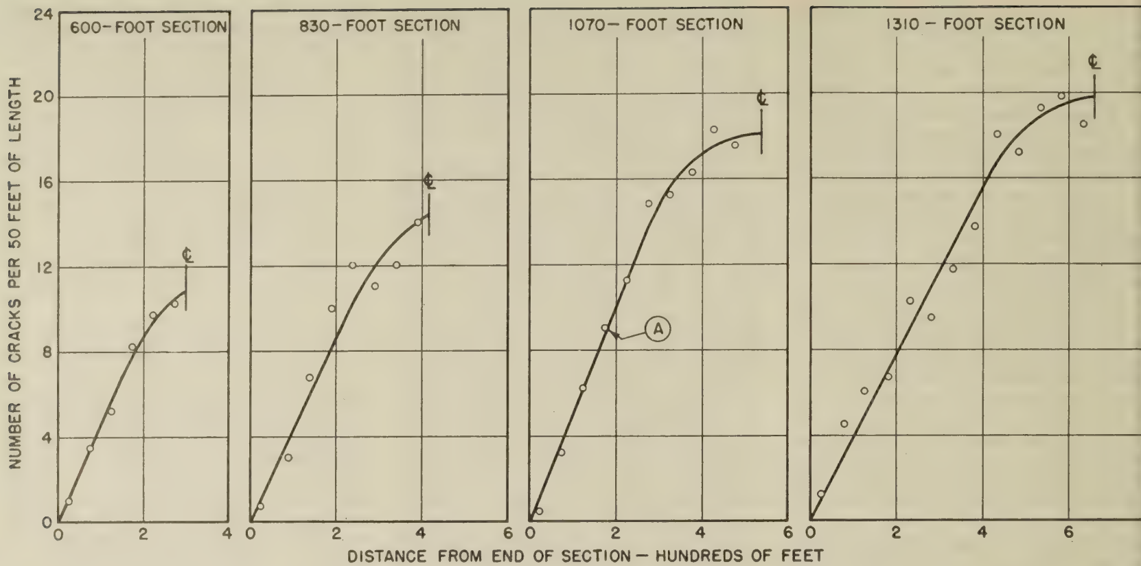
Figure 20.—Frequency distribution of cracking at the end of 10 years for sections reinforced with 1-inch diameter rail-steel bars (1 percent steel); average of both lanes.
