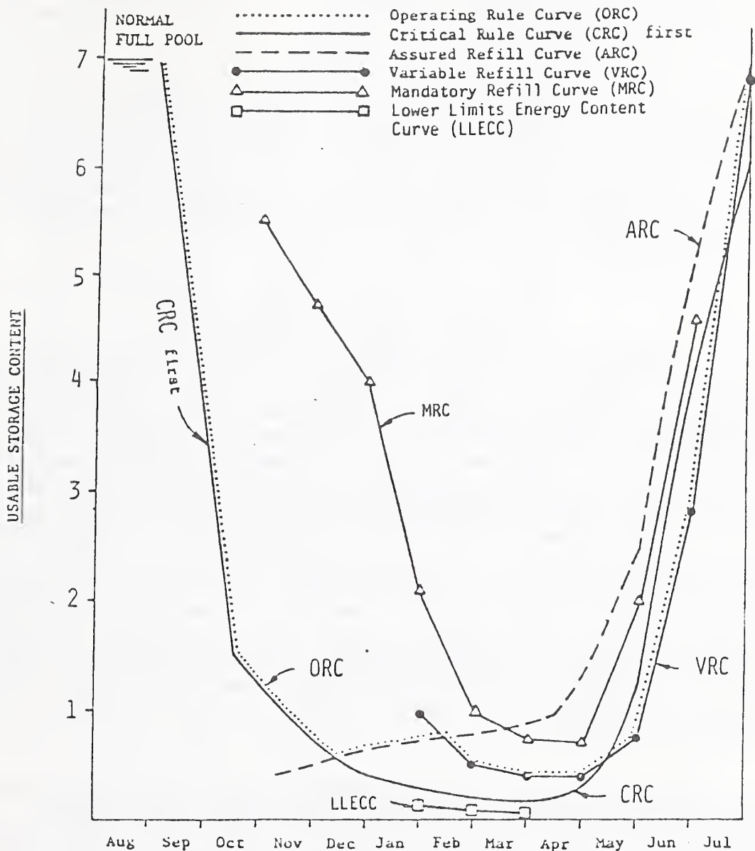
Figure 8. Hypothetical rule curves illustrating how an operational rule curve (ORC) is formed for Columbia River flood control-hydroelectric projects (modified from Columbia River Treaty Committee 1983).
