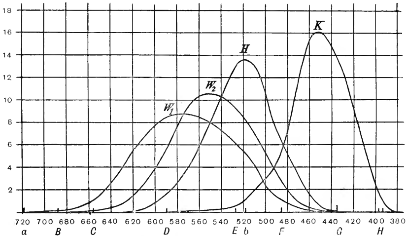
Fig. 44. Equal-area gauging curves for dichromats and monochromats ( H ). W_1 , deuteranopic "warm" curve; W_2 , protanopic "warm" curve; K , "cold" curve common to both types of dichromats. Abscissae, wave-lengths of the interference spectrum of sunlight; ordinates, arbitrary scale. (König.)
