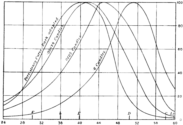
Fig. 23. "Persistency of light" curves corresponding to the "extinction of light" curves for different degrees of light adaptation. Abscissae, wave-lengths; ordinates, reciprocals of extinction values. (Abney.)
