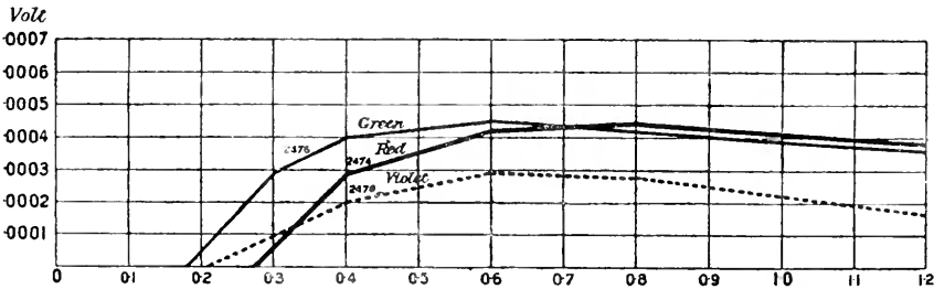
Fig. 3. Curves constructed from typical electrometer records of eyeball responses to the light from the red, green, and violet regions of the interference spectrum of the arc light. (Gotch.)
