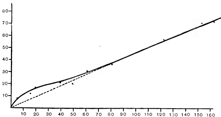
Fig. 18. Curve of equivalent luminosities of red ( 670\mu\mu ) and blue ( 450\mu\mu ) lights at different intensities (slit-widths). (König.)
