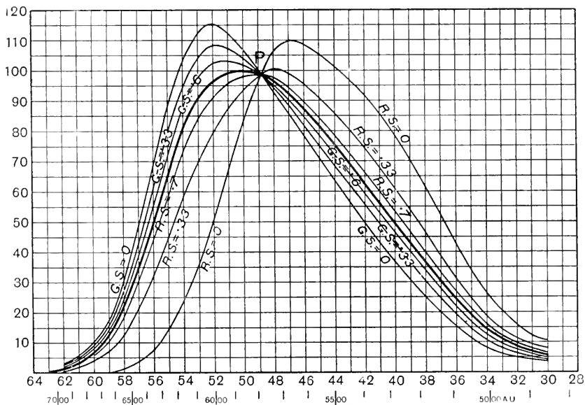
Fig. 68. Luminosity curves of persons having normal and reduced red and green sensations. Abscissae, wave-lengths of the prismatic spectrum of the arc light; ordinates, arbitrary scale. (Watson.)
