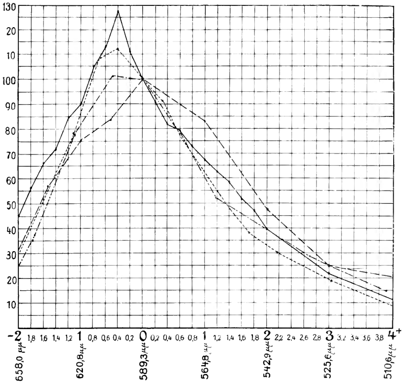
Fig. 27. ——— "Minimal-field luminosity curve." - - - - - Photopic periphery luminosity curve. - · - · - Photopic central luminosity curve (licker method). ······ "W-curve" of a deuteranope (see Fig. 45). (Siebeck.)
