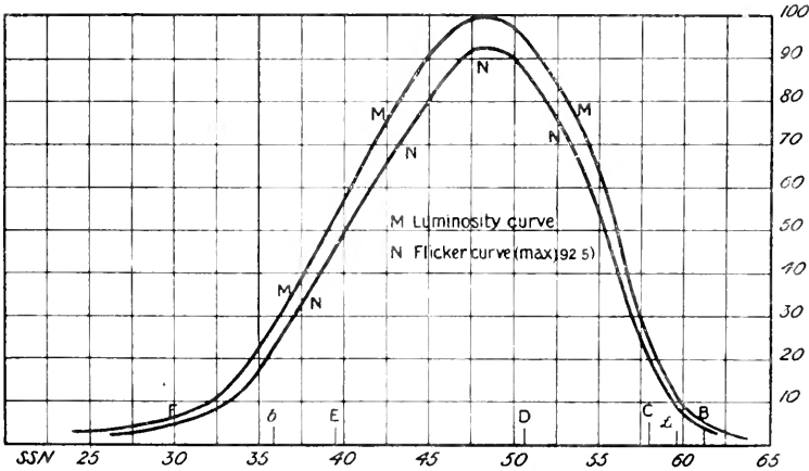
Fig. 12. Normal trichromat's photopic luminosity curves with the equality of brightness and the flicker methods. Abscissae, arbitrary scale of the prismatic spectrum of the arc light ; ordinates, arbitrary scale, the maximum luminosity by the equality of brightness method being 100. (Abney.) (Cf. Fig. 38.)
