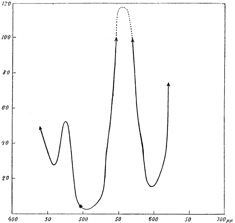
Fig. 66. Curve of discrimination sensibility for hues of the interference spectrum of the arc light for a protanope. * Neutral point. Abscissae, wave-lengths; ordinates, differences of wave-length ( \delta\lambda ) capable of being discriminated. (Steindler.)
