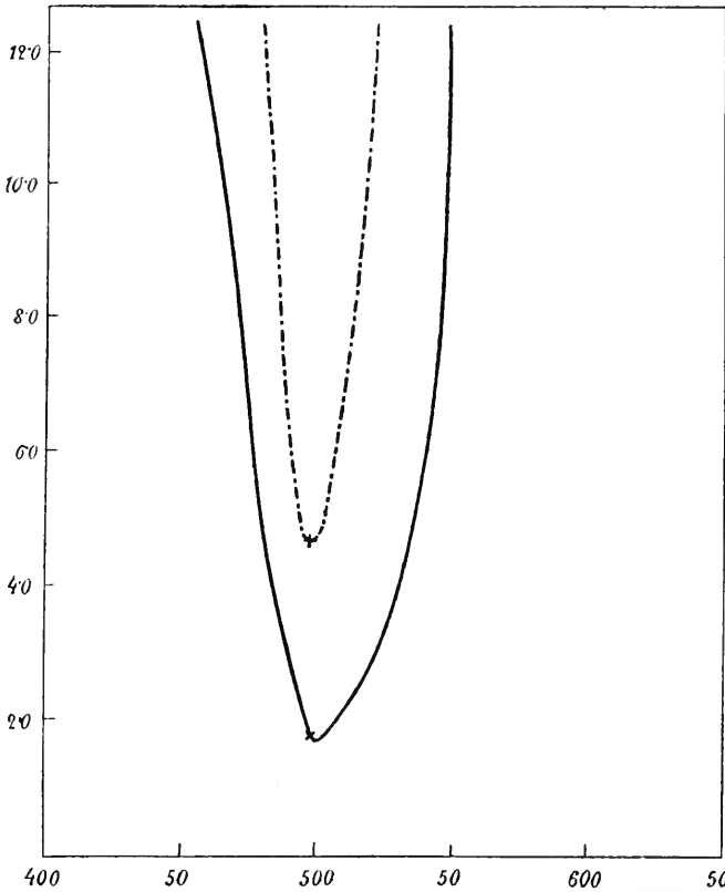
Fig. 67. Curves of discrimination sensibility for hues of the interference spectrum of the arc light for two deuteranopes. × Neutral point. (Steindler.)
