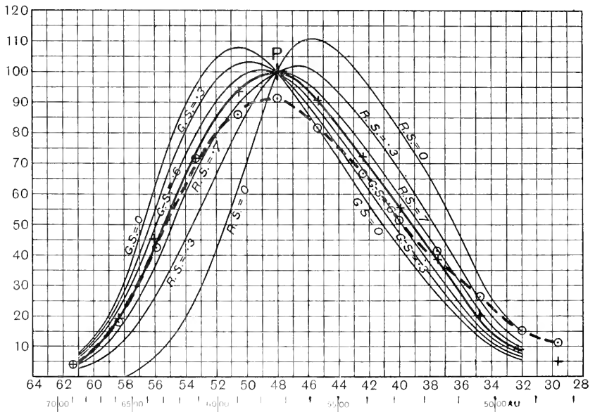
Fig. 71. Luminosity curves of a normal trichromat with average macular pigmentation. + + + foveal; ○ ○ ○ parafoveal. (Watson.)
