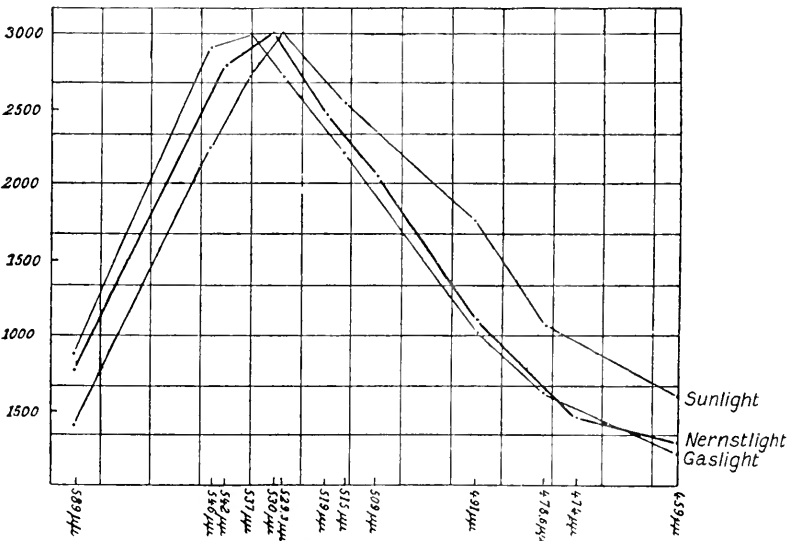
Fig. 16. Scotopic luminosity curves for direct sunlight (Schaternikoff), gas light (Schaternikoff), and Nernst light (Trendelenburg), reflected from a magnesium oxide-coated surface. Abscissae, wave-lengths of the prismatic spectrum; ordinates, arbitrary scale, the maximum of luminosity being in each case 3000. (Trendelenburg.)
