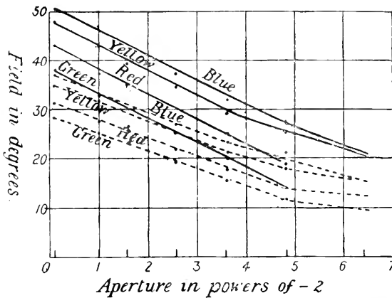
Fig. 33. The temporal (————) and nasal (-----) limits of the fields of vision for four spectral colours for different areas of stimulation. (Abney.)
