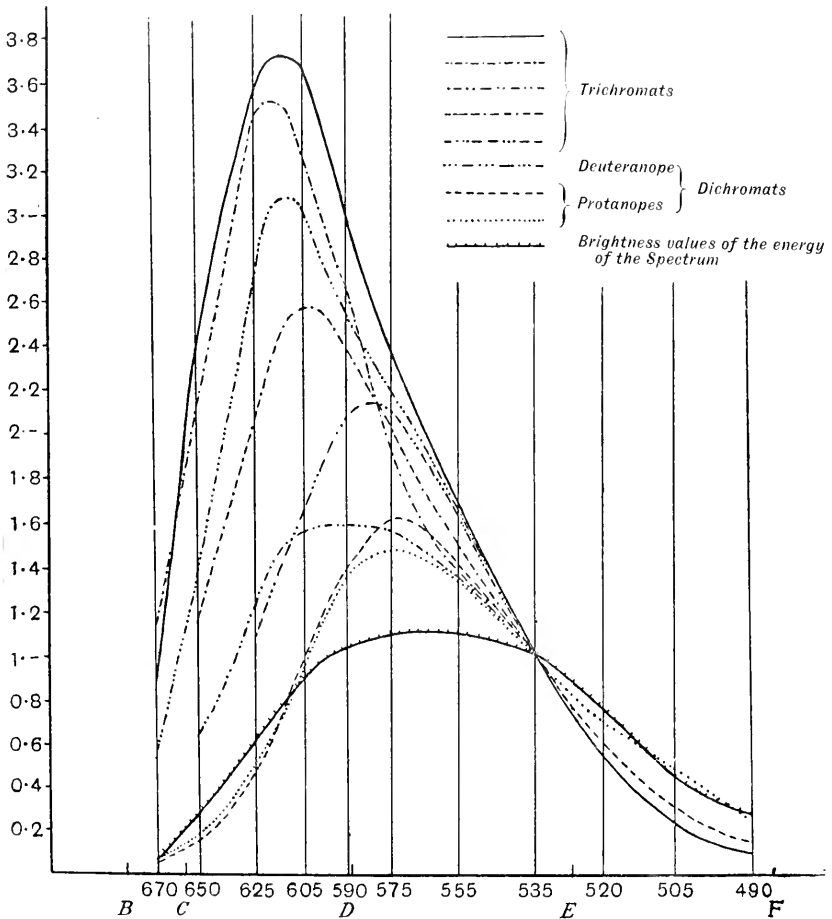
Fig. 48. Photopic luminosity curves (intensity I ) of trichromats and dichromats. Abscissae, wave-lengths of the prismatic spectrum of gaslight; ordinates, arbitrary scale. (König.)
