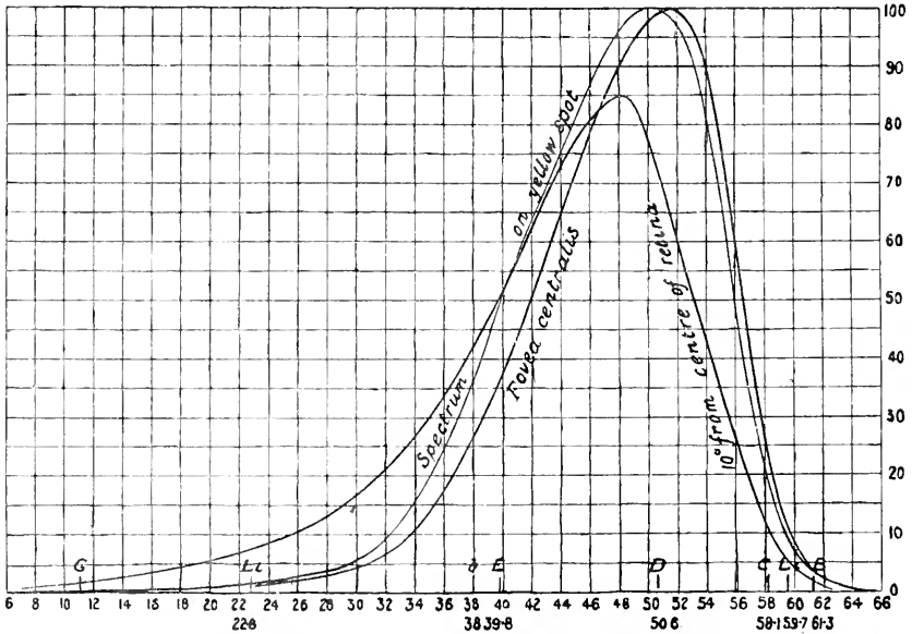
Fig. 11. Normal trichromat's photopic luminosity curves for the fovea, macular region, and 10° from the fovea. Abscissae, arbitrary scale of the prismatic spectrum of the are light, the Fraunhofer lines and some important wave-lengths being indicated ; ordinates, arbitrary scale, the maximum luminosity being 100. (Abney.)
