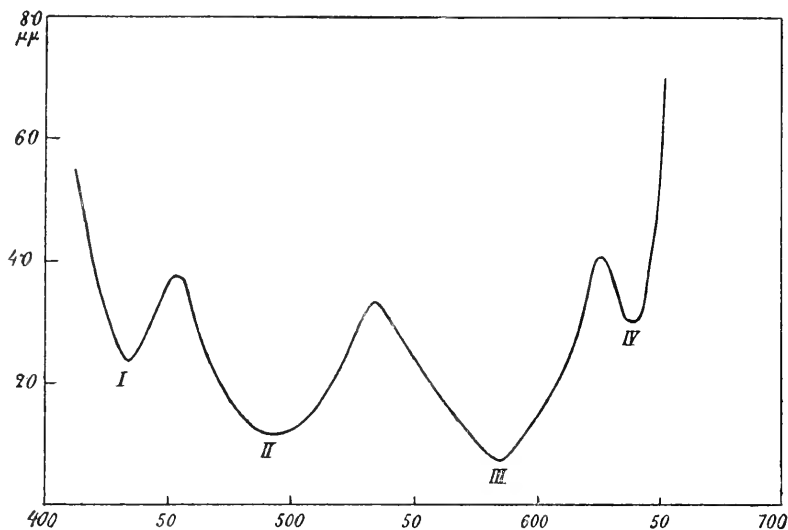
Fig. 5. Curve of discrimination sensibility for hues of the interference spectrum of the arc light. Abscissae, wave-lengths of the lights; ordinates, differences of wave-length ( \delta\lambda ) capable of being discriminated. (Steindler.)
