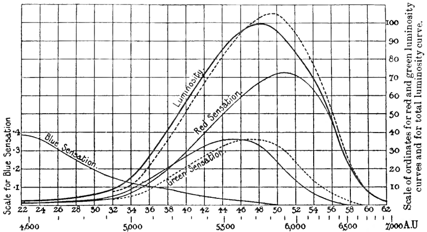
Fig. 73. Normal sensation curves in terms of luminosity. (Abney and Watson.)
