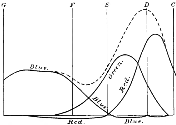
Fig. 58. Clerk-Maxwell's sensation curves. The dotted line is the algebraical sum of the ordinates at each point; it is not a true luminosity curve. Abscissae, wave-lengths of the prismatic spectrum of sunlight; ordinates, arbitrary scale. (Clerk-Maxwell.)
