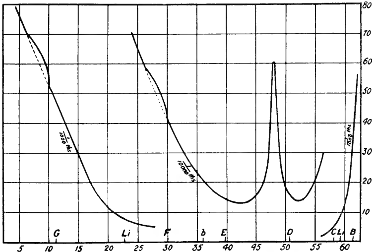
Fig. 19. "Extinction of colour" curve. Abscissae, wave-lengths of the prismatic spectrum; ordinates, intensity of the illumination in candle-feet on the screen when the colour just vanishes. (Abney.)
