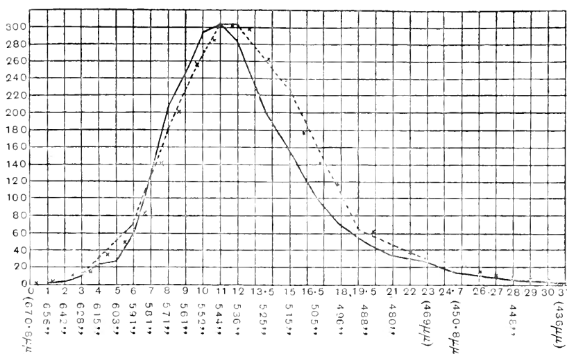
Fig. 51. ——— Achromatic scotopic luminosity curve of a deuteranope. . . . . Luminosity curve of a monochromat. Abscissae, wave-lengths of the prismatic spectrum of gaslight; ordinates, arbitrary scale. (v. Kries.)
