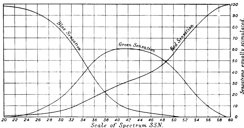
Fig. 65. Percentage of the R , G , and B sensations in the spectrum colours when equal stimulations of the three sensations give rise to the sensation of white. (Abney.)
