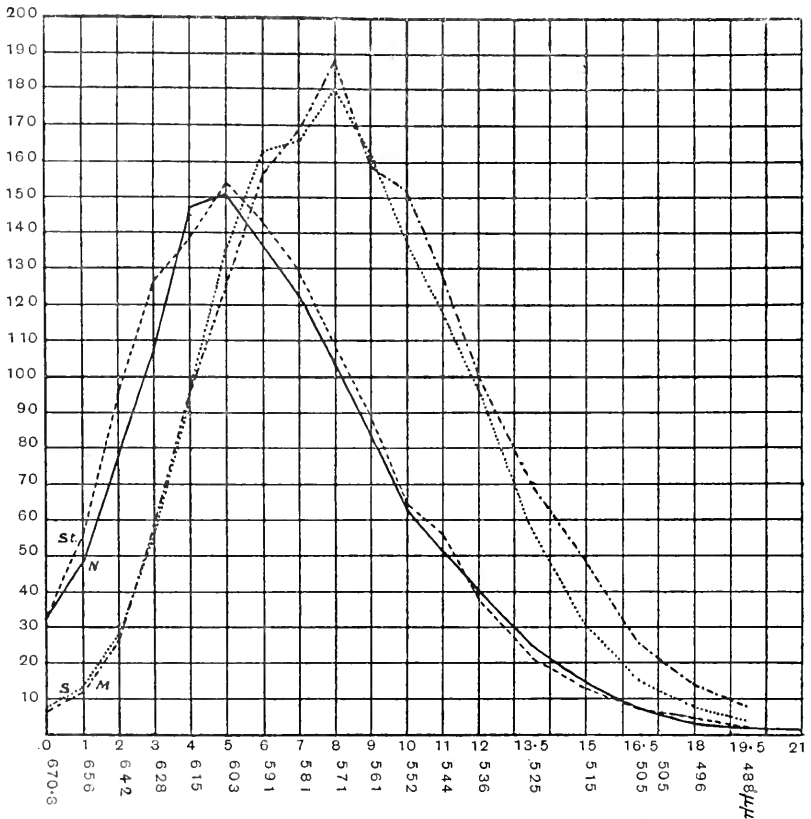
Fig. 45. Gauging curves for dichromats: "warm" curves. S and M , two protanopes; N and St , two deuteranopes. Abscissae, arbitrary scale of prismatic spectrum of gaslight, indicating certain wave-lengths; ordinates, arbitrary scale. (v. Kries.)
