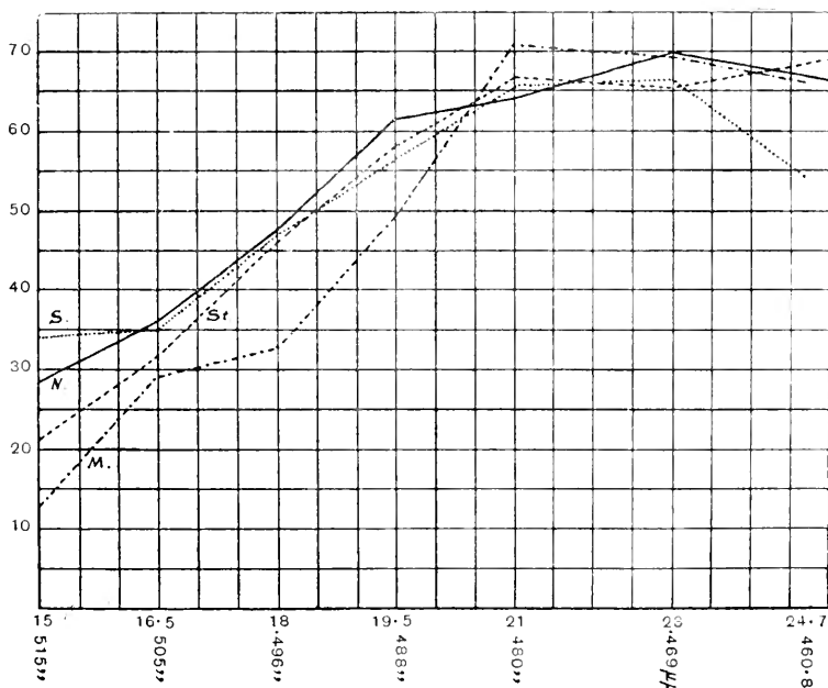
Fig. 46. Gauging curves for dichromats: "cold" curves. Same observers as in Fig. 45. (v. Kries.)
