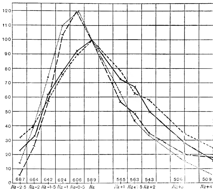
Fig. 51. . . . . Photopic luminosity curve of a deuteranope (flicker method). — — — Periphery luminosity curve of the same deuteranope. - - - - - Photopic luminosity curve of the same trichromat as in Fig. 50 (flicker method). ——— Periphery luminosity curve of the same trichromat. (Polimanti.)
