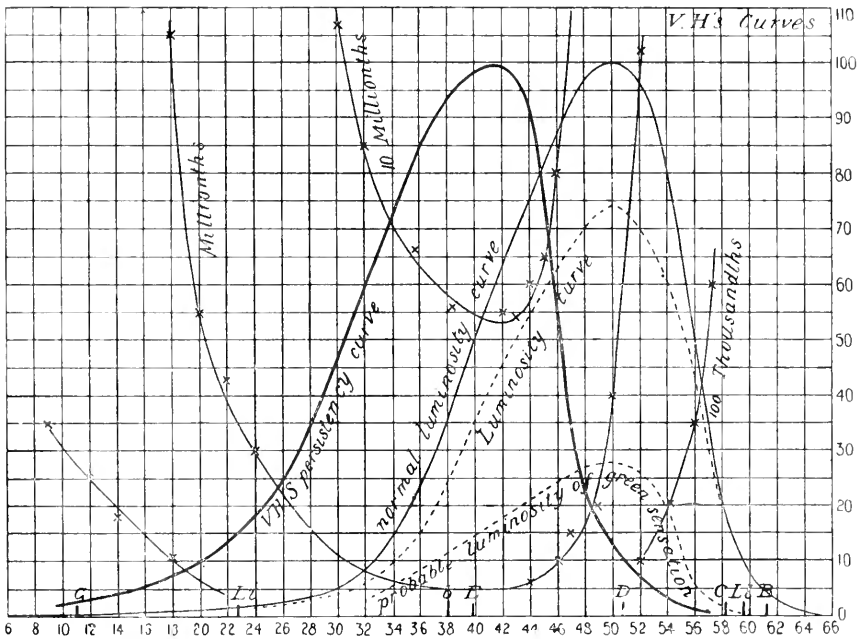
Fig. 21. "Persistence curve" of a deuteranope. The values are the reciprocals of the "extinction of light" values, which are also shown. The "normal luminosity curve" is the curve for higher intensities of light (the photopic luminosity curve). The persistency curve is the achromatic scotopic luminosity curve (compare Fig. 14). (Abney and Festing.)
