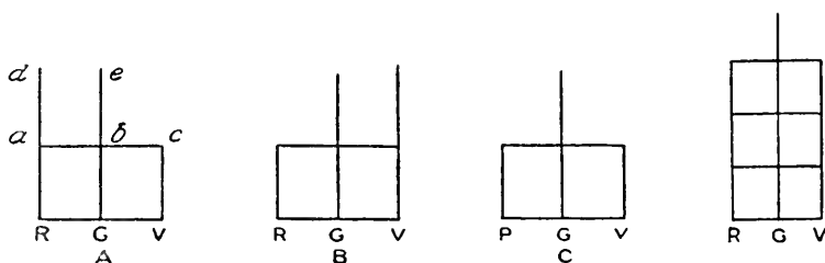
Fig. 61. Diagrams illustrating Abney's method of determining the normal sensation curves.
