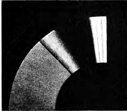
Fig. 37. Appearance of a narrow slit, 2^\circ to 5^\circ in width, in a large disc, rotating at one revolution per 3'' , before a milk-glass illuminated with one acetylene-gas burner, as seen by the light-adapted eye which has been kept covered for about three minutes and then fixed upon any point in or near the path of the moving slit—"Bidwell's ghost." (McDougall.)
