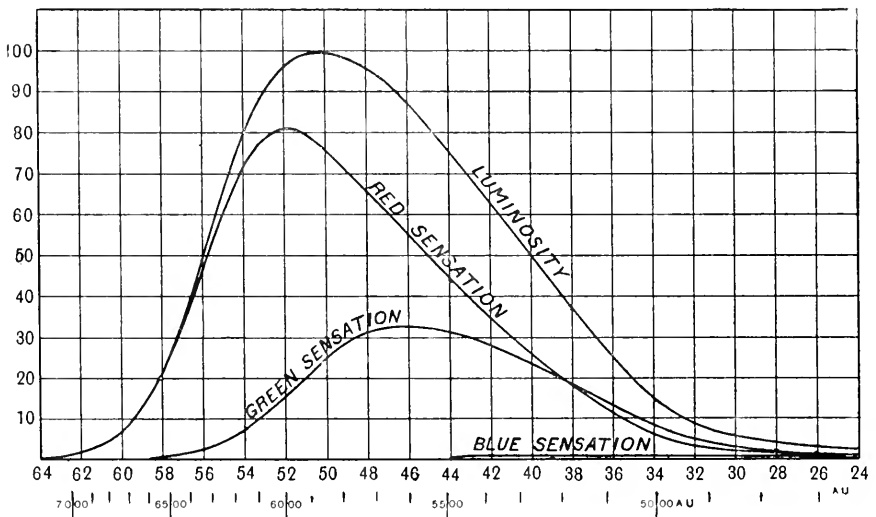
Fig. 63. Abney's R , G , and B sensation curves in terms of luminosity. The sums of the ordinates at any point are equal to the ordinate of the photopic luminosity curve. (Watson.)
