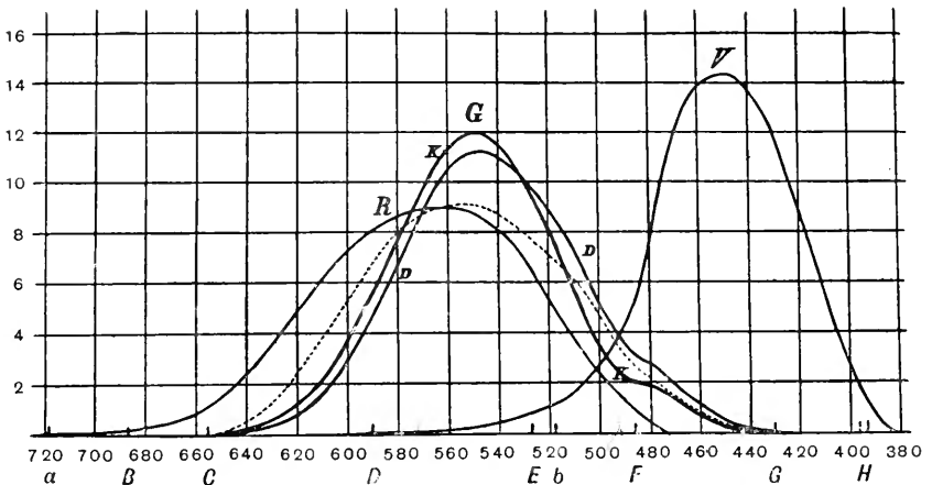
Fig. 59. R , G , and V . sensation curves. K , König's G -curve; D , Dieterici's G -curve; . . . . . G -curve of an anomalous trichomat. Abscissae, wave-lengths of the interference spectrum of sunlight; ordinates, arbitrary scale. (König and Dieterici.)
