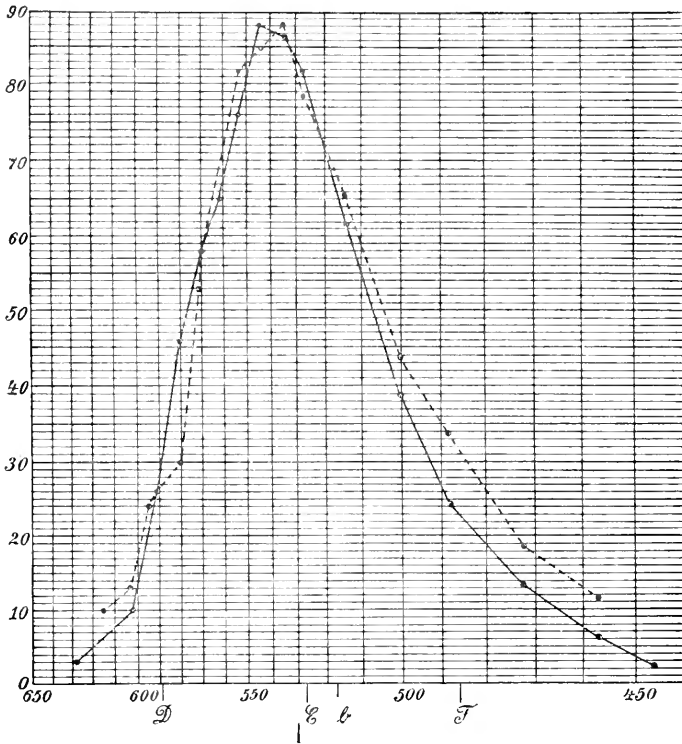
Fig. 55. ———— Achromatic scotopic luminosity curve of a deuteranope. . . . . Luminosity curve of a monochromat. Abscissae, wave-lengths of the prismatic spectrum of the Nernst light; ordinates, arbitrary scale. (Nagel and May.)
