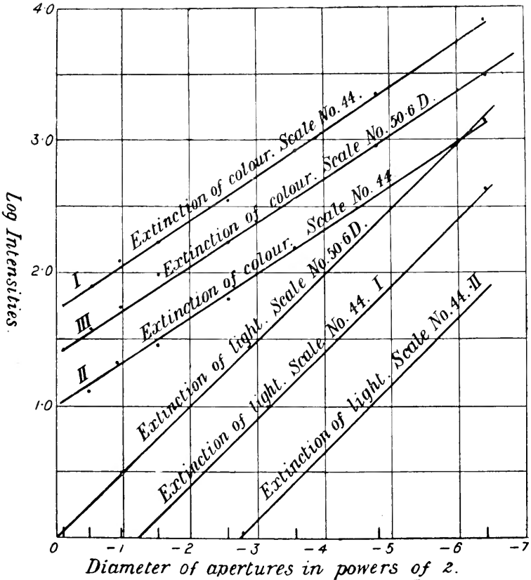
Fig. 40. Extinction of colour and light curves with different areas of stimulation. SSN 44 = 548.1 \mu\mu ; SSN 50.6 = D line: I and II, different observers and different intensities. (Abney.)
