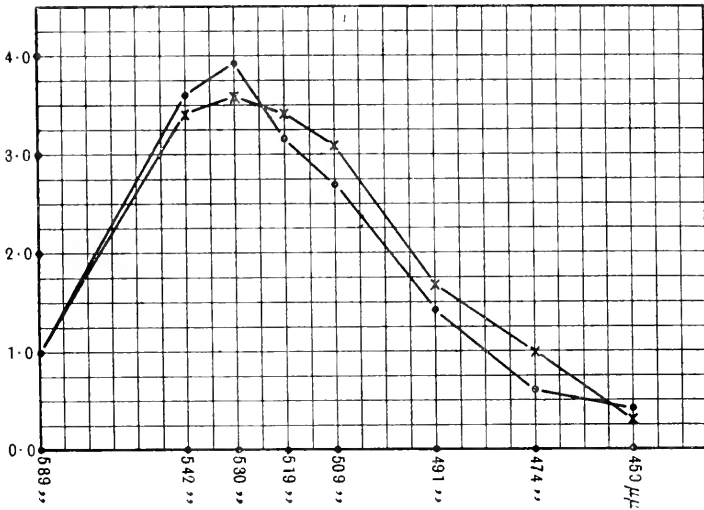
Fig. 1. . . . . the bleaching values of spectral lights for frog's visual purple, and \times - \times - \times the human achromatic scotopic luminosity curve. Abscissae, wave-lengths of the prismatic spectrum of the Nernst light; ordinates, an arbitrary scale. (Trendelenburg.)
