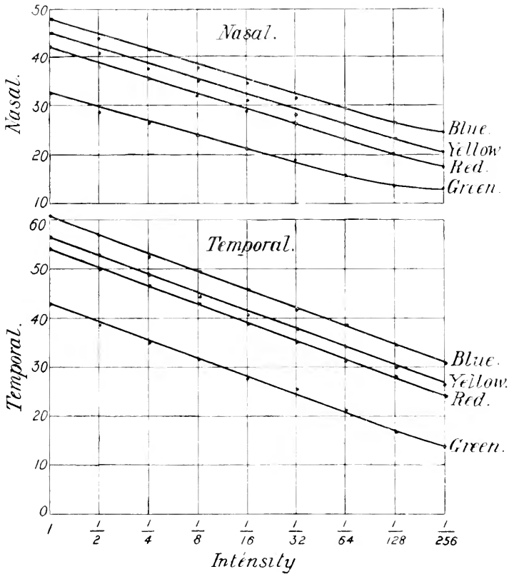
Fig. 32. The temporal and nasal limits of the fields of vision for four spectral colours at different intensities of illumination. (Abney.)
