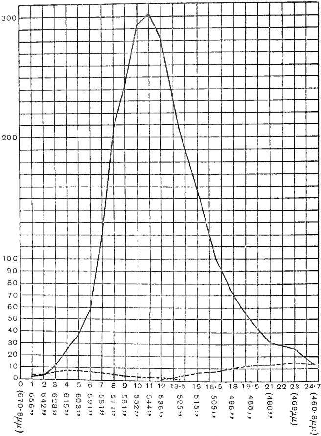
Fig. 52. ——— Scotopic values of the homogeneous lights. ..... Scotopic values of the photopic equivalent red (642 μμ)—blue (460.8 μμ) mixture. Abscissae, wave-lengths of the prismatic spectrum of gaslight; ordinates, arbitrary scale. (v. Kries and Nagel.)
