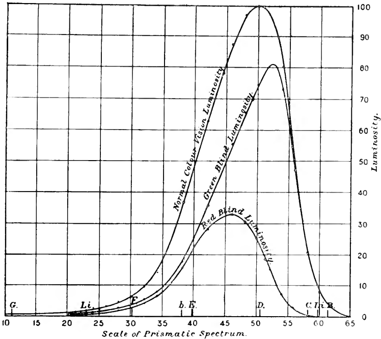
Fig. 49. Photopic luminosity curves of trichromats and dichromats. (Abney.)
