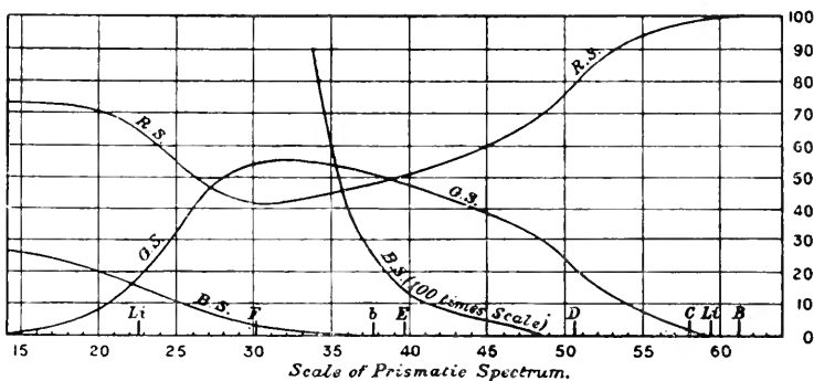
Fig. 62. Percentage of the R , G , and B sensations in the spectrum colours in terms of luminosity. Abscissae, wave-lengths of the prismatic spectrum of the arc light ordinates, arbitrary scale. (Abney.)
