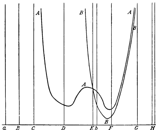
Fig. 4. Curves of discrimination sensibility for hues of the spectrum of gas light. A, A, A , for normal trichromat; B, B, B , for a deuteranope. Abscissae, wave-lengths, (König.)
