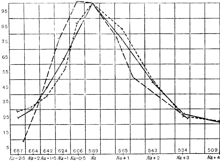
Fig. 26. ——— Photopic periphery luminosity curve (flicker method). ····· Photopic central luminosity curve (flicker method). - - - - - Photopic periphery luminosity curve (equality of brightness method). Abscissae, arbitrary scale of wave-lengths of prismatic spectrum of gas light, measured from the D line ( Na ), with certain absolute wave-lengths indicated; ordinates, arbitrary scale. (Polimanti.)
