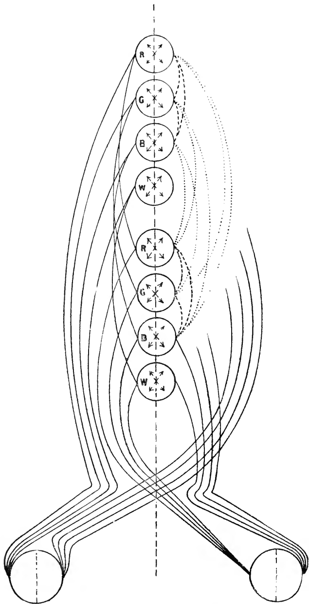
Fig. 75. Diagram representing the two retinae and the cortical centres connected with them. The upper four circles represent the cortical levels of the red, green, blue, and white systems connected with the left retina, the lower four those connected with the right retina. The broken line bisecting all the circles represents the purely anatomical separation of each centre into two halves lying in opposite cerebral hemispheres. The continuous lines on the left side represent the sympathetic relation between corresponding points of the two systems of similar function connected with the right and left retinae respectively. The dotted lines represent the antagonism between any point of any one colour-system of the one eye and the corresponding points of the other two colour-systems of the other eye. The broken lines represent the feebler antagonism between any point of any one colour-system of one eye and the corresponding points of the other two colour-systems of the same eye. The arrows radiating from the centre of each circle represent the antagonism between any point of the cortical level of any one of the systems and every other point of the same. (McDongall.)
