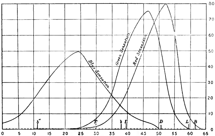
Fig. 64. Abney's R , G , and B equal-area sensation curves. The sums of equal ordinates of the three curves at any point represent the sensation of the unanalysed white light. (Abney.)
