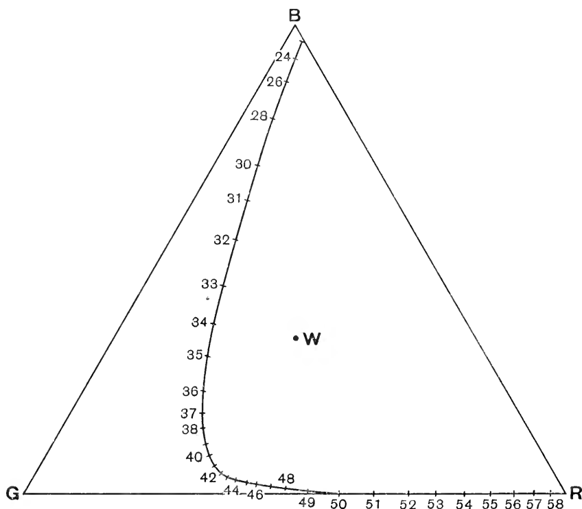
Fig. 9. Colour triangle. W, white; R, red; G, green; B, blue. The numbers are those of an arbitrary scale of the spectrum of the arc light. (Abney and Watson.)
