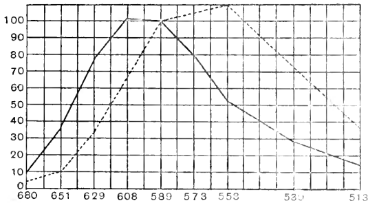
Fig. 53. Photopic peripheral luminosity curves for the normal trichromat (—) and for the protanope (.....). Abscissae, wave-lengths of the prismatic spectrum of gaslight; ordinates, arbitrary scale. (v. Kries.)
