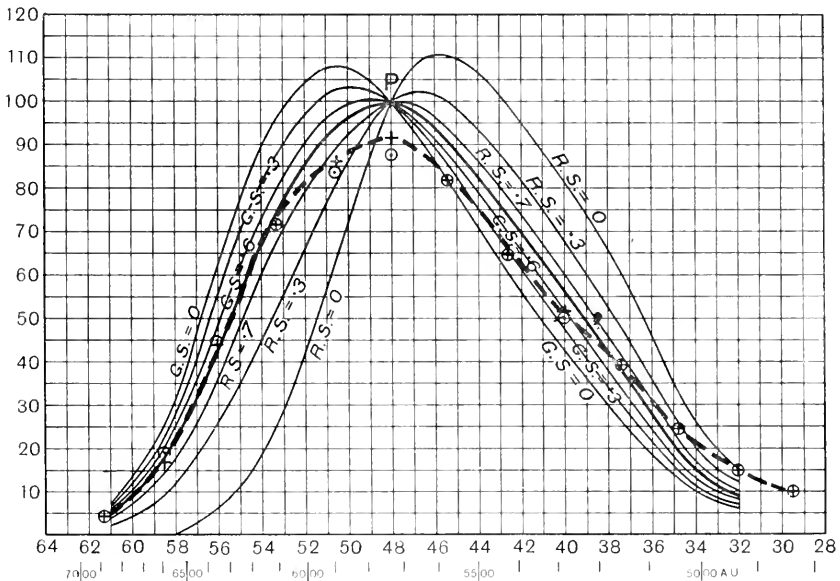
Fig. 70. Luminosity curves of a normal trichomat with subnormal macular pigmentation. + + + foveal; o o o parafoveal. (Watson.)
