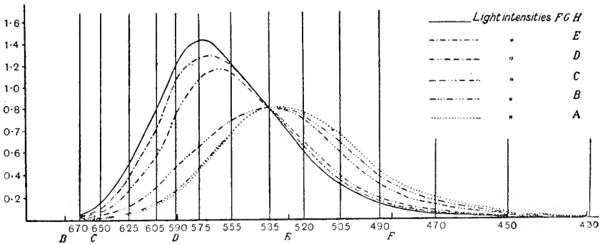
Fig. 47. Protanopic luminosity curves for different intensities of light, A being the lowest, H the highest. Abscissae, wave-lengths of the prismatic spectrum of gas-light; ordinates, arbitrary scale. (König.)
