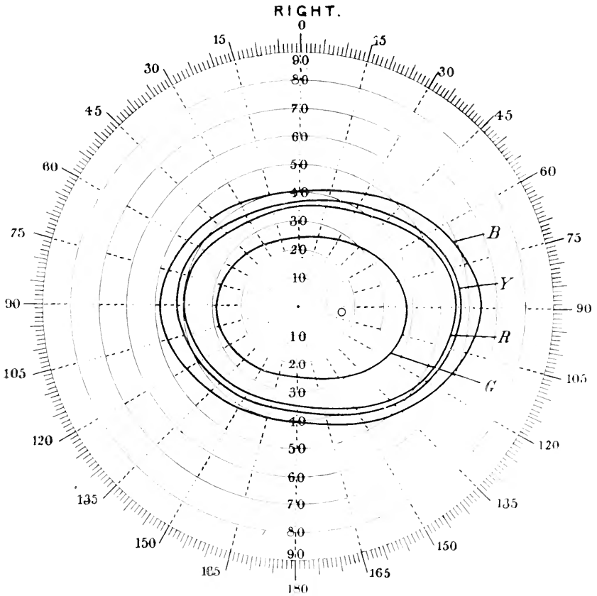
Fig. 28. The fields of vision for spectral colours with moderate illumination ( D light = 3.95 foot-candles at the screen). (Abney.)
