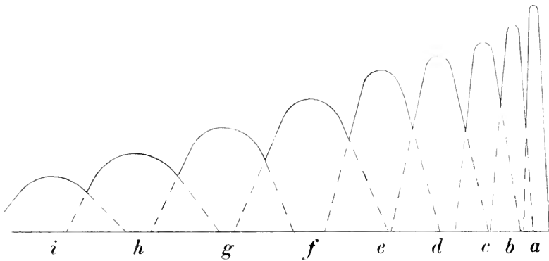
Fig. 36. Diagram illustrating the primary response to a single momentary stimulus. The series of pulses of sensation commences at a and lasts through a period of about \frac{2}{3} sec., represented by a—i . The height to which each curve rises represents the intensity of the pulse of sensation. The effects of a momentary stimulus of less intensity are represented by a part of the series of curves, e.g., e—i . The overlapping of the curves represents the fact that the intervals between the pulses of sensation are not quite dark. (McDougall.)
