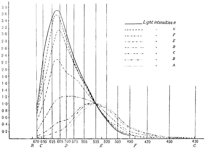
Fig. 10. Normal trichromat's luminosity curves for different intensities of light ( A, B, C, etc. ; A being the lowest, and H the highest intensity). Abscissae, wave-lengths of the prismatic spectrum of gas light ; ordinates, an arbitrary scale. (König.)
