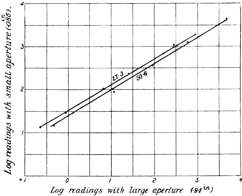
Fig. 41. Equality of brightness curves for different sized apertures. SSN 27.3 = 575 \mu\mu ; SSN 50.6 = D line. (Abney.)
