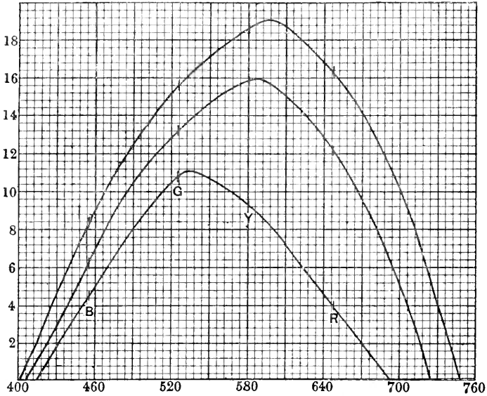
Fig. 17. Luminosity curves determined by the flicker method (critical frequency readings). The upper curve represents a bright spectrum, the lower a dark spectrum, and the middle curve one of intermediate intensity. (Haycraft.)
