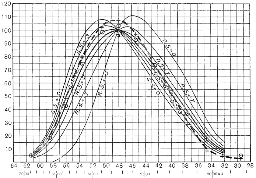
Fig. 69. Luminosity curves of a normal trichromat with excessive macular pigmentation. + + + foveal; o o o parafoveal. (Watson.)
