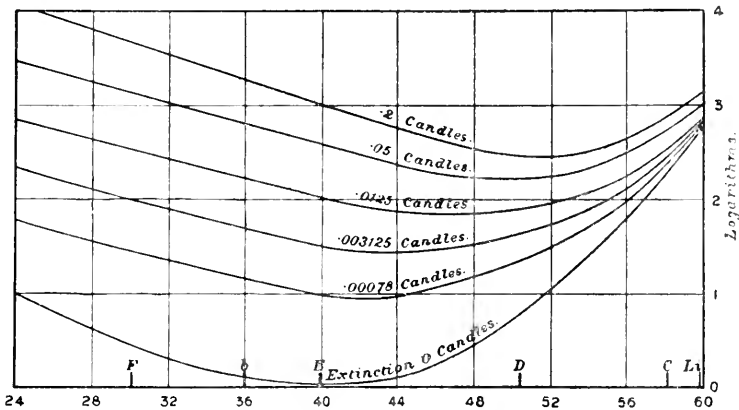
Fig. 22. "Extinction of light" curves for different degrees of light adaptation. Abscissae, wave-lengths; ordinates, logarithms of the intensities of the light. (Abney.)
