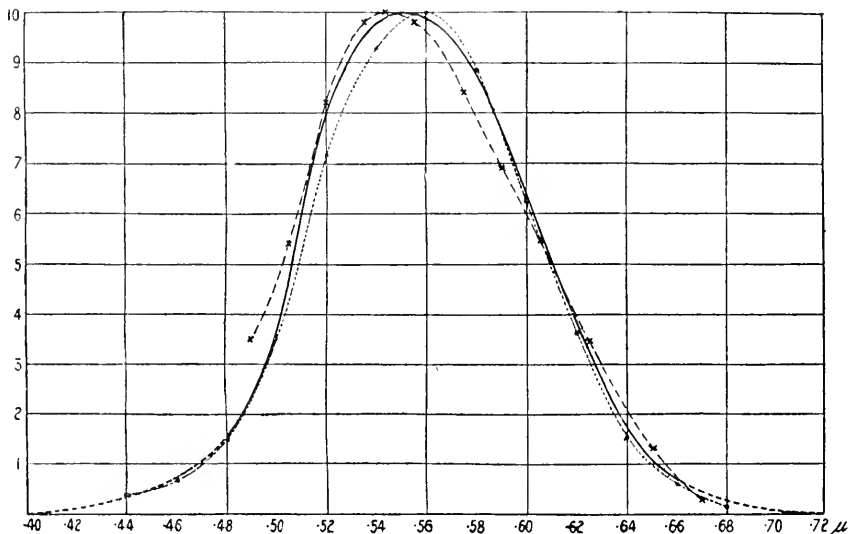
Fig. 39. ———. Average photopic luminosity curve of 18 observers. - - - - - König's photopic luminosity curve (equality of brightness method). ..... Thürmel's photopic luminosity curve (flicker method). (Ives.)
