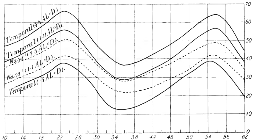
Fig. 31. The temporal and nasal limits of the fields of vision for spectral colours at three different intensities of illumination. (Abney.)
