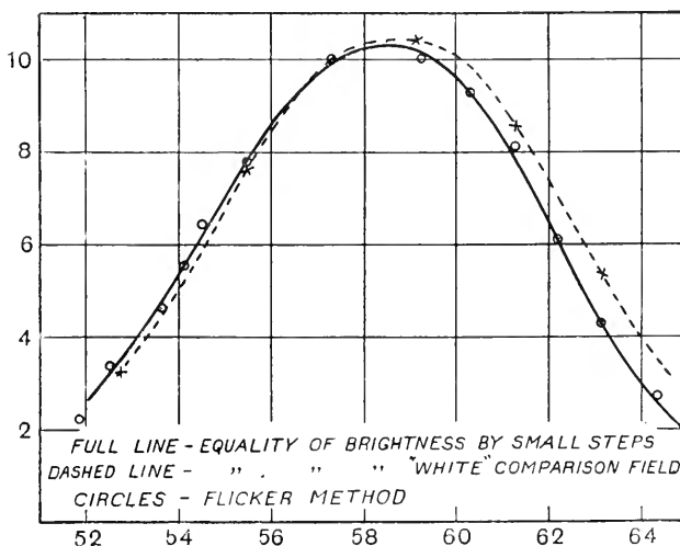
Fig. 38. Photopic luminosity curves taken by the flicker and equality of brightness methods. Abscissae, wave-lengths from 520 \mu\mu to 640 \mu\mu ; ordinates, arbitrary scale. (Ives.)
