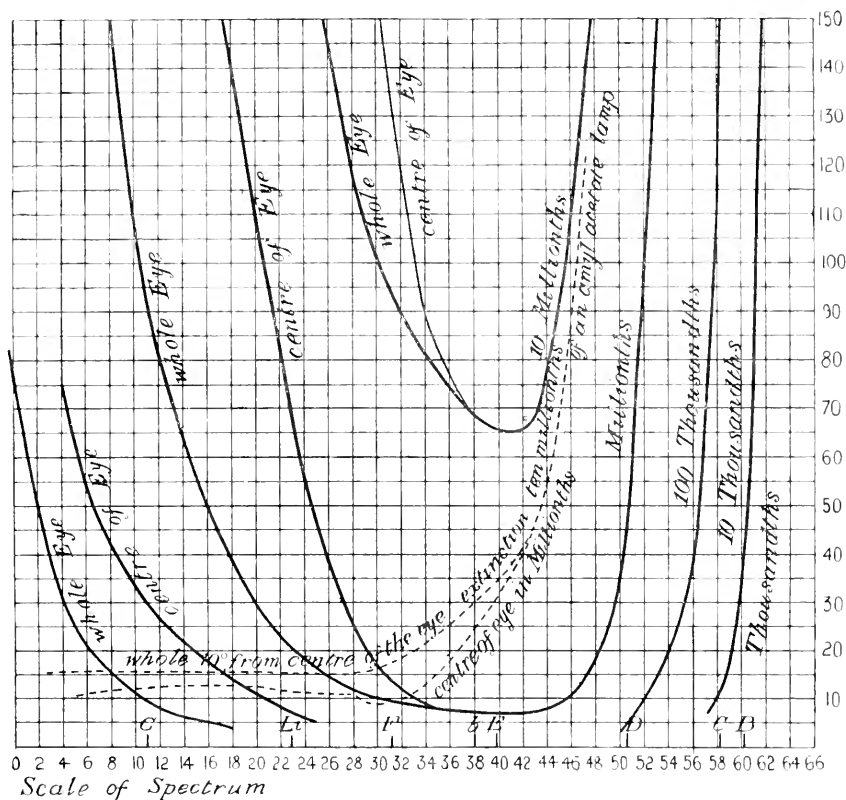
Fig. 20. "Extinction of light" curve. Abscissae, wave-lengths of the prismatic spectrum; ordinates, the fractions of the beams which are just invisible, the unreduced illumination of the D light at the screen being one Hefner-foot (0.9 candle-foot). The dotted lines show the proportion on the assumption that each beam has the same intensity as that of the D light.
