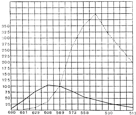
Fig. 25. ——— Photopic luminosity curve for the totally colour-blind peripheral zone of the retina. . . . . Scotopic luminosity curve. Abscissae, wave-lengths of the prismatic spectrum of gas light; ordinates, arbitrary scale. (v. Kries.)
