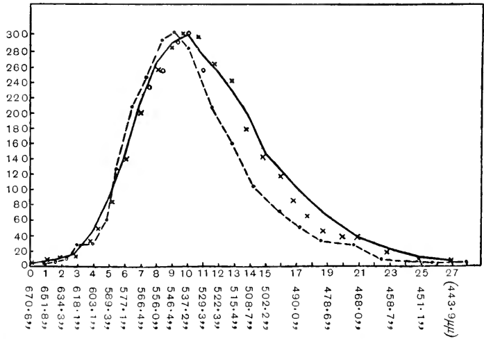
Fig. 15. Scotopic luminosity curves. — Schaternikoff's curve (normal trichromat). - - - Nagel's curve (deuteranope). x x x x and o o o o, other observations by Nagel. Abscissae, wave-lengths of the prismatic spectrum of gas light; ordinates, arbitrary scale. (Schaternikoff.)
