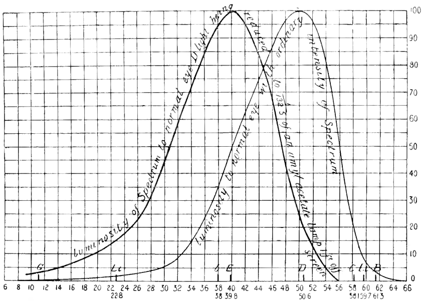
Fig. 14. Normal trichromat's photopic and scotopic luminosity curves. (One amyl acetate or Hefner unit is equal to 0.9 international candle power.) Abscissae, arbitrary scale of the prismatic spectrum of the arc light; ordinates, arbitrary scale, the maximum of luminosity being in each case 100. (Abney and Festing.)
