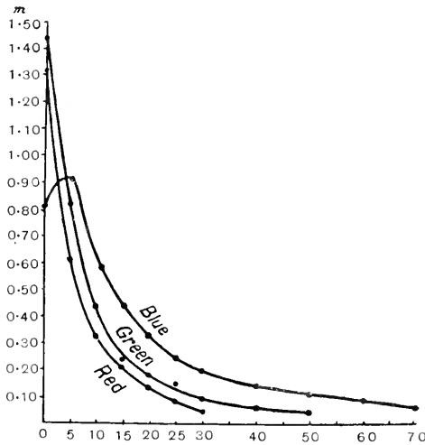
Fig. 24. Perception of colours in different parts of the field of vision. Abscissae, degrees to the nasal side of the fovea ( O ); ordinates, maximum distance at which the colour is perceptible in a coloured paper 2 mm. square. (Charpentier.)
