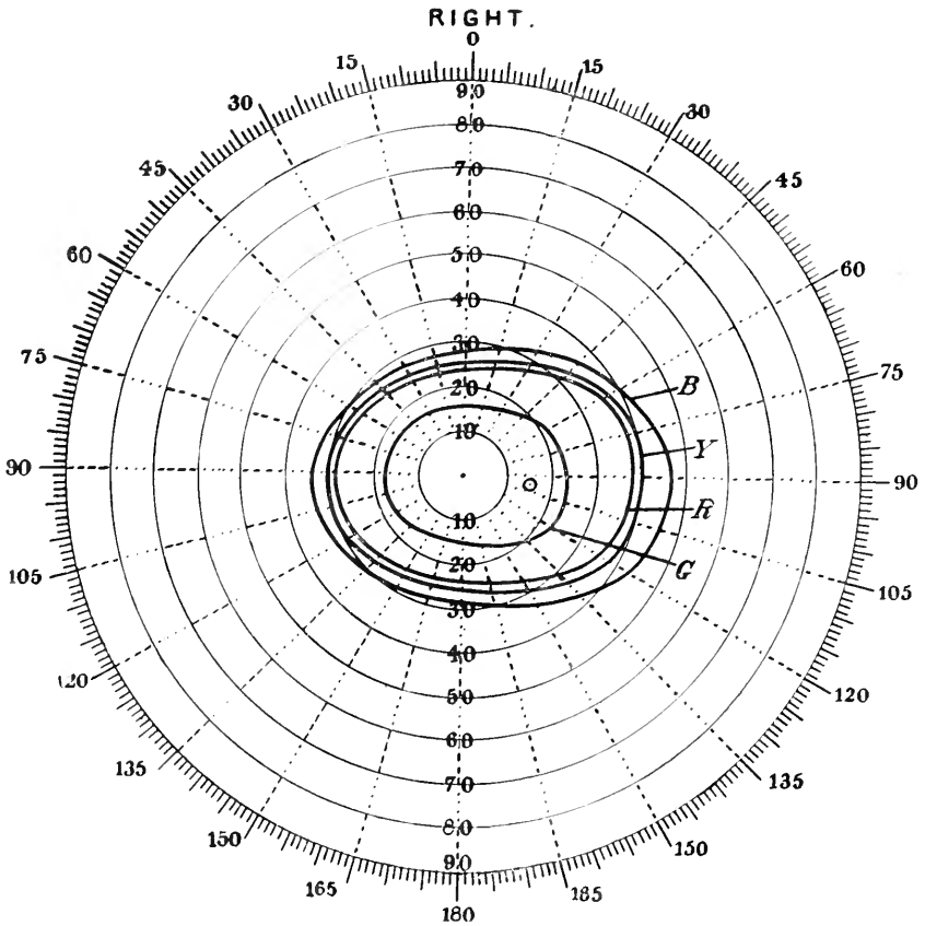
Fig. 29. The fields of vision for spectral colours with low illumination ( D light — 0.21 foot-candle at the screen). (Abney.)
