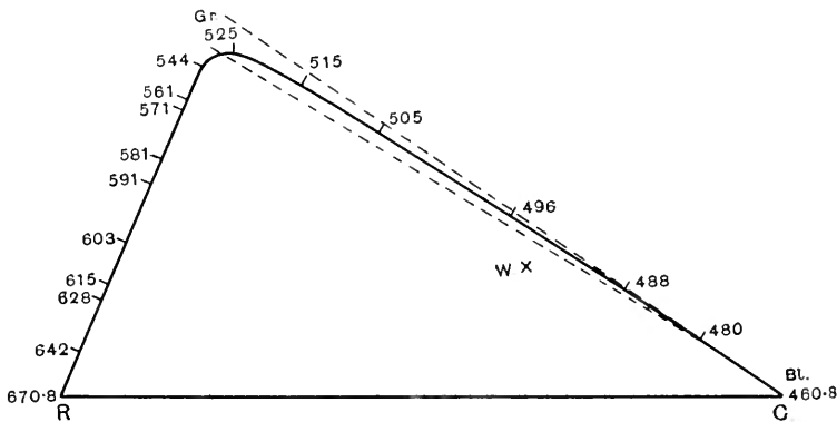
Fig. 57. Normal trichromatic colour diagram constructed from combined protanopic and deuteranopic observations. A , null-point of protanopes; B , null-point of deuteranopes. (v. Kries.)
