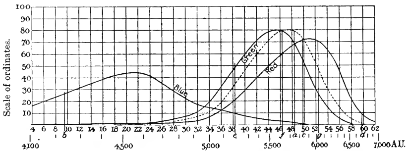
Fig. 74. Normal sensation curves on equal area scale. (Abney and Watson.)
