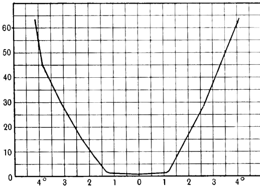
Fig. 13. Sensibility of the fovea and parafoveal region for mixed bluish-white light. Abscissae, to the left of zero degrees to the temporal, to the right, degrees to the nasal side of the fovea (0); abscissae, arbitrary scale. (Breuer and Pertz.)
