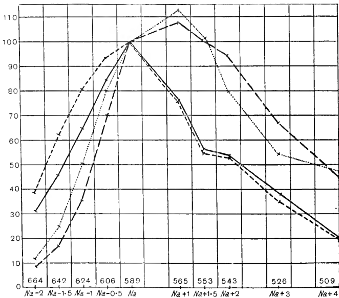
Fig. 50. . . . . Photopic luminosity curve of a protanope (flicker method). — — — Periphery luminosity curve of the same protanope. - - - - Photopic luminosity curve of a trichromat (flicker method). ————— Periphery luminosity curve of the same trichromat. (Polimanti.)
