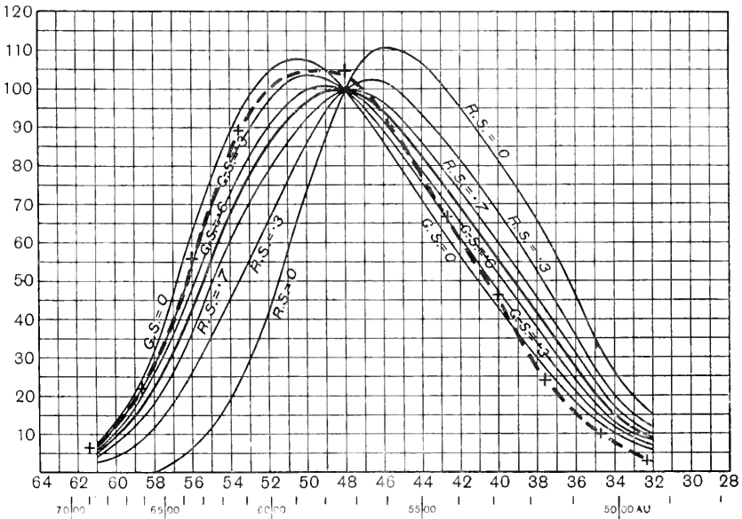
Fig. 72. Foveal luminosity curve of a deuteranope with excessive macular pigmentation. (Watson.)
