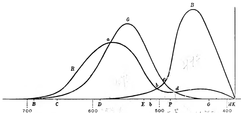
Fig. 60. R , G , and B , sensation curves. These are König and Dieterich's curves corrected to new determinations of the points of section, a , b , c , d . Abscissae, wave-lengths of the interference spectrum of the arc light; ordinates, arbitrary scale. (F. Exner.)
