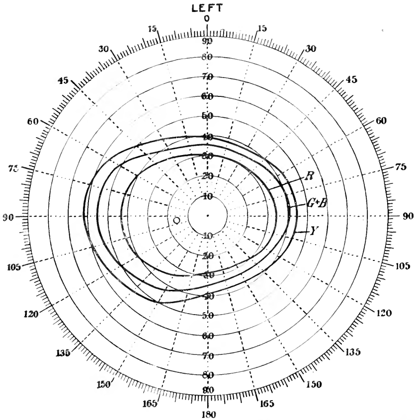
Fig. 30. The fields of vision for complementary spectral colours. The relative luminosities of the red and green were 225 and 270 ; those of the yellow-green and blue 96.5 and 21.5. (Abney.)
