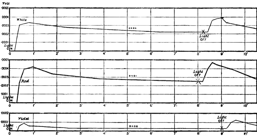
Fig. 2. Electrical changes in the frog's eye caused by light. Plotted curves from the analyses of three capillary electrometer records. The illumination in the case of the upper record was white light, in that of the middle red light, and in that of the lowest violet light. Abscissae, time after the commencement of the illumination in seconds; ordinates, the electromotive force in ten thousandths of a volt. (Gotch.)
