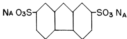
DISODIUM FLUORENE-2,7-DISULFONATE
