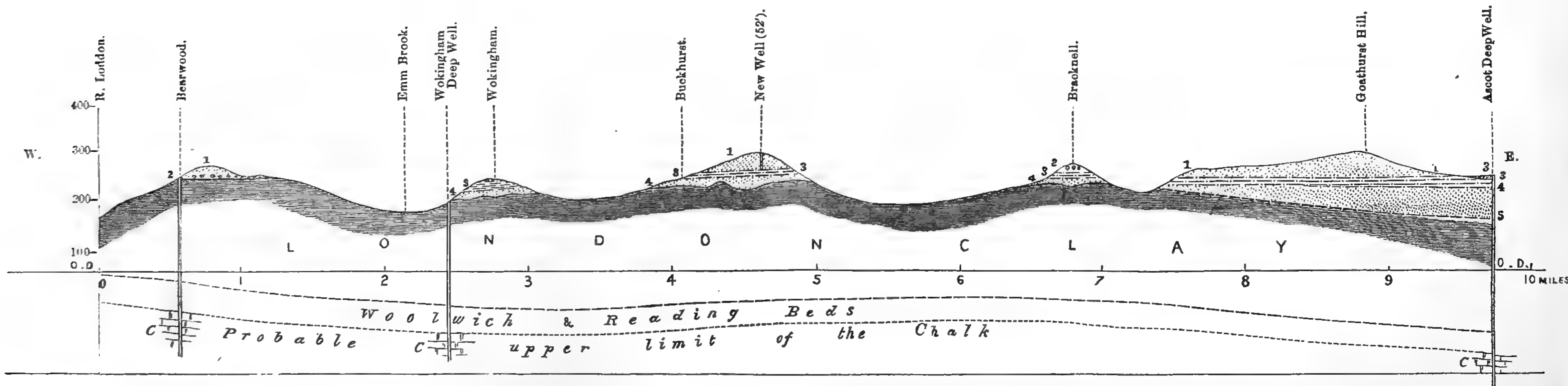
Fig. 2.—Horizontal Section from the River Loddon to Ascot Race-course.
