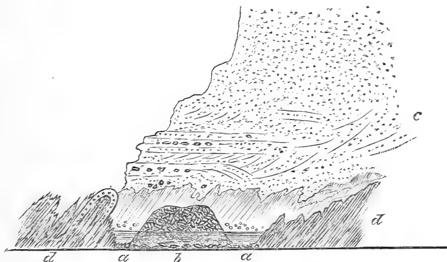
Fig. 5.— Boulder of Grey Porphyry at base of Cliff South of Saunton Down, North end of Barnstaple Bay (April 11, 1887). (Scale 7\frac{1}{2} feet to 1 inch.)
