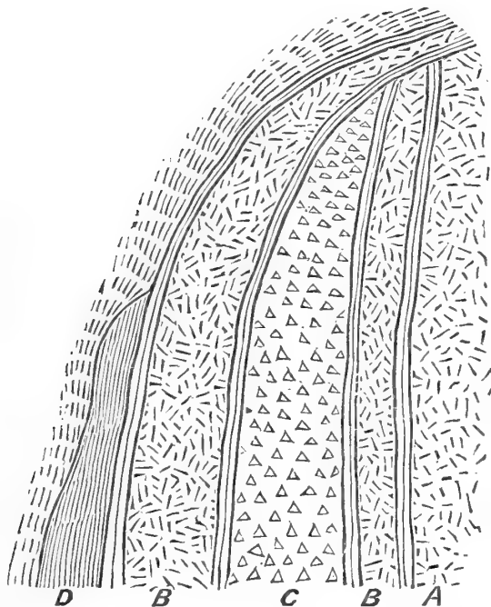
Fig. 3.— Plan of Vein-structure in Schistose Rocks.
