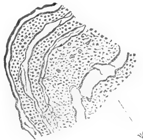
Fig. 1 A.— Small portion of one of the Contortions shown in Fig. 1, about 8 inches in diameter, showing the quartz-felspar bands with occasional cracks parallel with cleavage, the dotted part being the more cleaved micaceous bands.
