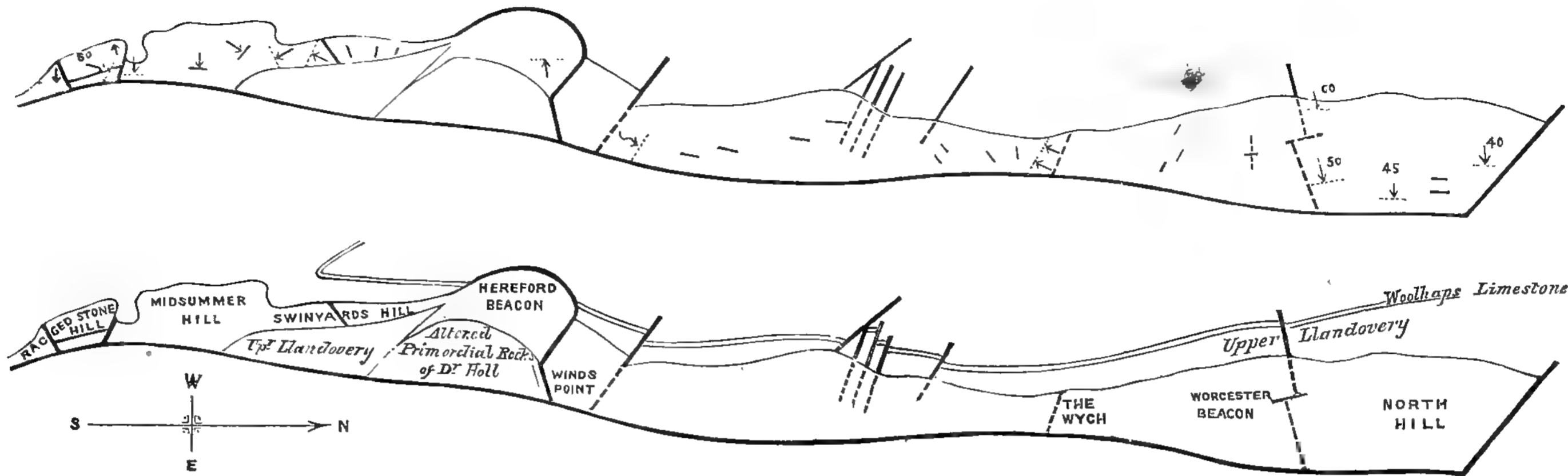
Fig. 2.—General Plan of the Malvern Range, indicating Localities and Faults. (Scale 1 inch to a mile.)
