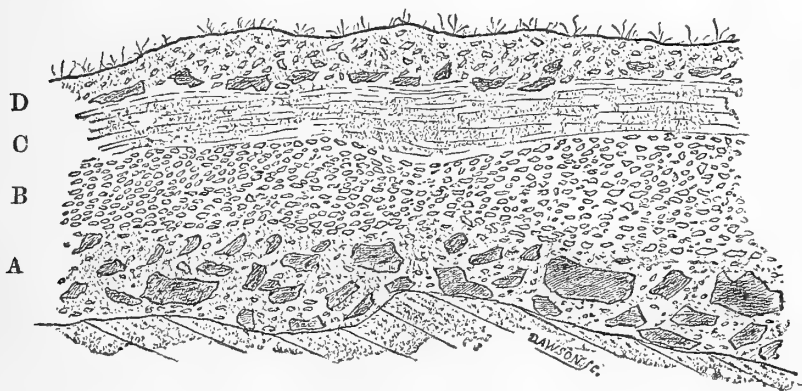
Fig. 2.—Section at Stopham Bridge.
