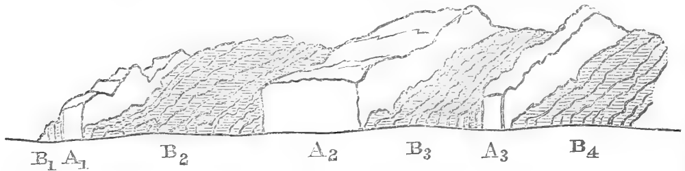
Fig. 4.— At Roscoff. (Length about 7 feet.)
