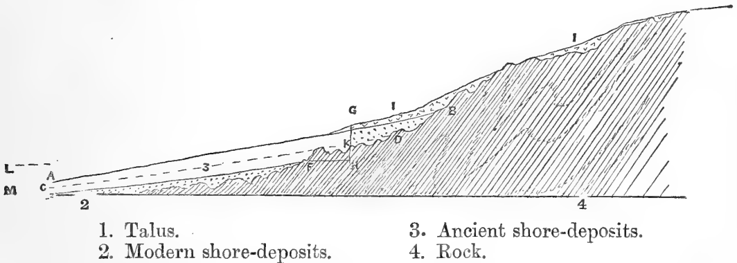
Fig. 1.— Diagram Section showing the Mode of Formation of some of the High-level Beaches of Devonshire.
