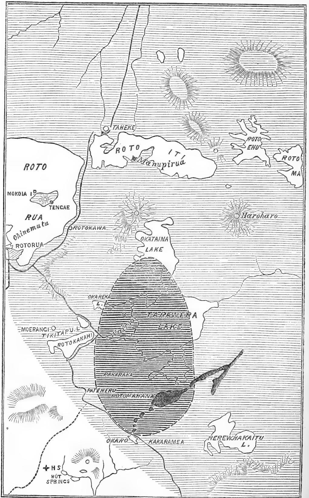
Fig. 2.—Map of the country around Tarawera Volcano after the Eruption of 10th June, 1886. (Scale 5 miles to 1 inch.)
