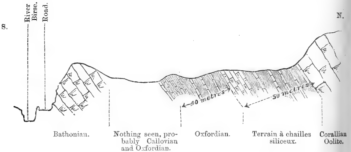
Fig. 1.—Section in Quarry near Roadside, south-east of Liesberg.
