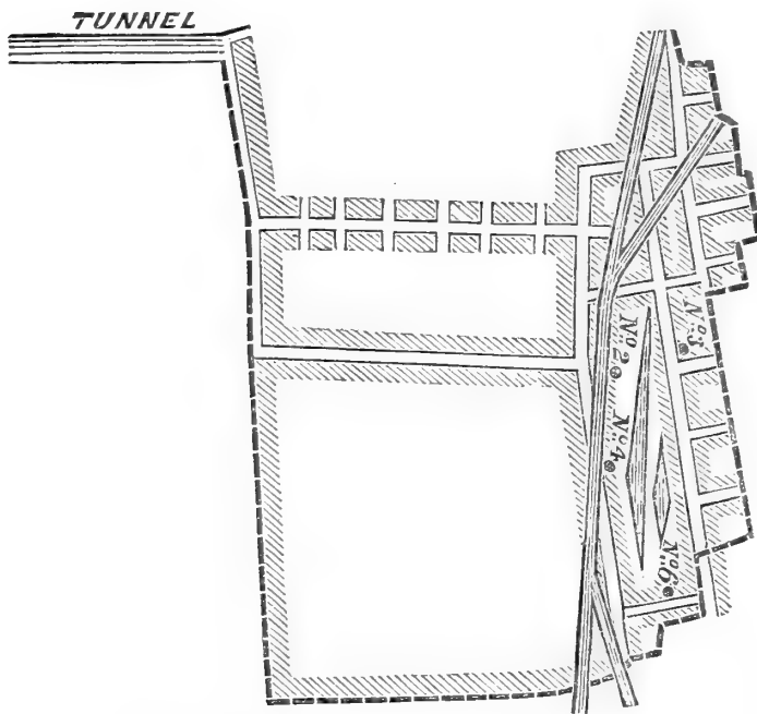
Fig. 1.— Plan of the Roger Mine, Dukinfield. (Scale 100 yards to 1 inch.)
