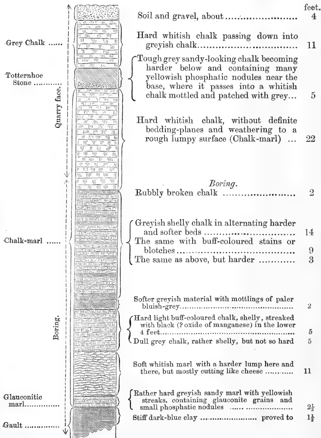
Fig. 3.—Section at Stoke Ferry, partly seen in the quarry, and partly proved by boring. (Scale \frac{1}{20} inch to 1 foot.)
