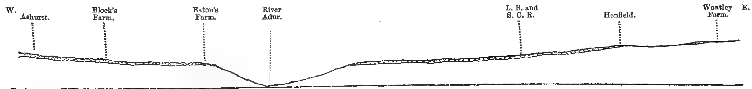
Fig. 13.—Section from Ashurst to Henfield, across the Adur Valley. (Horizontal scale, \frac{1}{21120} . Vertical scale, \frac{1}{2400} .)
