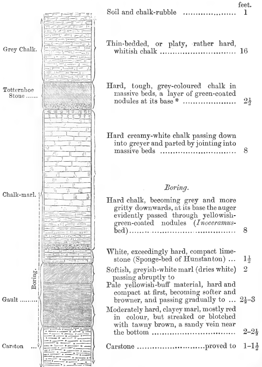
Fig. 4.— Diagram of the section shown and obtained by boring in the Dersingham Parish Chalk-pit. (Scale \frac{1}{8} inch to 1 foot.)
