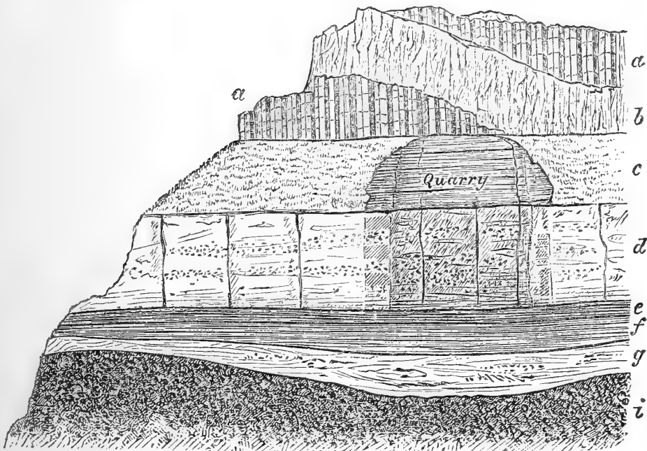
Fig. 3.—Quarry in east side of Ravine, Ardtun Head.
