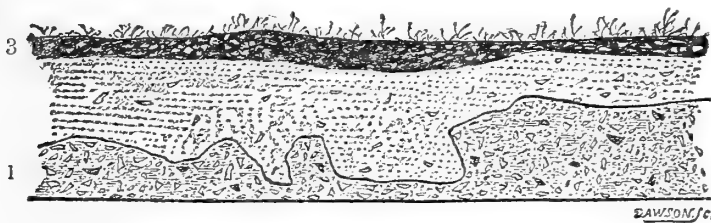
Fig. 4.—Section on Sullington Common.
