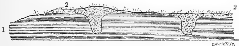
Fig. 7.—Section at Inholmes Farm.
