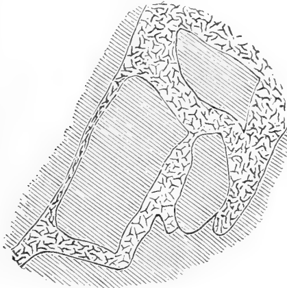
Fig. 1.— Section of Granite in Jointed Diorite.
