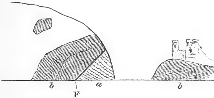
Fig. 3.—Cliff opposite the Old Castle near Salcombe.
