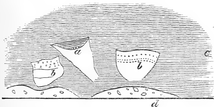
Fig. 1.—Diagram-Section seen at bend of River Elwy, near Dol.
