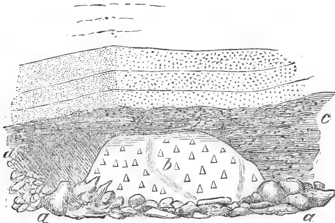
Fig. 6.— Boulder of Red Granite in base of Ancient Beach South of Saunton Down, North end of Barnstaple Bay (April 11, 1887). (Scale 7\frac{1}{2} feet to 1 inch.)
