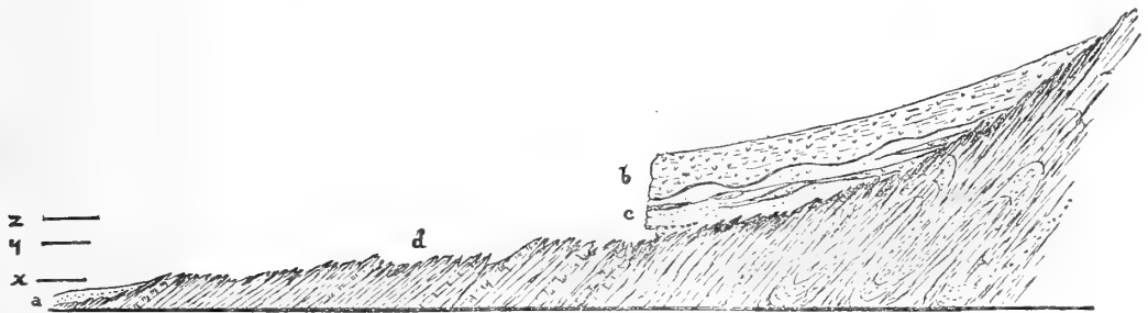
Fig. 3.—Diagram Section across so-called Raised Beach under Saunton Down, North end of Barnstaple Bay. (Scale 200 feet to 1 inch.)
