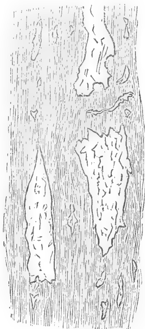
Fig. 3.— Small intrusions of Coarse Granite in a Micaceous Gneiss, both showing effects of pressure. Near the Ferry House, Belon River. (Size about 6\frac{1}{2} by 2\frac{1}{2} feet.)
