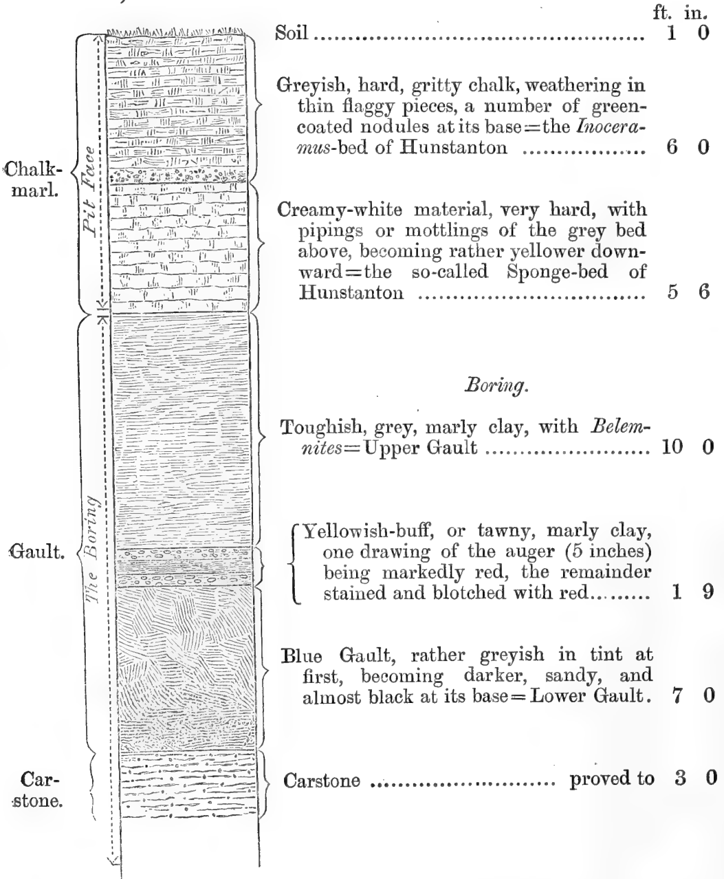
Fig. 2.—Diagram of Section shown and obtained by boring in the Pit about \frac{1}{2} mile N.N.E. of Roydon Church. (Scale \frac{1}{8} inch to 1 foot.)
