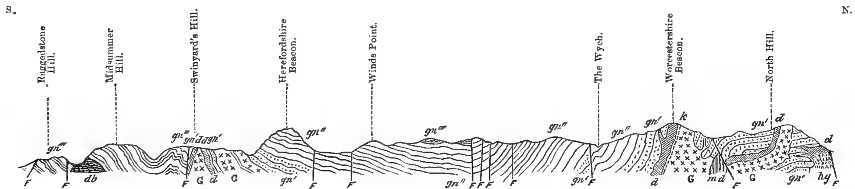
Fig. 3.—Diagrammatic Section from South to North, through the Malvern Hills.
