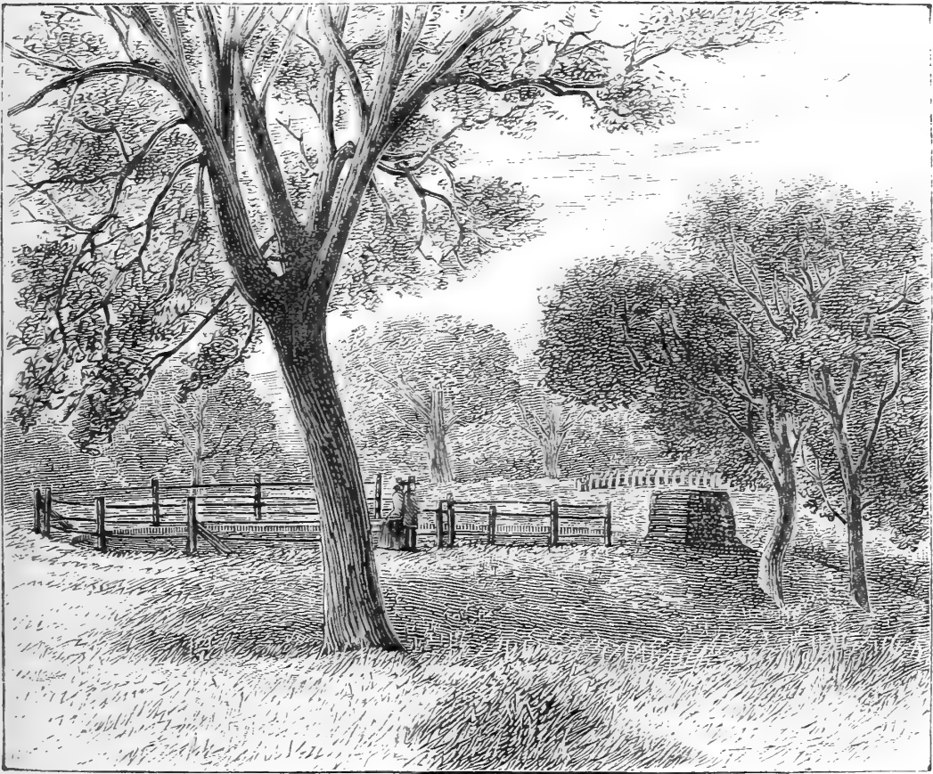
Fig. 5.—View of Old Fence, Ffynnon Beuno.
