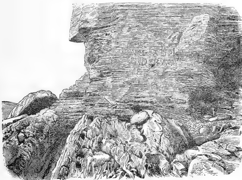
Fig. 4.—Cliff of Consolidated Sand resting on Cleaved Rock (Pilton Beds), Saunton Down, North Devon.
