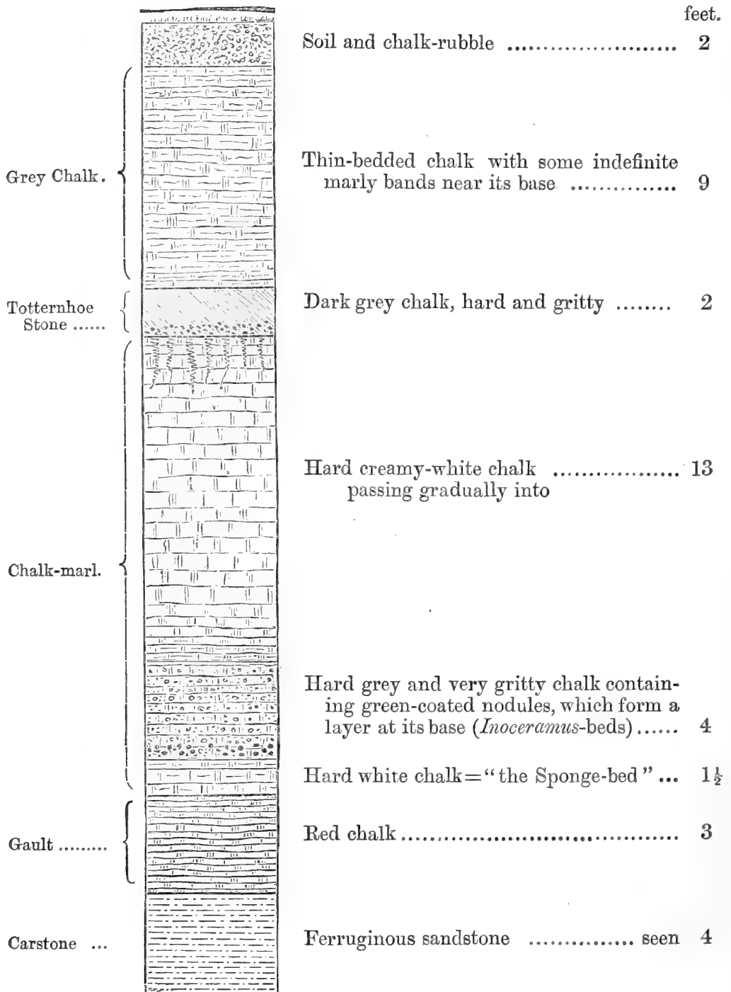
Fig. 5.—Section of Cliff near the Lighthouse at Hunstanton. (Scale \frac{1}{8} inch to 1 foot.)
