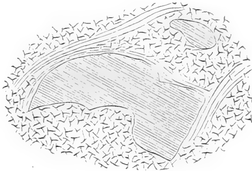
Fig. 3.— Section of Diorite in foliated Granite.
