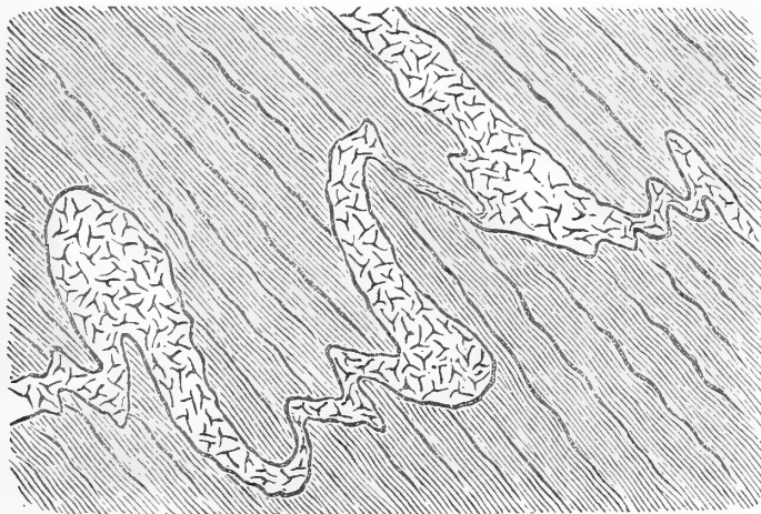
Fig. 1.— Contorted Granite-vein in Gneiss.
