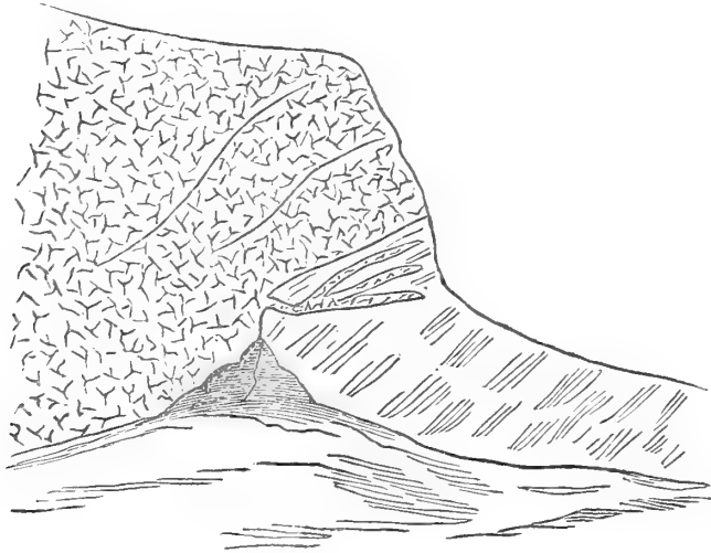
Fig. 5.— Rough sketch of Granite overlying Hornblende-schists at south-east junction on Little Sark. Schists perfectly bedded, dipping S.W.
