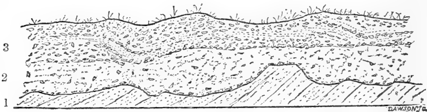
Fig. 5.—Section at Cootham Firs.
