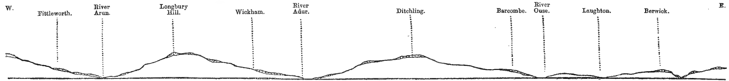
Fig. 10.—General Section across the River-Valleys. (Horizontal scale, \frac{1}{253440} . Vertical scale, \frac{1}{9800} .)
