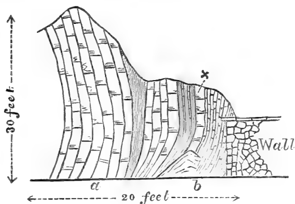
Fig. 2.—Section in Railway-cutting north of Moutier Station.
