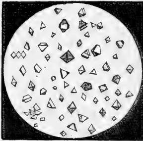
Crystals of arsenious acid by sublimation, magnified 20 diameters.
