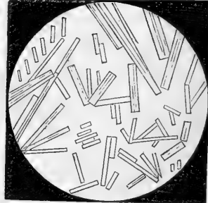
Oxalic acid magnified 30 diameters.
