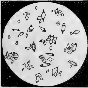
Crystals of morphia, 124 diameters, p. 293.
