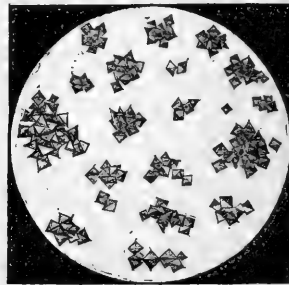
Crystals of arsenious acid, magnified 124 diameters, p. 203.
