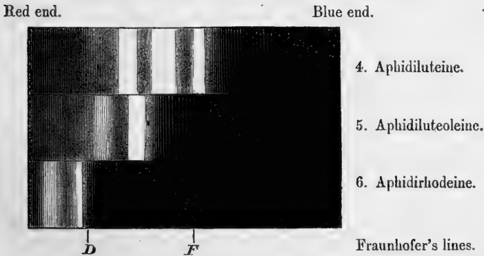
Fig. 2.—Spectra of the Light of Fluorescence.
