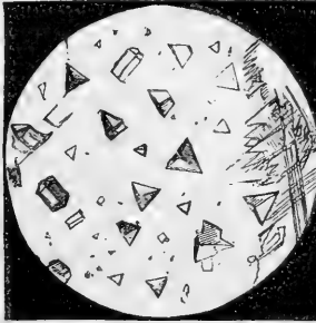
Crystals of tartar emetic magnified 30 diameters, p. 251.
