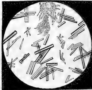
Crystals of daturia, 30 diameters, p. 370.
