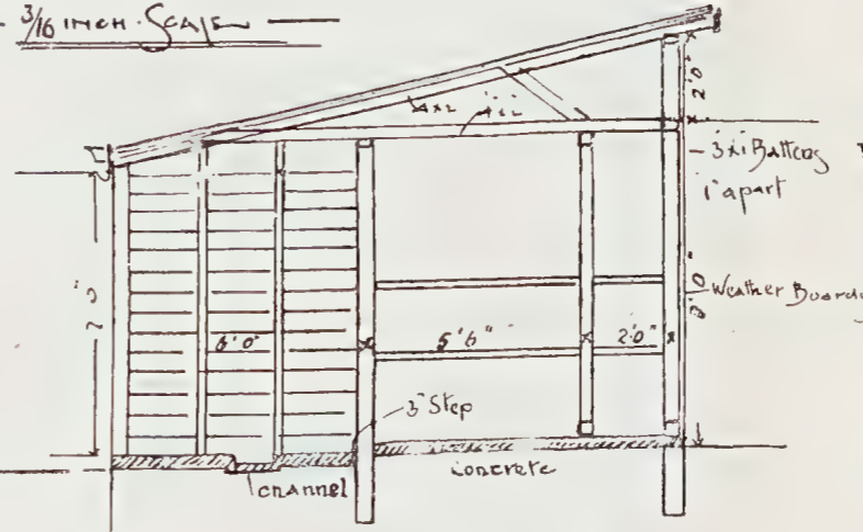
SECTION OF BAILS
