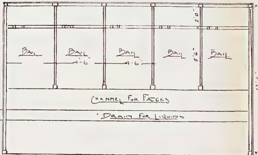
PLAN OF MILKING SHED
