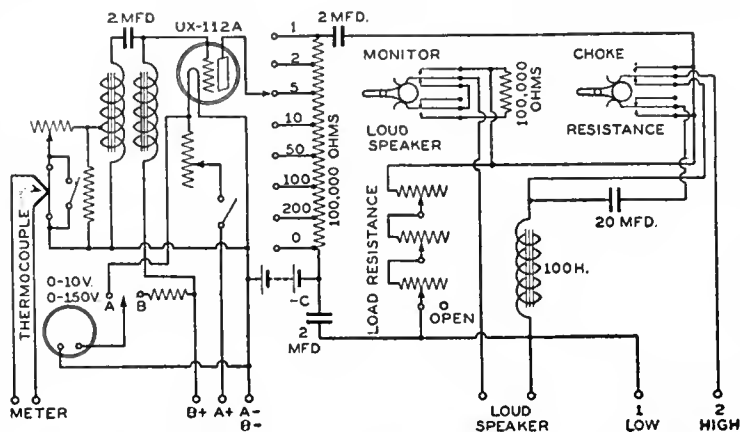
Fig. 1—Circuit of A.F. voltmeter and loading device.
