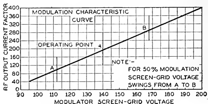
Fig. 2—Modulation characteristic curve.
