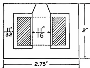
CORE LAMINATION
