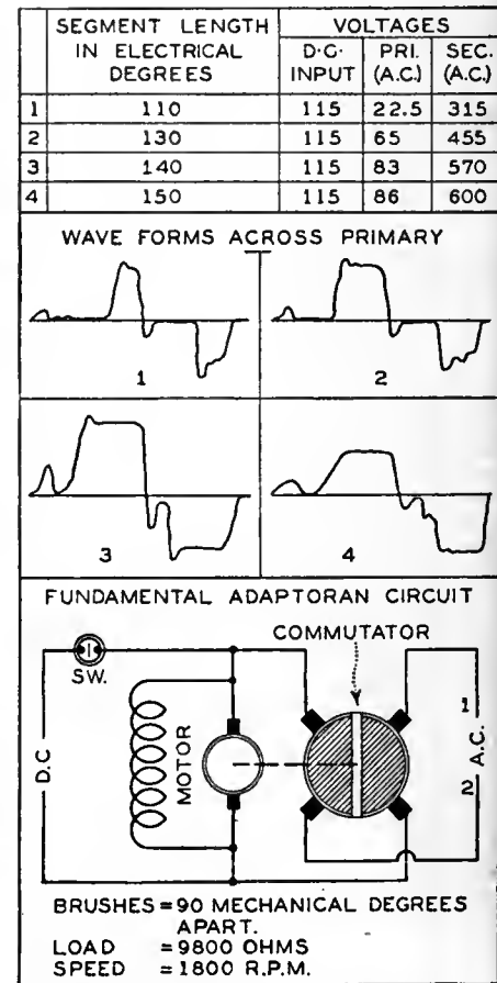
Fig. 4—Effect of varying length of commutator segments.
