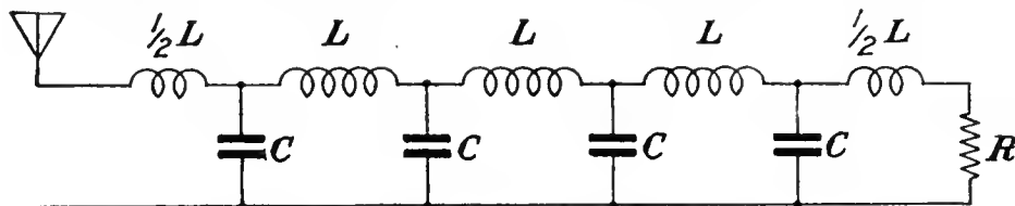
Fig. 1—Circuit arrangement in test where coupling condensers C are grounded and transmission line is terminated in resistor R
