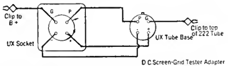
Fig. 2—The a.c. screen-grid tester adapter.
