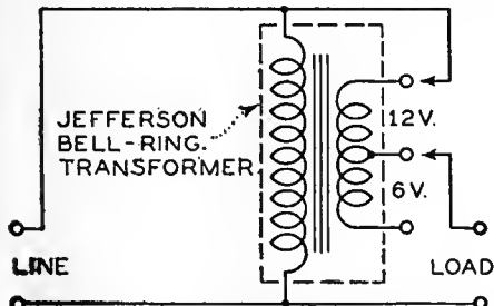
Fig. 2—A somewhat familiar but always practical method of compensating a consistent line variation.
