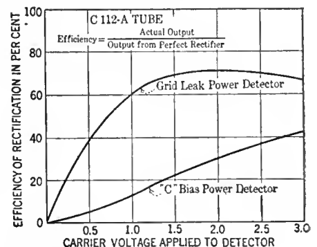
Fig. 2—Efficiency of rectification as a function of the input voltage.
