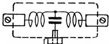
Fig. 9—Fundamental circuit arrangement of a multicoupler.
