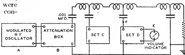
Fig. 14—Method of determining amount of interaction between receivers.
