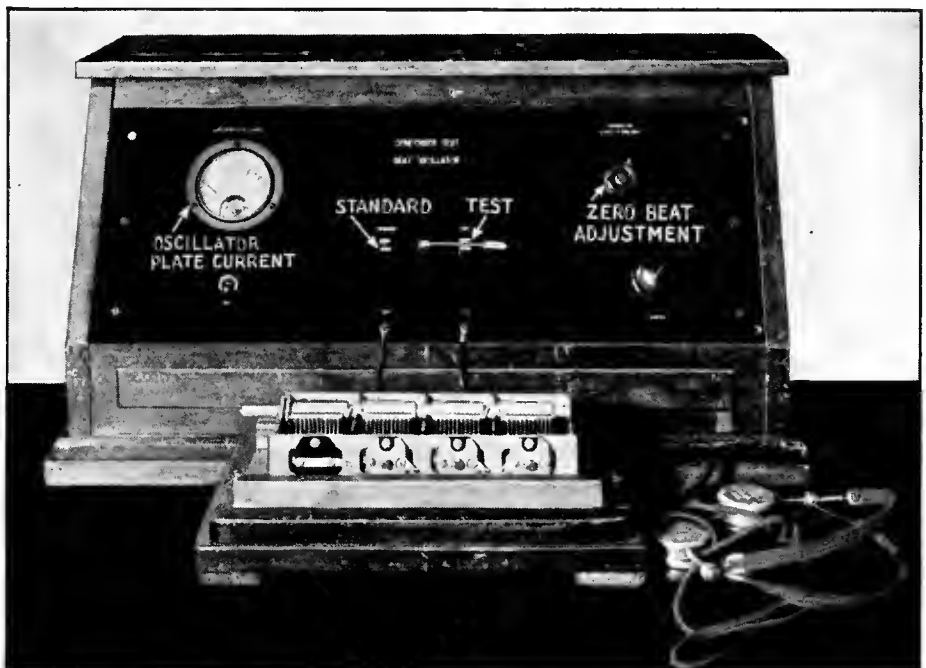
A machine for production testing of coupling condensers.
