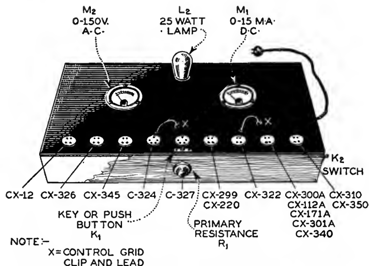
The arrangement of tube sockets, meters, voltage control, etc., of the tube-tester is indicated in this panel layout.
