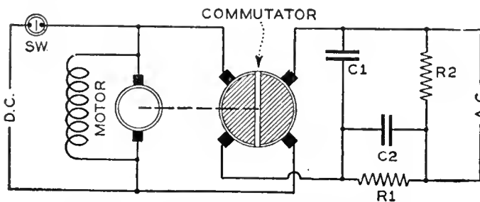
Fig. 1—The neon-tube Adaptoron circuit.
