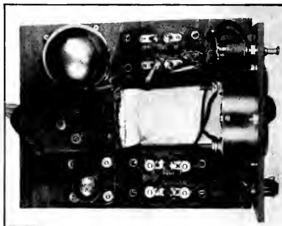
Baseboard view of output meter.
