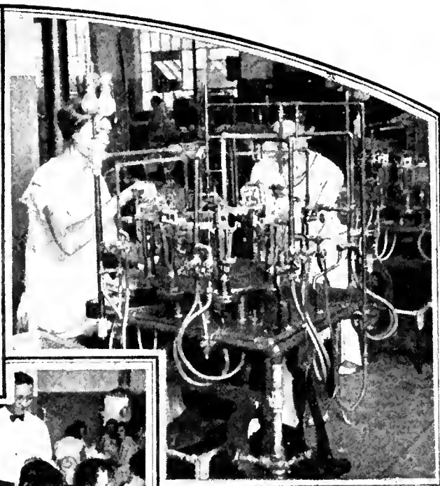
Stem forming machine. (Left) Mounting vacuum tubes.
